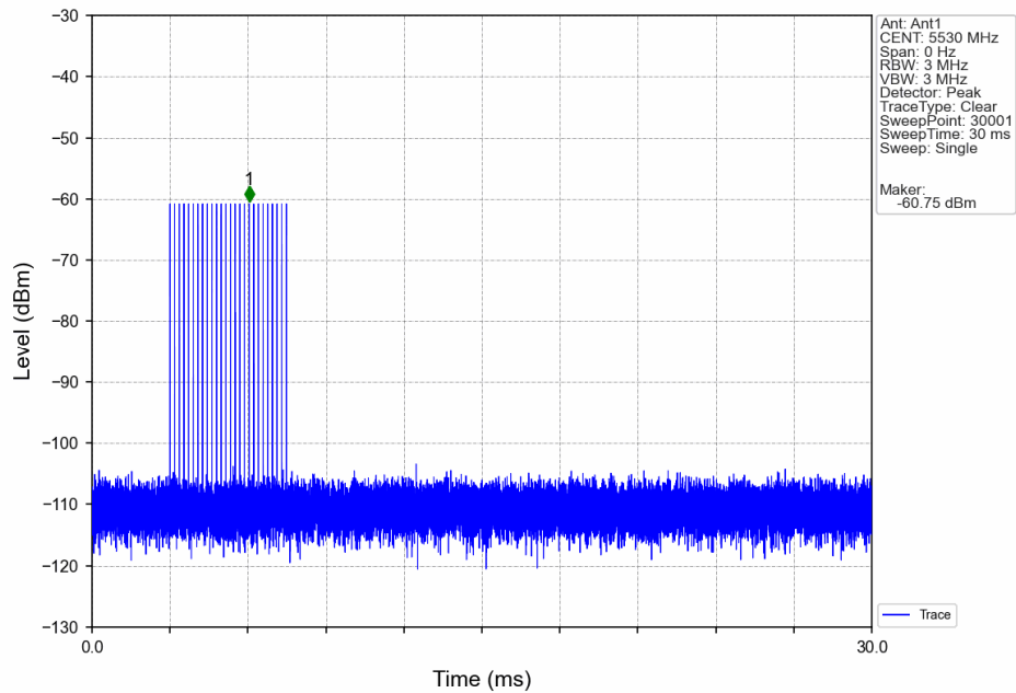
Signal Calibration_802.11ac(VHT80)_2C_5530MHz_RadarType3_Trial0
