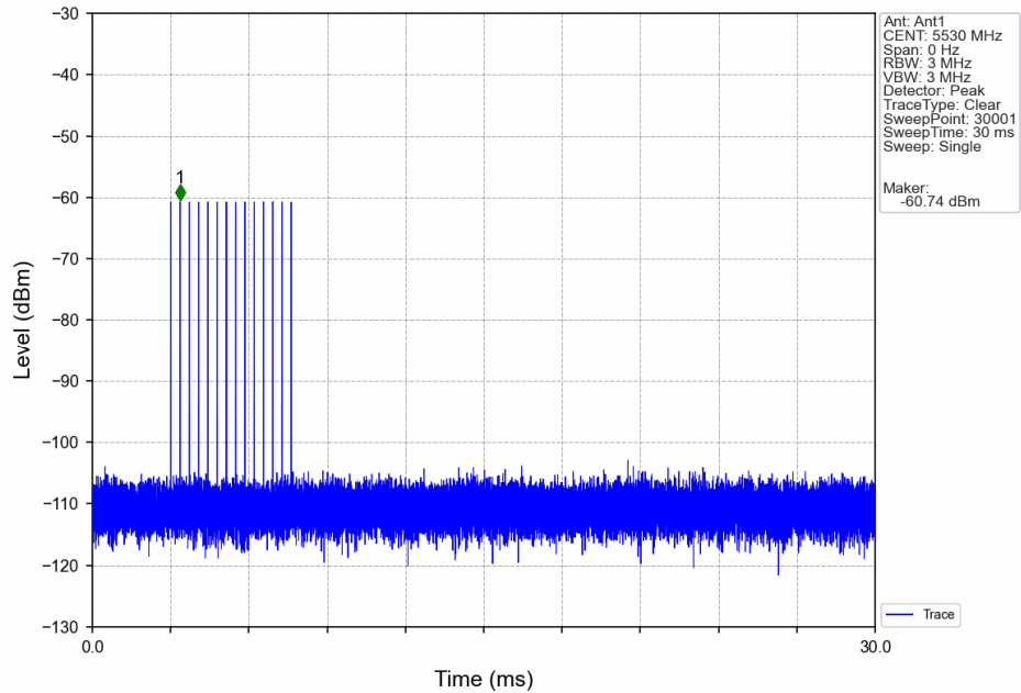
Signal Calibration_802.11ac(VHT80)_2C_5530MHz_RadarType5_Trial0
