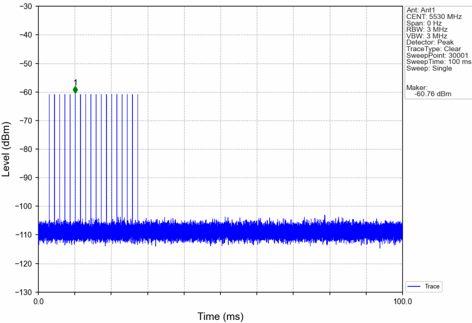
Signal Calibration_802.11ac(VHT80)_2C_5530MHz_RadarType1_Trial0
