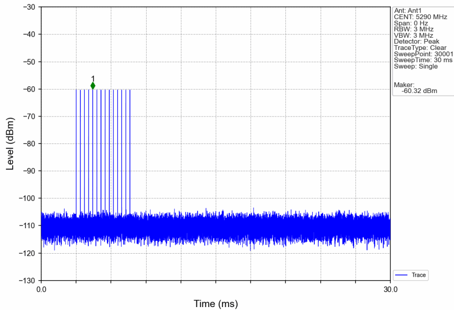
Signal Calibration_802.11ac(VHT80)_2A_5290MHz_RadarType5_Trial0
