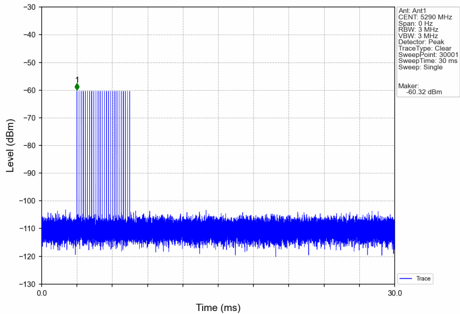
Signal Calibration_802.11ac(VHT80)_2A_5290MHz_RadarType3_Trial0
