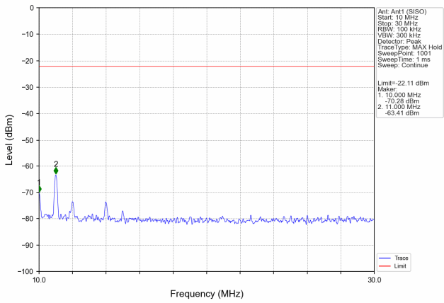
Mode: TX 11b channel 1
