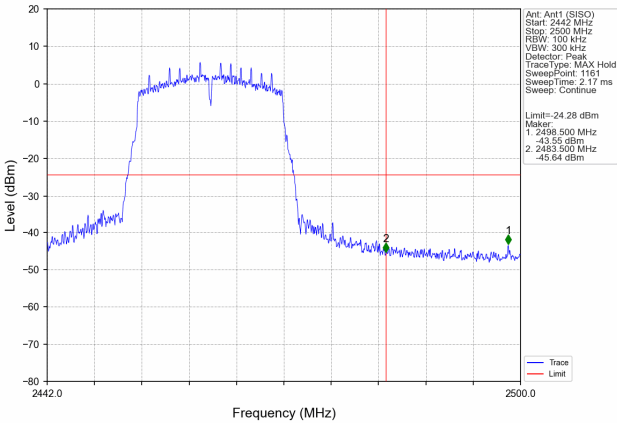
TX 11n HT20: Band edge-right side
