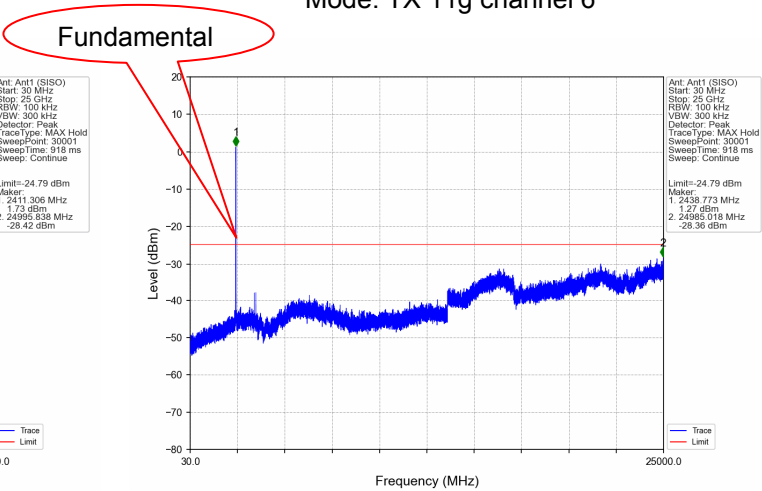
Mode: TX 11g channel 6
