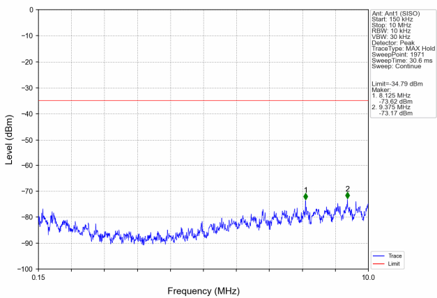
Mode: TX 11g channel 11
