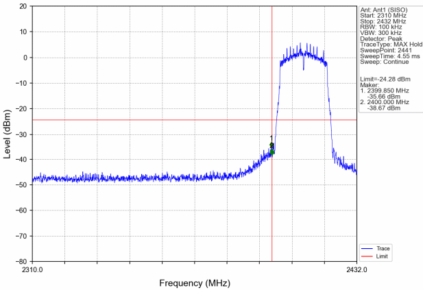
TX 11n HT20: Band edge-left side
