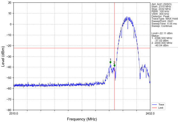
TX 11b: Band edge-left side
