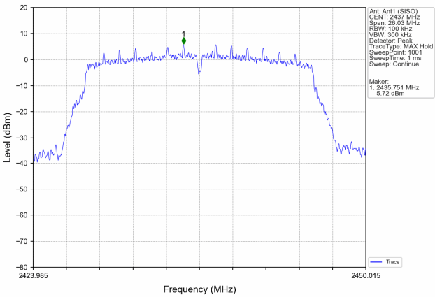
Mode: TX 11n HT20
