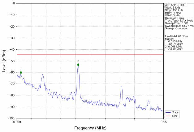
Mode: TX 11n HT20 channel 1
