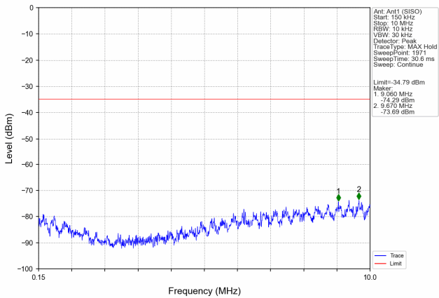
Mode: TX 11g channel 1
