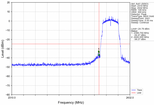
TX 11g: Band edge-left side
