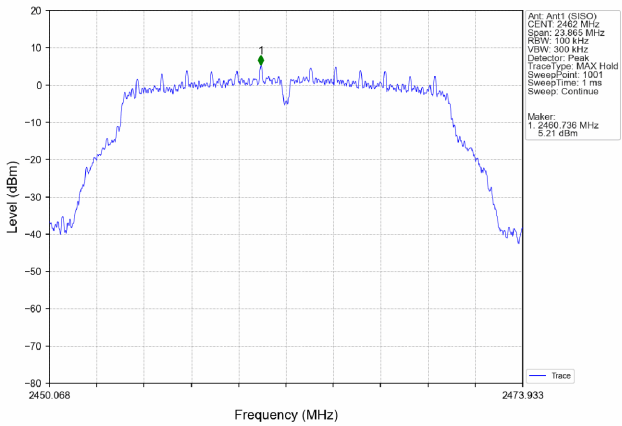
Mode: TX 11g
