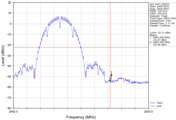
TX 11b: Band edge-right side
