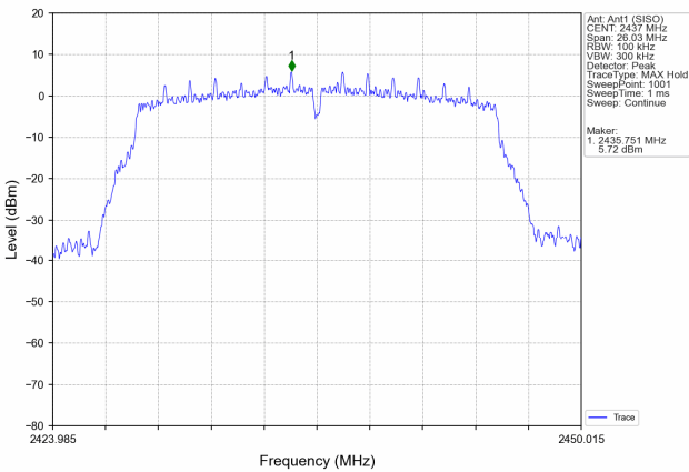
Mode: TX 11n HT20
