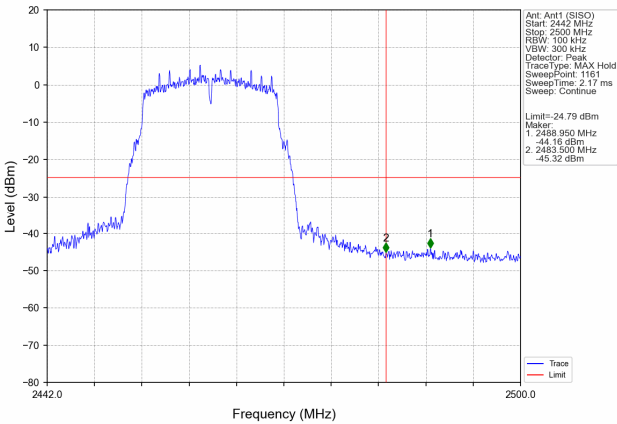
TX 11g: Band edge-right side
