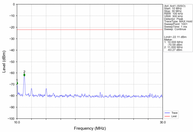
Mode: TX 11b channel 11
