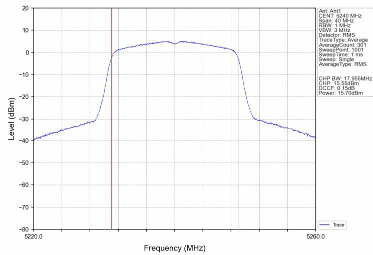
802.11ac(VHT20) U-NII-1 High channel
