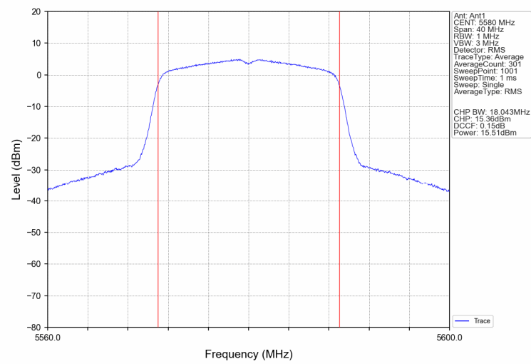
802.11n(HT20) U-NII-2C Middle channel
