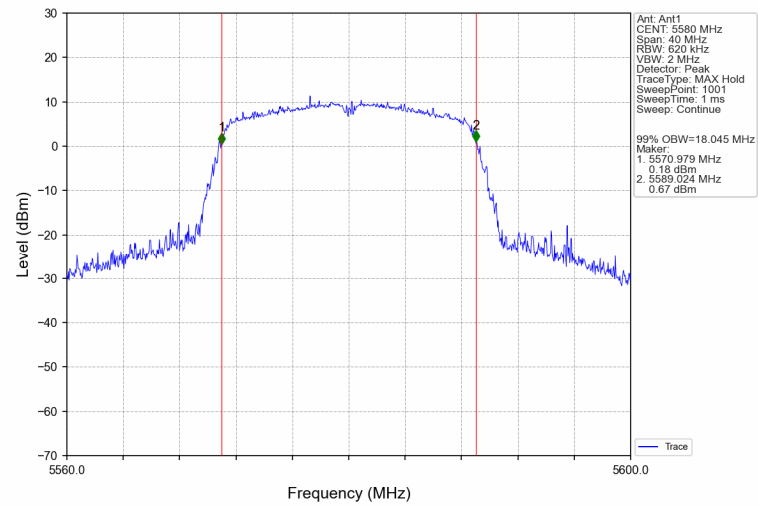
802.11ac(VHT20) U-NII-2C Middle channel
