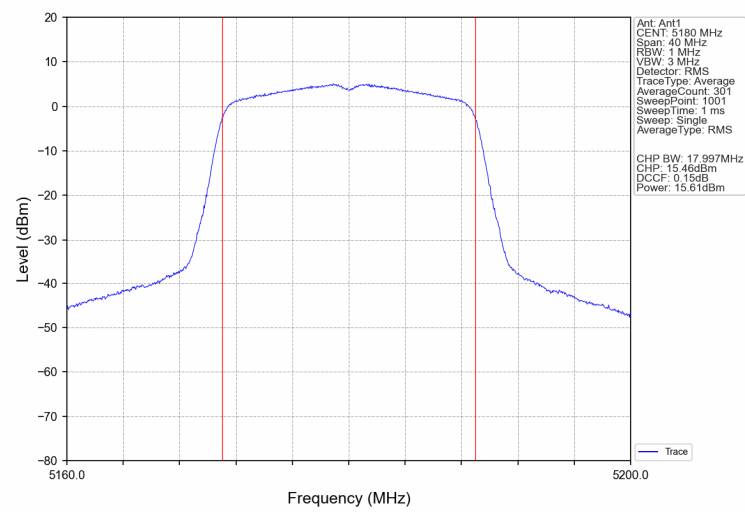
802.11n(HT20) U-NII-1 Low channel
