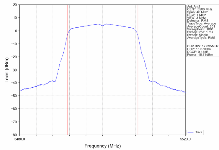
802.11a U-NII-2C Low channel
