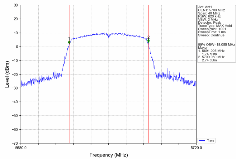
802.11ac(VHT20) U-NII-2C High channel
