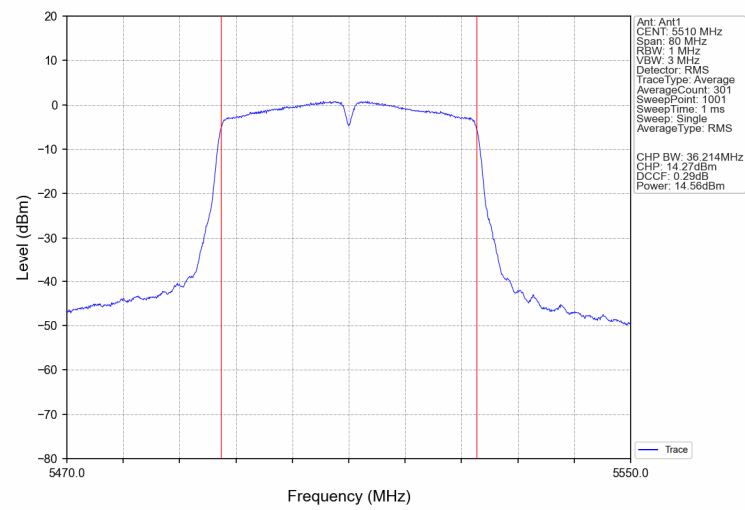
802.11n(HT40) U-NII-2C Low channel
