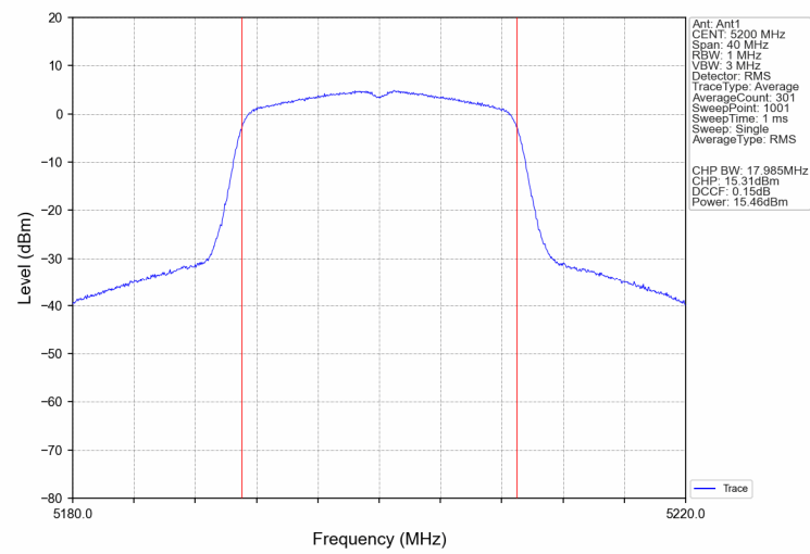
802.11n(HT20) U-NII-1 Middle channel
