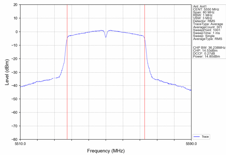
802.11n(HT40) U-NII-2C Middle channel
