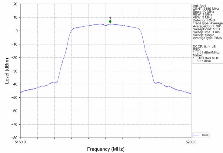
802.11a U-NII-1 Low channel
