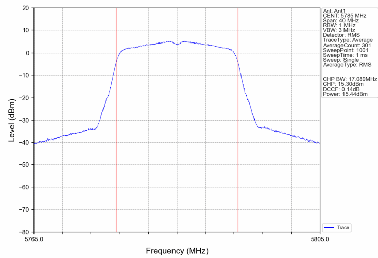
802.11a U-NII-3 Middle channel
