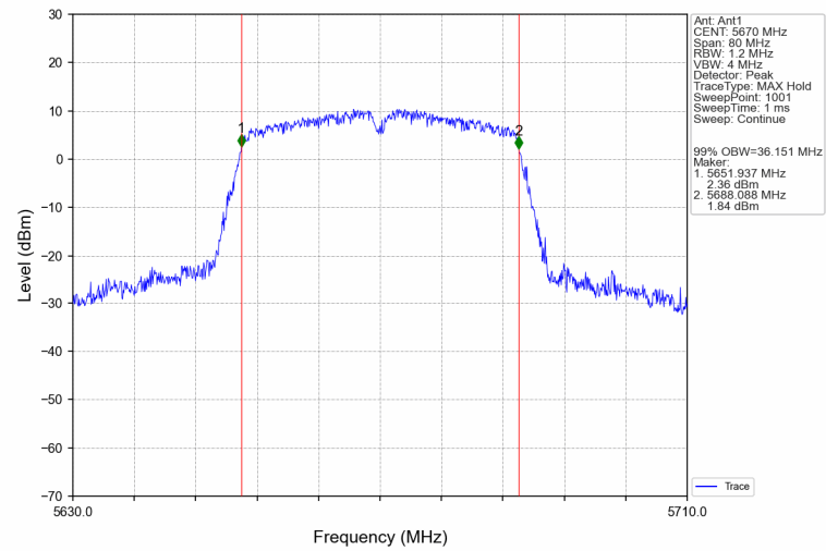
802.11 ac(VHT40) U-NII-2C High channel
