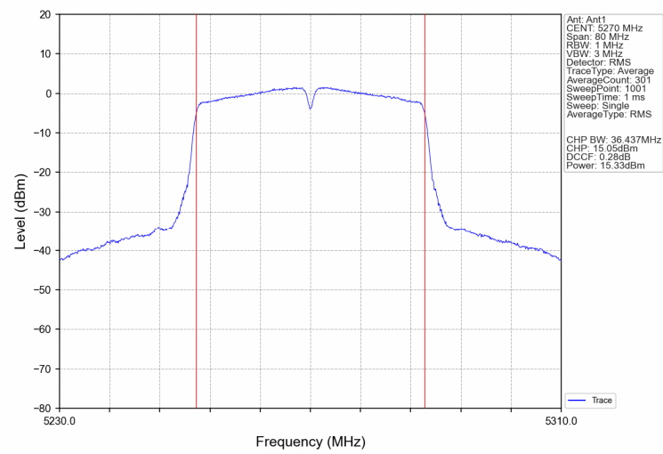
802.11n(HT40) U-NII-2A Low channel
