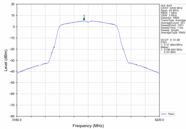
802.11a U-NII-1 Middle channel
