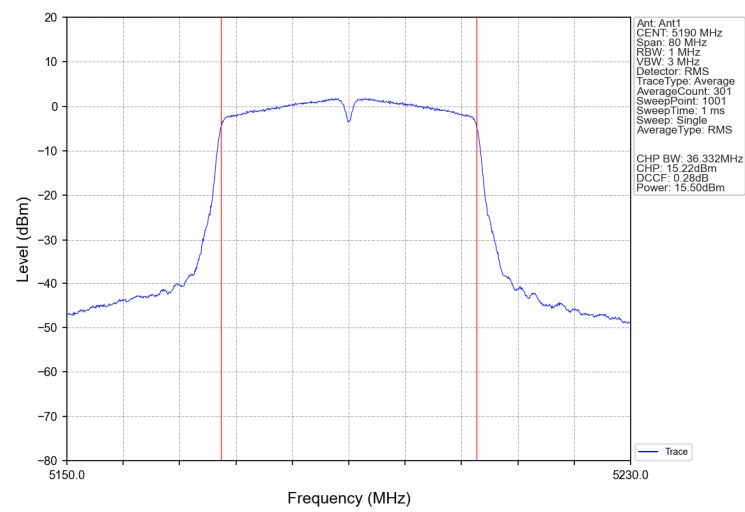
802.11ac(VHT40) U-NII-1 Low channel
