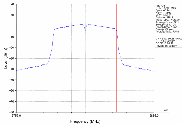
802.11n(HT40) U-NII-3 High channel
