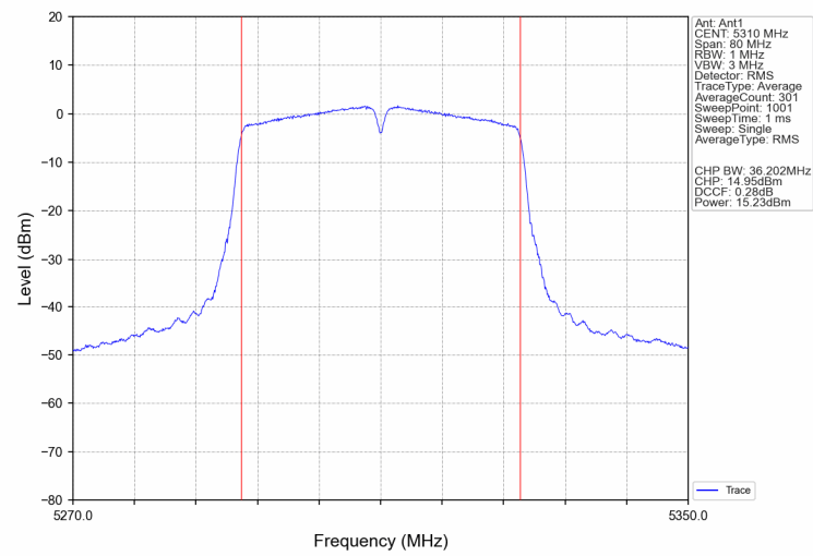
802.11n(HT40) U-NII-2A High channel
