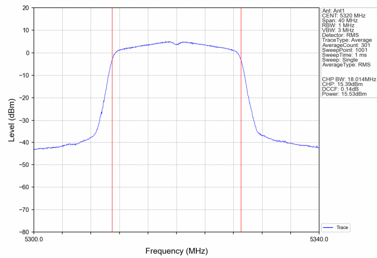
802.11n(HT20) U-NII-2A High channel
