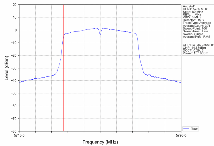
802.11n(HT40) U-NII-3 Low channel
