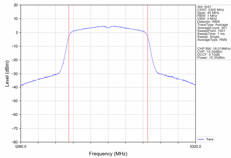
802.11n(HT20) U-NII-2A Middle channel
