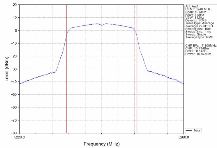
802.11a U-NII-1 High channel
