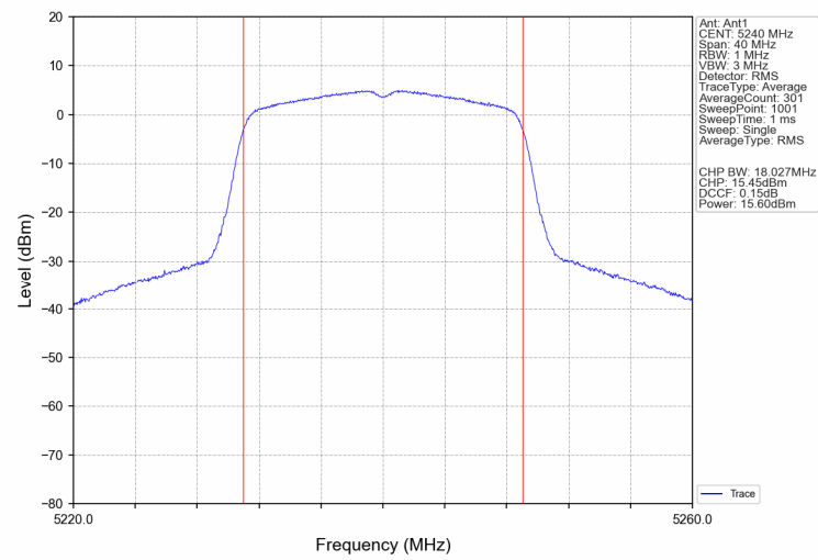
802.11n(HT20) U-NII-1 High channel
