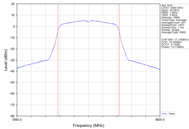
802.11a U-NII-2C Middle channel
