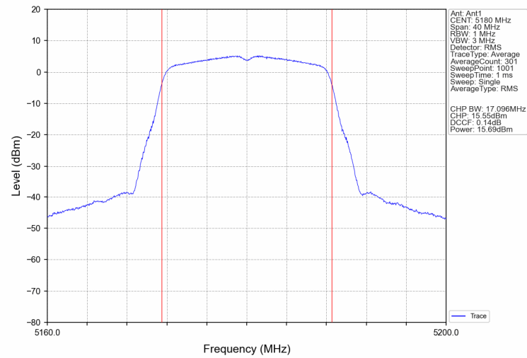
802.11a U-NII-1 Low channel
