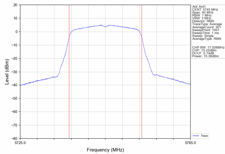
802.11a U-NII-3 Low channel
