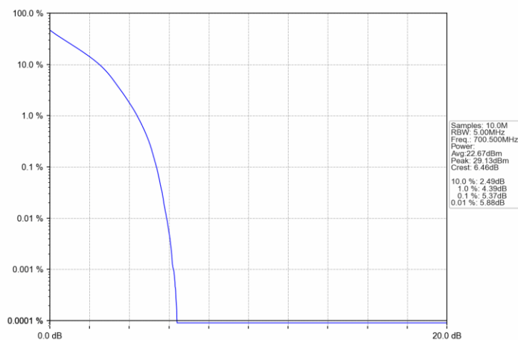
Band12_3MHz_QPSK_LCH_700.5MHz_RB_15_0_NTNV
