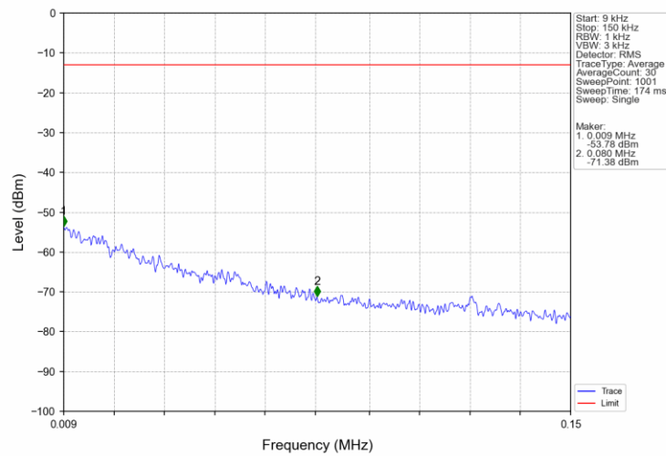
Band12 3MHz QPSK LCH 700.5MHz RB 1 0 NTNv
