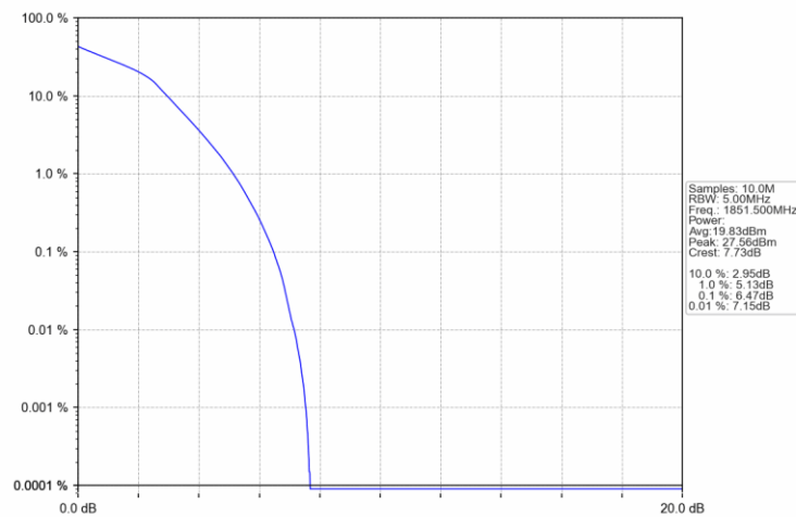
Band2 3MHz 16QAM LCH 1851.5MHz RB 15 0 NTV
