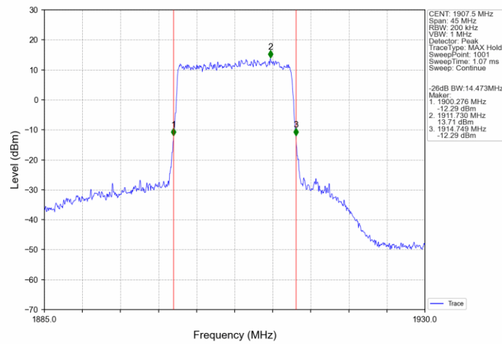
Band25_15MHz_16QAM_HCH_1907.5MHz_RB_75_0_NTNV
