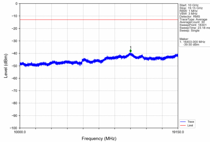
Band25_20MHz_16QAM_MCH_1882.5MHz_RB_1_0_NTNV
