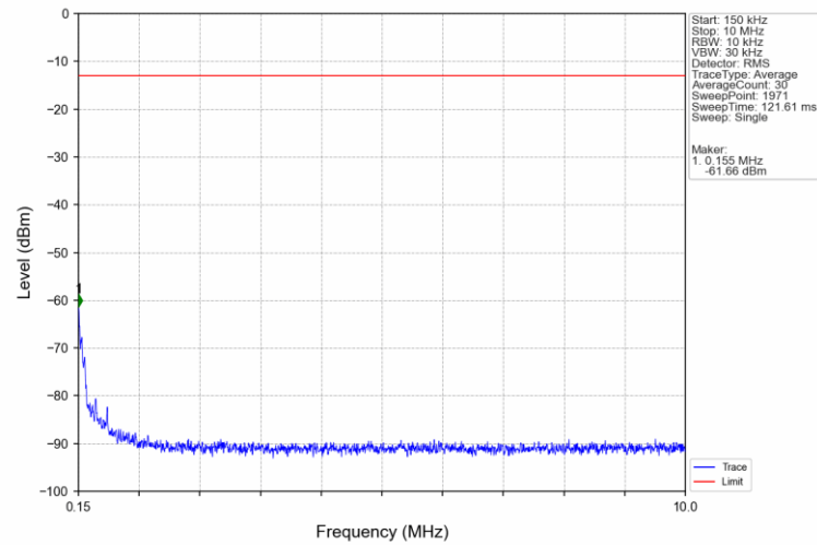
Band25_15MHz_16QAM_MCH_1882.5MHz_RB_1_0_NTNV
