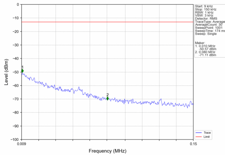
Band25_20MHz_16QAM_MCH_1882.5MHz_RB_1_0_NTNV
