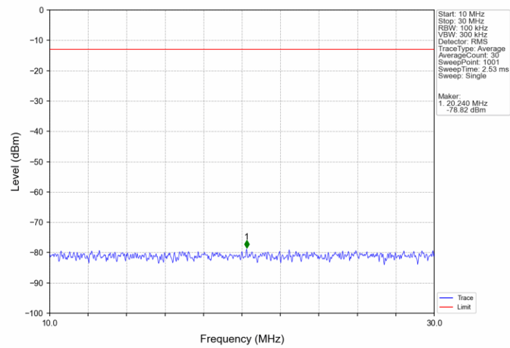
Band25_15MHz_16QAM_MCH_1882.5MHz_RB_1_0_NTNV
