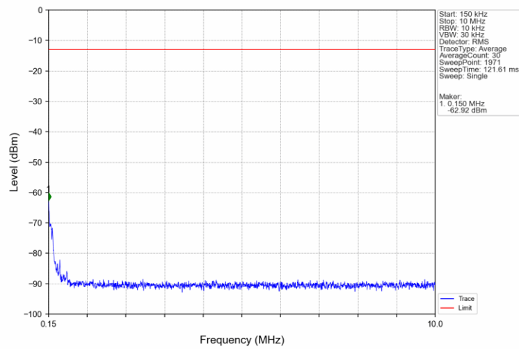
Band26a_3MHz_16QAM_MCH_819MHz_RB_1_0_NTNV
