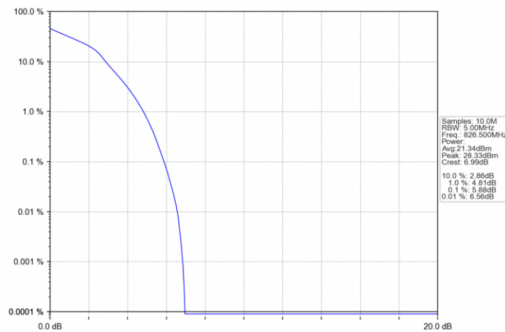
Band26b 5MHz 16QAM LCH 826.5MHz RB 25 0 NTN
