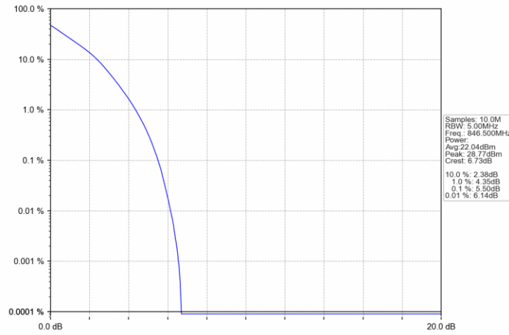
Band26b 5MHz QPSK HCH 846.5MHz RB 25 0 NTN
