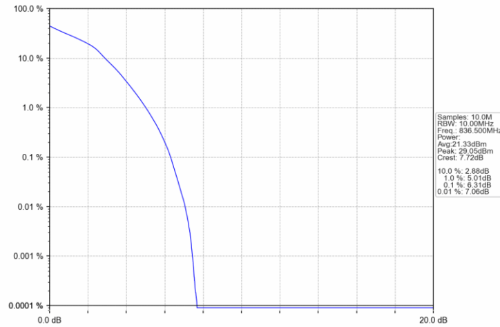
Band26b 10MHz 16QAM MCH 836.5MHz RB 50 0 NTV
