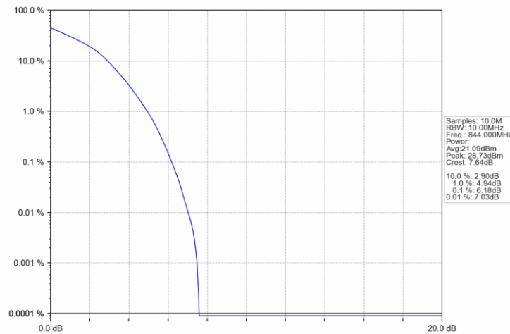
Band26b 10MHz 16QAM HCH 844MHz RB 50 0 NTV
