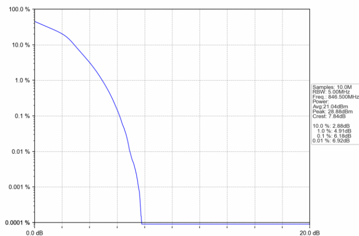
Band26b 5MHz 16QAM HCH 846.5MHz RB 25 0 NTNV
