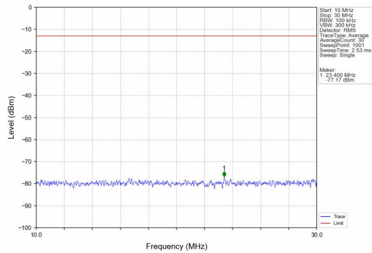
Band26b_5MHz_16QAM_LCH_826.5MHz_RB_1_0_NTNV
