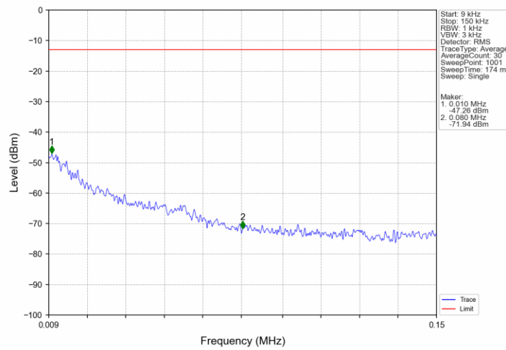
Band26b_10MHz_16QAM_HCH_844MHz_RB_1_0_NTNV
