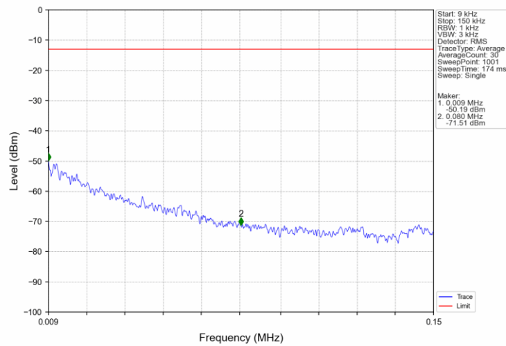
Band26b_5MHz_QPSK_LCH_826.5MHz_RB_1_0_NTNV
