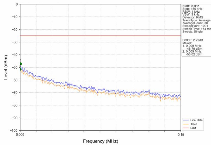
Band38_15MHz_16QAM_HCH_2612.5MHz_RB_1_0_NTNV
