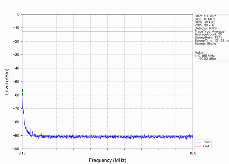
Band4_3MHz_16QAM_HCH_1753.5MHz_RB_1_0_NTNV
