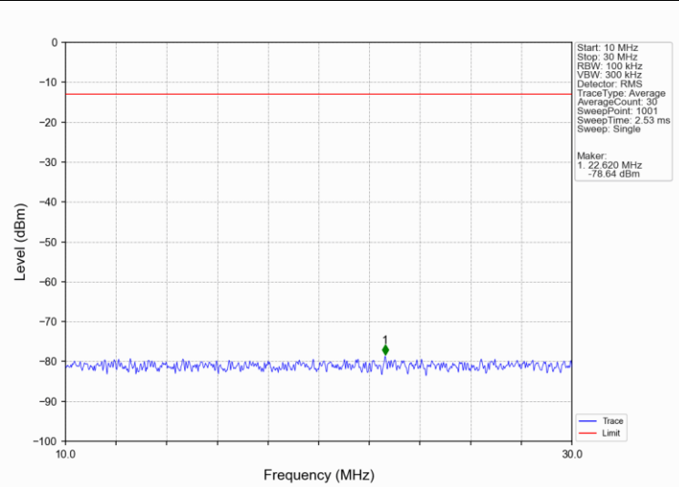
Band4_3MHz_16QAM_HCH_1753.5MHz_RB_1_0_NTNV
