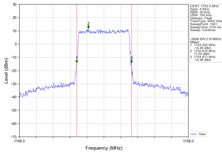
Band4 3MHz 16QAM HCH 1753.5MHz RB 15 0 NTN
