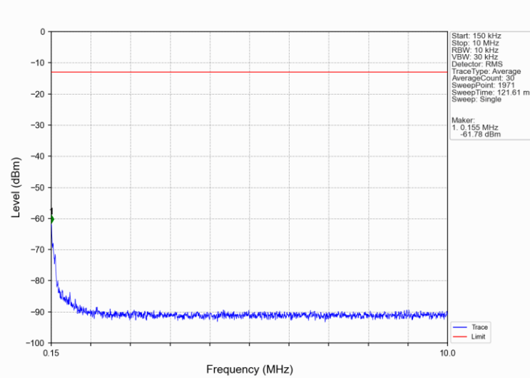
Band4_10MHz_16QAM_MCH_1732.5MHz_RB_1_0_NTNV
