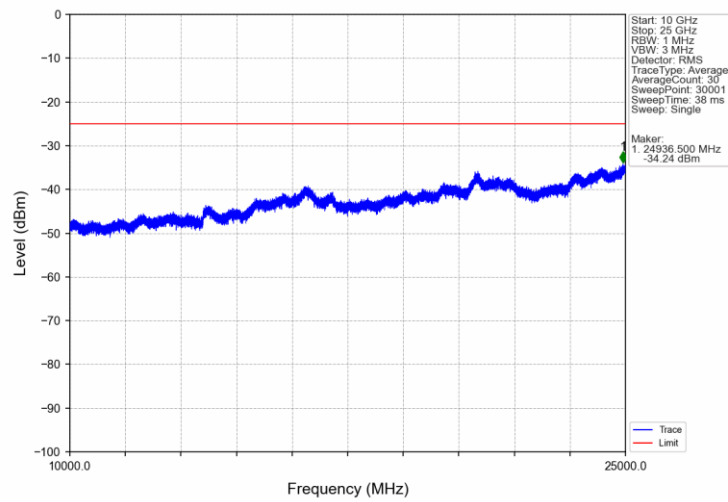
Band7_10MHz_16QAM_MCH_2535MHz_RB_1_0_NTNV
