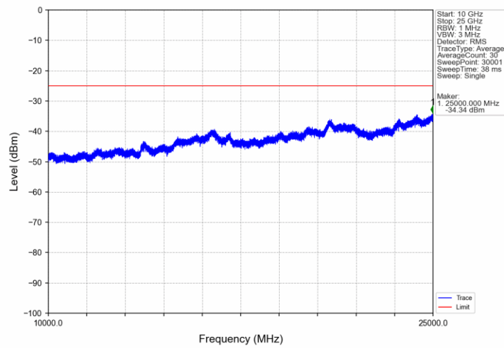
Band7_15MHz_16QAM_MCH_2535MHz_RB_1_0_NTNV
