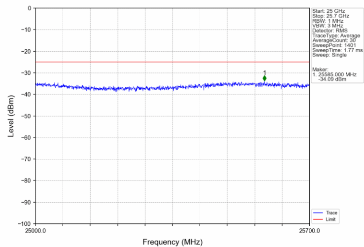
Band7_15MHz_QPSK_HCH_2562.5MHz_RB_1_0_NTNV
