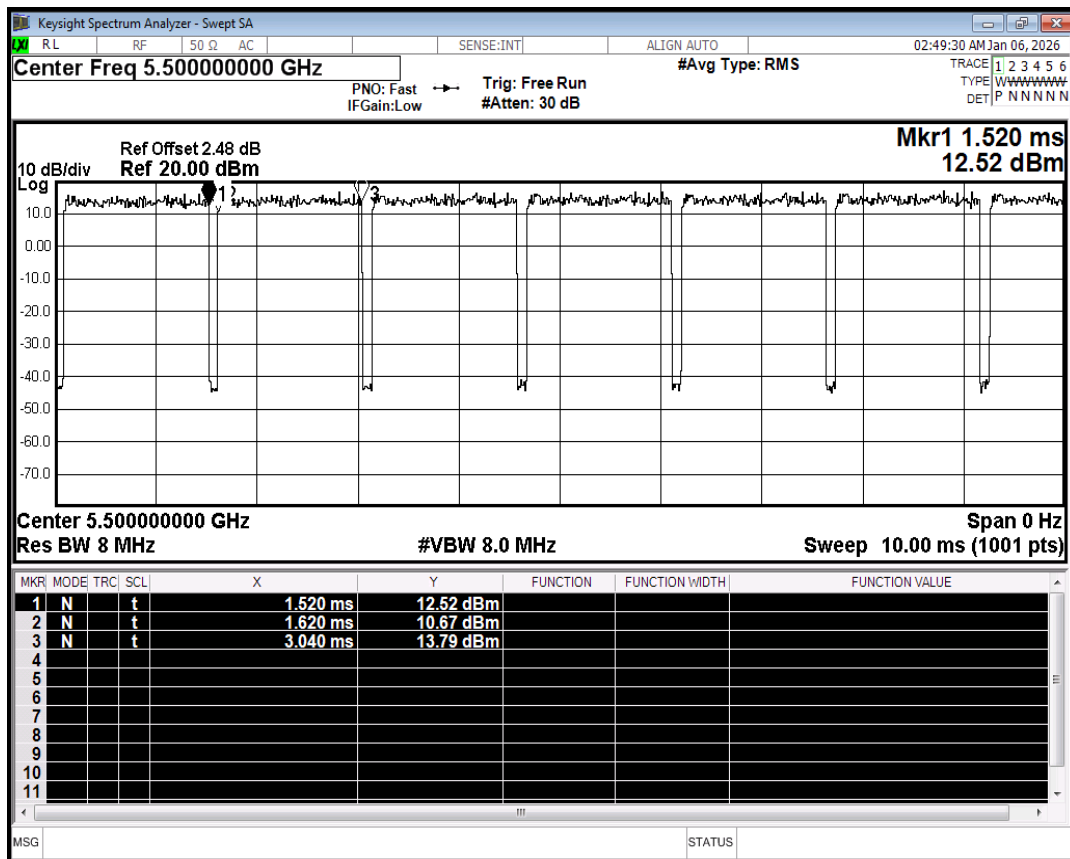
Duty Cycle NVNT a 5500MHz Ant1
