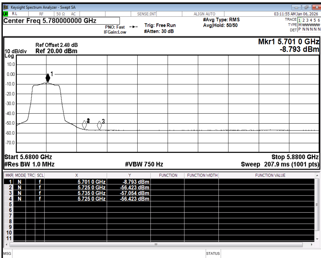
Restrict Band NVNT ac20 5700MHz Ant1 Average
