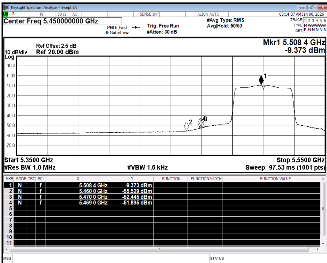
Restrict Band NVNT n40 5510MHz Ant1 Average
