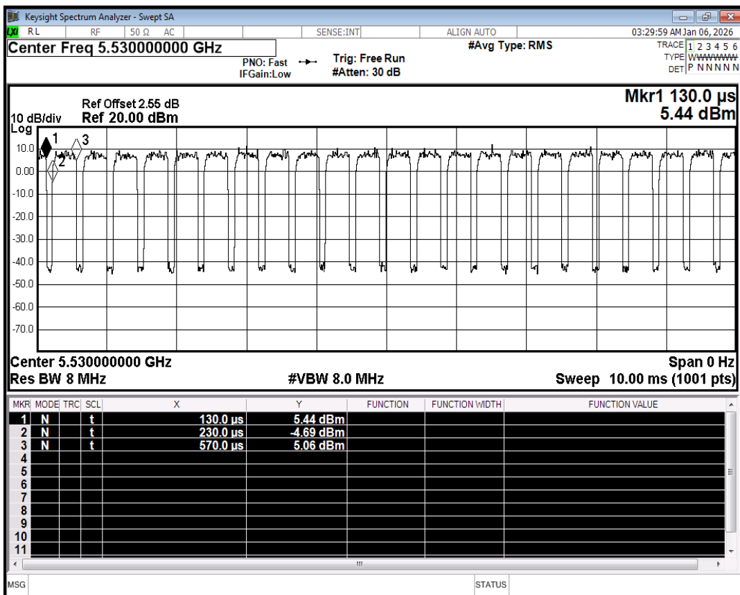
Duty Cycle NVNT ac80 5530MHz Ant1
