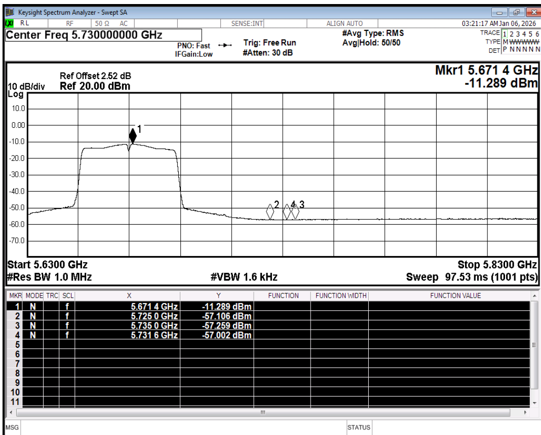
Restrict Band NVNT n40 5670MHz Ant1 Average
