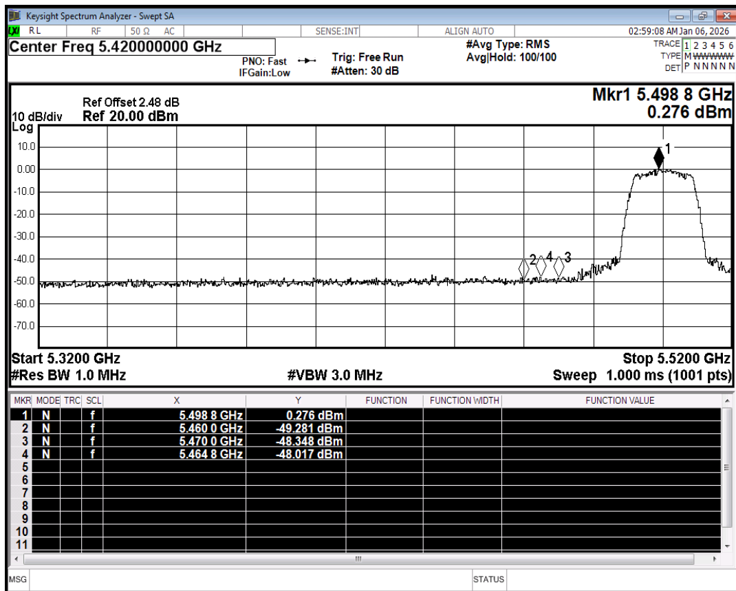
Restrict Band NVNT n20 5500MHz Ant1 Peak
