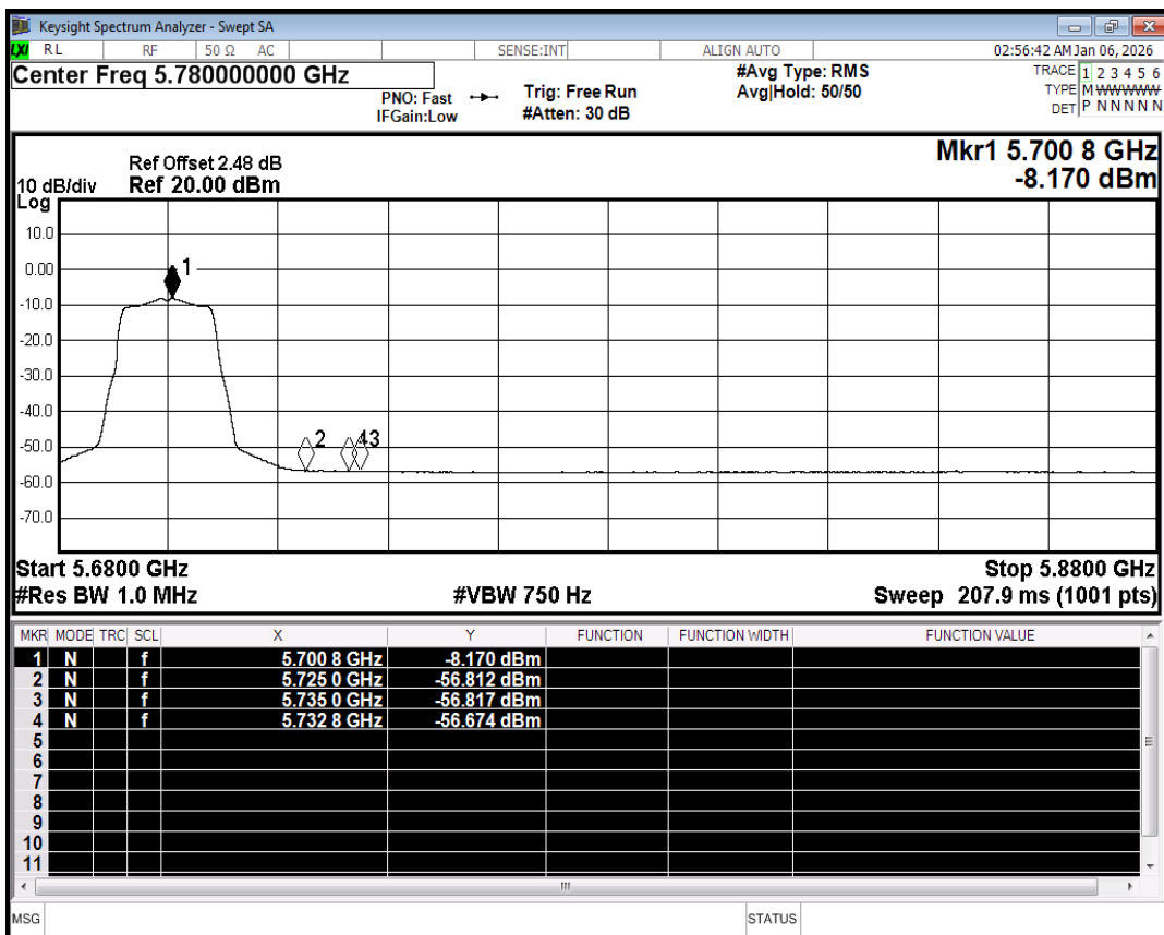
Restrict Band NVNT a 5700MHz Ant1 Average
