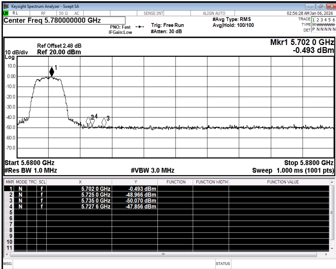
Restrict Band NVNT a 5700MHz Ant1 Peak
