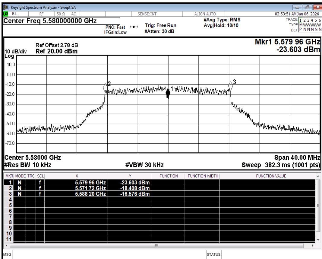
Freq. Stability NVNT a 5580MHz Ant1
