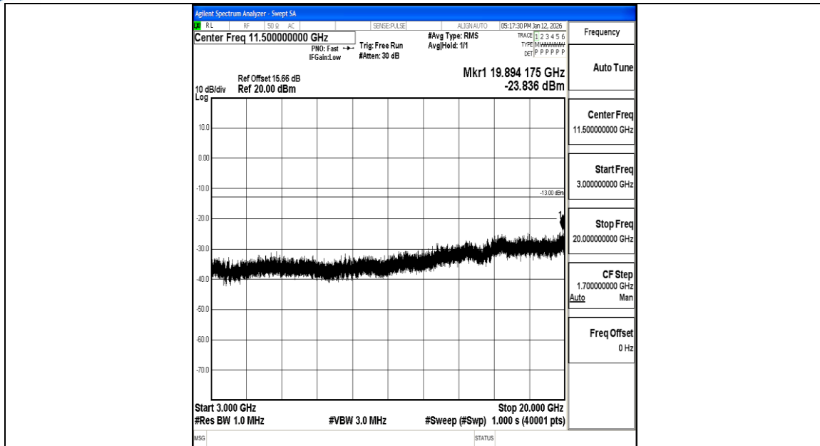
Band2_20MHz_16QAM_18700_1RB#0_3000~20000_3000~20000
