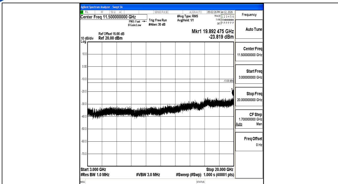
Band2_15MHz_16QAM_18900_1RB#0_3000~20000_3000~20000
