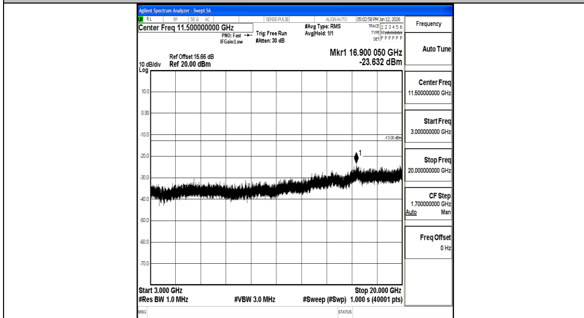
Band2_15MHz_QPSK_19125_1RB#0_3000~20000_3000~20000
