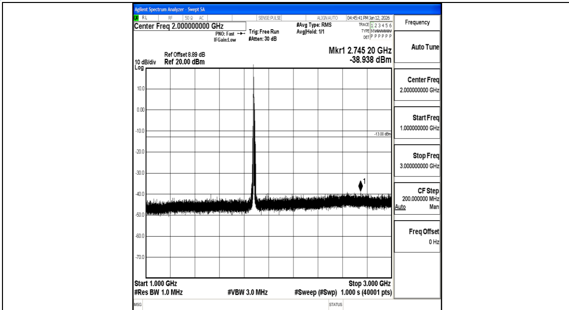
Band2_10MHz_QPSK_18900_1RB#0_1000~3000_1000~3000
