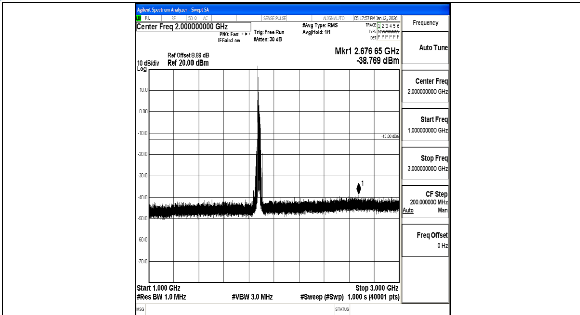
Band2_20MHz_QPSK_18900_1RB#0_1000~3000_1000~3000
