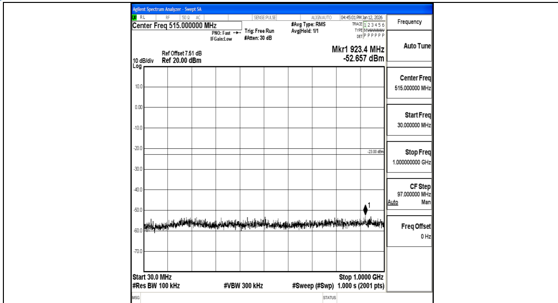
Band2_10MHz_16QAM_18650_1RB#0_30~1000_30~1000
