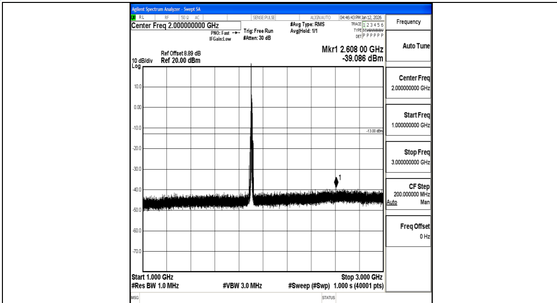
Band2_10MHz_QPSK_19150_1RB#0_1000~3000_1000~3000
