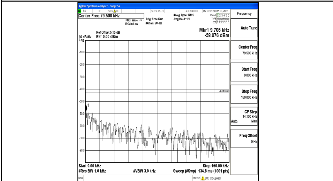
Band2_20MHz_QPSK_18700_1RB#0_0.009~0.15_0.009~0.15
