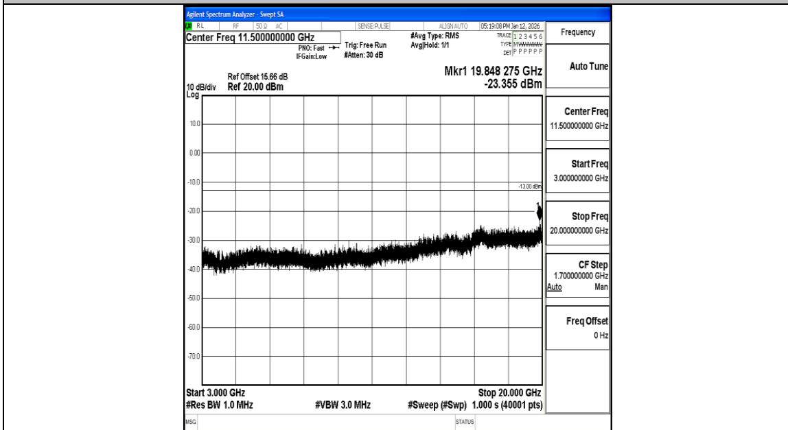
Band2_20MHz_QPSK_19100_1RB#0_3000~20000_3000~20000
