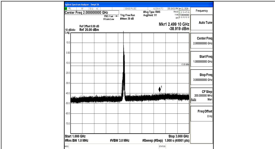
Band2_20MHz_QPSK_19100_1RB#0_1000~3000_1000~3000
