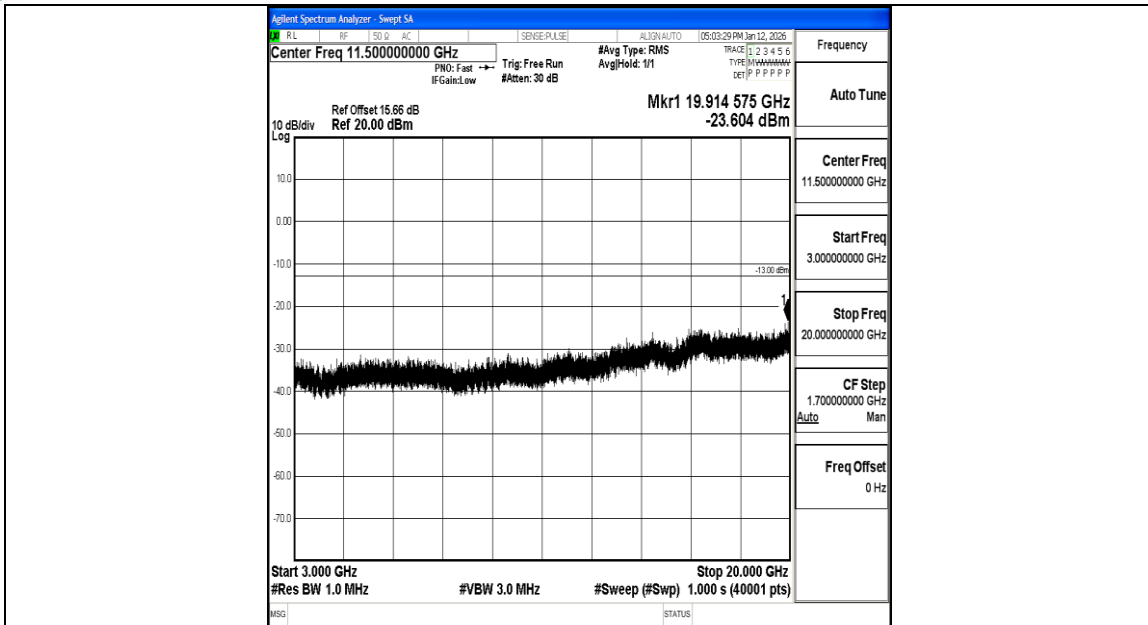
Band2_15MHz_16QAM_19125_1RB#0_3000~20000_3000~20000
