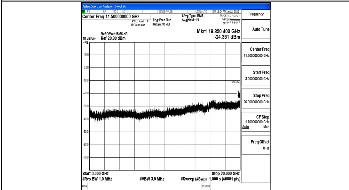
Band2_20MHz_QPSK_18900_1RB#0_3000~20000_3000~20000
