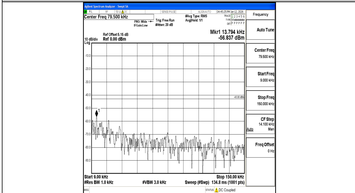
Band2_10MHz_QPSK_18900_1RB#0_0.009~0.15_0.009~0.15
