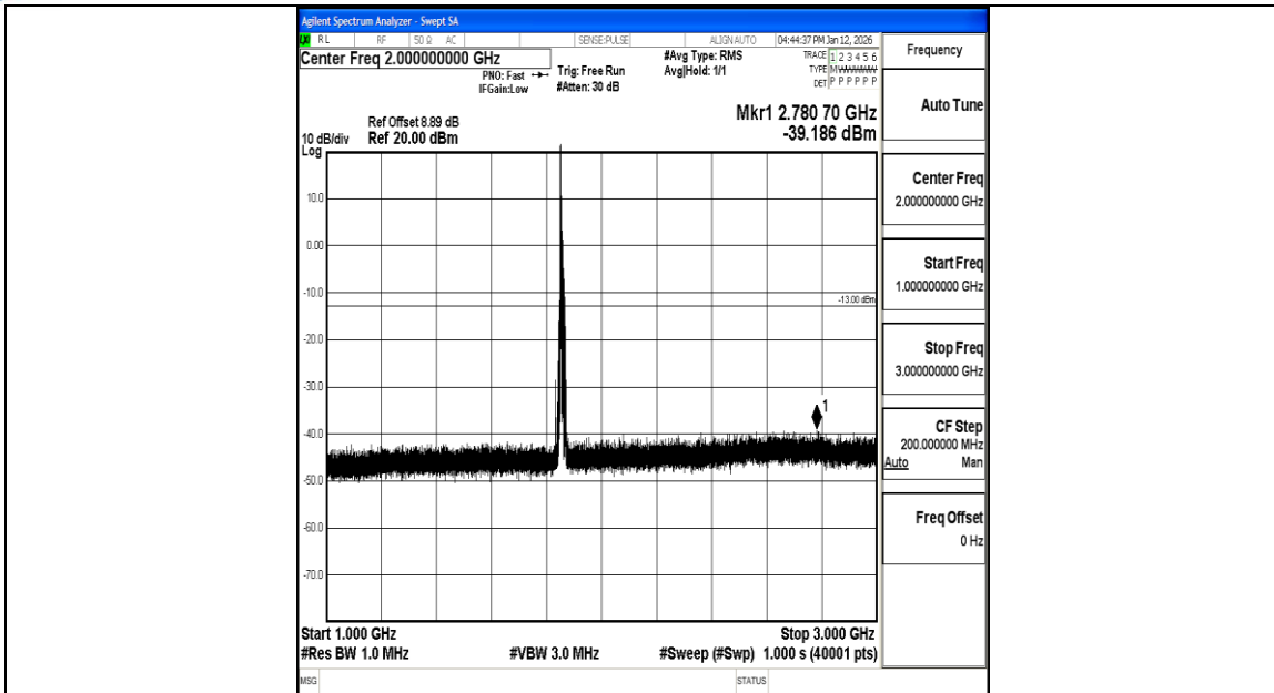
Band2_10MHz_QPSK_18650_1RB#0_1000~3000_1000~3000
