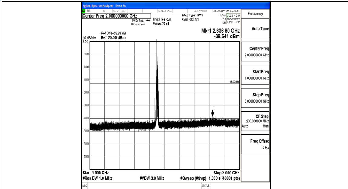
Band2_15MHz_QPSK_19125_1RB#0_1000~3000_1000~3000
