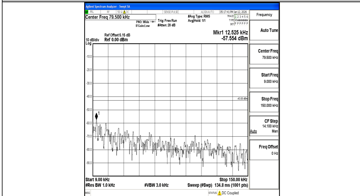
Band2_20MHz_QPSK_18900_1RB#0_0.009~0.15_0.009~0.15
