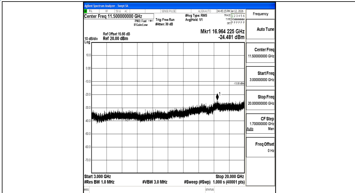
Band2_10MHz_16QAM_18650_1RB#0_3000~20000_3000~20000
