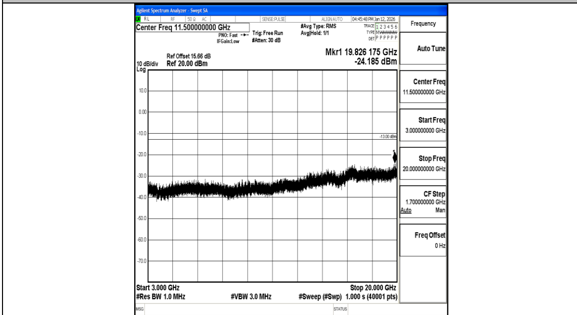
Band2_10MHz_QPSK_18900_1RB#0_3000~20000_3000~20000
