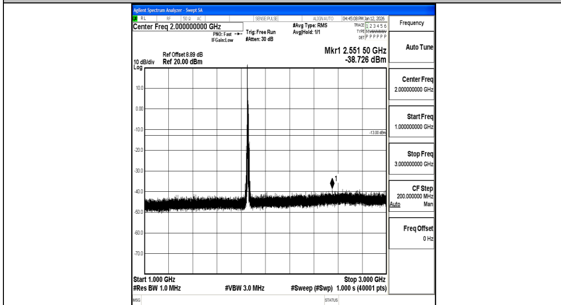
Band2_10MHz_16QAM_18650_1RB#0_1000~3000_1000~3000
