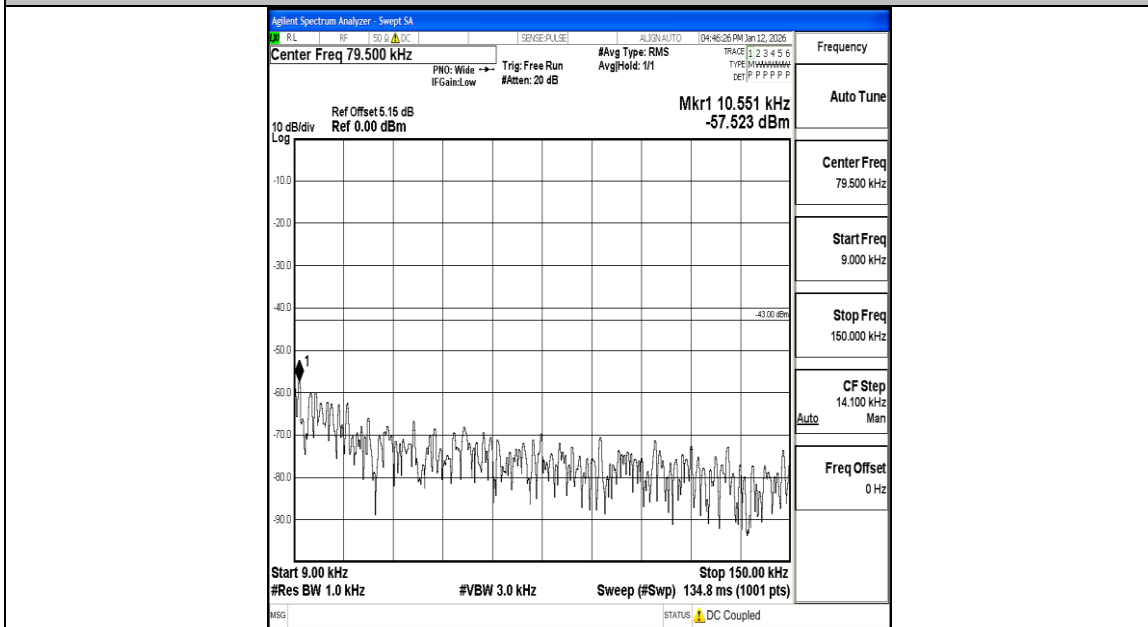
Band2_10MHz_QPSK_19150_1RB#0_0.009~0.15_0.009~0.15
