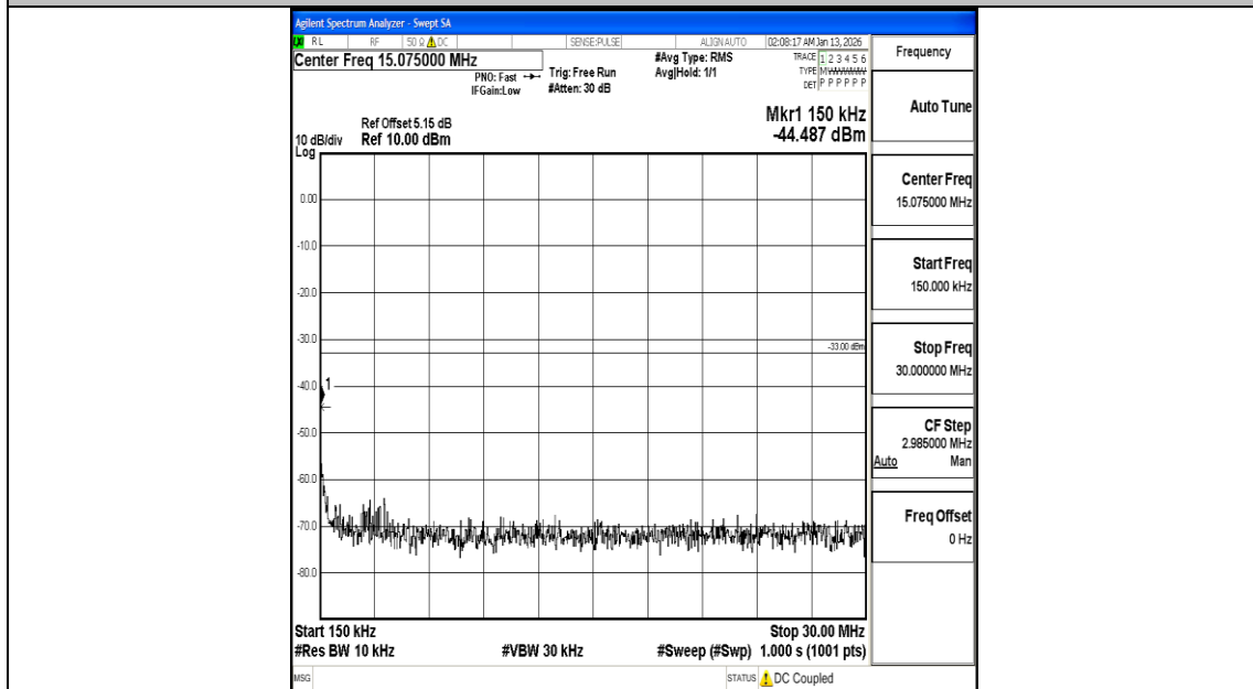
Band25_15MHz_16QAM_26365_1RB#0_0.15~30_0.15~30
