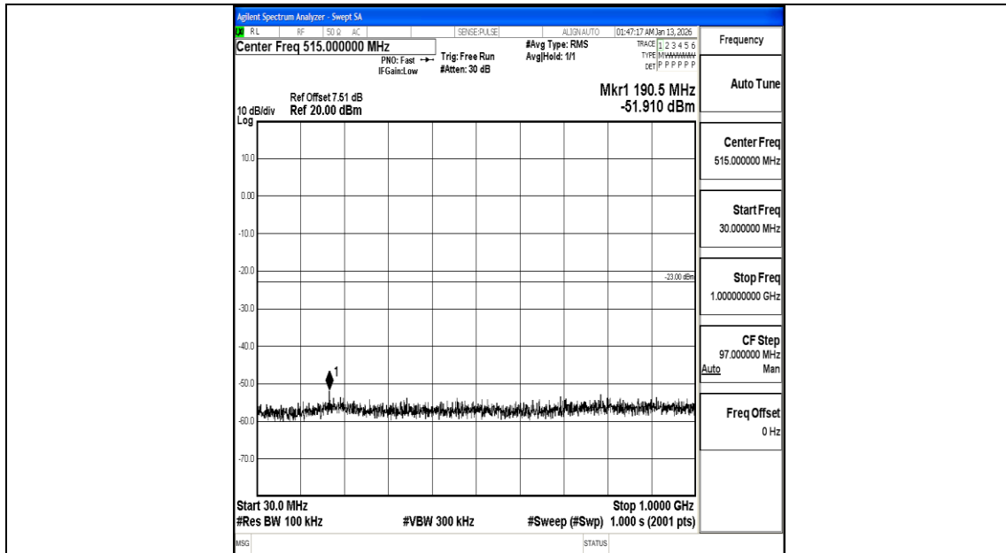
Band25_10MHz_16QAM_26090_1RB#0_30~1000_30~1000
