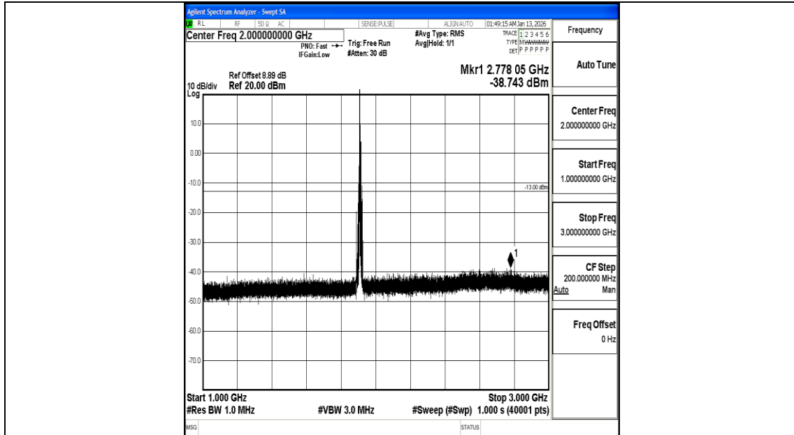
Band25_10MHz_QPSK_26640_1RB#0_1000~3000_1000~3000
