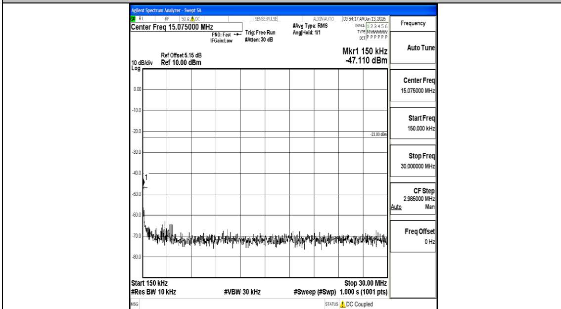
Band26_10MHz_16QAM_26740_1RB#0_0.15~30_0.15~30
