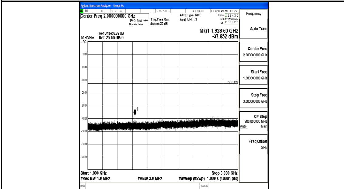
Band26_5MHz_16QAM_26715_1RB#0_1000~3000_1000~3000
