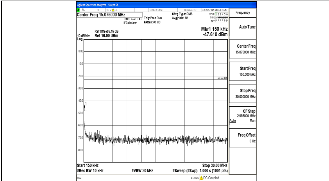
Band26_5MHz_QPSK_26715_1RB#0_0.15~30_0.15~30
