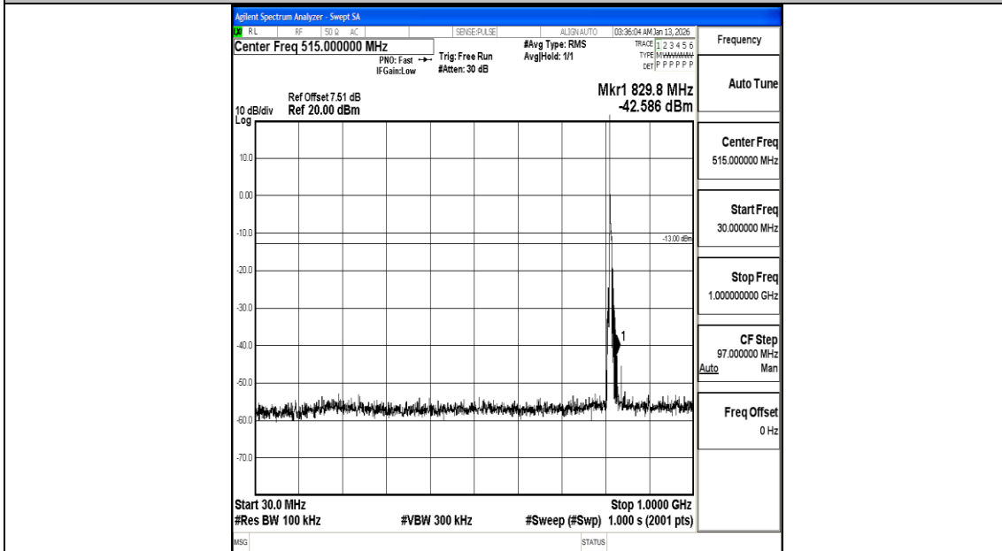
Band26_5MHz_QPSK_26715_1RB#0_30~1000_30~1000
