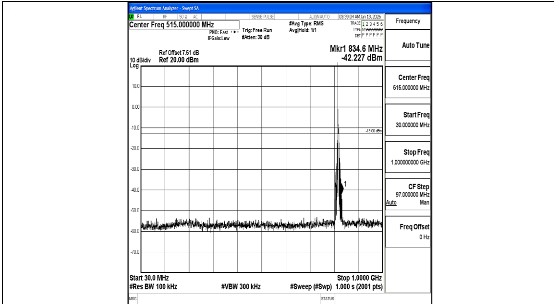
Band26_5MHz_16QAM_26765_1RB#0_30~1000_30~1000
