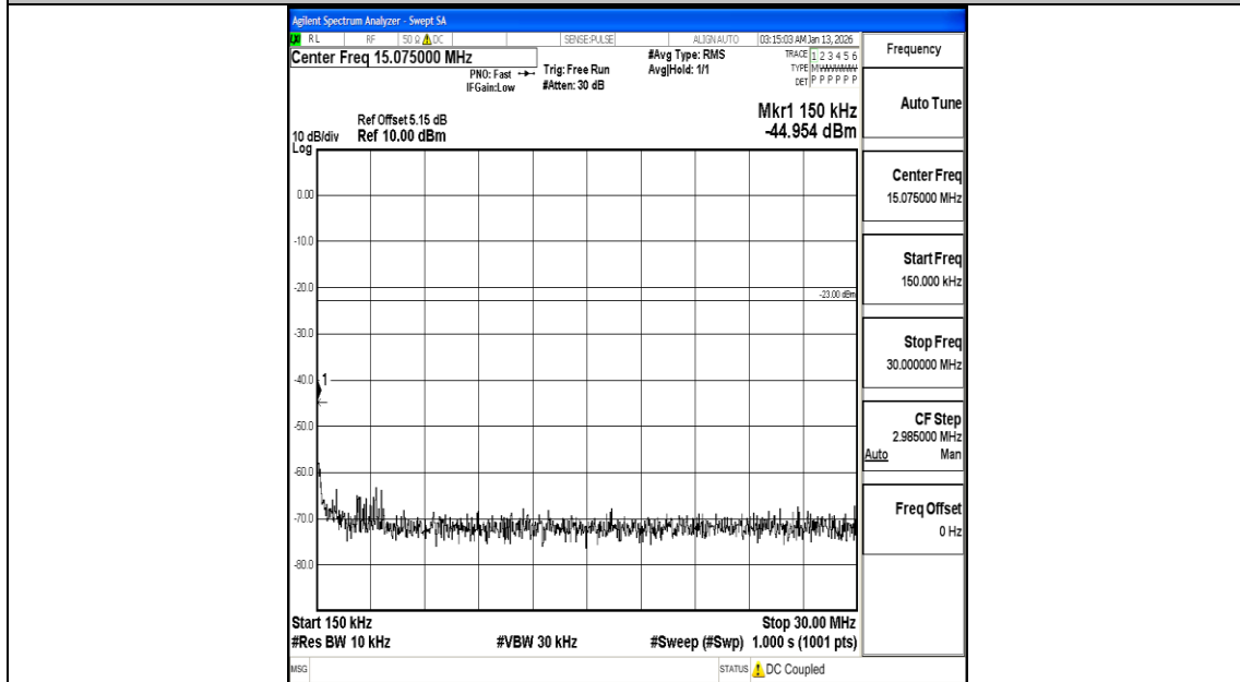
Band26_3MHz_16QAM_26740_1RB#0_0.15~30_0.15~30
