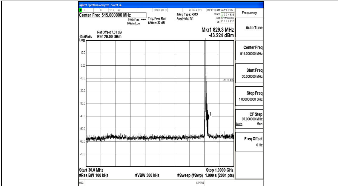
Band26_5MHz_16QAM_26715_1RB#0_30~1000_30~1000
