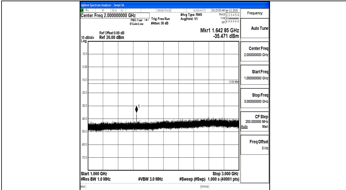
Band26_3MHz_QPSK_26775_1RB#0_1000~3000_1000~3000
