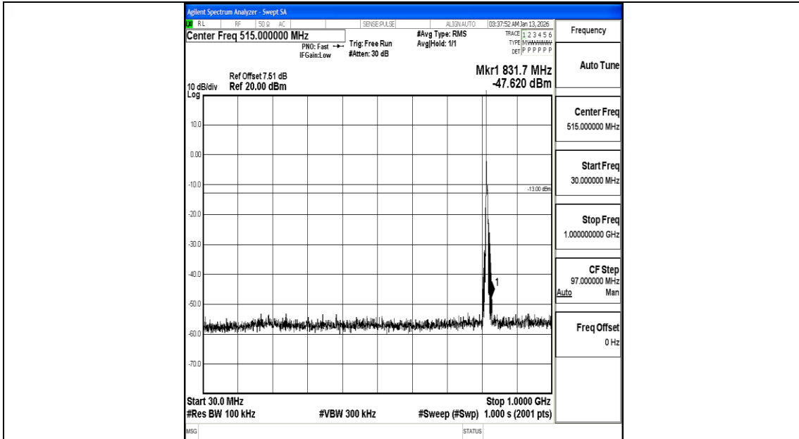
Band26_5MHz_16QAM_26740_1RB#0_30~1000_30~1000
