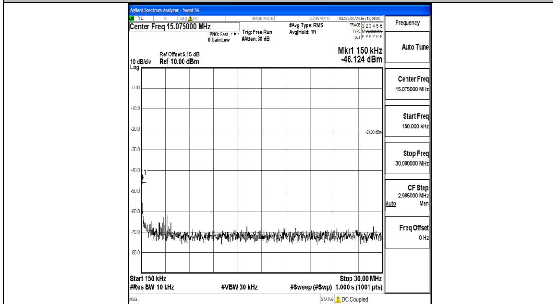
Band26_5MHz_16QAM_26715_1RB#0_0.15~30_0.15~30
