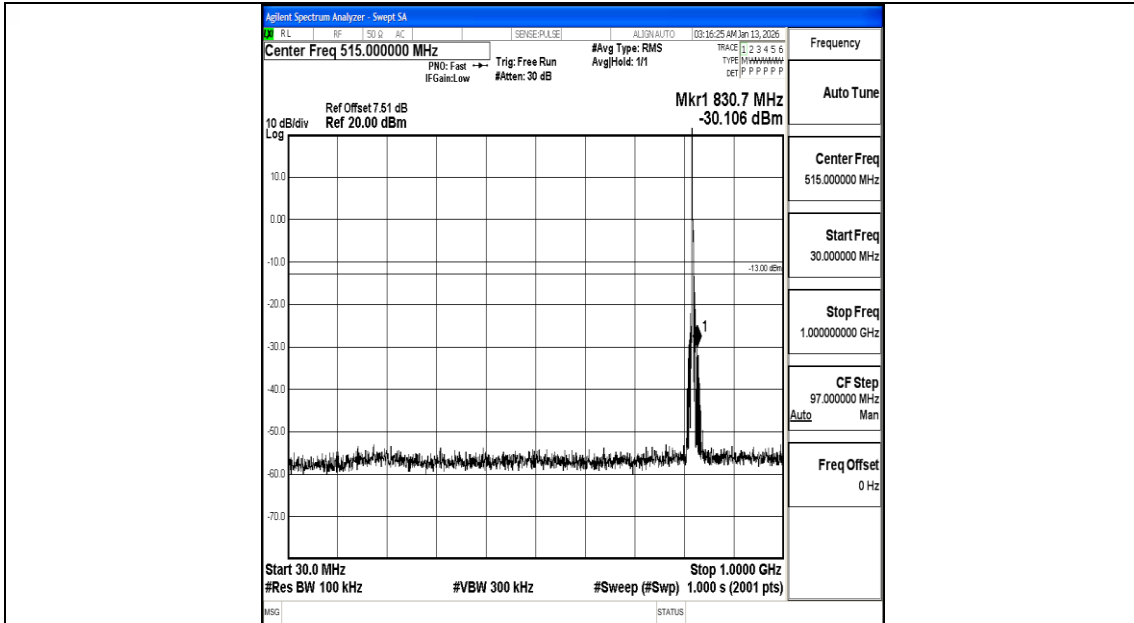
Band26_3MHz_16QAM_26775_1RB#0_30~1000_30~1000
