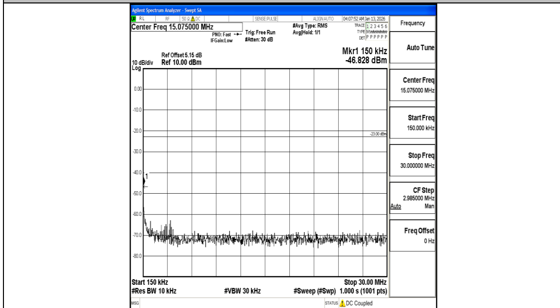
Band26_1.4MHz_QPSK_27033_1RB#0_0.15~30_0.15~30
