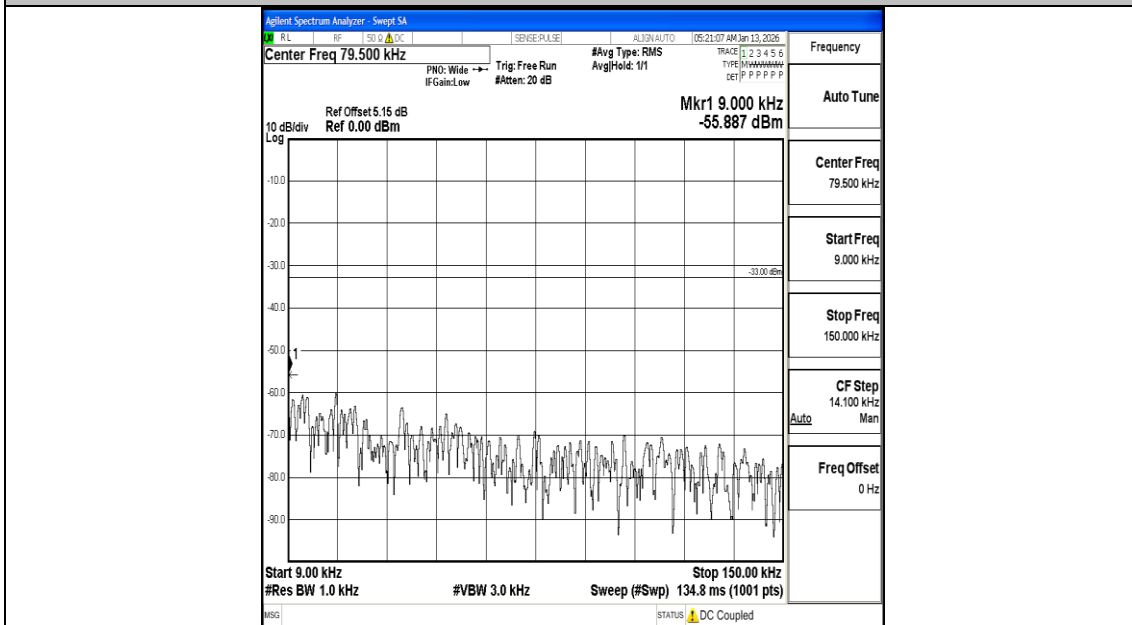
Band26_10MHz_16QAM_26840_1RB#0_0.009~0.15_0.009~0.15
