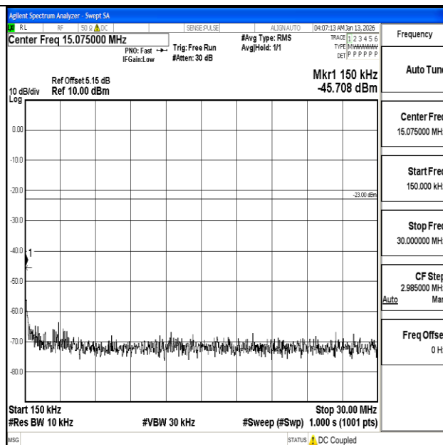
Band26_1.4MHz_16QAM_26915_1RB#0_0.15~30_0.15~30
