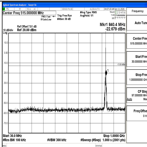
Band26_1.4MHz_16QAM_26915_1RB#0_30~1000_30~1000
