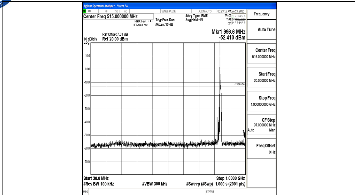
Band26_10MHz_QPSK_26990_1RB#0_30~1000_30~1000
