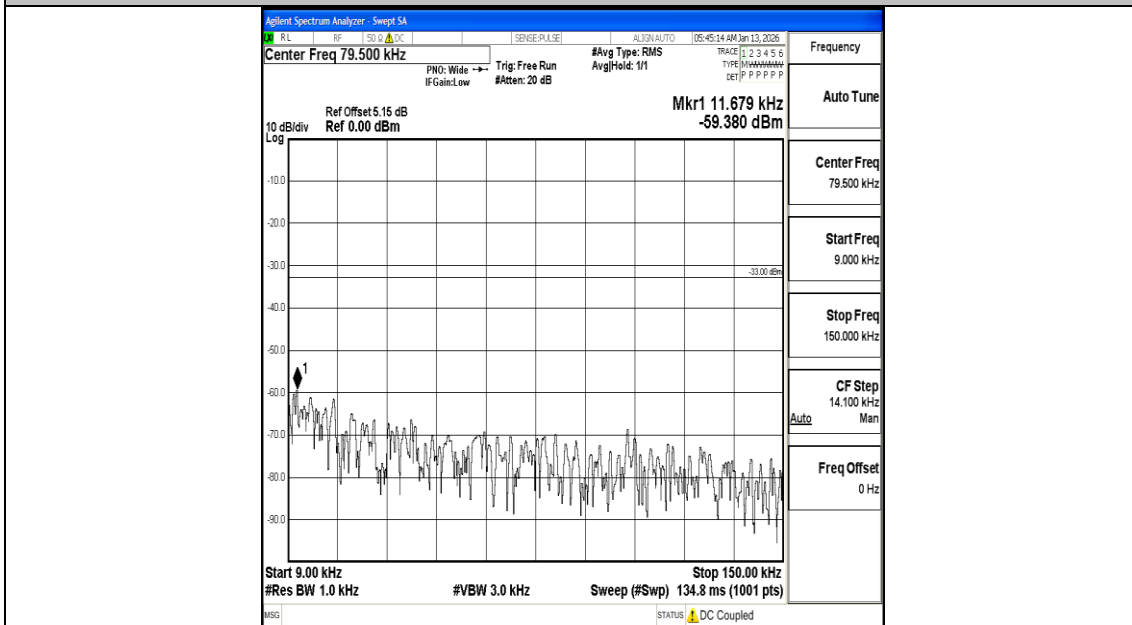
Band26_15MHz_16QAM_26965_1RB#0_0.009~0.15_0.009~0.15
