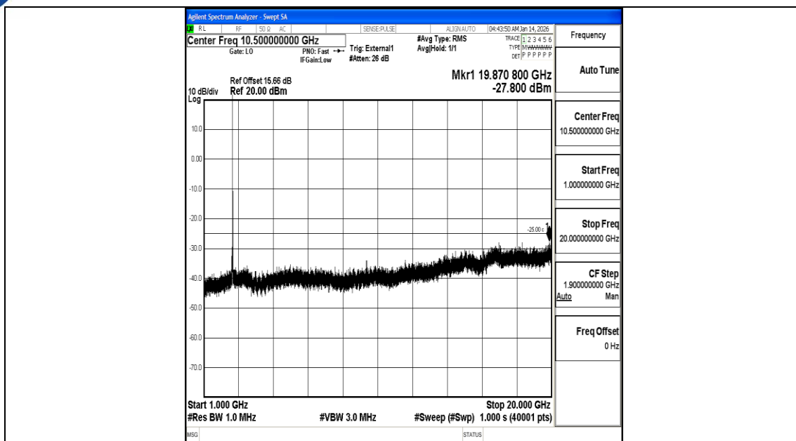
Band38_20MHz_16QAM_37850_1RB#0_1000~20000_1000~20000
