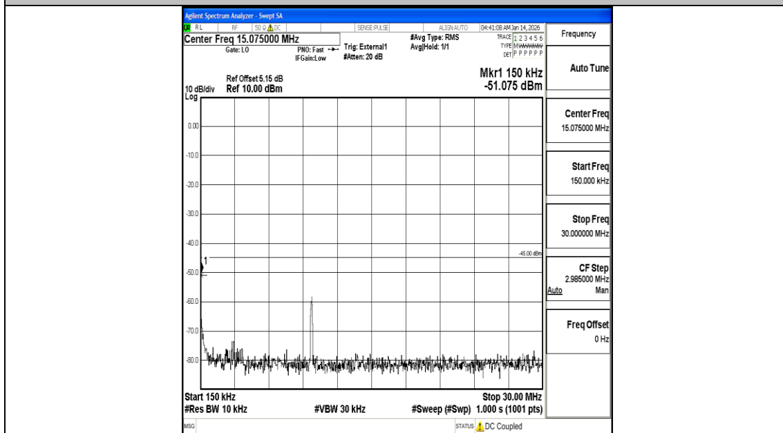
Band38_20MHz_QPSK_37850_1RB#0_0.15~30_0.15~30
