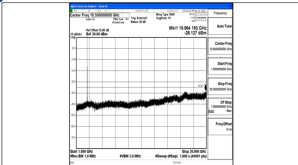
Band38_15MHz_16QAM_38175_1RB#0_1000~20000_1000~20000
