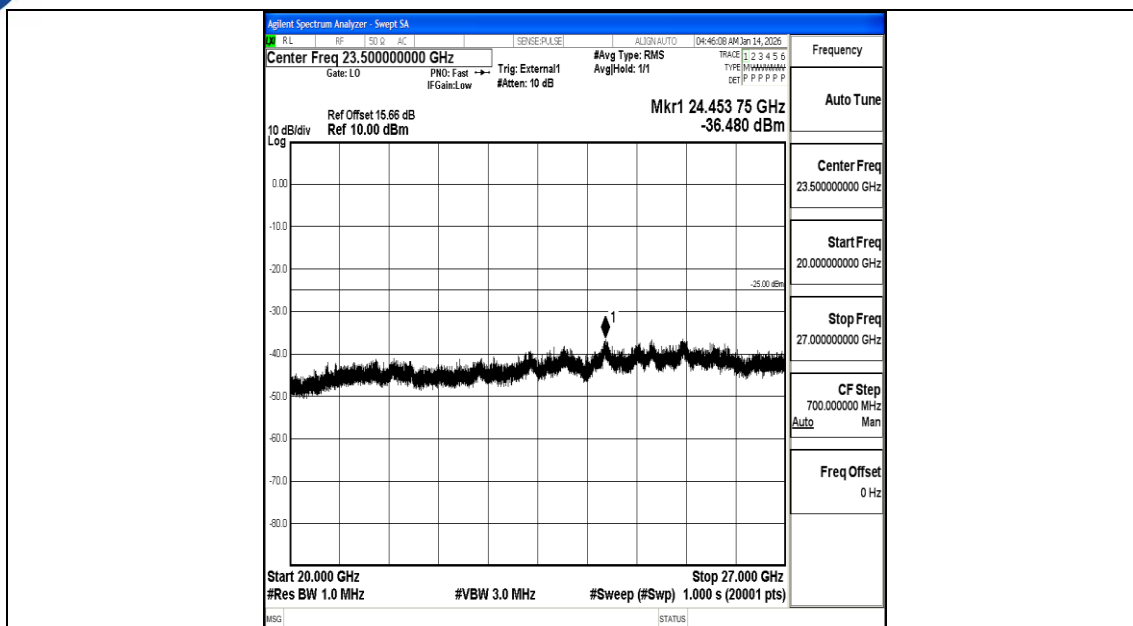
Band38_20MHz_QPSK_38000_1RB#0_20000~27000_20000~27000
