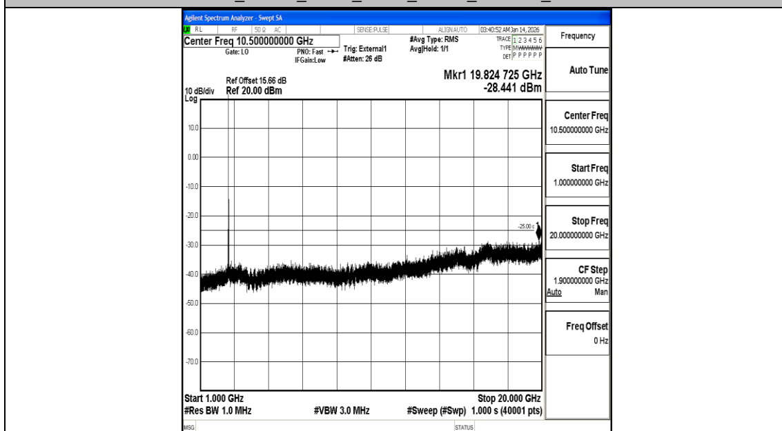
Band38_10MHz_QPSK_37800_1RB#0_1000~20000_1000~20000
