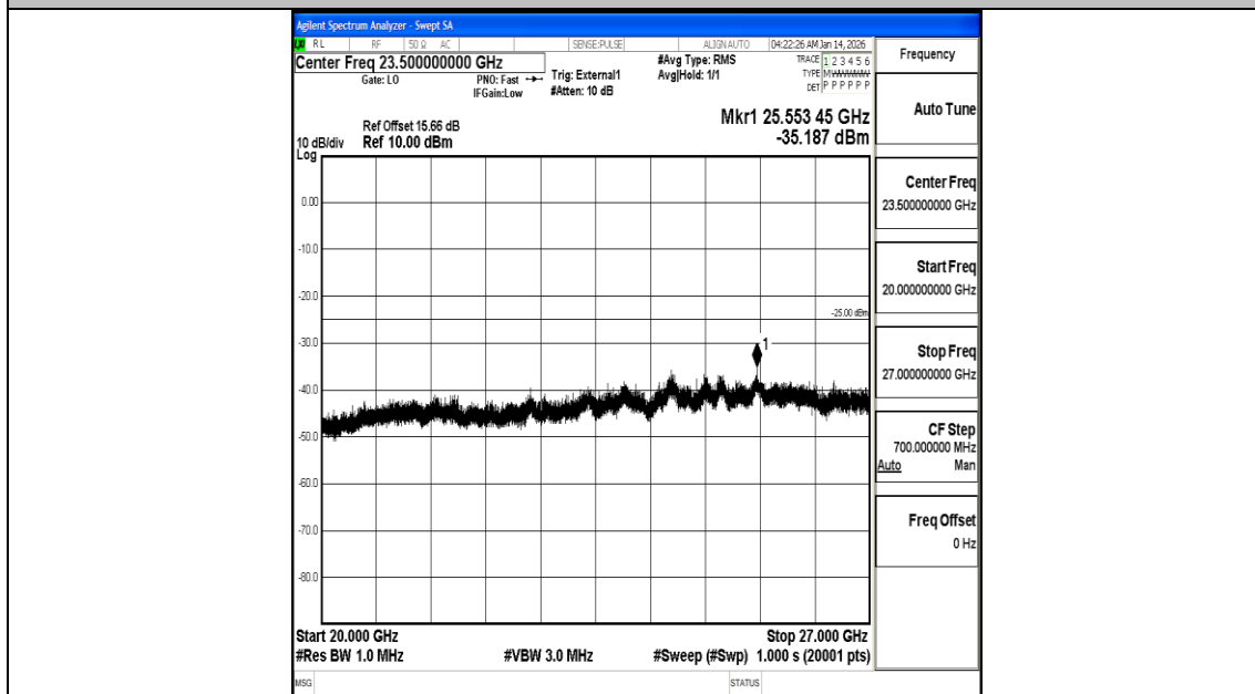
Band38_15MHz_16QAM_38175_1RB#0_20000~27000_20000~27000
