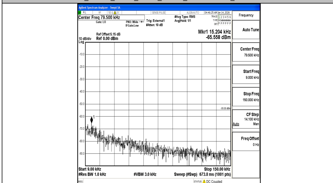
Band38_20MHz_16QAM_38000_1RB#0_0.009~0.15_0.009~0.15
