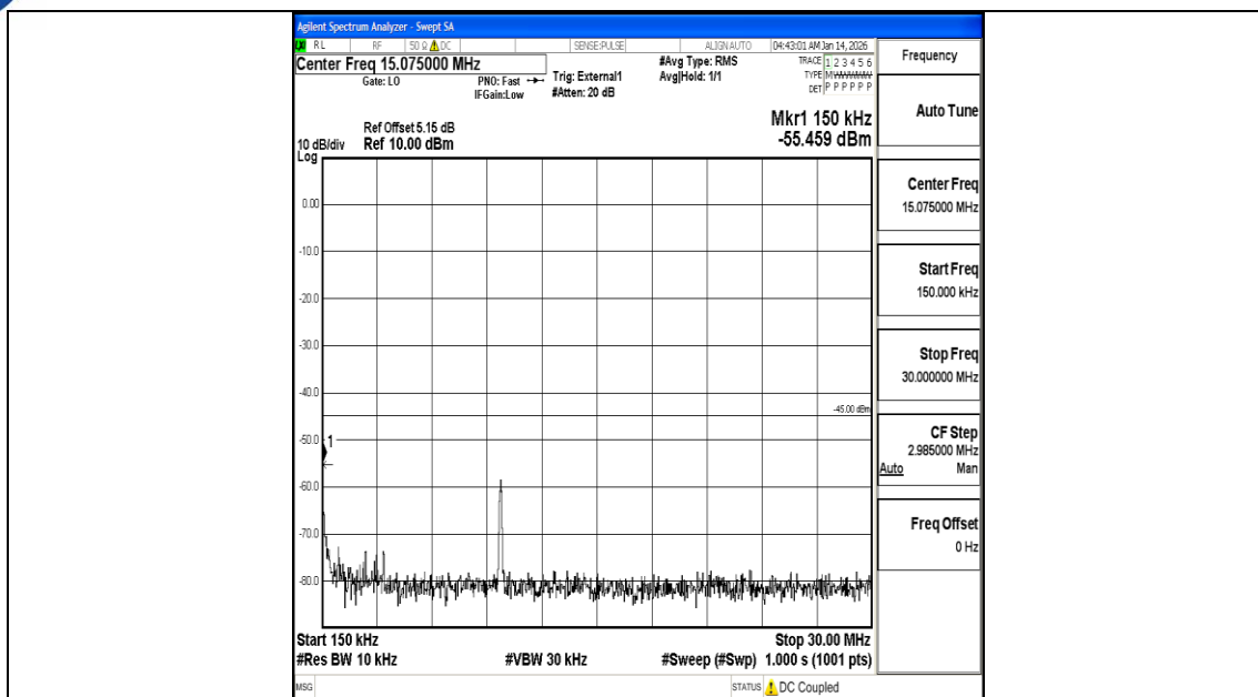
Band38_20MHz_16QAM_37850_1RB#0_0.15~30_0.15~30
