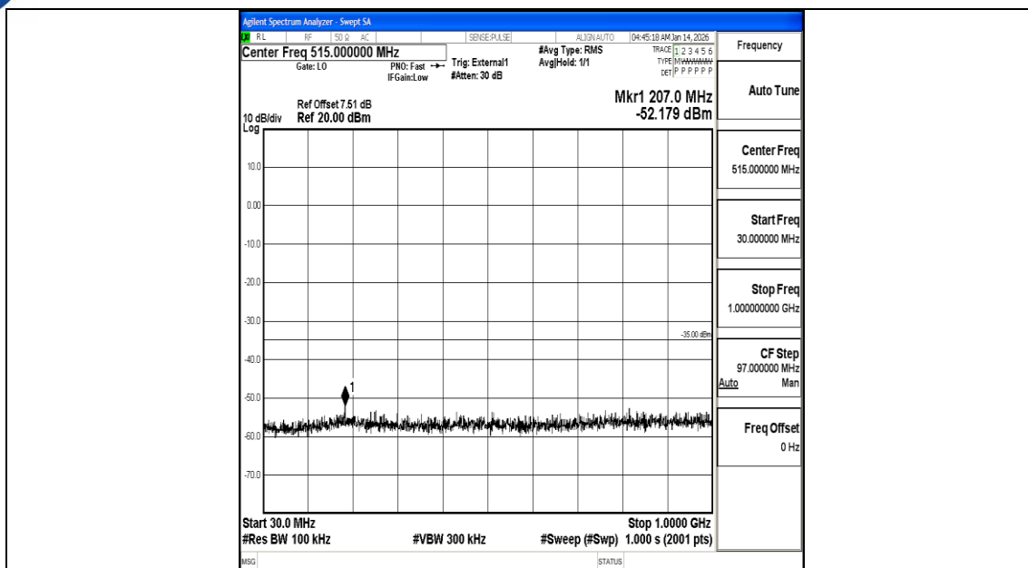
Band38_20MHz_QPSK_38000_1RB#0_30~1000_30~1000
