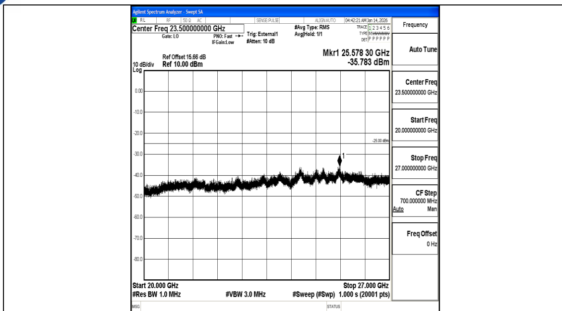
Band38_20MHz_QPSK_37850_1RB#0_20000~27000_20000~27000
