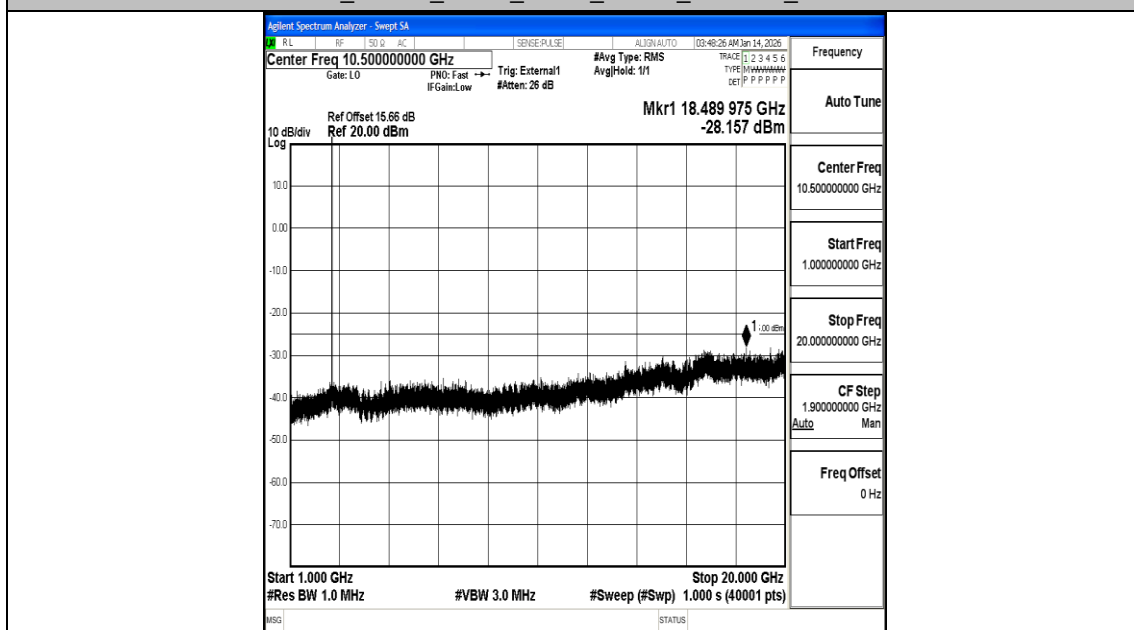
Band38_10MHz_QPSK_38200_1RB#0_1000~20000_1000~20000
