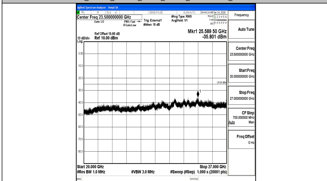
Band38_20MHz_16QAM_37850_1RB#0_20000~27000_20000~27000
