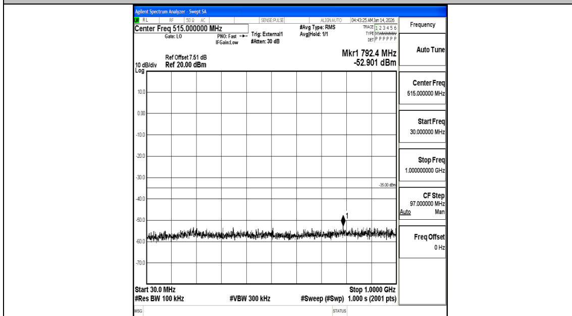
Band38_20MHz_16QAM_37850_1RB#0_30~1000_30~1000
