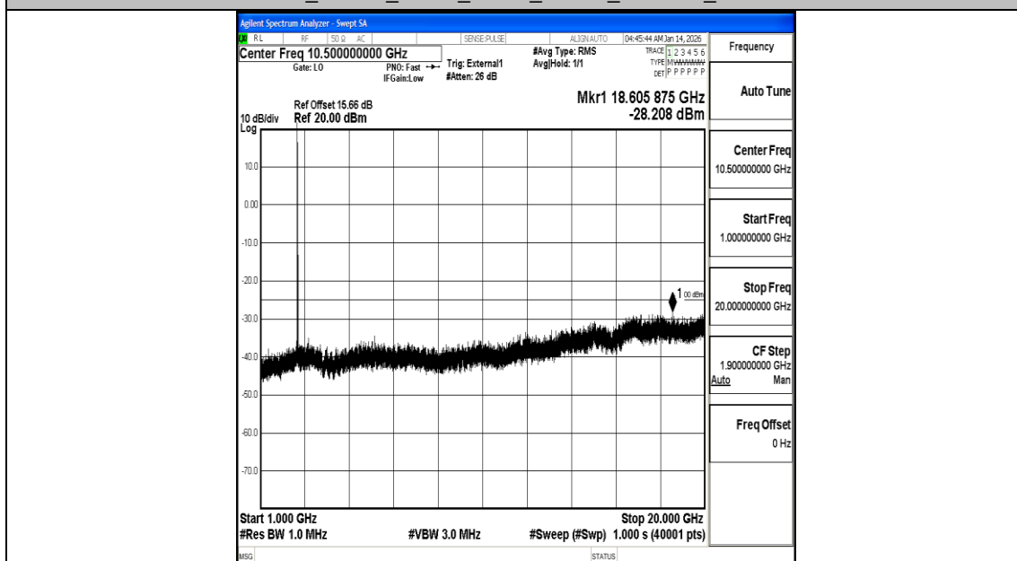
Band38_20MHz_QPSK_38000_1RB#0_1000~20000_1000~20000
