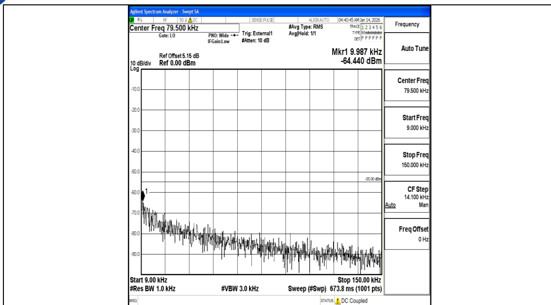
Band38_20MHz_QPSK_37850_1RB#0_0.009~0.15_0.009~0.15
