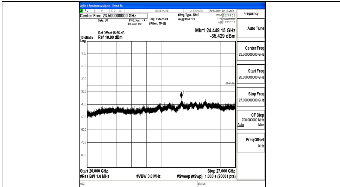
Band41_15MHz_QPSK_40620_1RB#0_20000~27000_20000~27000
