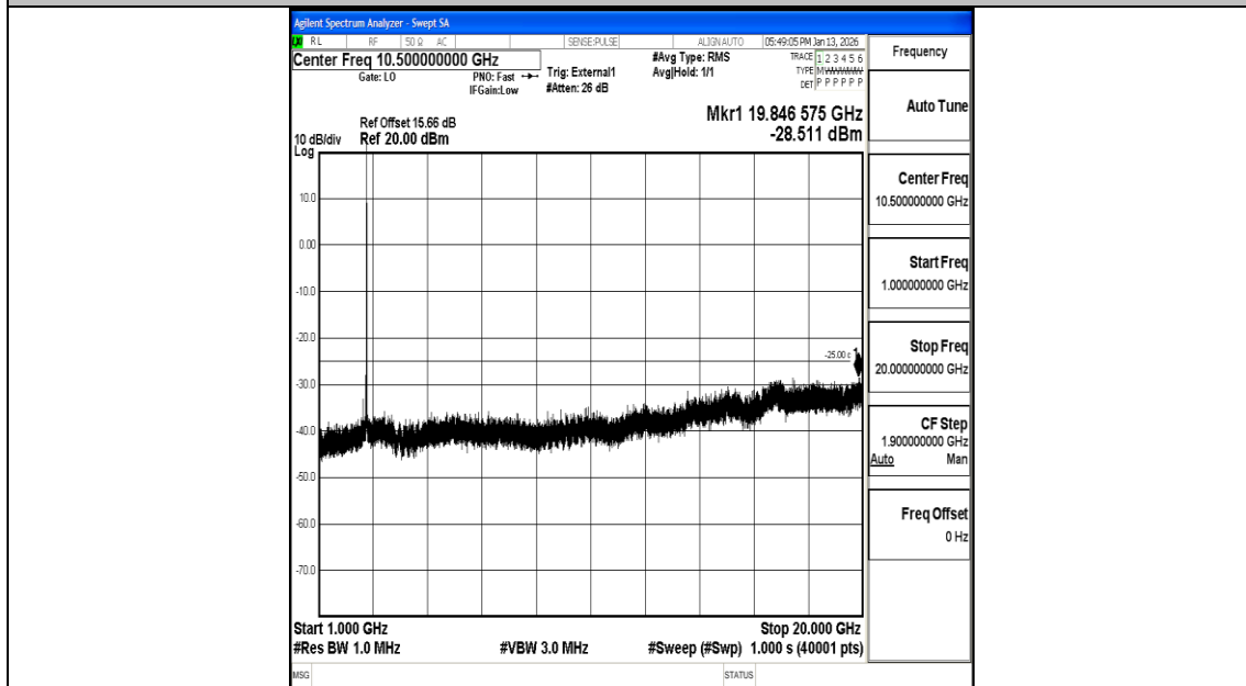
Band41_15MHz_QPSK_41515_1RB#0_1000~20000_1000~20000
