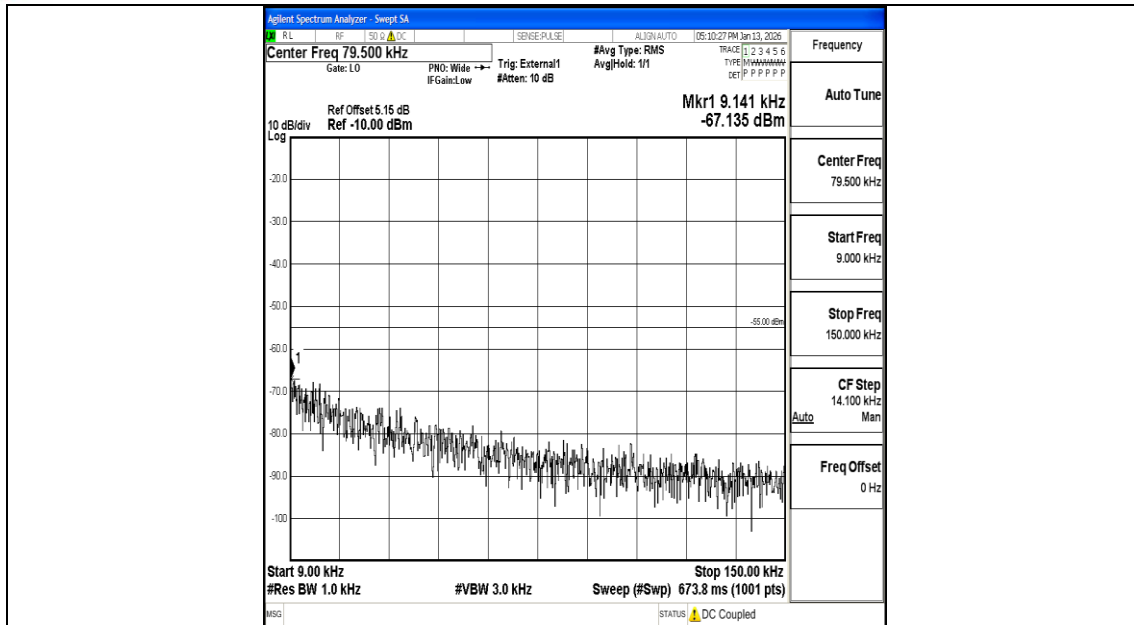
Band41_10MHz_QPSK_40620_1RB#0_0.009~0.15_0.009~0.15
