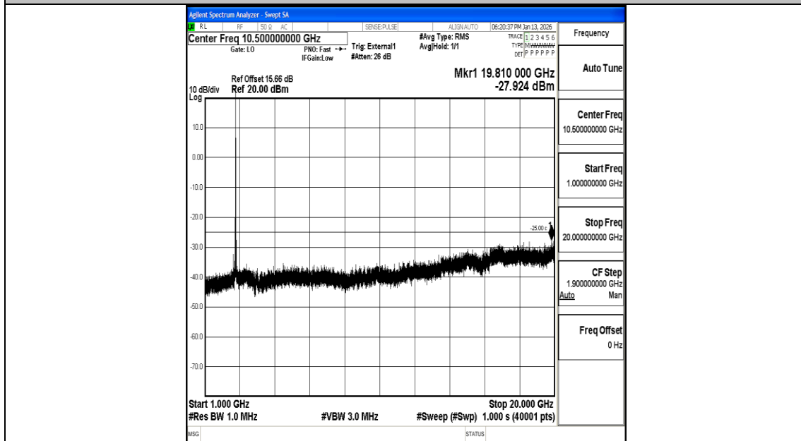
Band41_20MHz_QPSK_41490_1RB#0_1000~20000_1000~20000
