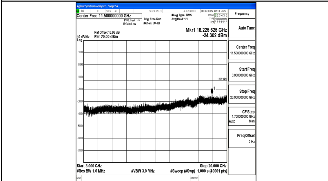
Band66_20MHz_16QAM_132322_1RB#0_3000~20000_3000~20000
