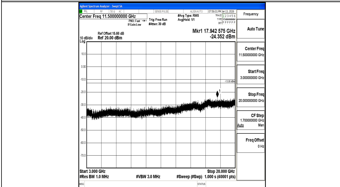
Band66_10MHz_16QAM_132622_1RB#0_3000~20000_3000~20000
