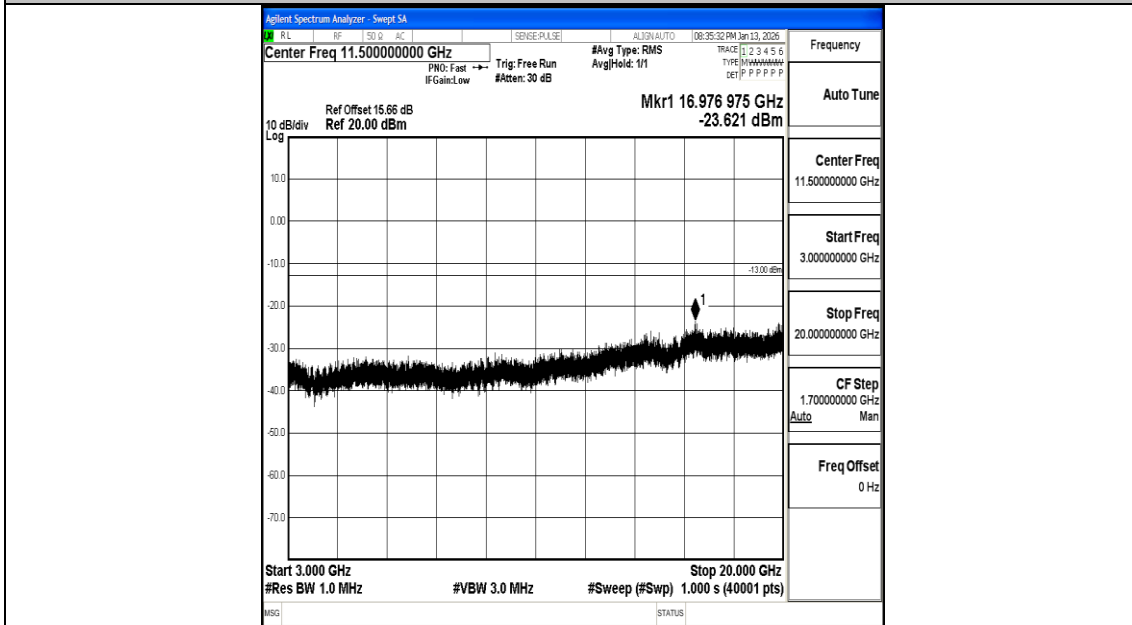
Band66_20MHz_16QAM_132072_1RB#0_3000~20000_3000~20000
