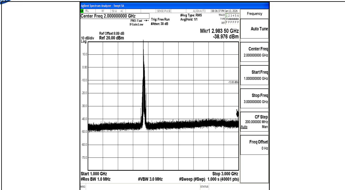
Band66_20MHz_16QAM_132322_1RB#0_1000~3000_1000~3000
