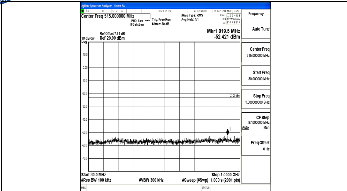
Band66_15MHz_QPSK_132597_1RB#0_30~1000_30~1000
