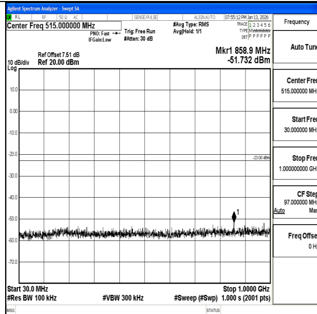
Band66_10MHz_QPSK_132622_1RB#0_30~1000_30~1000
