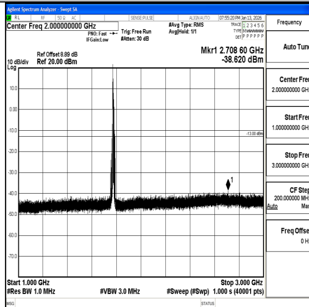
Band66_10MHz_QPSK_132622_1RB#0_1000~3000_1000~3000
