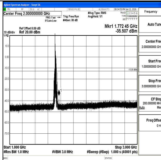
Band66_20MHz_QPSK_132072_1RB#0_1000~3000_1000~3000
