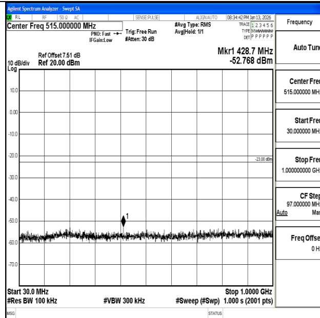
Band66_20MHz_QPSK_132072_1RB#0_30~1000_30~1000
