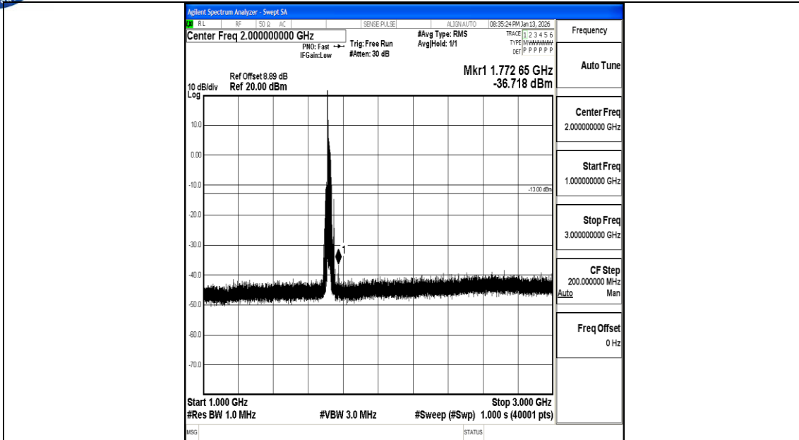
Band66_20MHz_16QAM_132072_1RB#0_1000~3000_1000~3000
