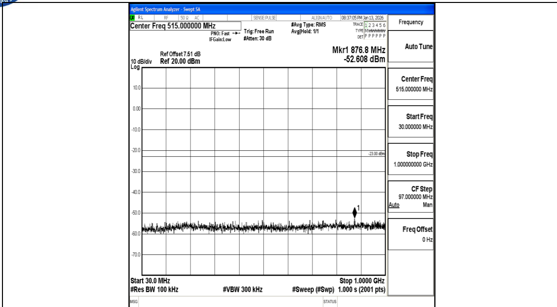
Band66_20MHz_QPSK_132572_1RB#0_30~1000_30~1000
