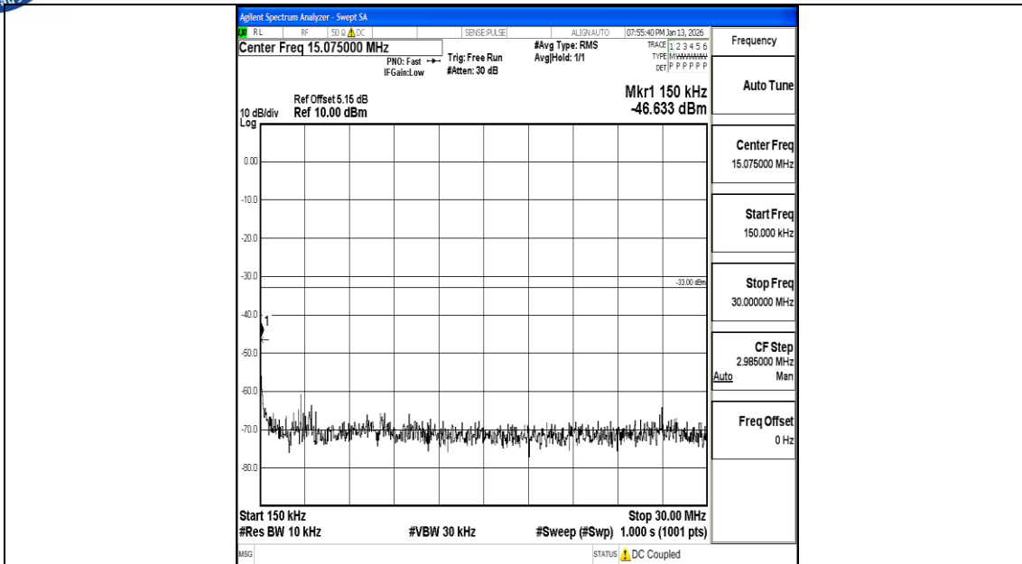
Band66_10MHz_16QAM_132622_1RB#0_0.15~30_0.15~30
