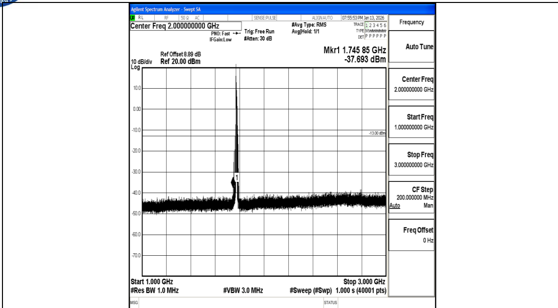
Band66_10MHz_16QAM_132622_1RB#0_1000~3000_1000~3000
