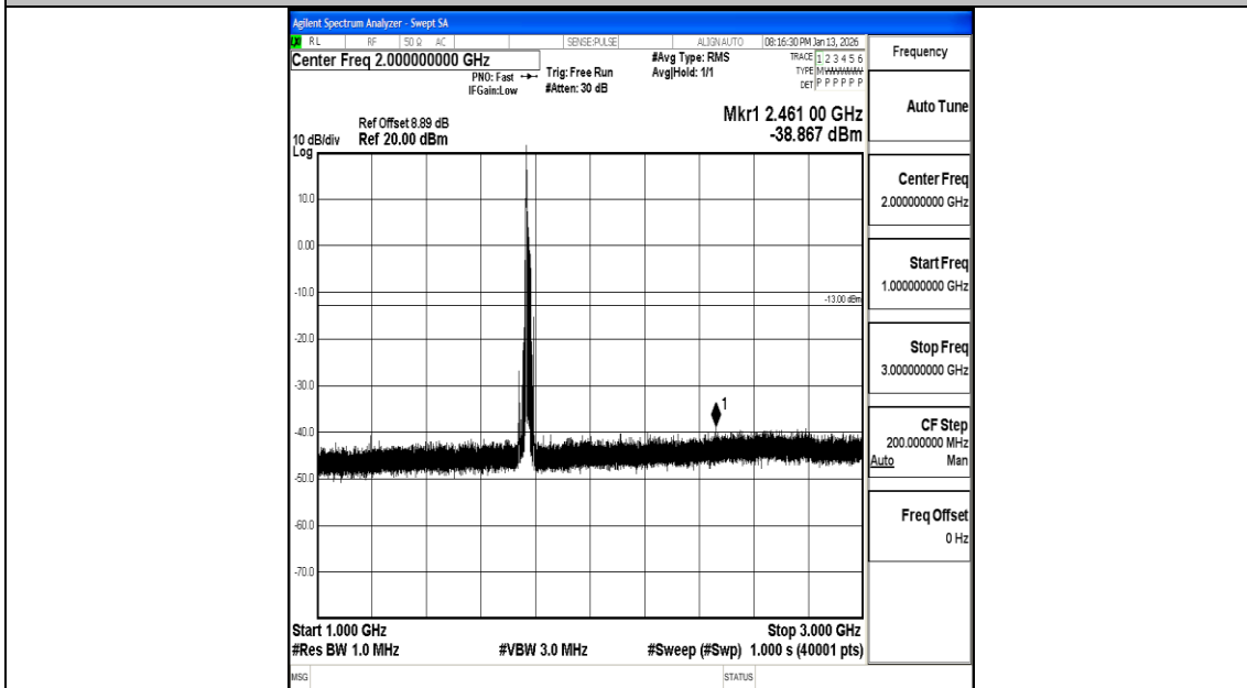
Band66_15MHz_QPSK_132597_1RB#0_1000~3000_1000~3000
