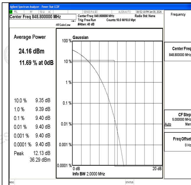
Channel 251 / 848.8 MHz
