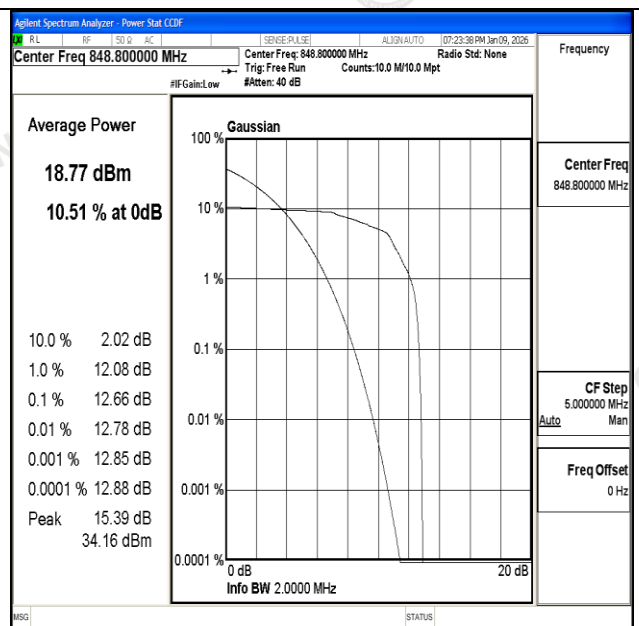
Channel 251 / 848.8 MHz
