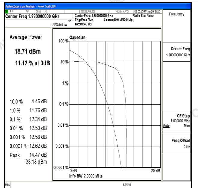
Channel 661 / 1880 MHz
