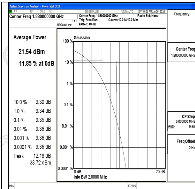
Channel 661 / 1880 MHz
