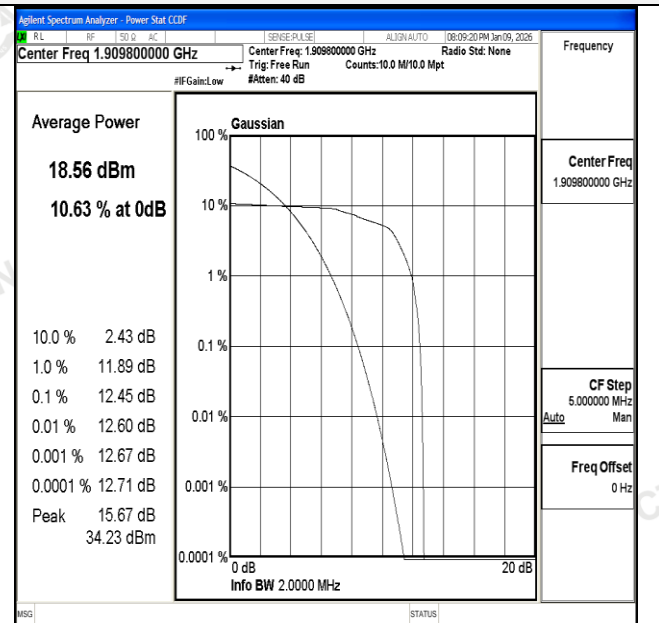
Channel 810 / 1909.8 MHz
