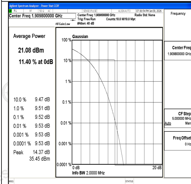
Channel 810 / 1909.8 MHz
