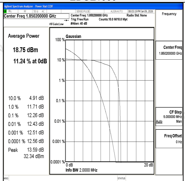
Channel 512 / 1850.2 MHz
