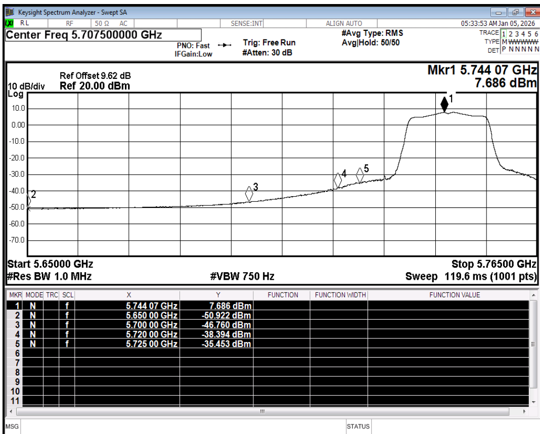
Restrict Band NVNT ac20 5745MHz Ant1 Average
