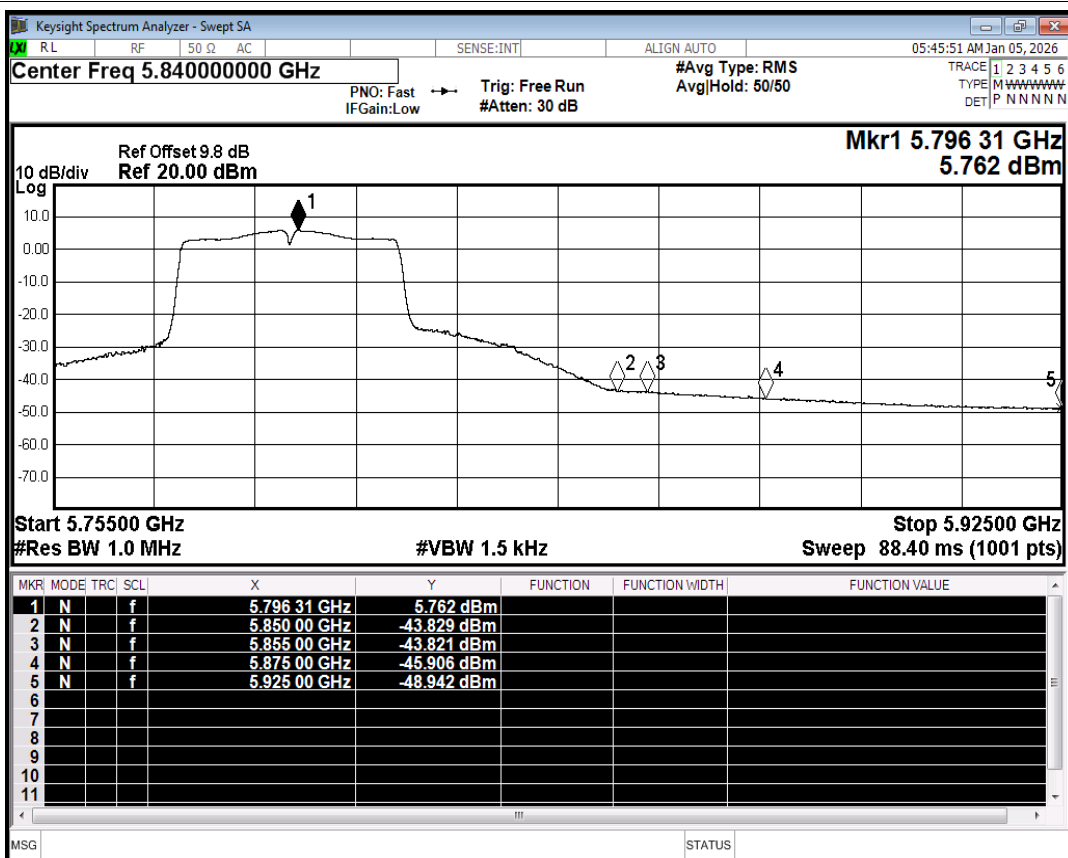
Restrict Band NVNT n40 5795MHz Ant1 Average
