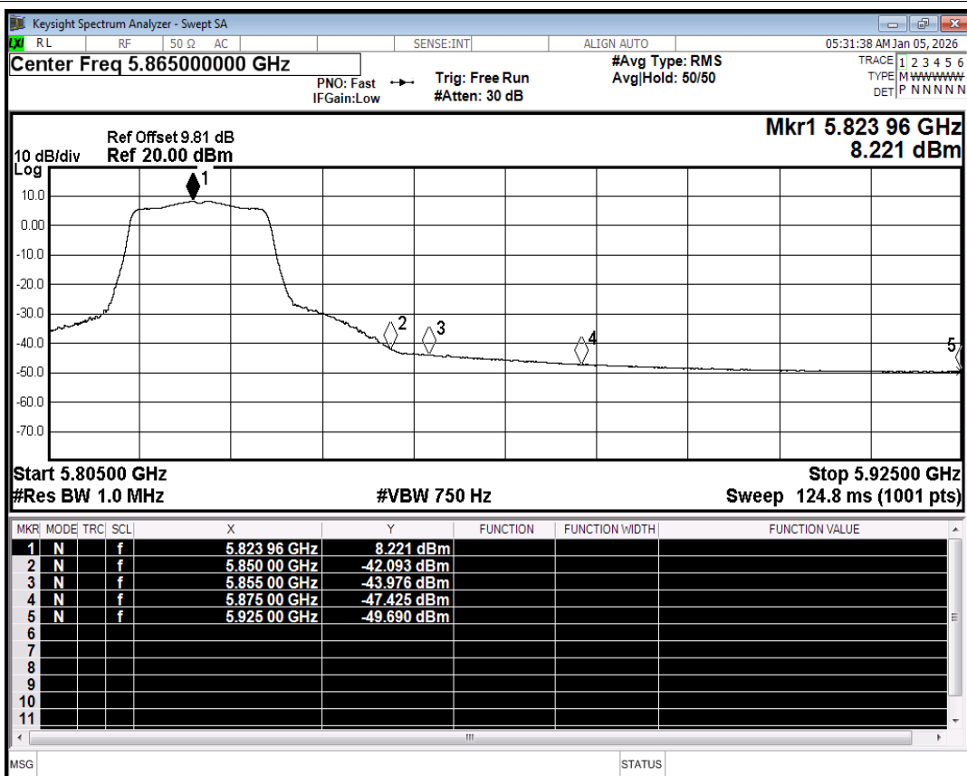
Restrict Band NVNT n20 5825MHz Ant1 Average
