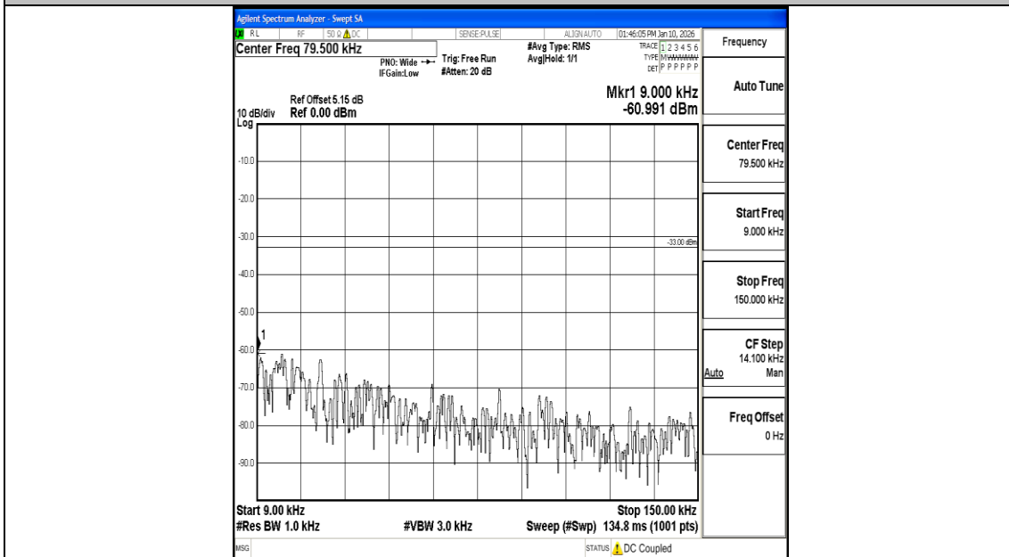
Band26_1.4MHz_16QAM_26915_1RB#0_0.009~0.15_0.009~0.15
