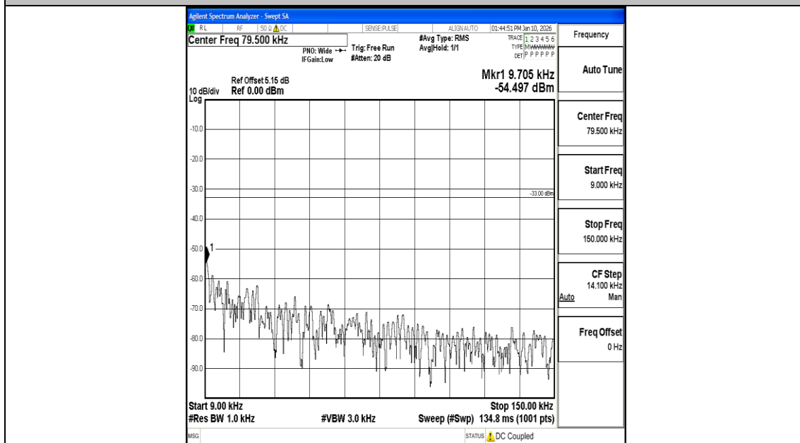
Band26_1.4MHz_16QAM_26797_1RB#0_0.009~0.15_0.009~0.15
