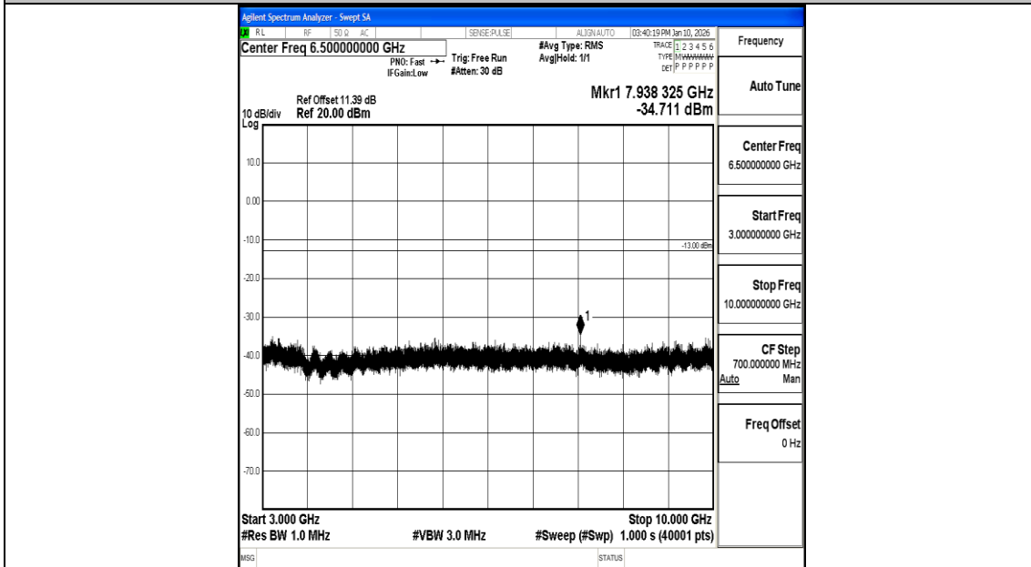
Band26_10MHz_16QAM_26840_1RB#0_3000~10000_3000~10000
