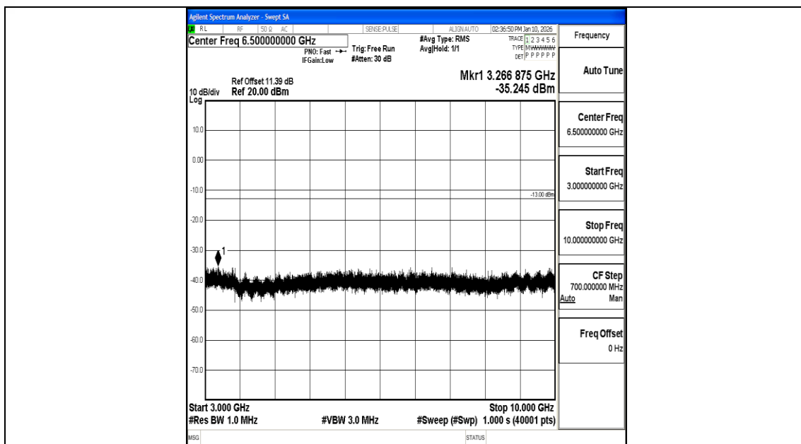
Band26_3MHz_QPSK_27025_1RB#0_3000~10000_3000~10000
