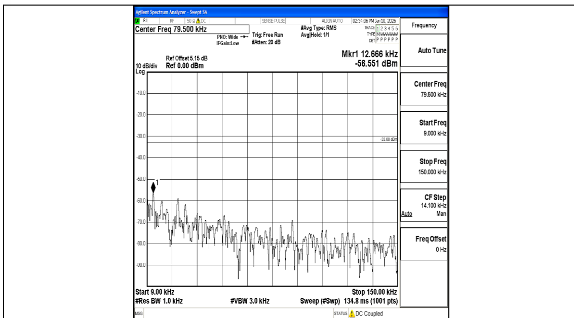
Band26_3MHz_QPSK_26805_1RB#0_0.009~0.15_0.009~0.15
