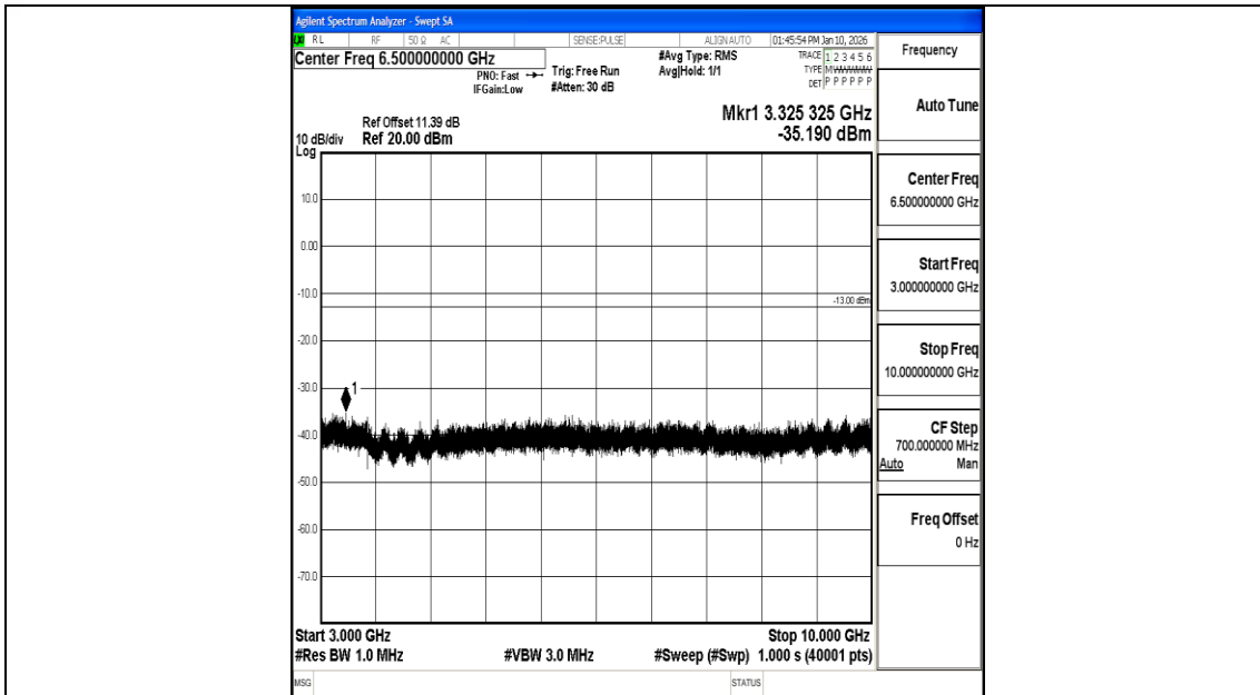
Band26_1.4MHz_QPSK_26915_1RB#0_3000~10000_3000~10000
