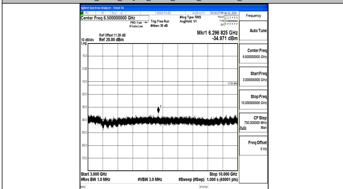
Band26_5MHz_16QAM_27015_1RB#0_3000~10000_3000~10000
