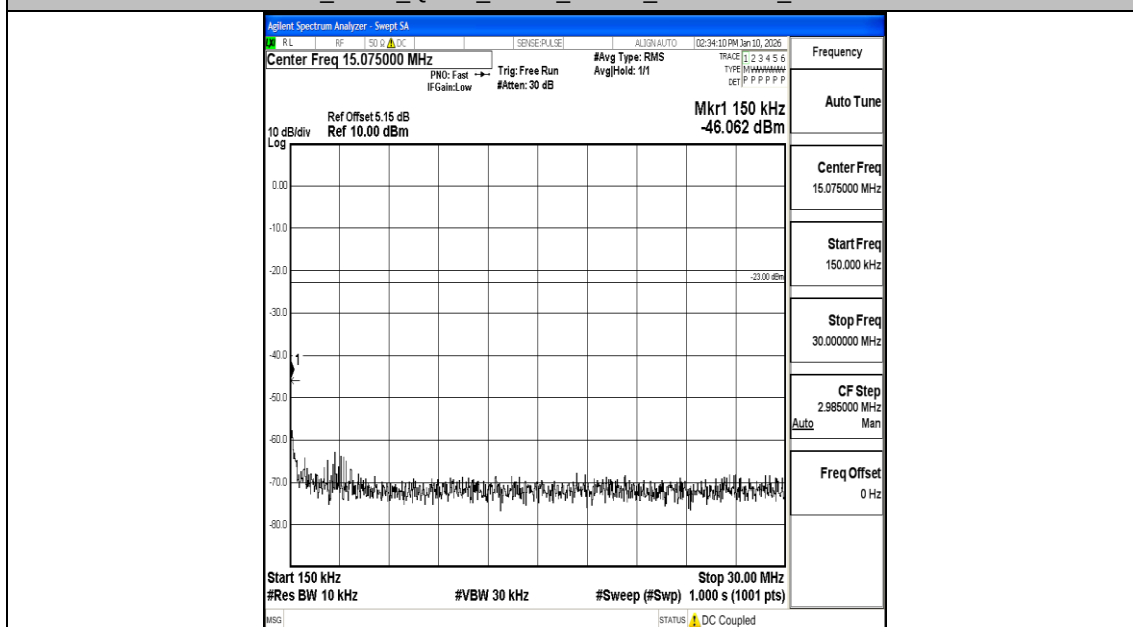
Band26_3MHz_QPSK_26805_1RB#0_0.15~30_0.15~30
