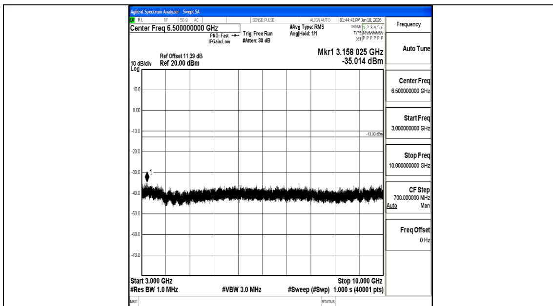
Band26_1.4MHz_QPSK_26797_1RB#0_3000~10000_3000~10000
