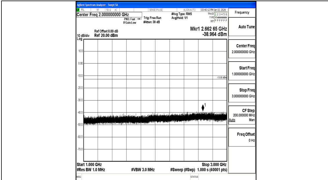
Band26_10MHz_16QAM_26840_1RB#0_1000~3000_1000~3000
