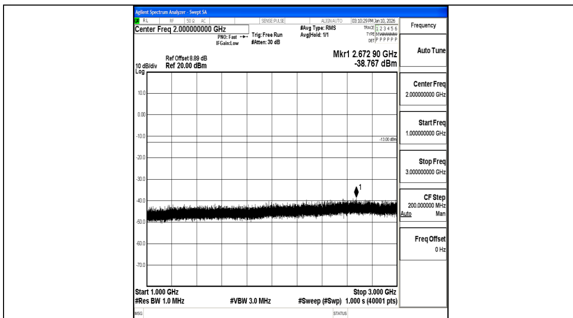
Band26_5MHz_16QAM_27015_1RB#0_1000~3000_1000~3000
