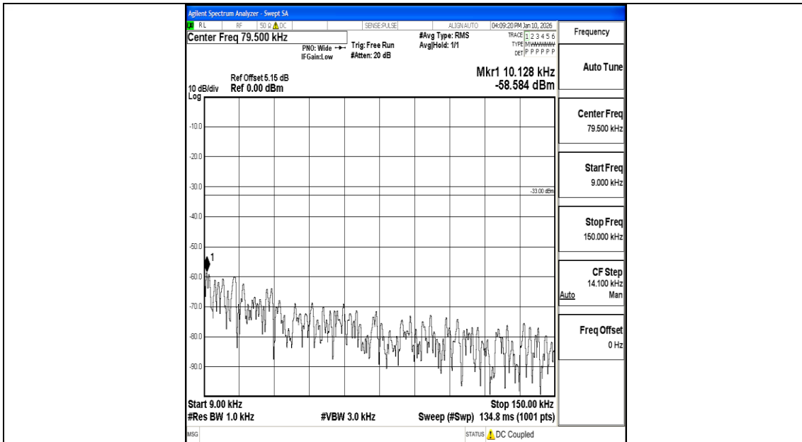
Band26_15MHz_QPSK_26965_1RB#0_0.009~0.15_0.009~0.15
