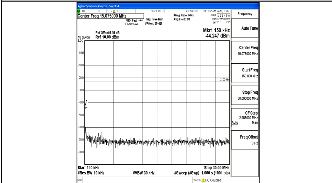
Band26_15MHz_QPSK_26965_1RB#0_0.15~30_0.15~30
