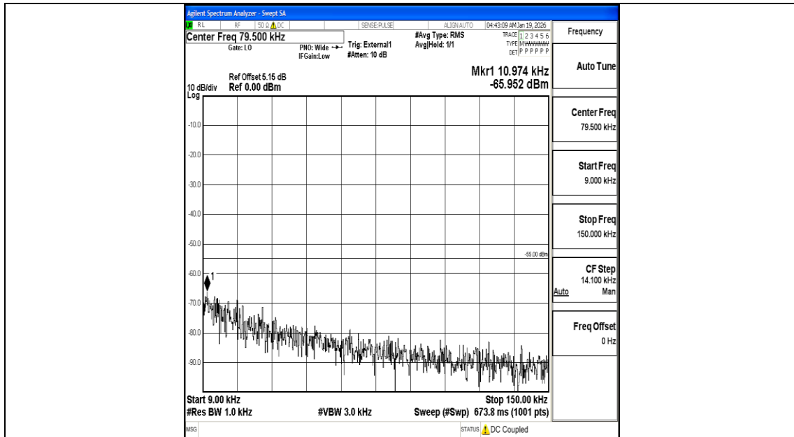
Band38_10MHz_QPSK_38000_1RB#0_0.009~0.15_0.009~0.15
