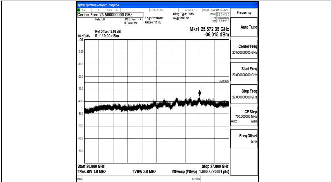
Band38_15MHz_QPSK_38175_1RB#0_20000~27000_20000~27000
