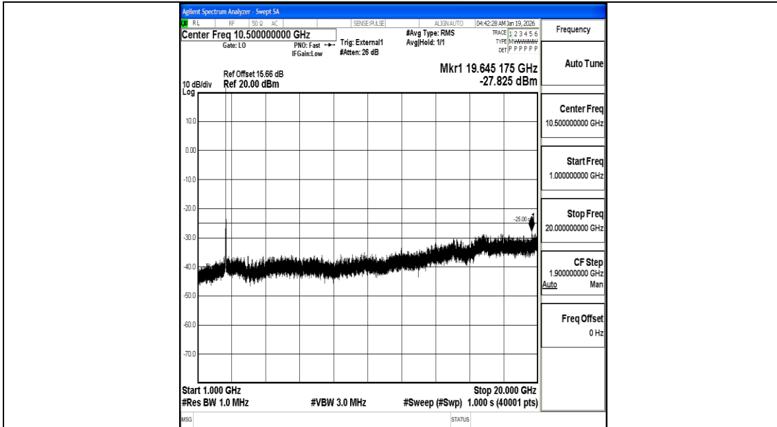
Band38_10MHz_16QAM_37800_1RB#0_1000~20000_1000~20000
