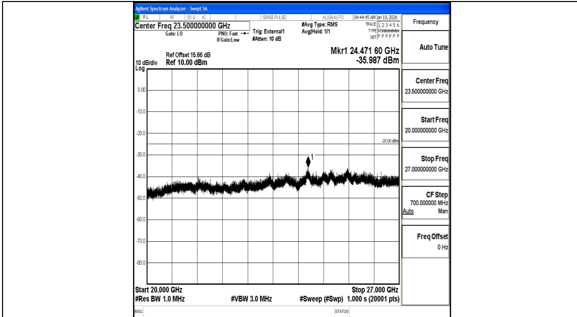
Band38_10MHz_QPSK_38000_1RB#0_20000~27000_20000~27000
