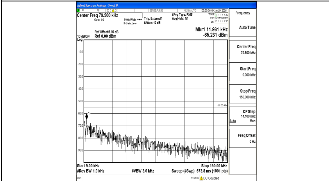
Band38_20MHz_16QAM_38150_1RB#0_0.009~0.15_0.009~0.15
