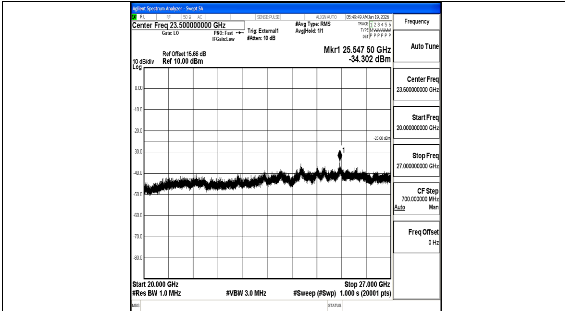
Band38_20MHz_QPSK_38150_1RB#0_20000~27000_20000~27000
