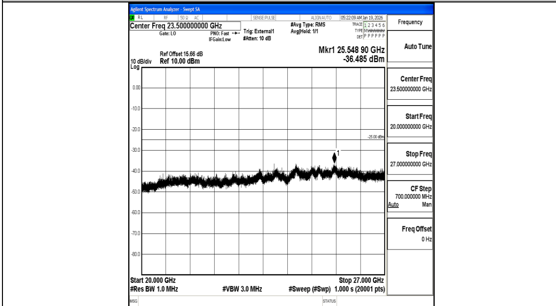
Band38_15MHz_16QAM_38175_1RB#0_20000~27000_20000~27000
