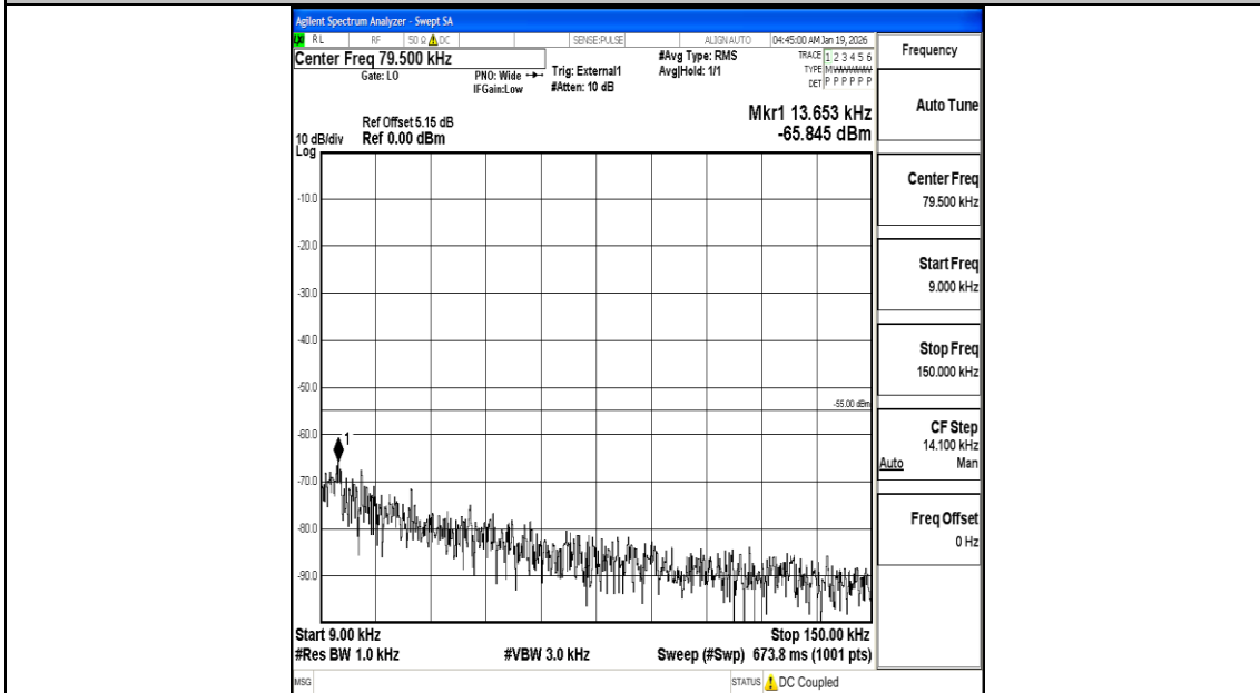
Band38_10MHz_16QAM_38000_1RB#0_0.009~0.15_0.009~0.15
