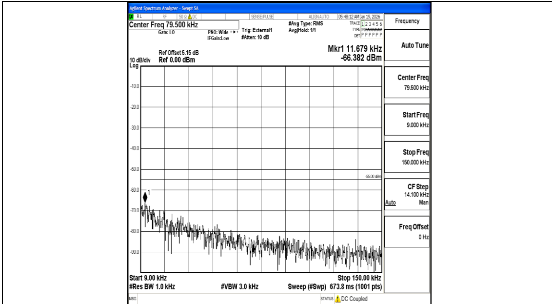
Band38_20MHz_QPSK_38150_1RB#0_0.009~0.15_0.009~0.15
