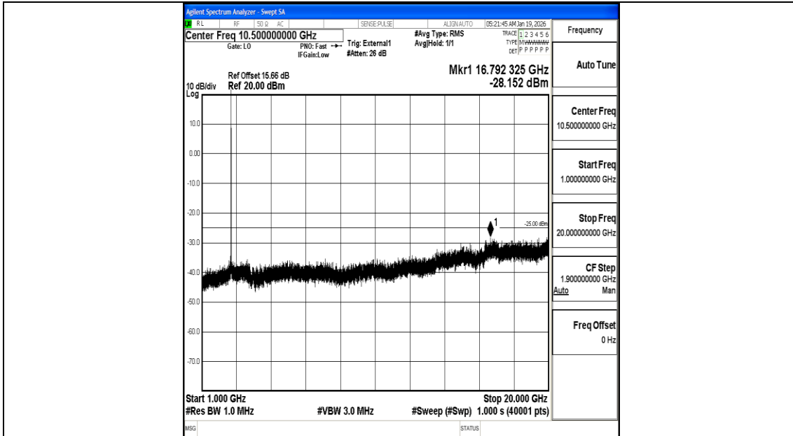
Band38_15MHz_16QAM_38175_1RB#0_1000~20000_1000~20000
