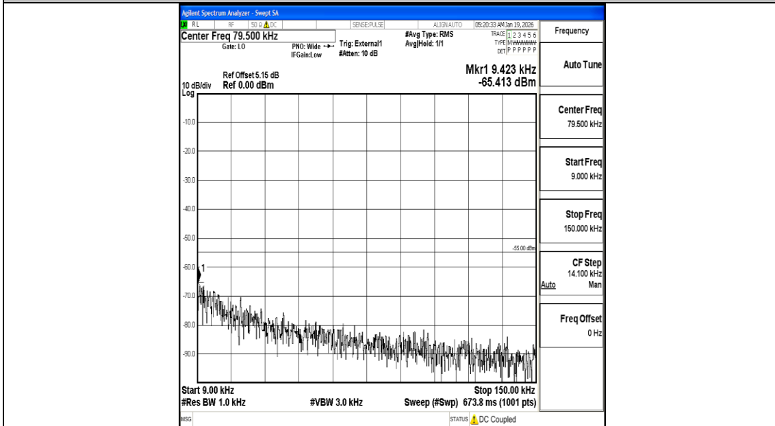
Band38_15MHz_16QAM_38175_1RB#0_0.009~0.15_0.009~0.15
