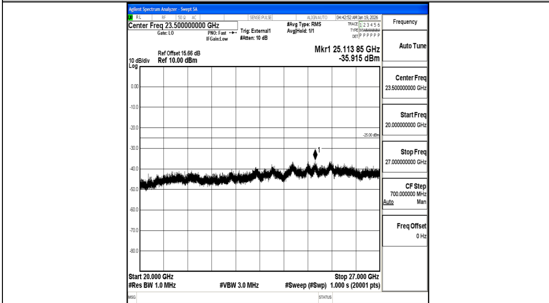
Band38_10MHz_16QAM_37800_1RB#0_20000~27000_20000~27000
