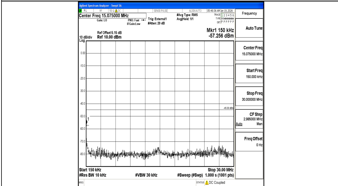
Band38_20MHz_QPSK_38150_1RB#0_0.15~30_0.15~30
