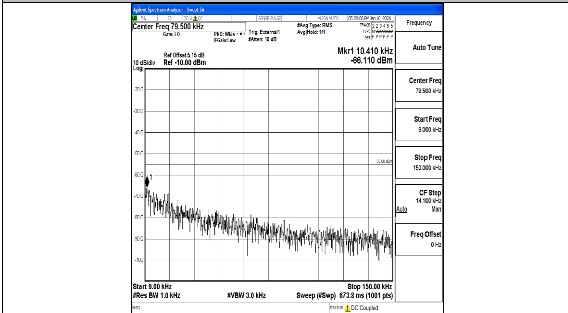
Band41_10MHz_16QAM_39700_1RB#0_0.009~0.15_0.009~0.15
