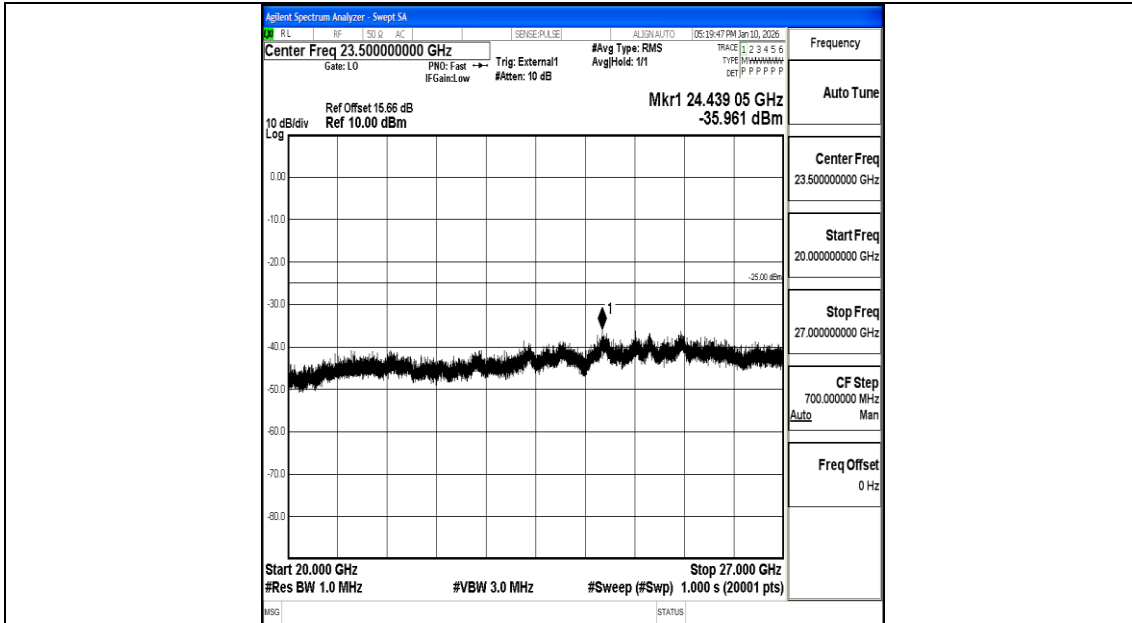
Band41_10MHz_QPSK_39700_1RB#0_20000~27000_20000~27000
