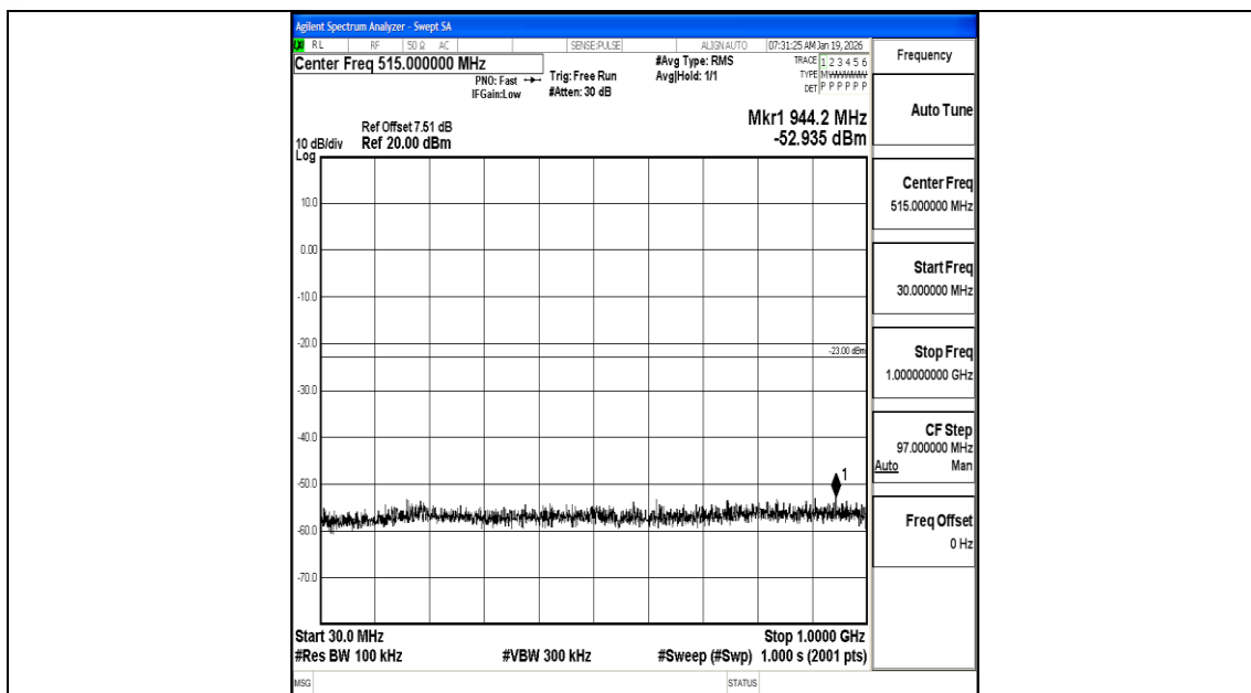
Band66_15MHz_16QAM_132597_1RB#0_30~1000_30~1000
