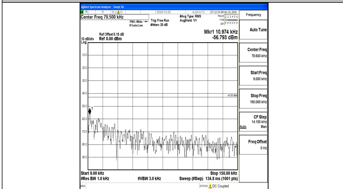
Band66_10MHz_QPSK_132622_1RB#0_0.009~0.15_0.009~0.15
