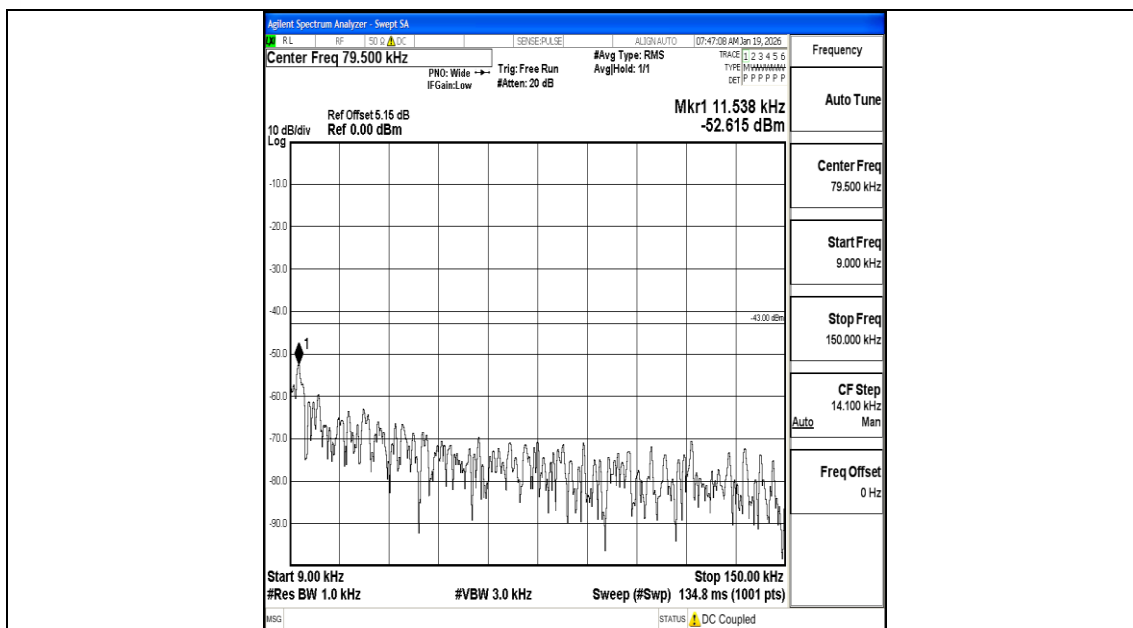
Band66_20MHz_16QAM_132072_1RB#0_0.009~0.15_0.009~0.15
