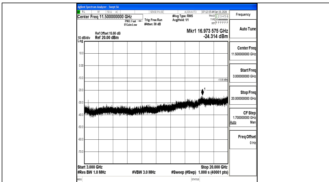
Band66_10MHz_16QAM_132322_1RB#0_3000~20000_3000~20000
