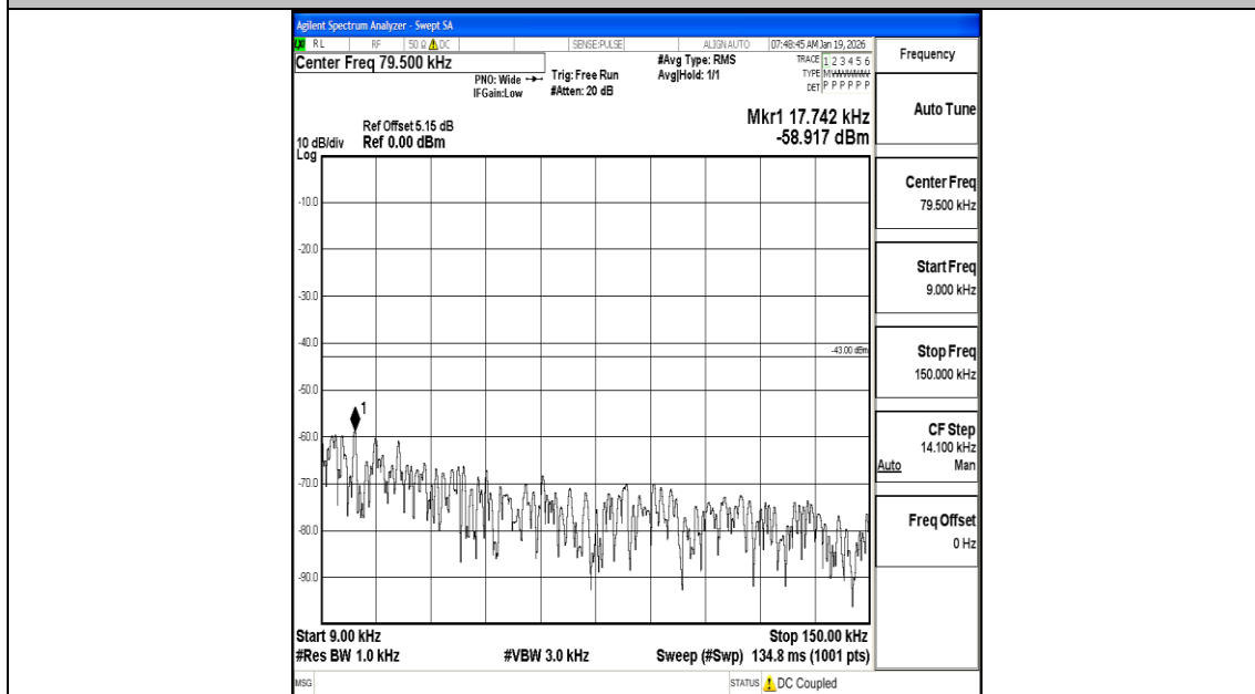
Band66_20MHz_QPSK_132572_1RB#0_0.009~0.15_0.009~0.15
