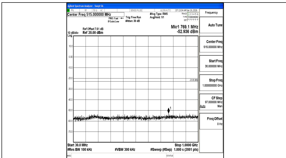
Band66_10MHz_16QAM_132622_1RB#0_30~1000_30~1000
