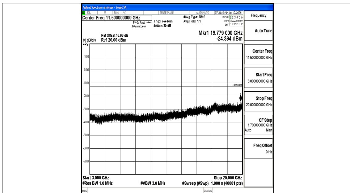
Band66_15MHz_16QAM_132597_1RB#0_3000~20000_3000~20000
