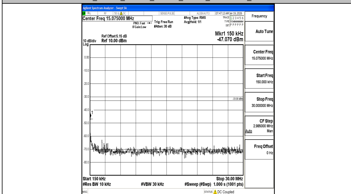
Band66_20MHz_16QAM_132072_1RB#0_0.15~30_0.15~30
