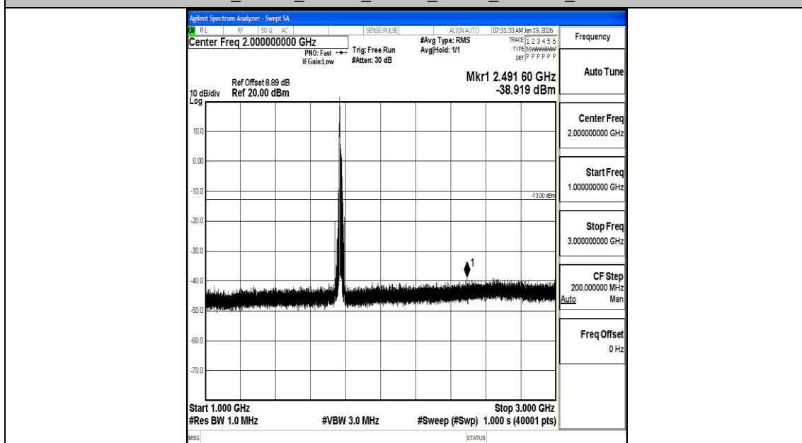
Band66_15MHz_16QAM_132597_1RB#0_1000~3000_1000~3000
