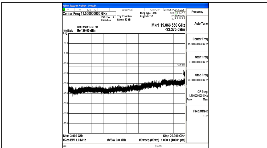
Band66_20MHz_16QAM_132322_1RB#0_3000~20000_3000~20000
