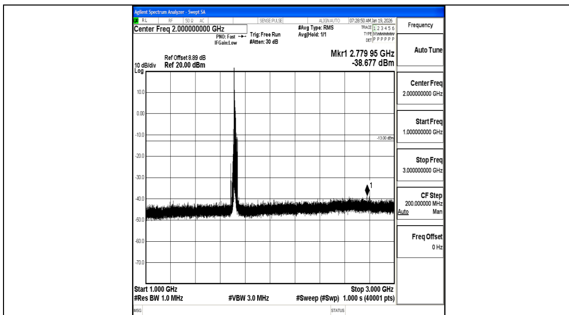
Band66_15MHz_QPSK_132047_1RB#0_1000~3000_1000~3000
