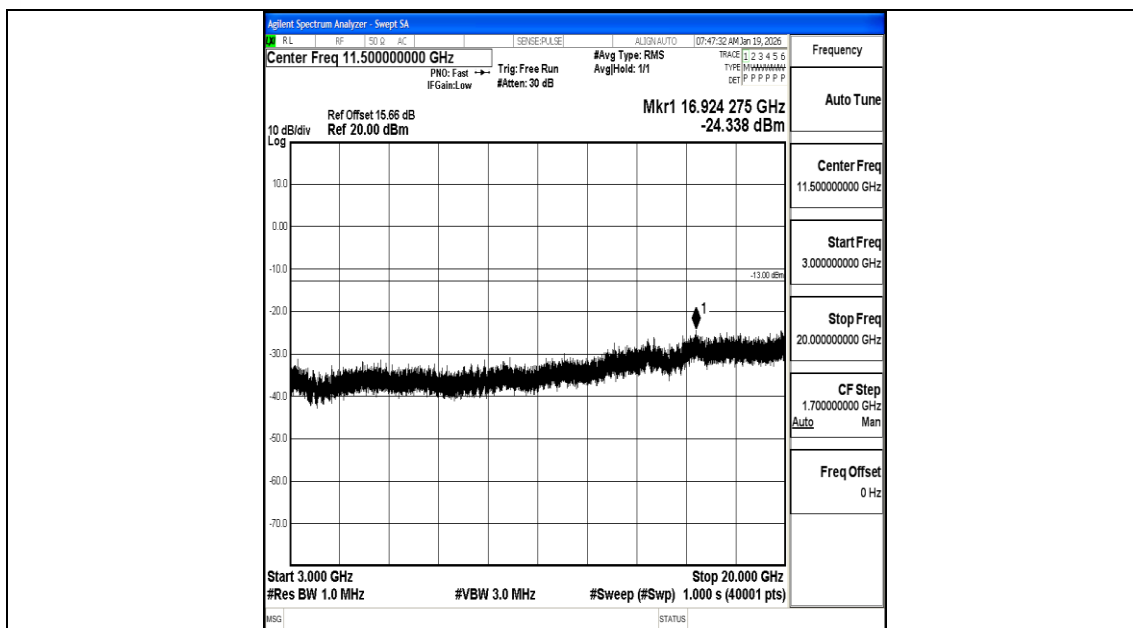
Band66_20MHz_16QAM_132072_1RB#0_3000~20000_3000~20000
