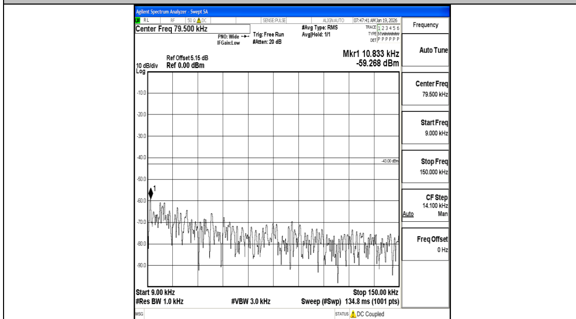
Band66_20MHz_QPSK_132322_1RB#0_0.009~0.15_0.009~0.15
