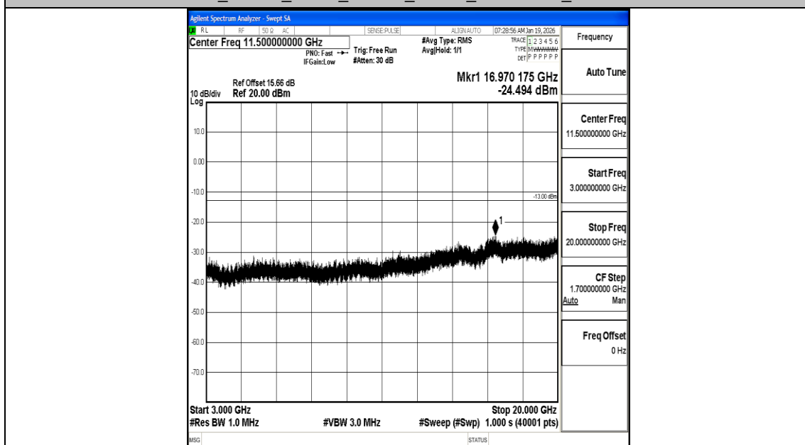
Band66_15MHz_QPSK_132047_1RB#0_3000~20000_3000~20000
