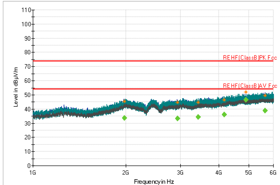
Figure 31: Radiated Emissions, Mid Channel from 1GHz – 6GHz
