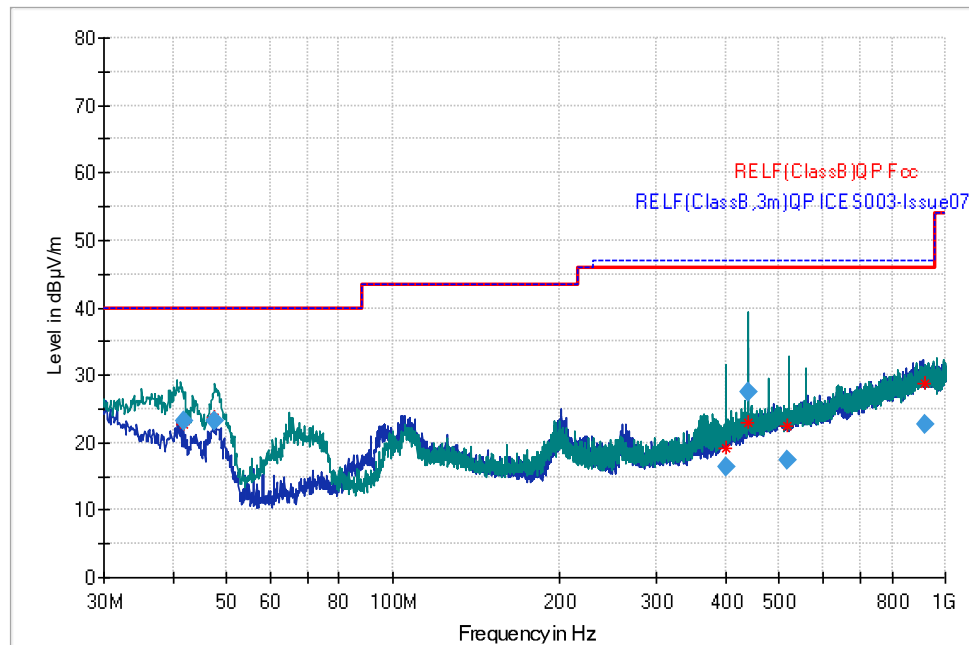
Figure 26: Radiated Emissions, Factory mode from 30MHz to 1GHz
