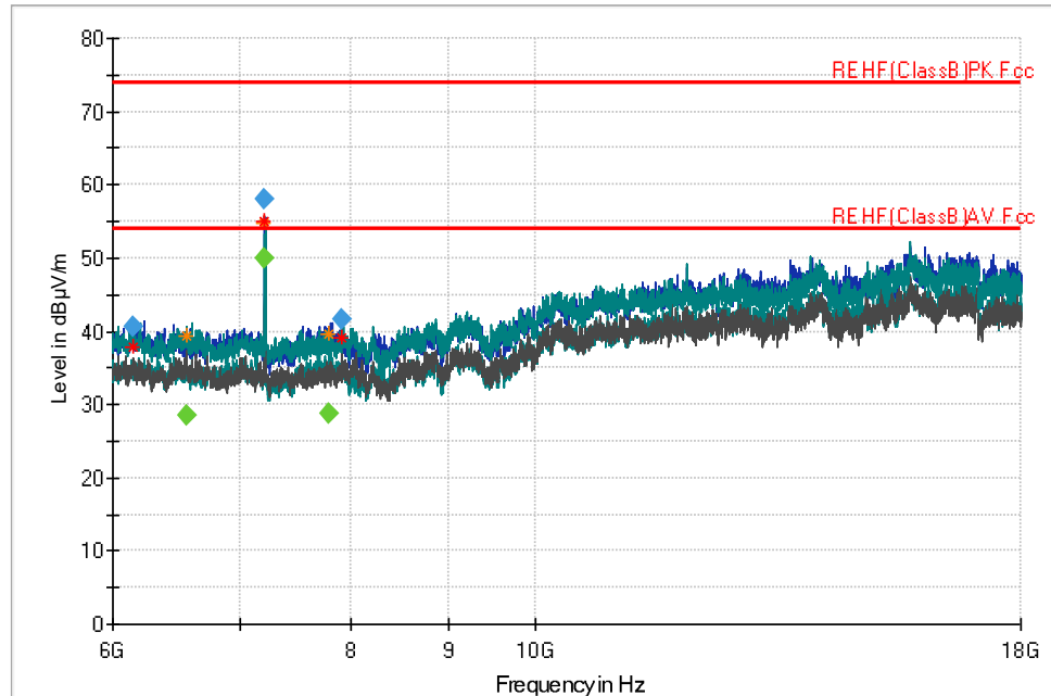
Figure 33: Radiated Emissions, Low Channel from 6GHz – 18GHz
