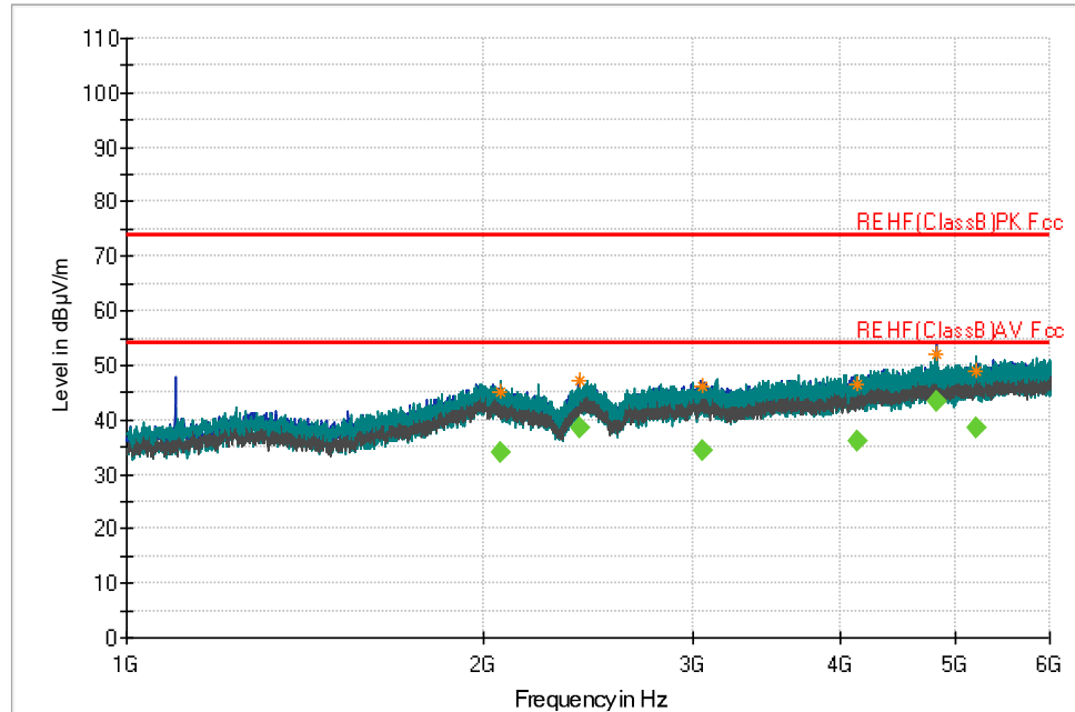
Figure 30: Radiated Emissions, Low Channel from 1GHz – 6GHz
