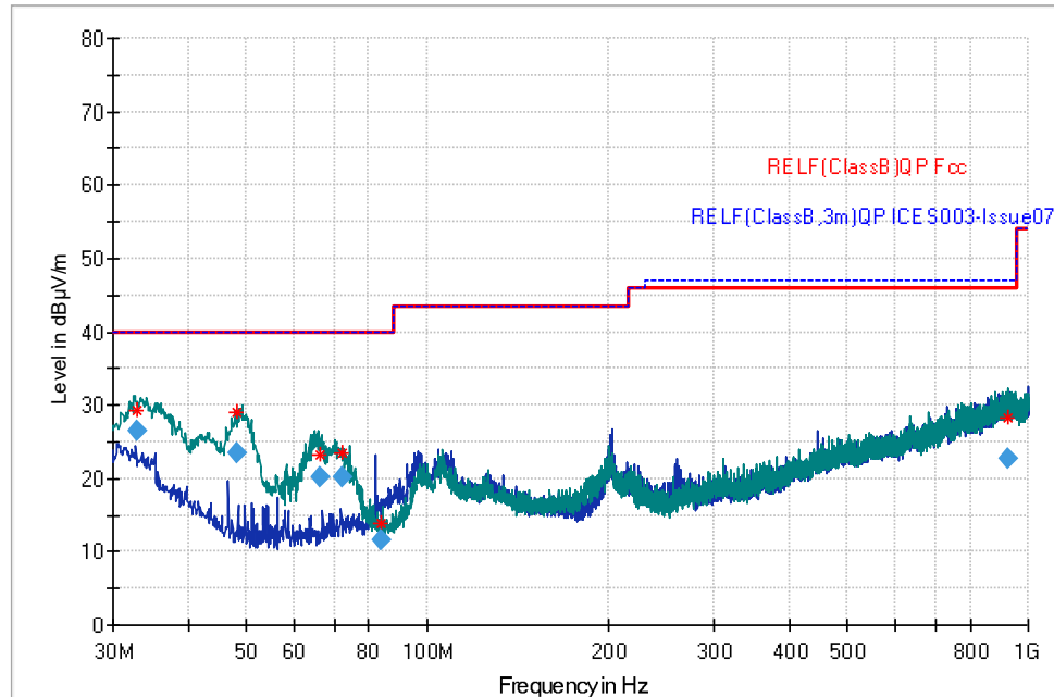
Figure 27: Radiated Emissions, Low Channel from 30MHz to 1GHz
