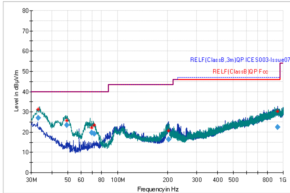
Figure 29: Radiated Emissions, High Channel from 30MHz to 1GHz
