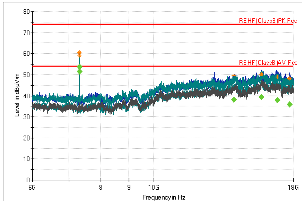
Figure 34: Radiated Emissions, Mid Channel from 6GHz – 18GHz
