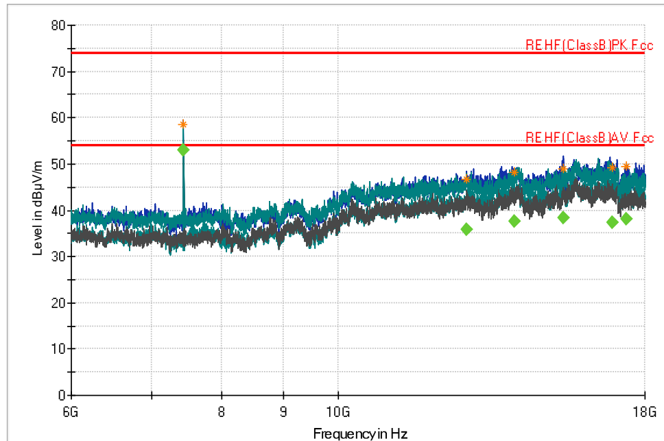
Figure 35: Radiated Emissions, High Channel from 6GHz – 18GHz
