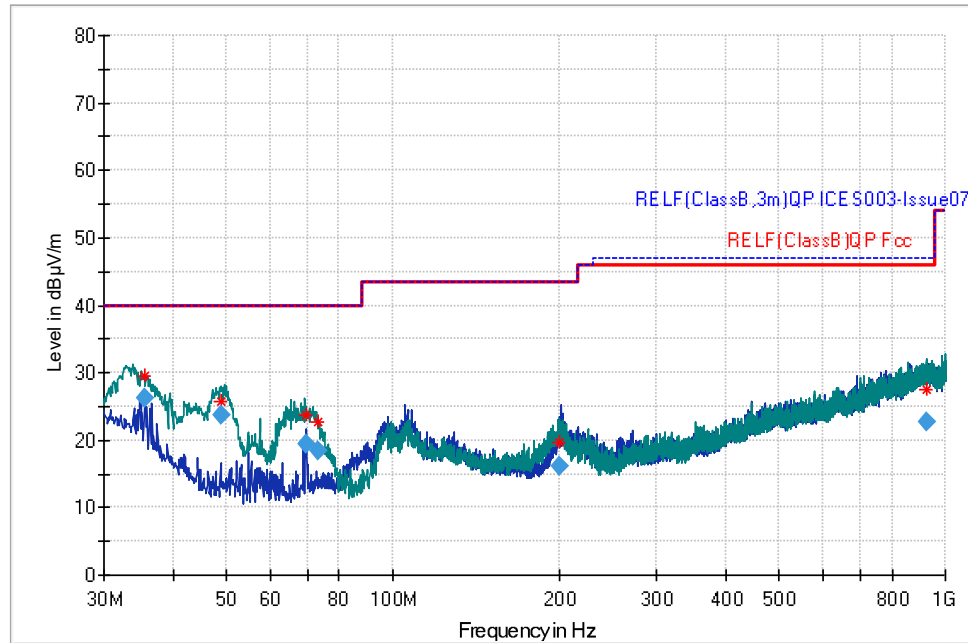
Figure 28: Radiated Emissions, Mid Channel from 30MHz to 1GHz
