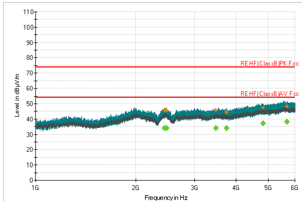
Figure 32: Radiated Emissions, High Channel from 1GHz – 6GHz
