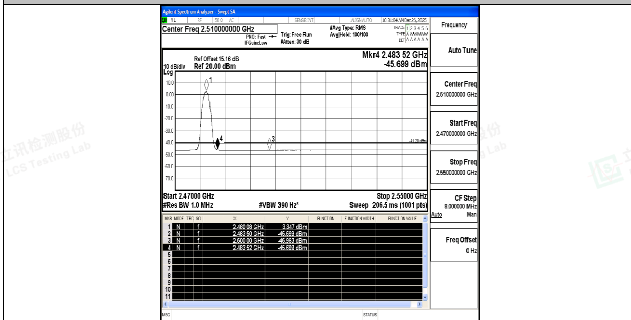
2DH5-Ant1-2480-PASS
