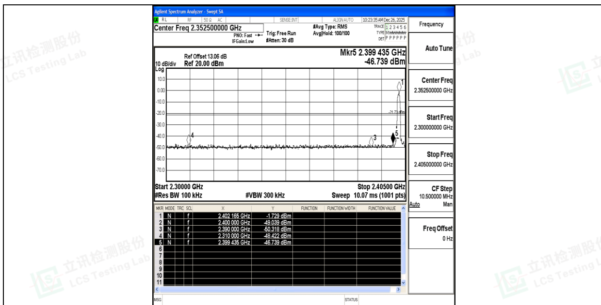
2DH5-Ant1-2402-PASS
