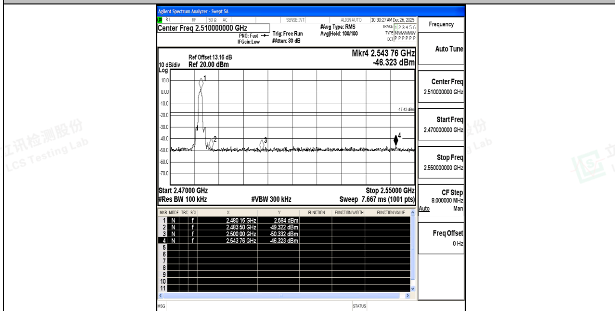
2DH5-Ant1-2480-PASS
