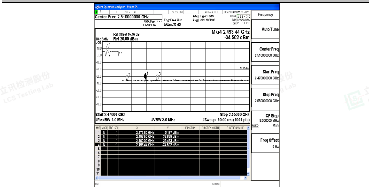
DH5-Ant1-Hop_2480-PASS
