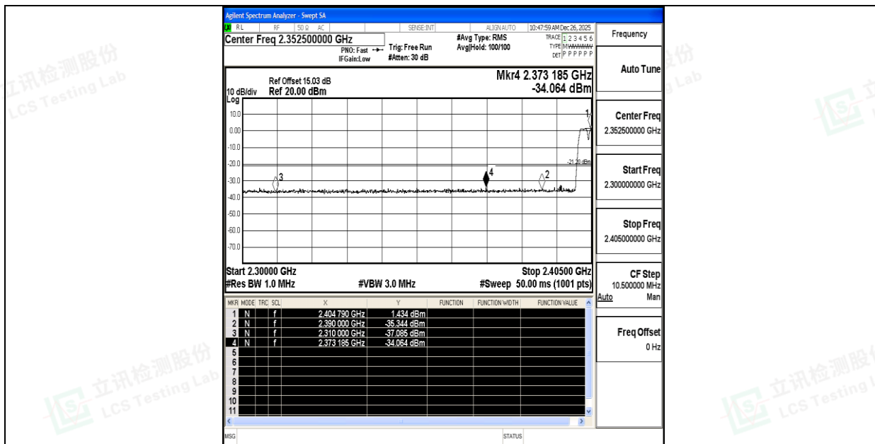
DH5-Ant1-Hop_2402-PASS
