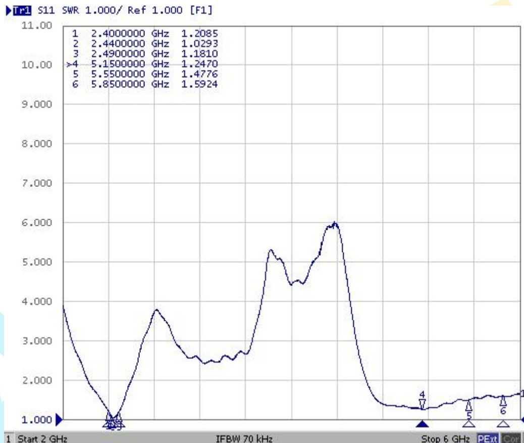
Figure 2: Model PD243035-T4-170G1303 VSWR
