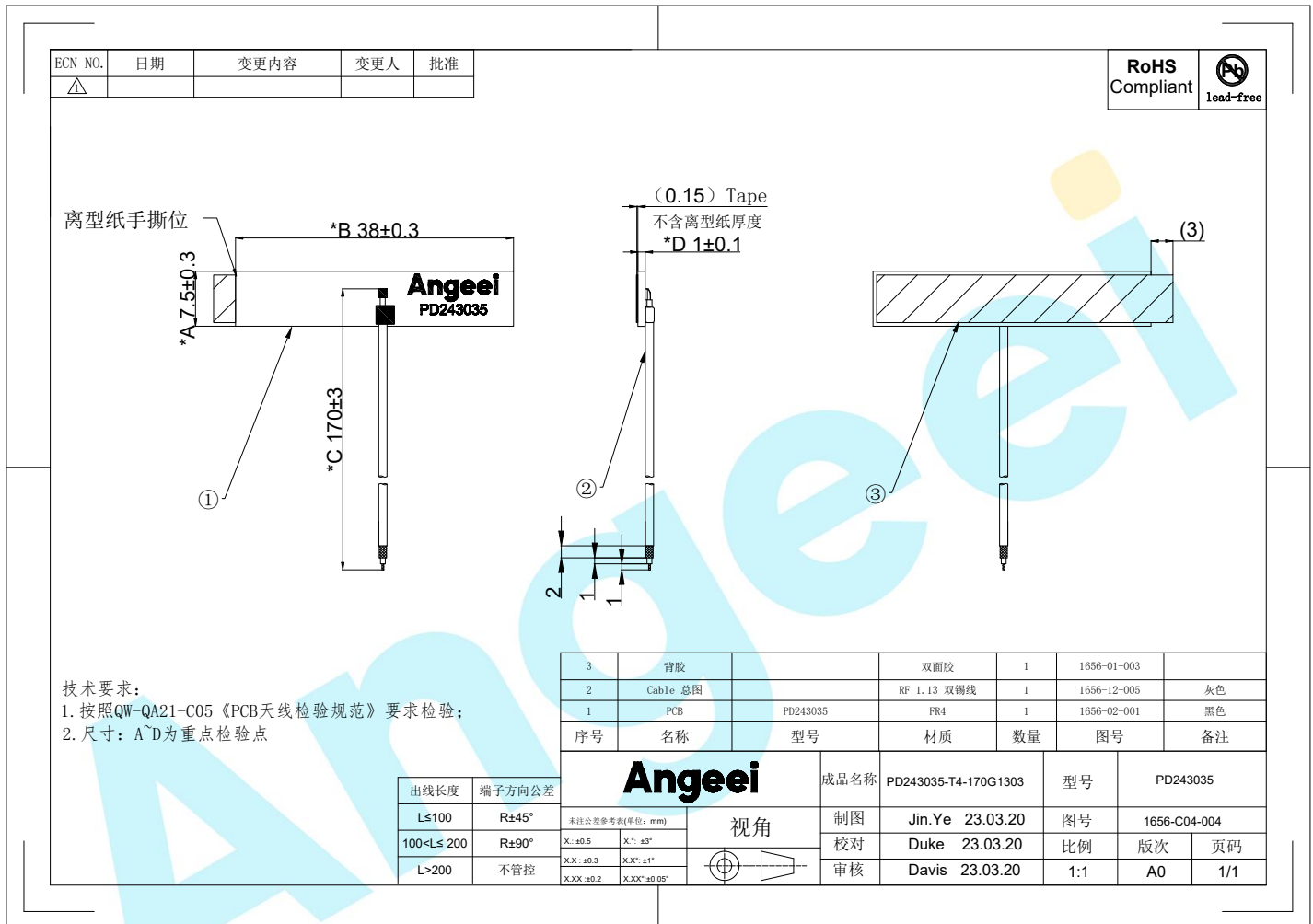
Figure 6: Model PD243035-T4-170G1303 Dimensions
