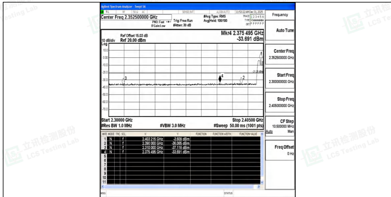
DH5-Ant1-Hop_2402-PASS
