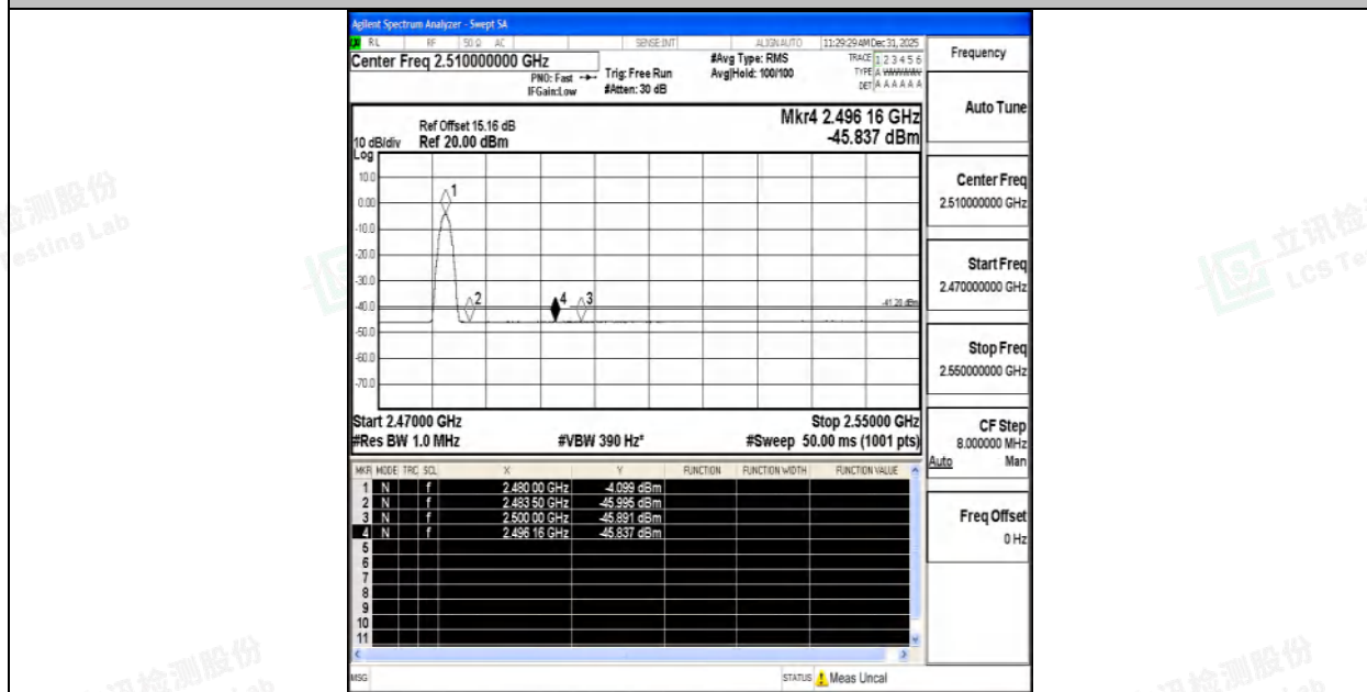
DH5-Ant1-2480-PASS
