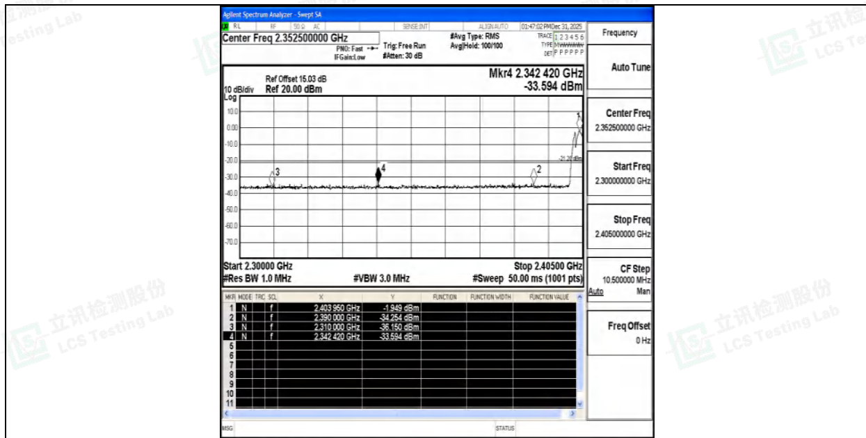
3DH5-Ant1-Hop_2402-PASS
