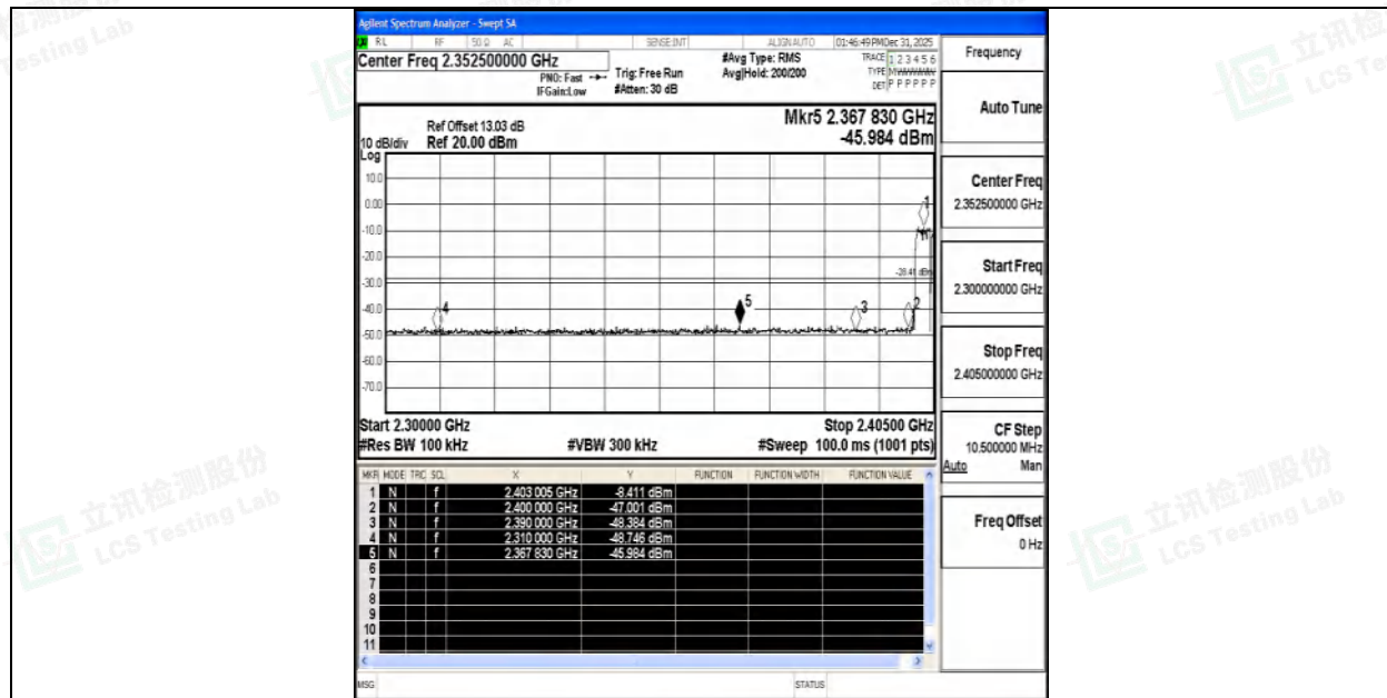
3DH5-Ant1-Hop_2402-PASS
