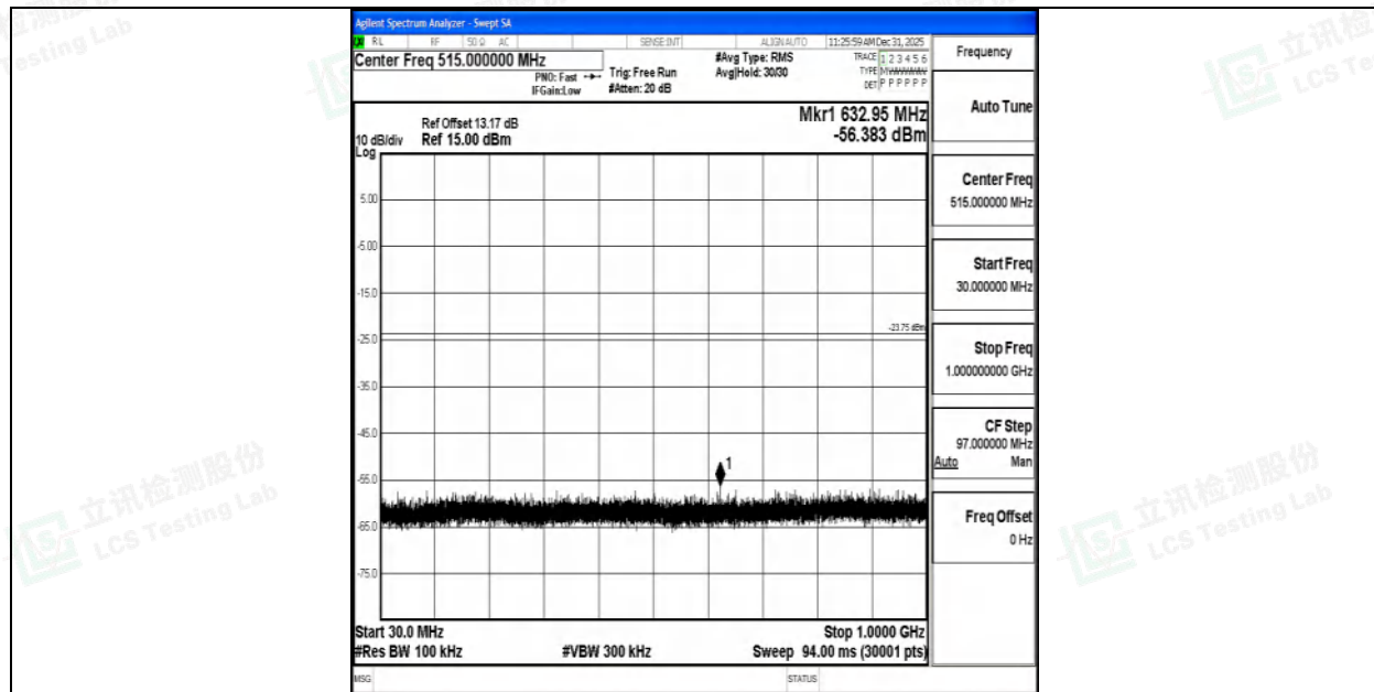
DH5-Ant1-2441-30~1000-PASS
