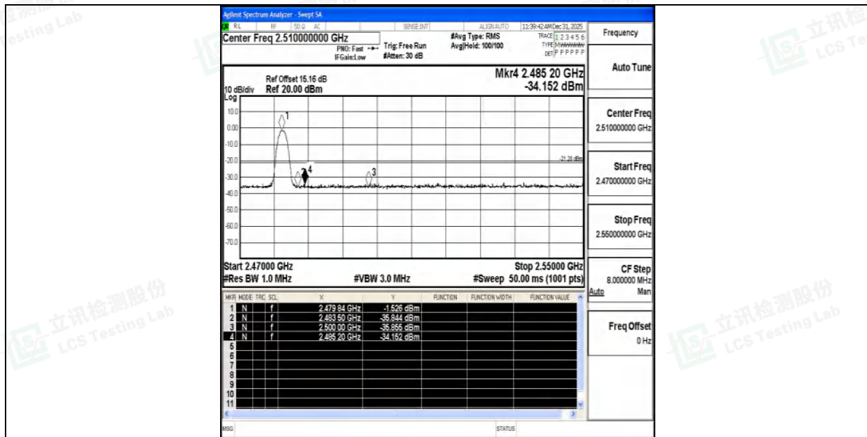
2DH5-Ant1-2480-PASS
