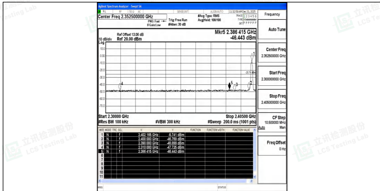
2DH5-Ant1-2402-PASS
