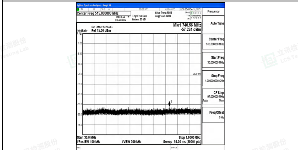
3DH5-Ant1-2480-30~1000-PASS
