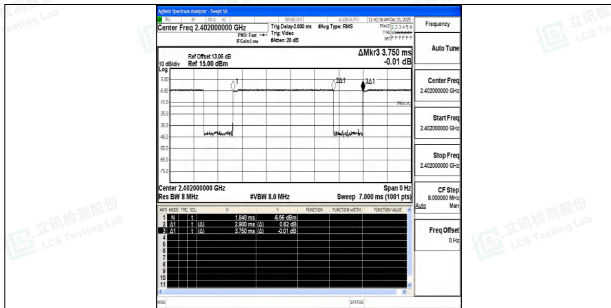
NTNV-3DH5-Ant1-2402
