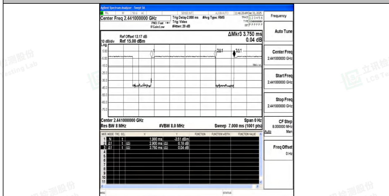
NTNV-3DH5-Ant1-2441
