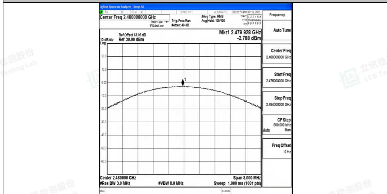
2DH5-Ant1-2480-PASS
