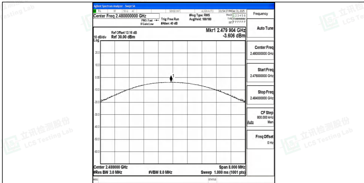
DH5-Ant1-2480-PASS
