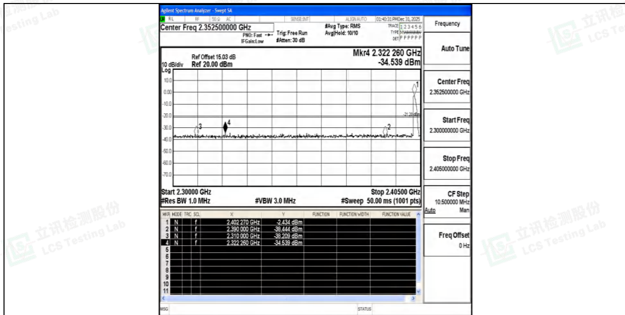
2DH5-Ant1-Hop_2402-PASS
