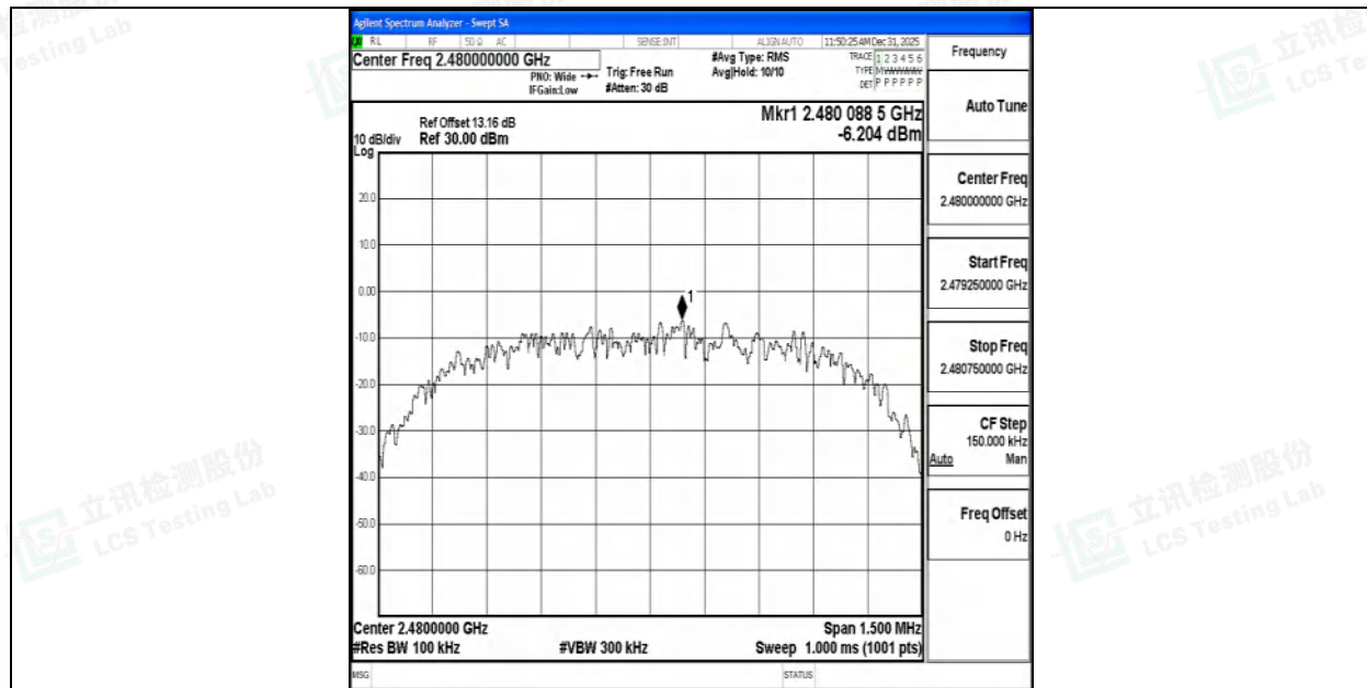
3DH5-Ant1-2480-0~Reference-PASS
