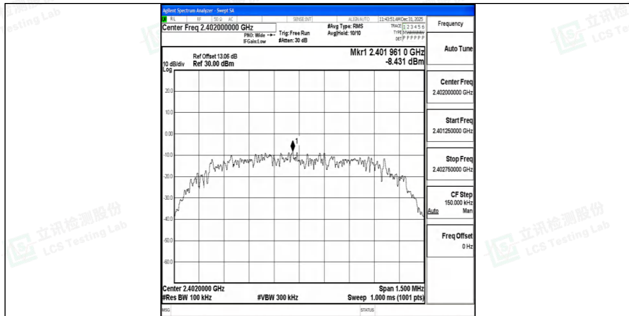
3DH5-Ant1-2402-0~Reference-PASS
