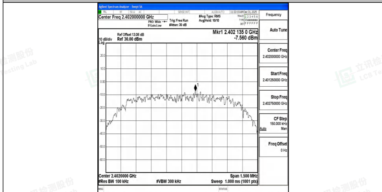
2DH5-Ant1-2402-0~Reference-PASS
