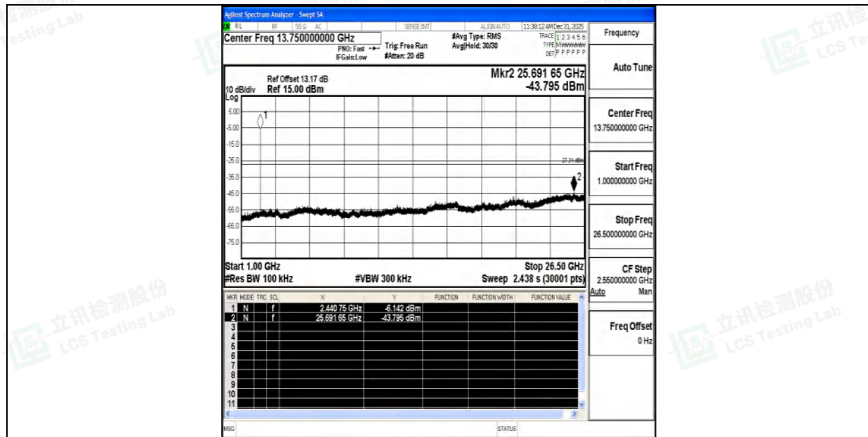
2DH5-Ant1-2441-1000~26500-PASS
