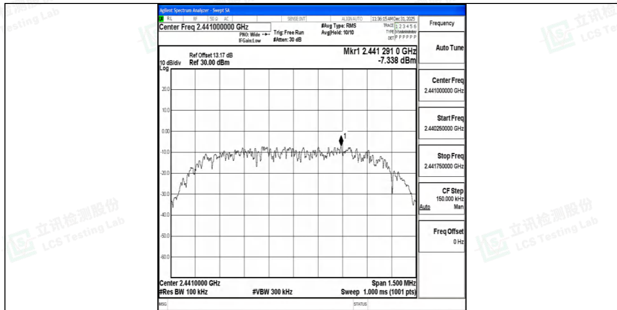
2DH5-Ant1-2441-0~Reference-PASS
