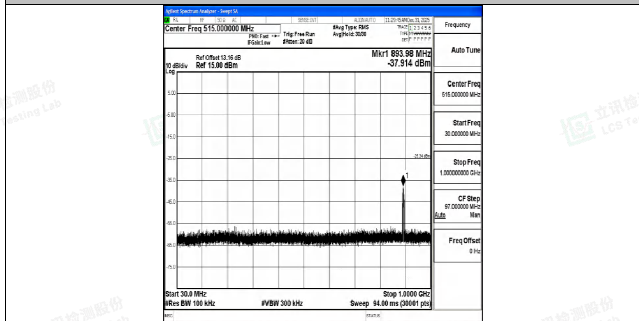
DH5-Ant1-2480-30~1000-PASS
