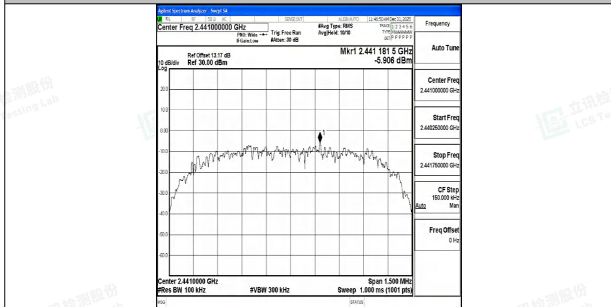
3DH5-Ant1-2441-0~Reference-PASS
