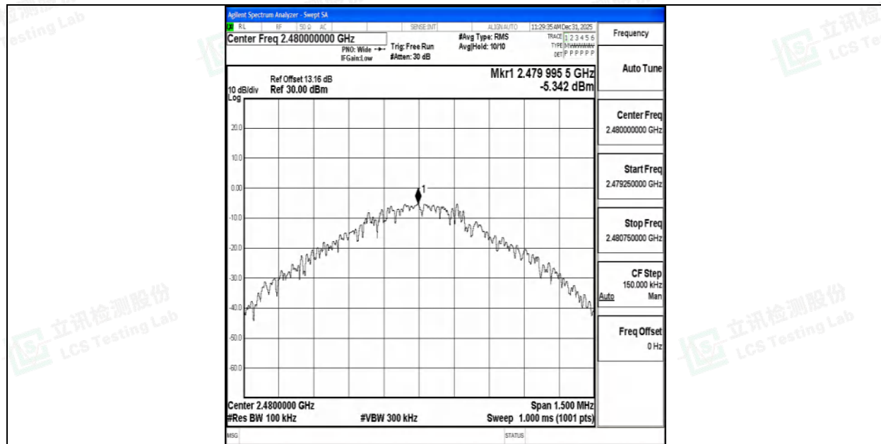
DH5-Ant1-2480-0~Reference-PASS
