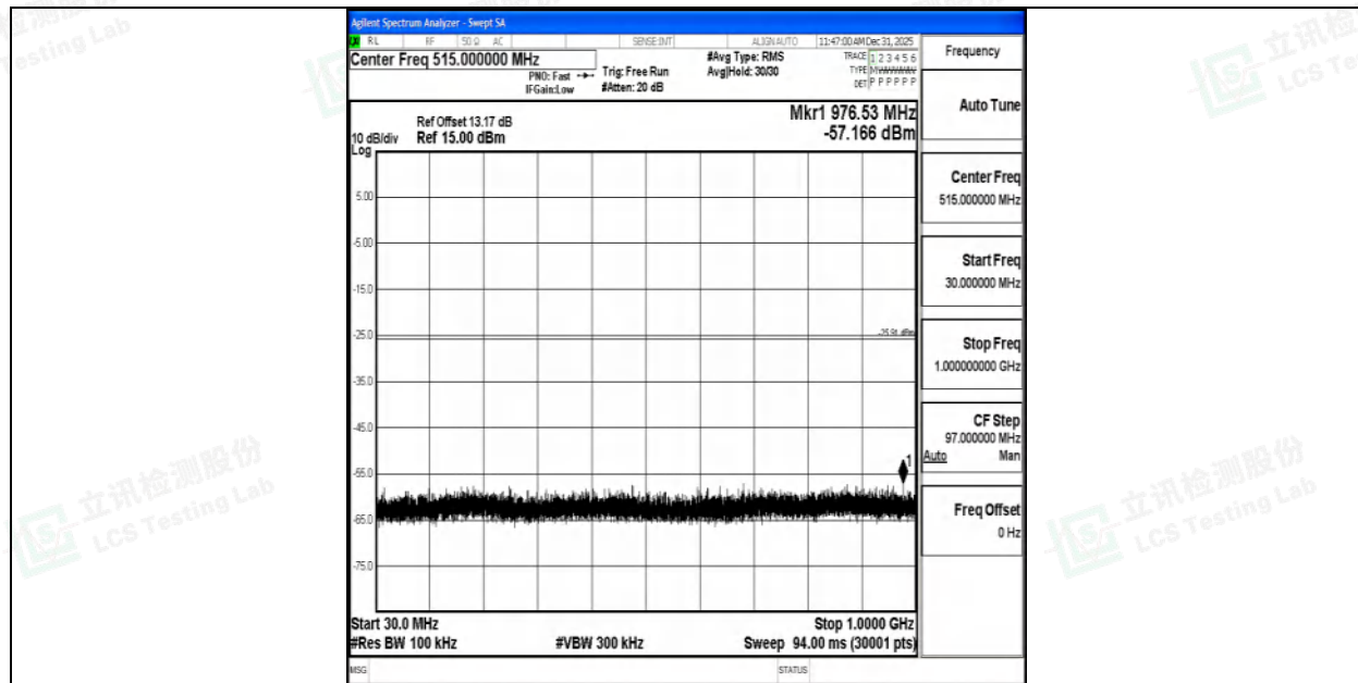
3DH5-Ant1-2441-30~1000-PASS
