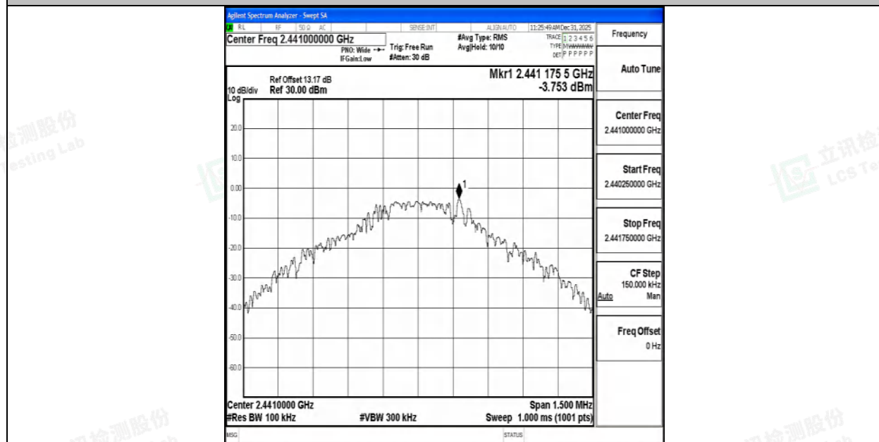
DH5-Ant1-2441-0~Reference-PASS
