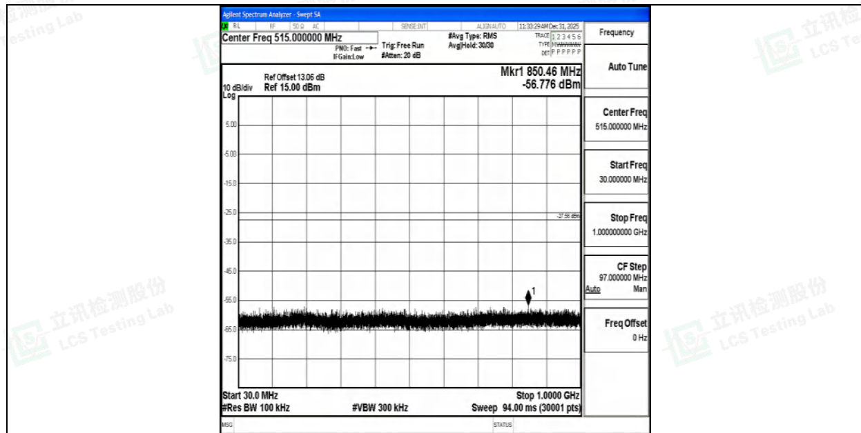
2DH5-Ant1-2402-30~1000-PASS
