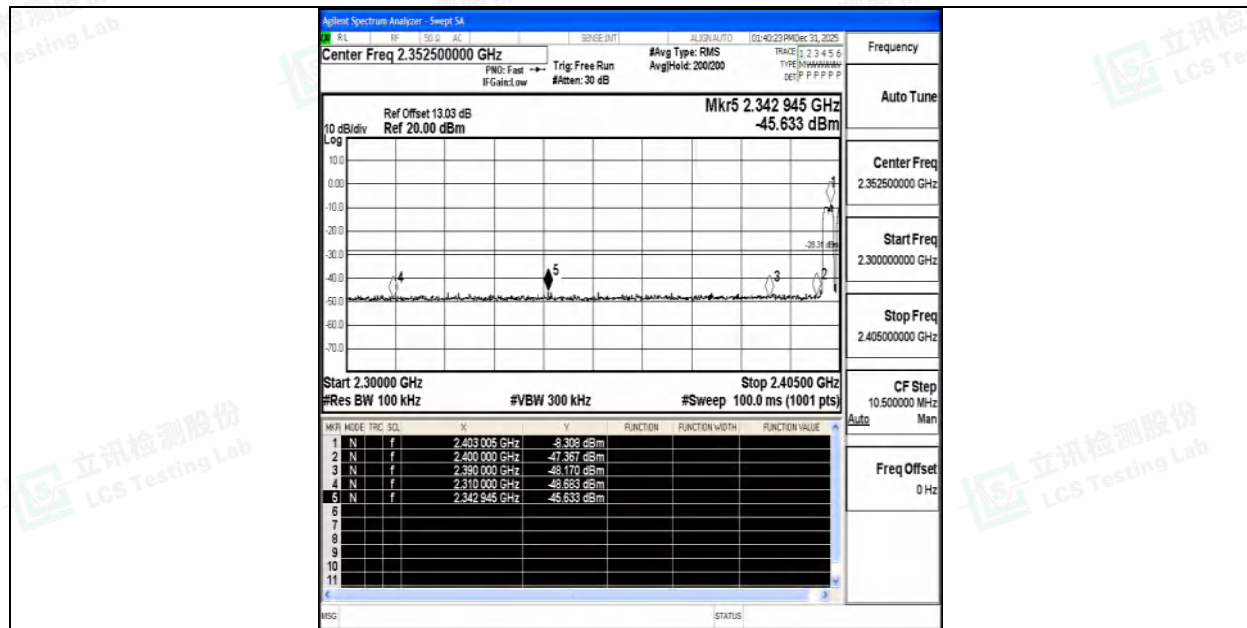
2DH5-Ant1-Hop_2402-PASS
