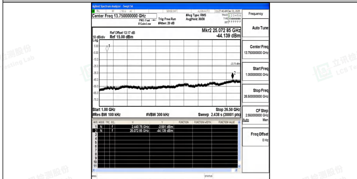
DH5-Ant1-2441-1000~26500-PASS
