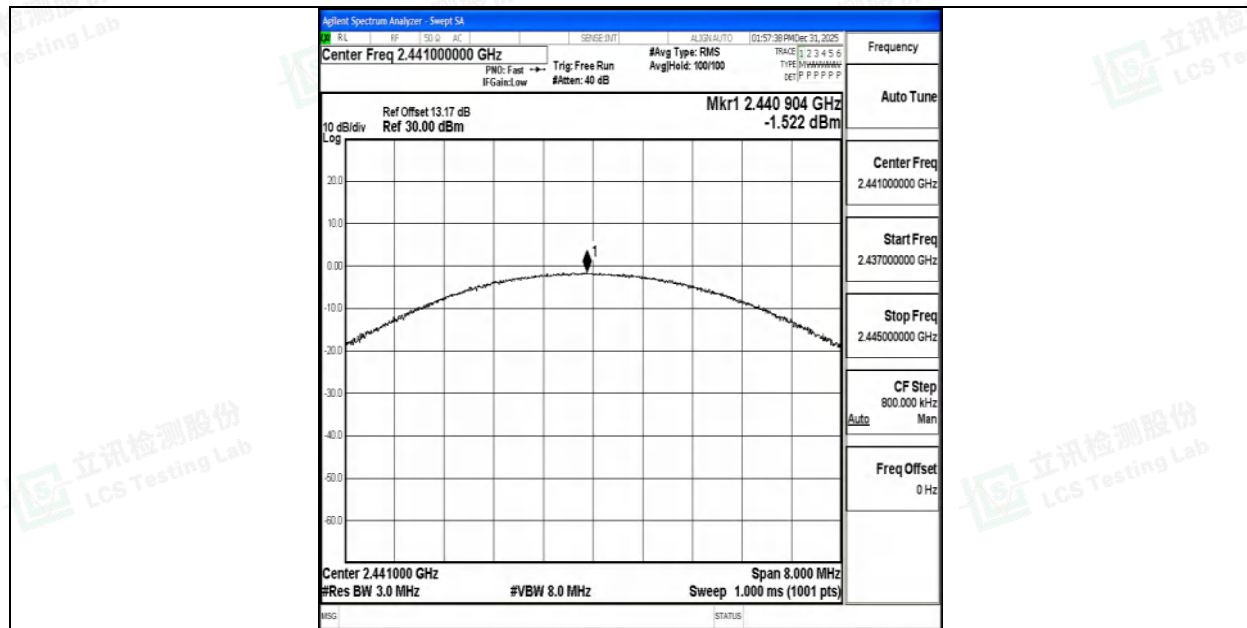
2DH5-Ant1-2441-PASS
