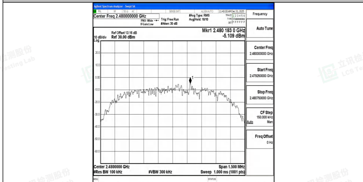
2DH5-Ant1-2480-0~Reference-PASS
