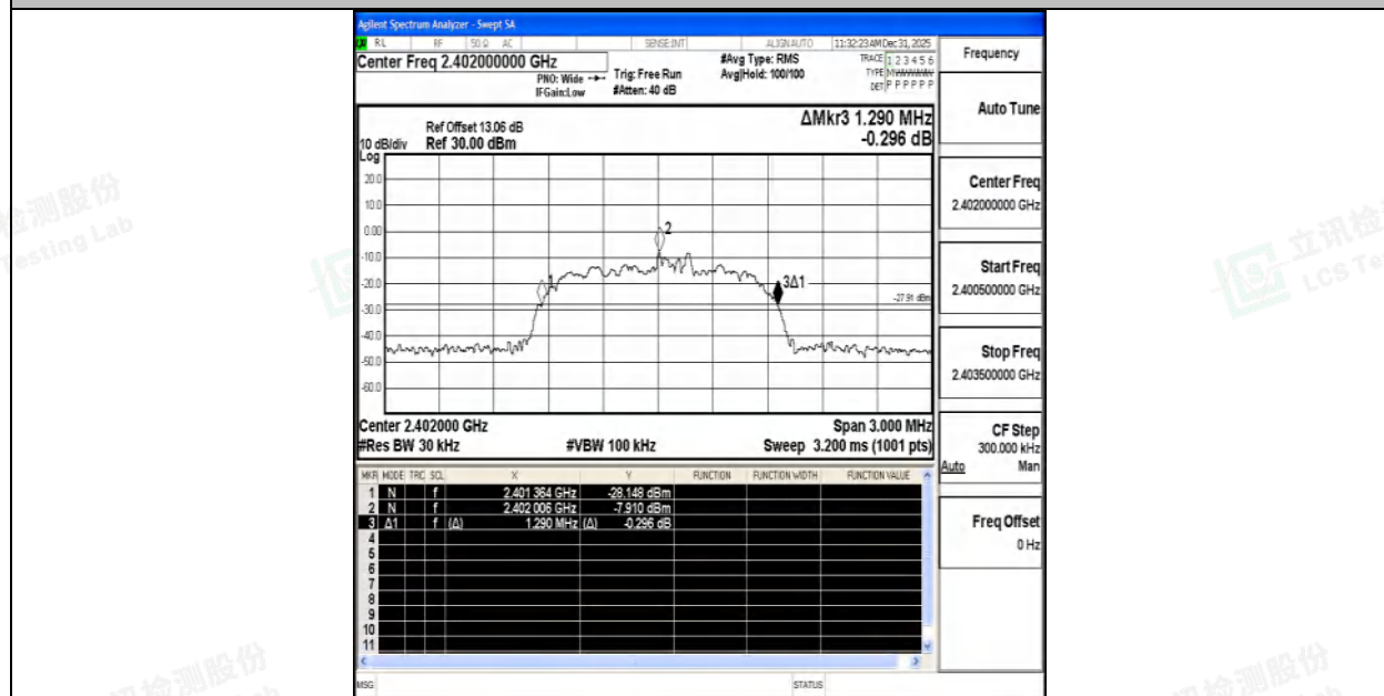
2DH5-Ant1-2402
