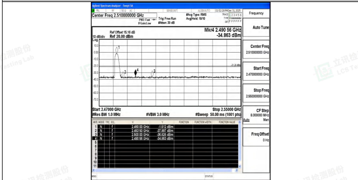
3DH5-Ant1-Hop_2480-PASS
