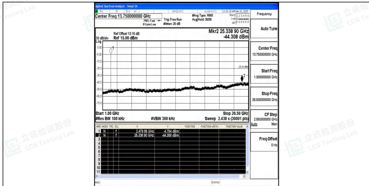
DH5-Ant1-2480-1000~26500-PASS
