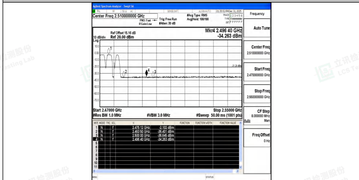
DH5-Ant1-Hop_2480-PASS
