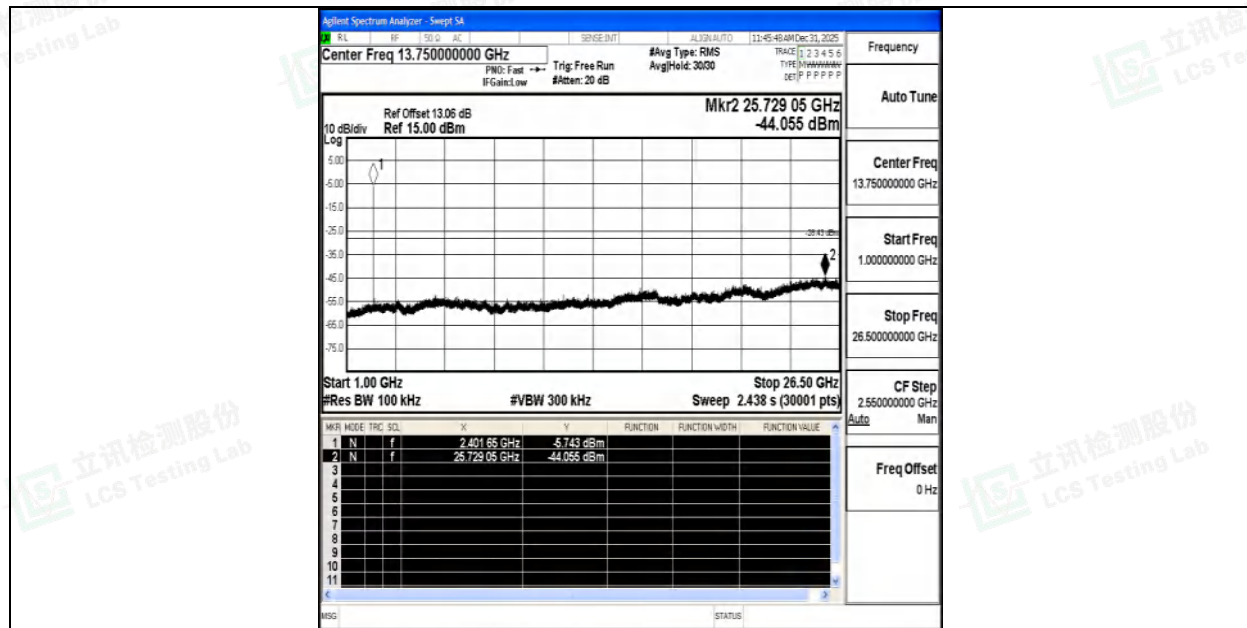
3DH5-Ant1-2402-1000~26500-PASS
