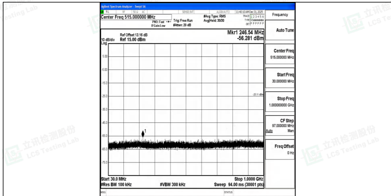
2DH5-Ant1-2480-30~1000-PASS
