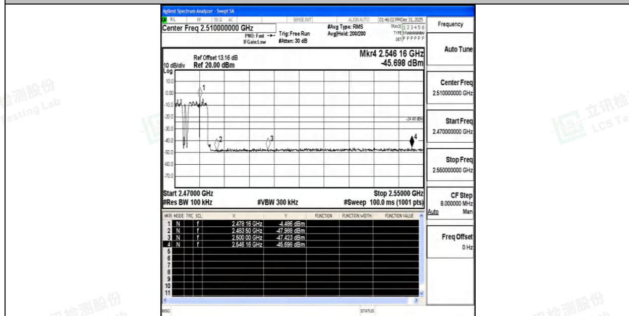
2DH5-Ant1-Hop_2480-PASS
