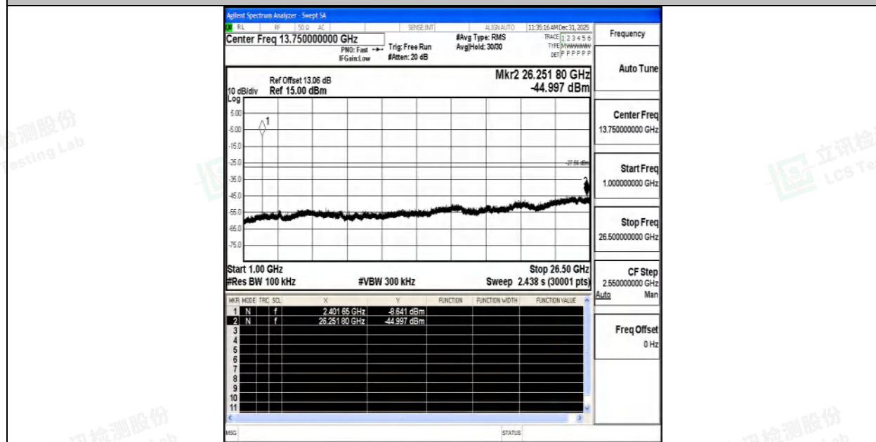
2DH5-Ant1-2402-1000~26500-PASS
