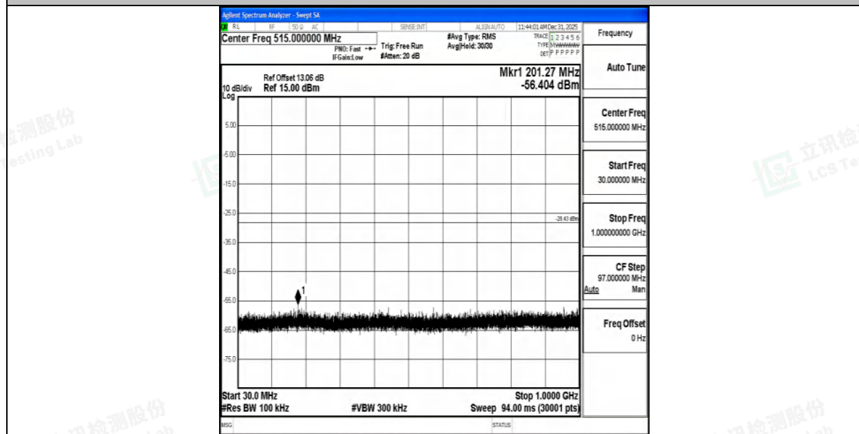
3DH5-Ant1-2402-30~1000-PASS
