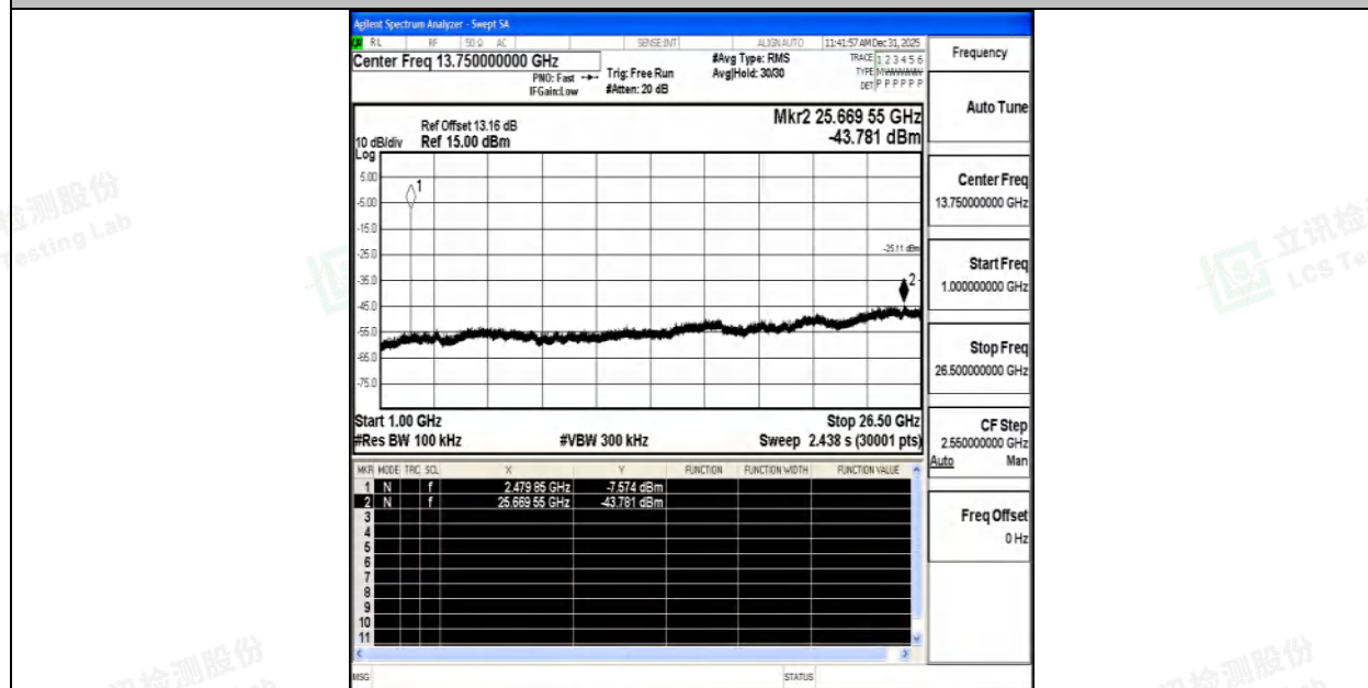
2DH5-Ant1-2480-1000~26500-PASS
