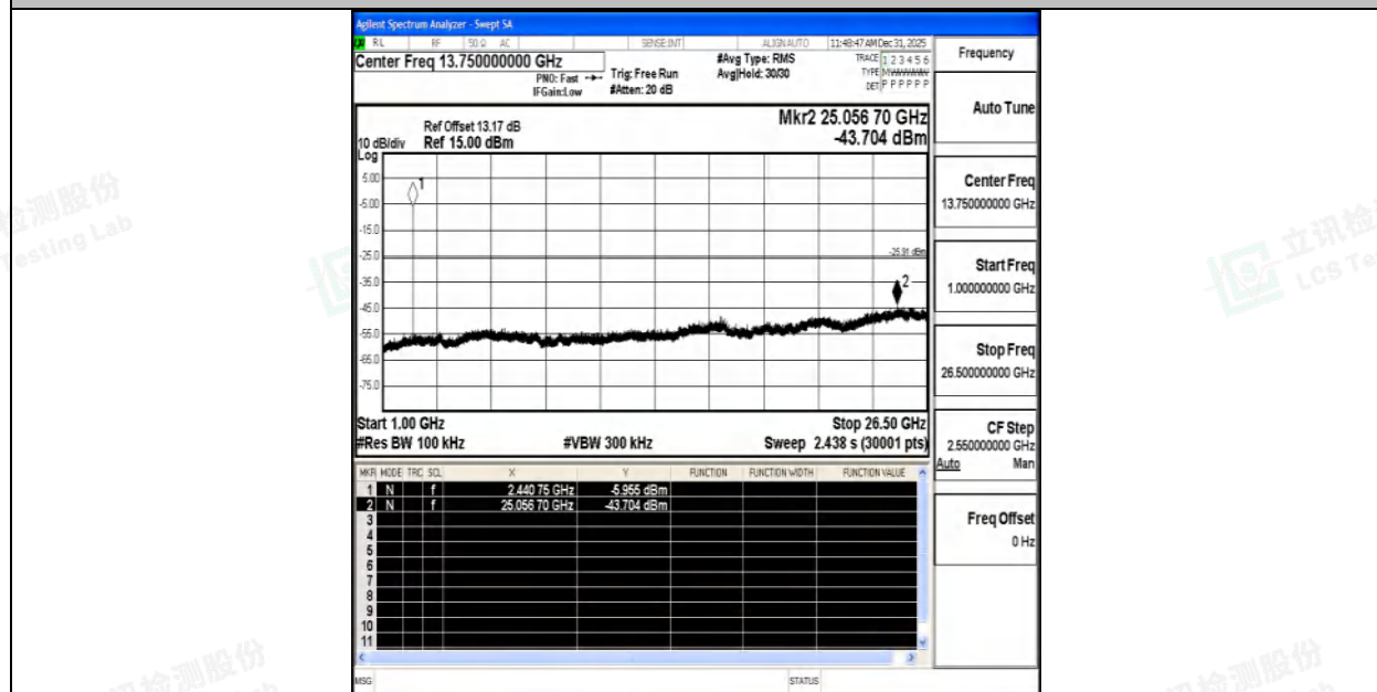
3DH5-Ant1-2441-1000~26500-PASS
