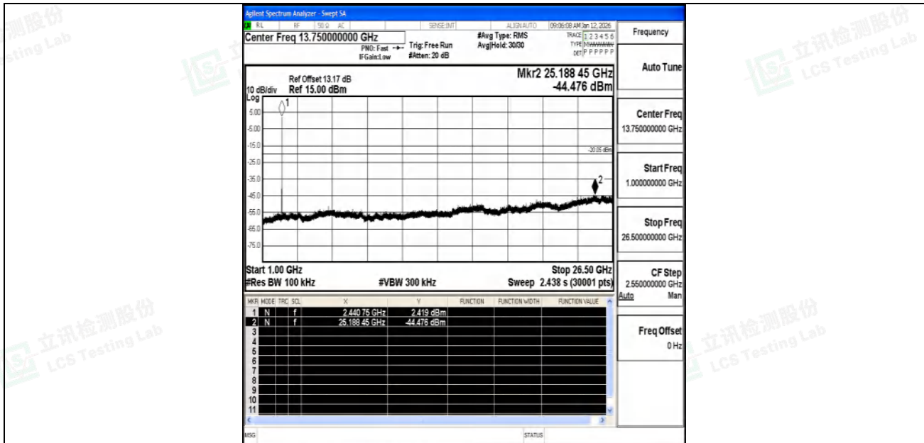
2DH5-Ant1-2441-1000~26500-PASS
