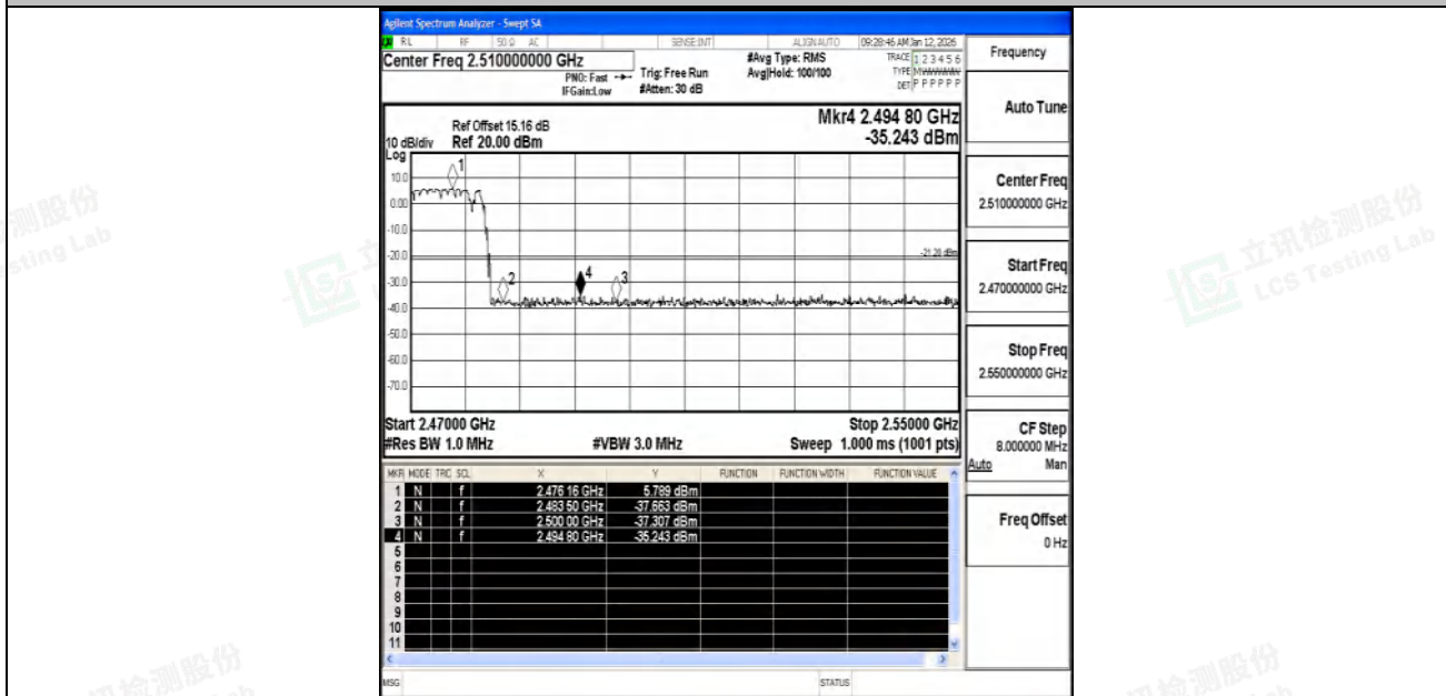
DH5-Ant1-Hop_2480-PASS
