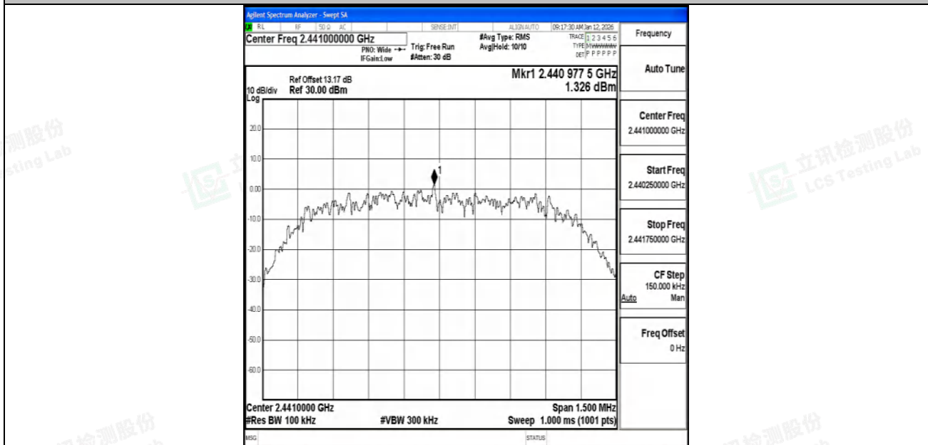
3DH5-Ant1-2441-0~Reference-PASS
