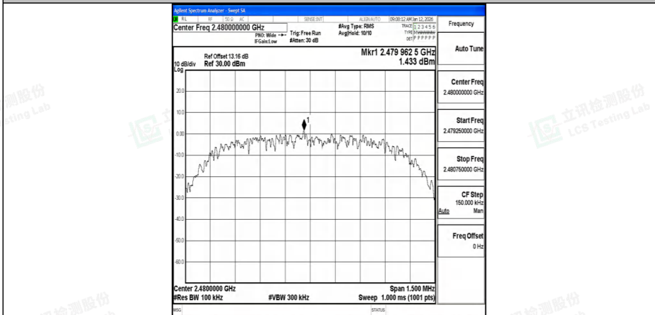
2DH5-Ant1-2480-0~Reference-PASS
