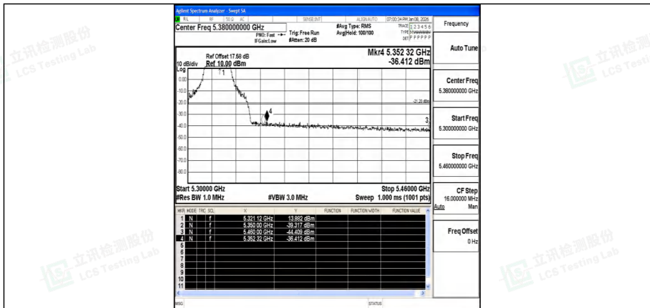
11N20SISO-Ant2-5320-PASS
