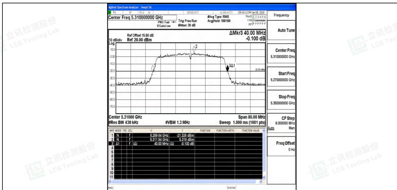
11AC40SISO-Ant1-5310
