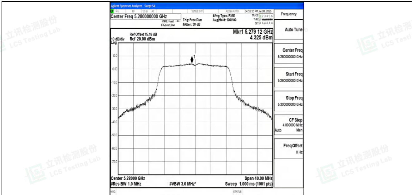
11N20SISO-Ant1-5280-PASS
