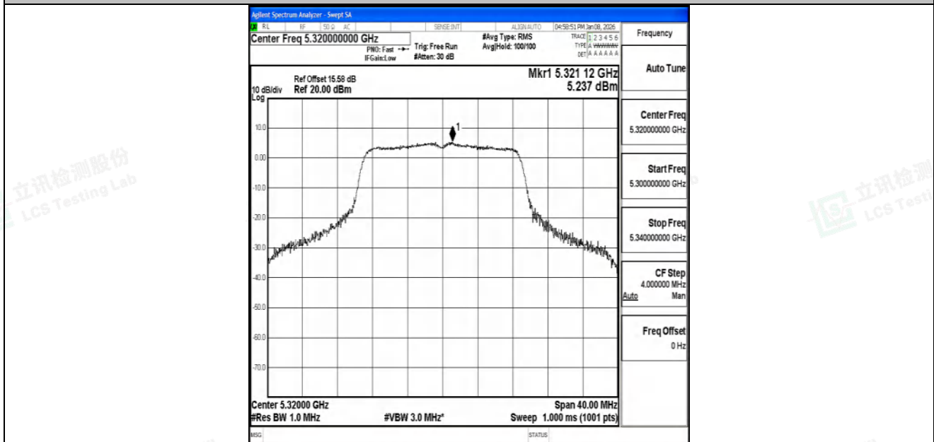
11N20SISO-Ant1-5320-PASS
