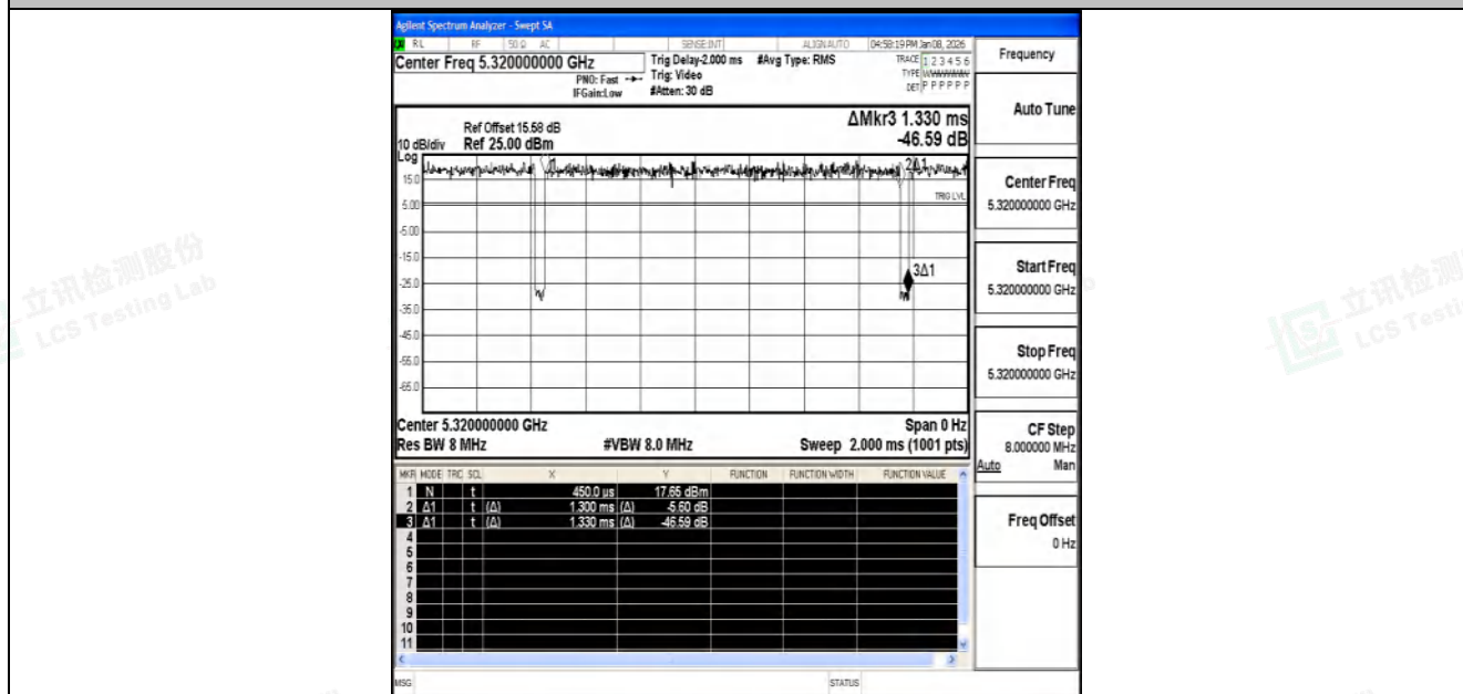
NTNV-11N20SISO-Ant1-5320
