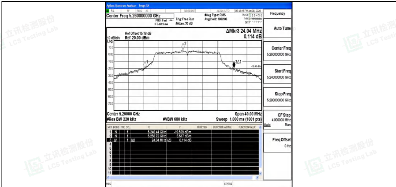
11AC20SISO-Ant1-5260
