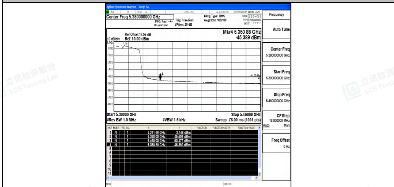
11AC40SISO-Ant2-5310-PASS
