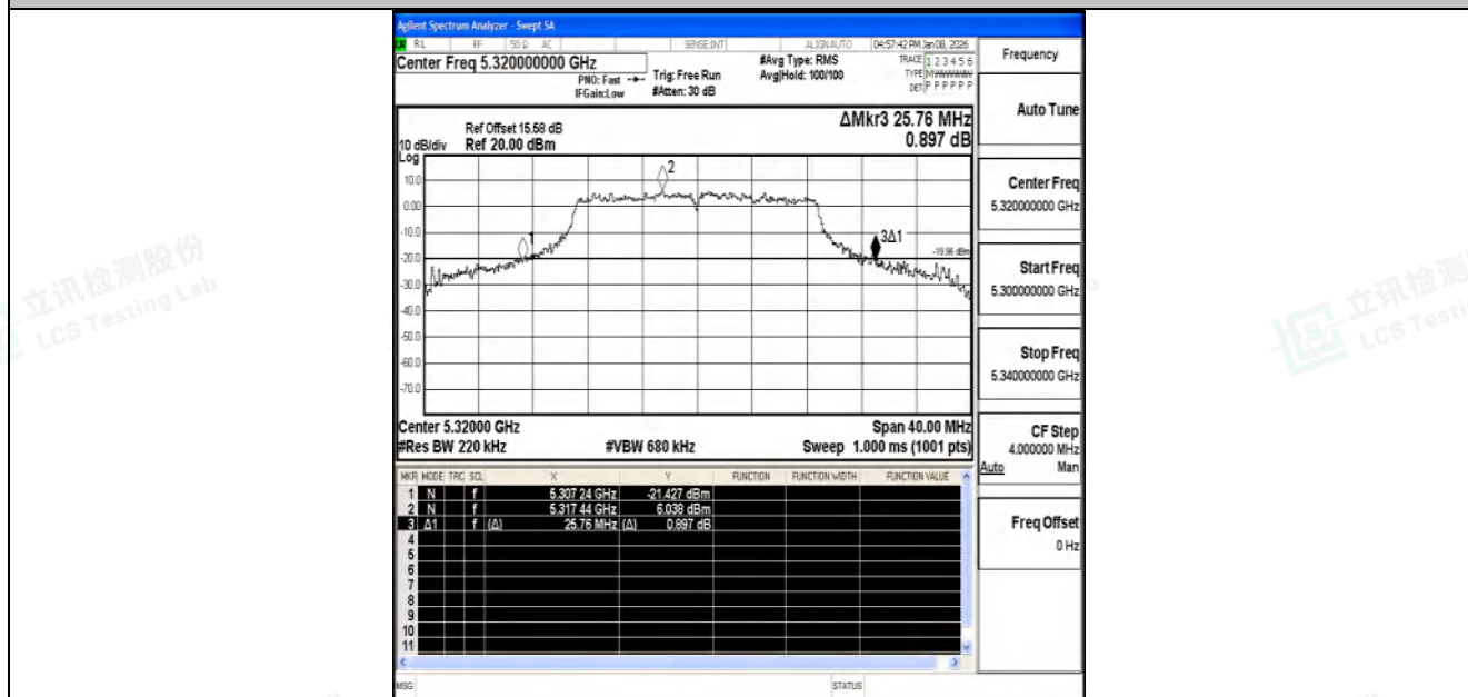
11N20SISO-Ant1-5320
