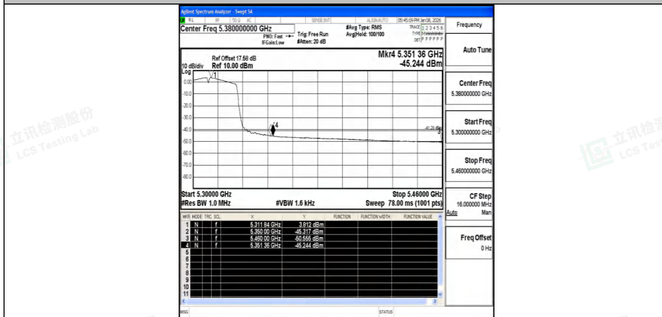
11AC40SISO-Ant1-5310-PASS
