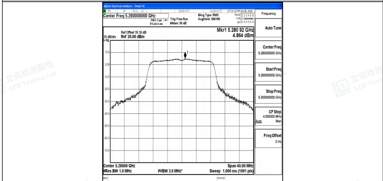
11AC20SISO-Ant2-5280-PASS
