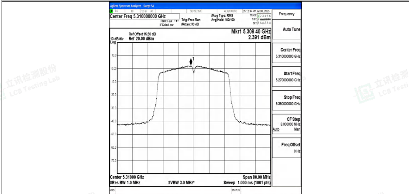
11N40SISO-Ant1-5310-PASS
