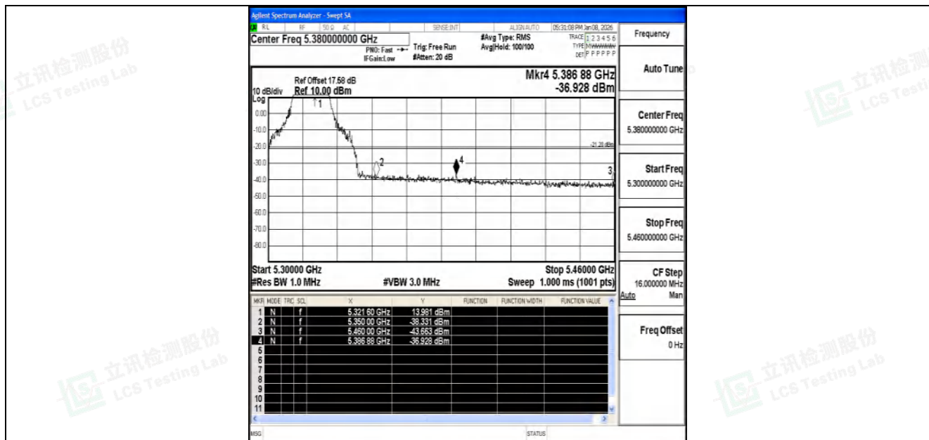
11AC20SISO-Ant1-5320-PASS
