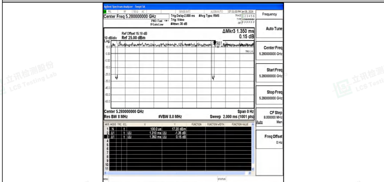
NTNV-11AC20SISO-Ant2-5280
