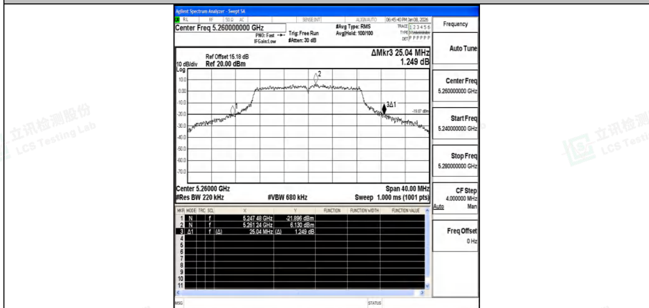
11N20SISO-Ant2-5260
