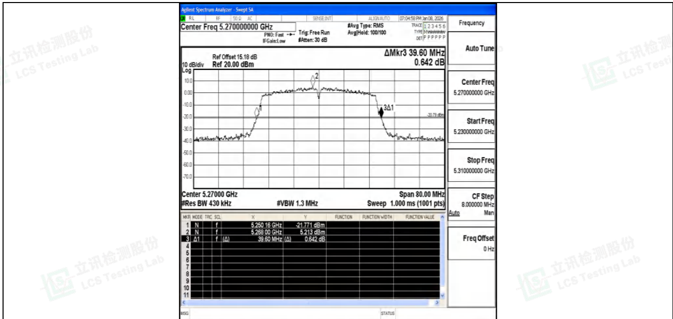
11N40SISO-Ant2-5270
