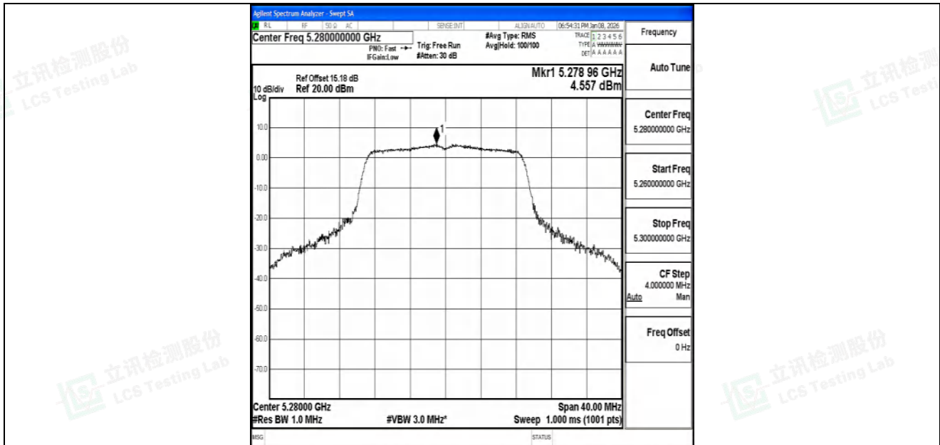
11N20SISO-Ant2-5280-PASS
