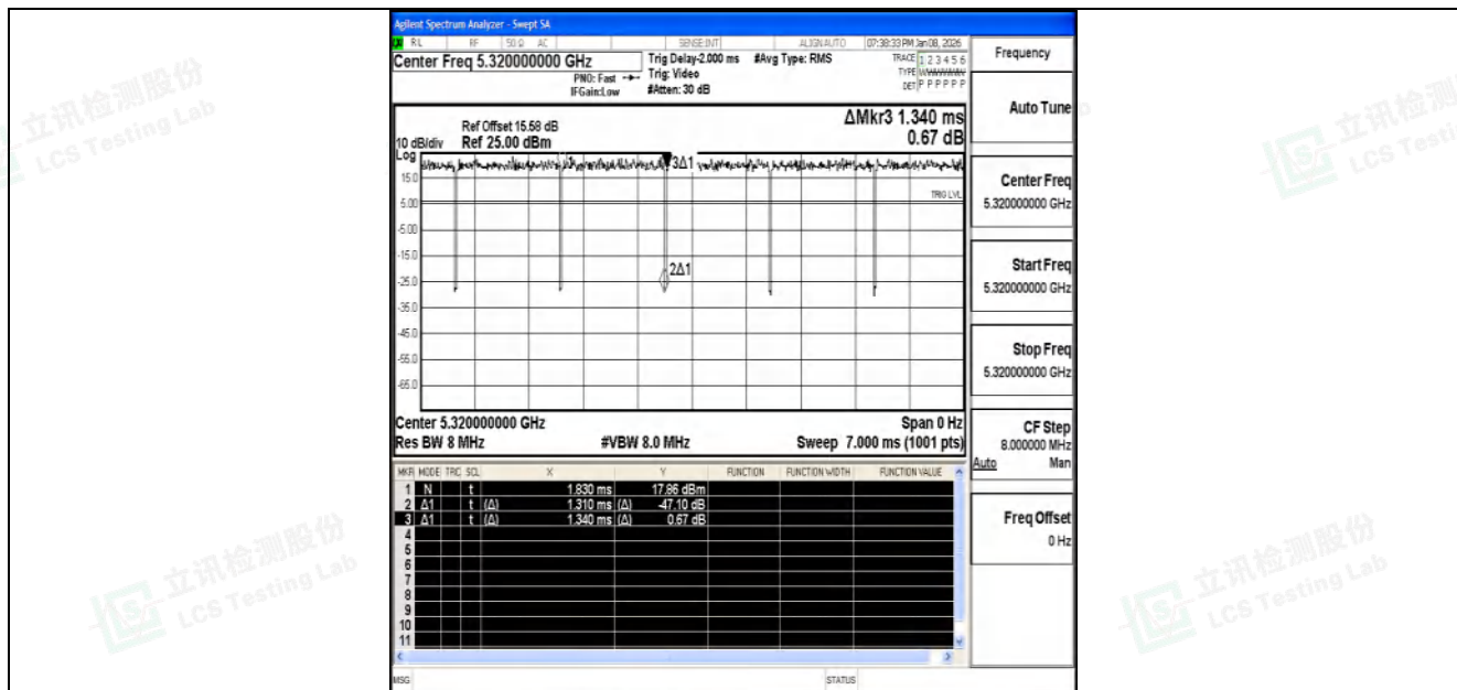
NTNV-11AC20SISO-Ant2-5320
