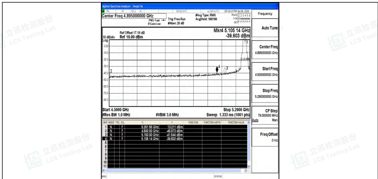
11AC20SISO-Ant1-5260-PASS
