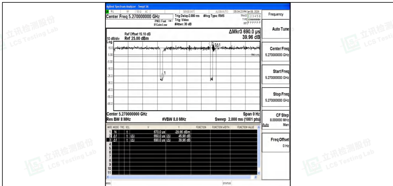
NTNV-11N40SISO-Ant1-5270
