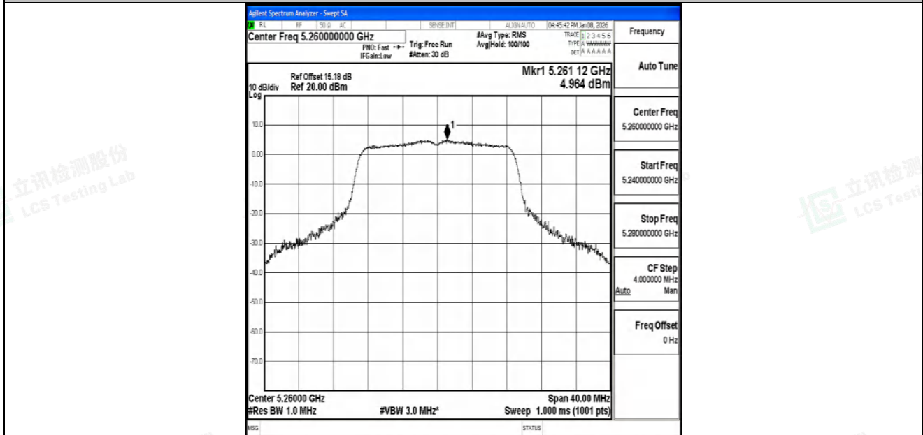
11N20SISO-Ant1-5260-PASS
