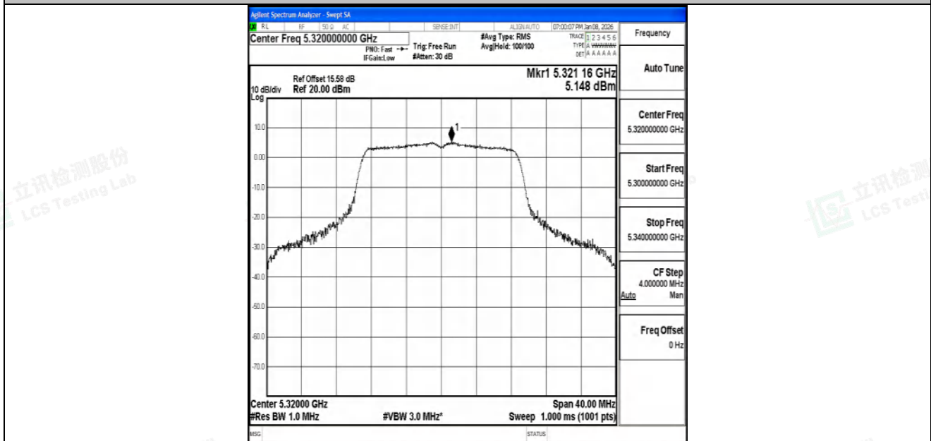
11N20SISO-Ant2-5320-PASS
