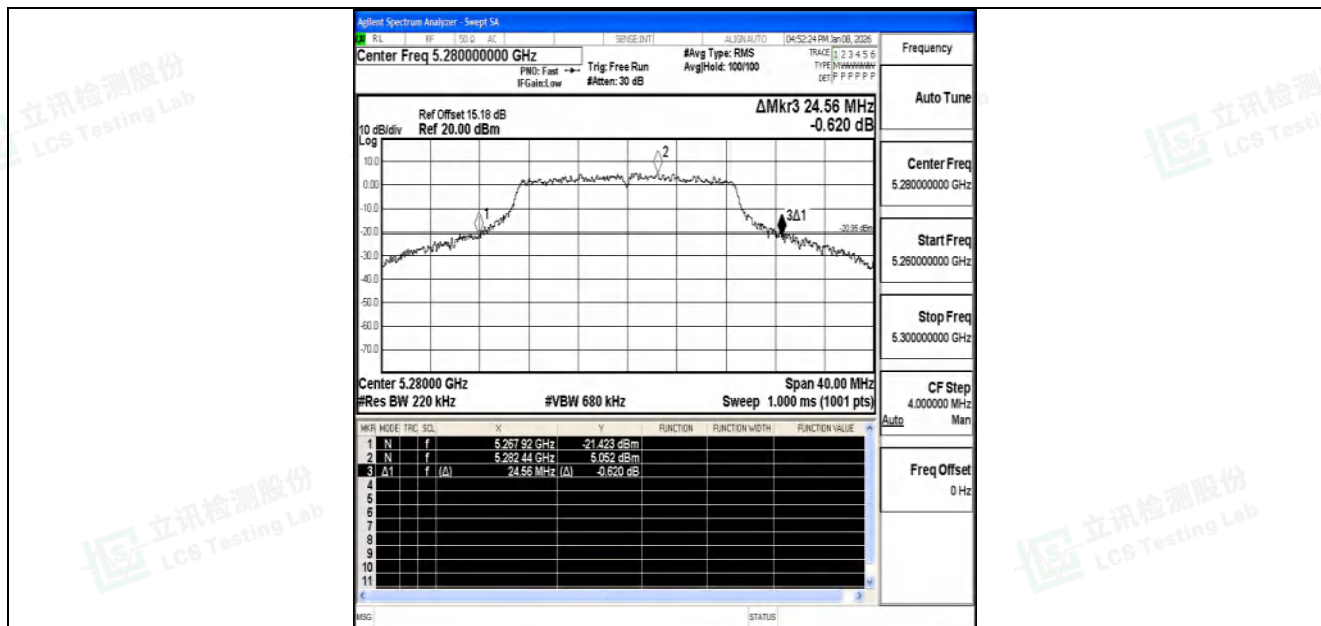
11N20SISO-Ant1-5280
