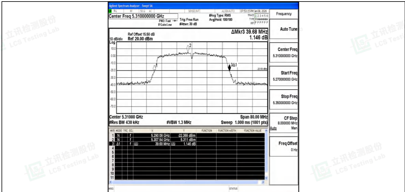
11AC40SISO-Ant2-5310
