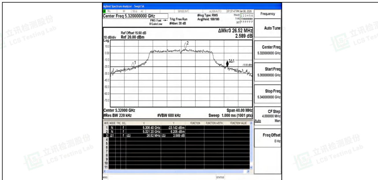
11AC20SISO-Ant2-5320
