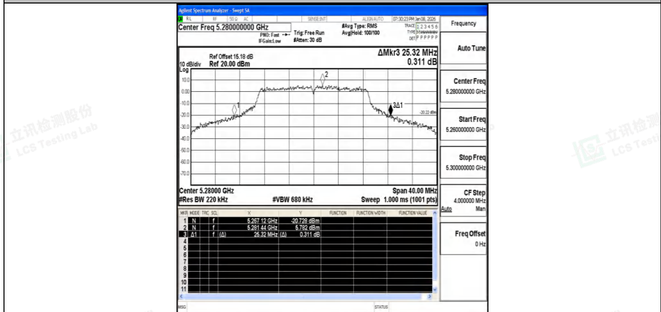
11AC20SISO-Ant2-5280
