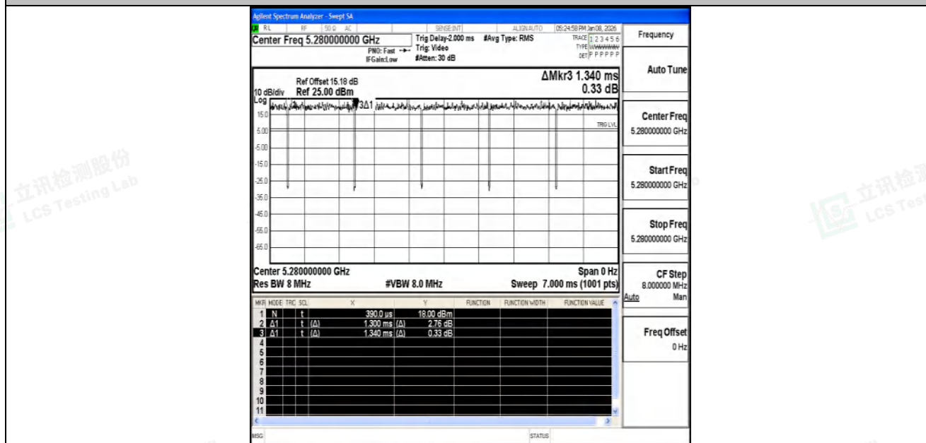
NTNV-11AC20SISO-Ant1-5280
