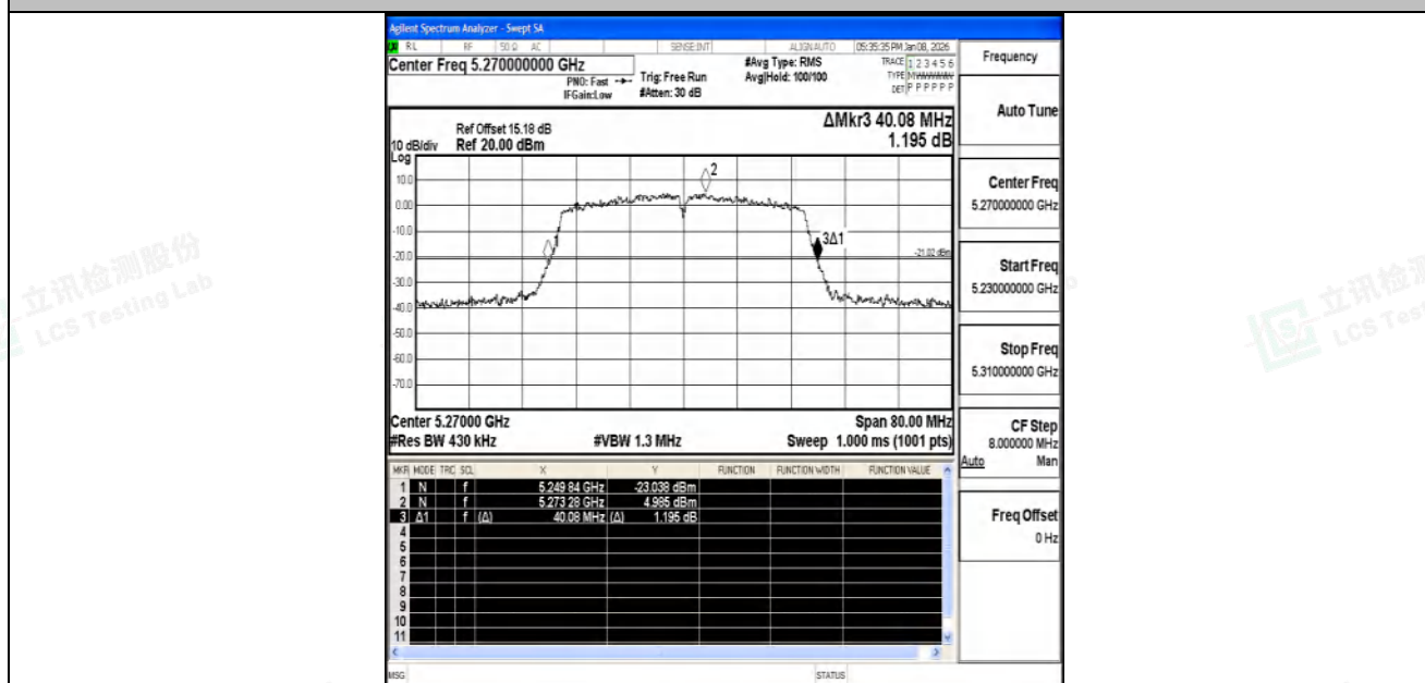
11AC40SISO-Ant1-5270
