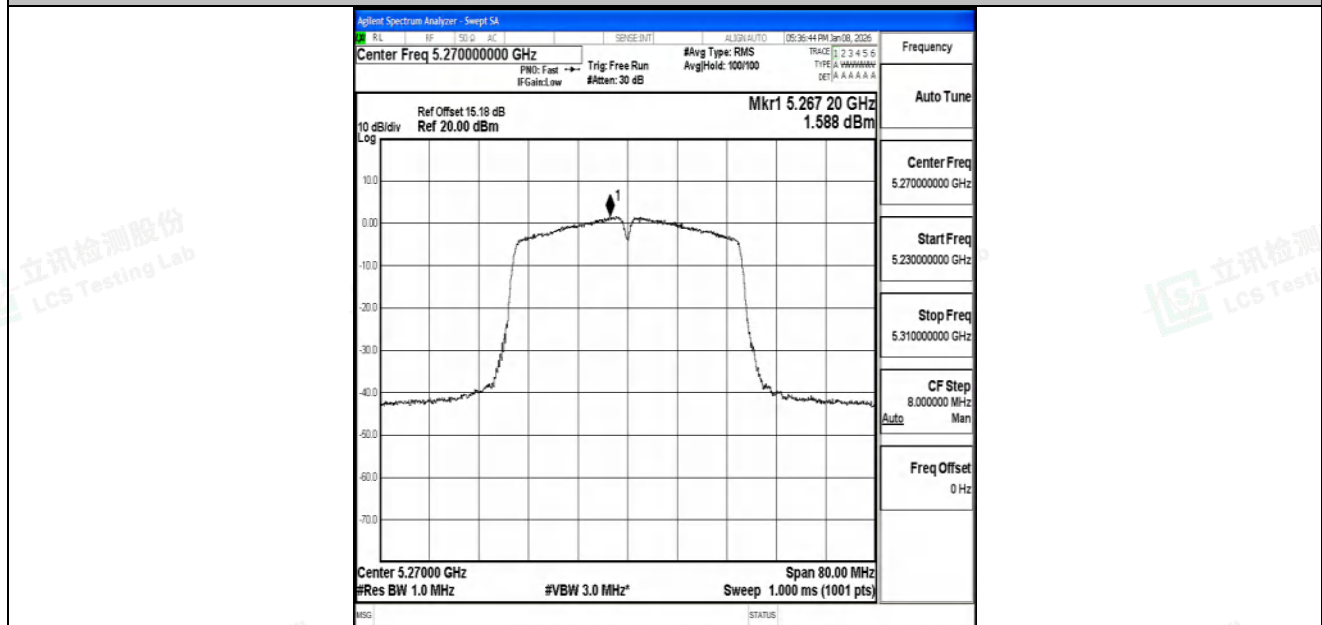
11AC40SISO-Ant1-5270-PASS
