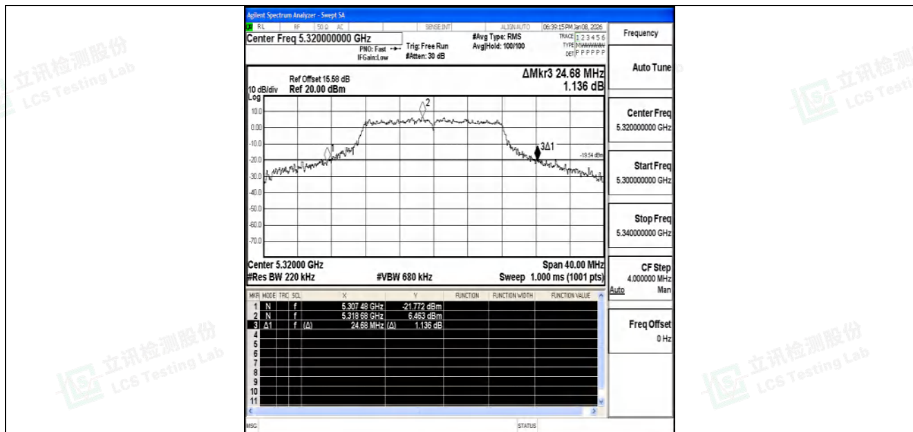
11A-Ant2-5320
