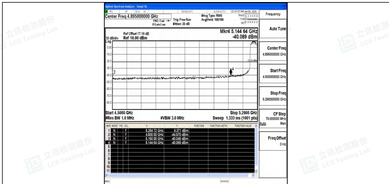
11AC40SISO-Ant2-5270-PASS
