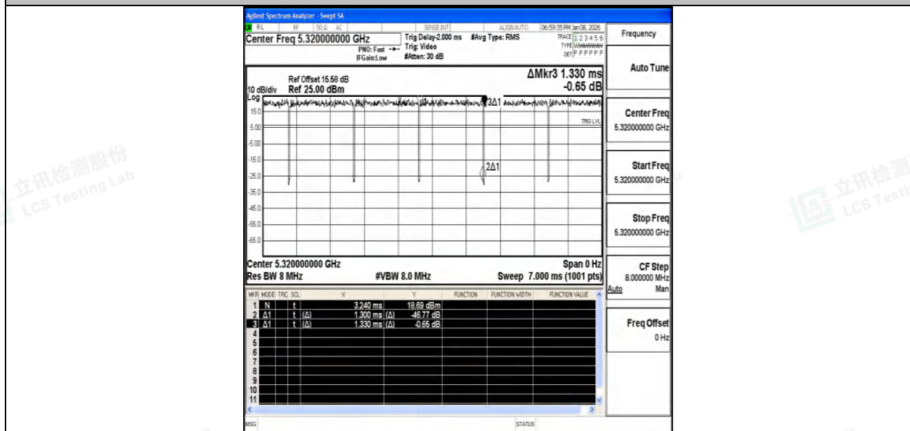
NTNV-11N20SISO-Ant2-5320
