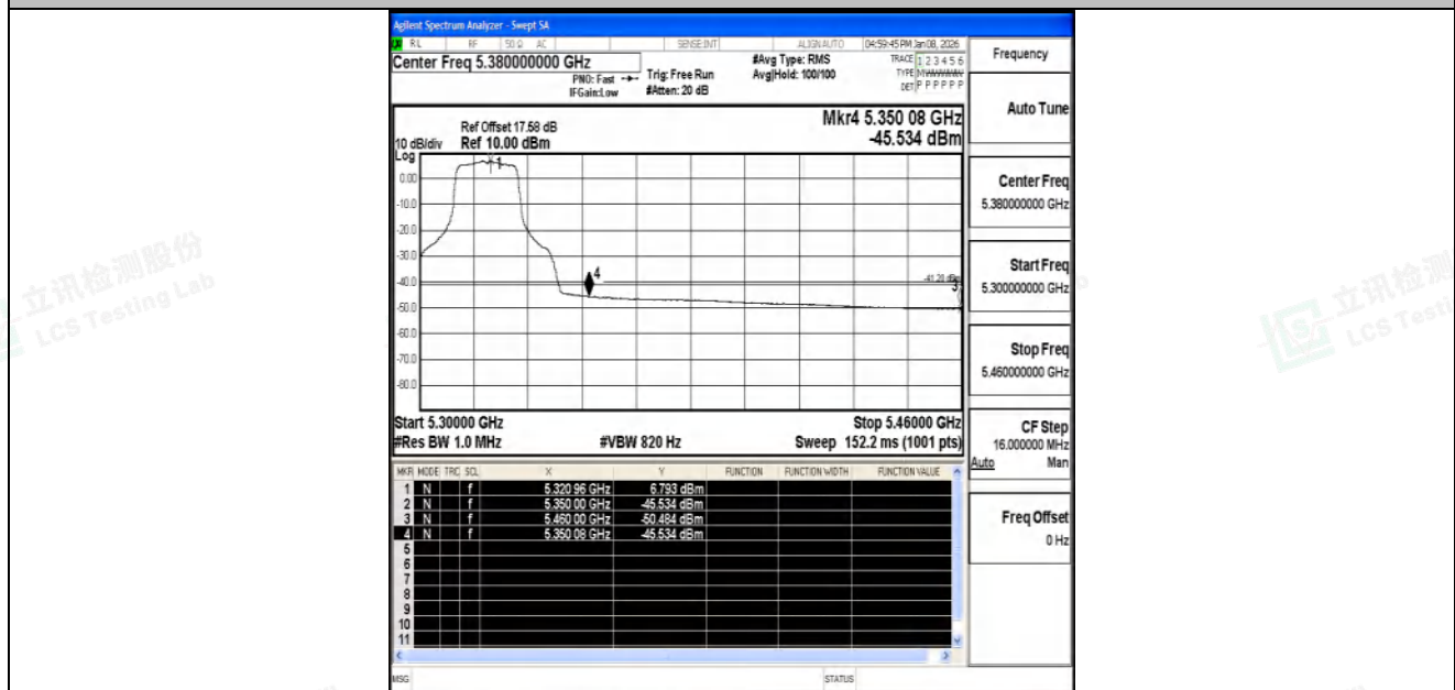
11N20SISO-Ant1-5320-PASS
