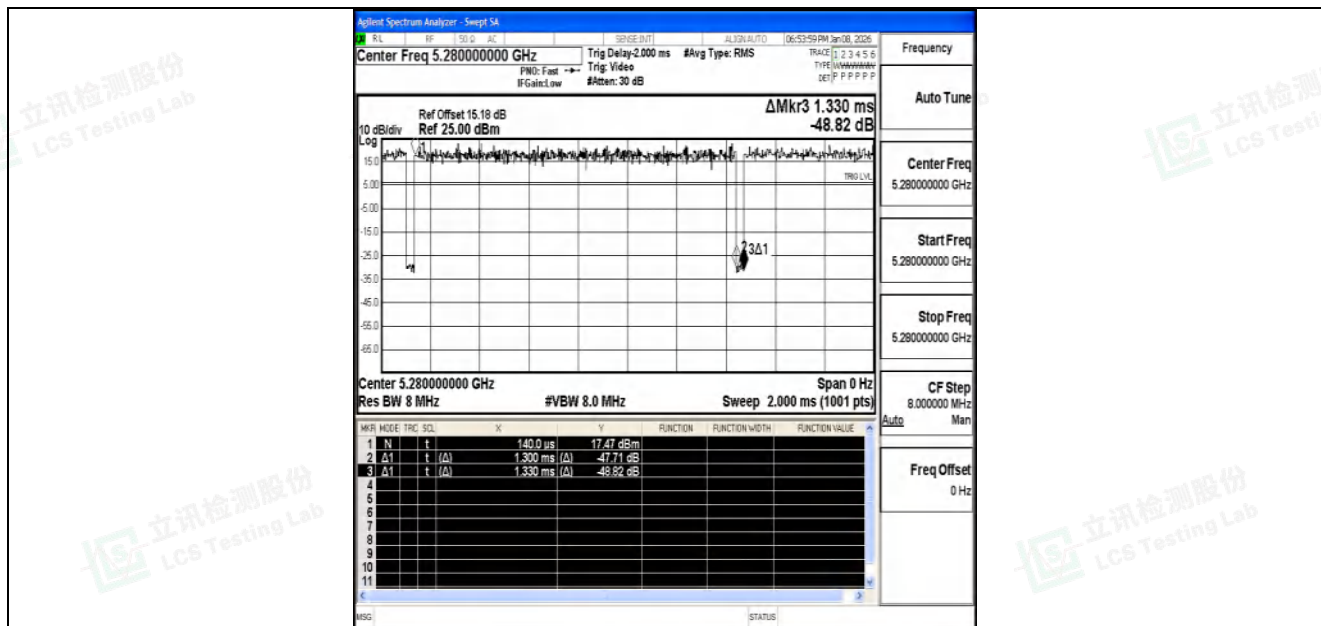
NTNV-11N20SISO-Ant2-5280
