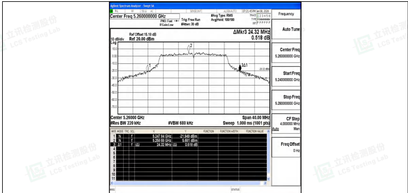
11AC20SISO-Ant2-5260
