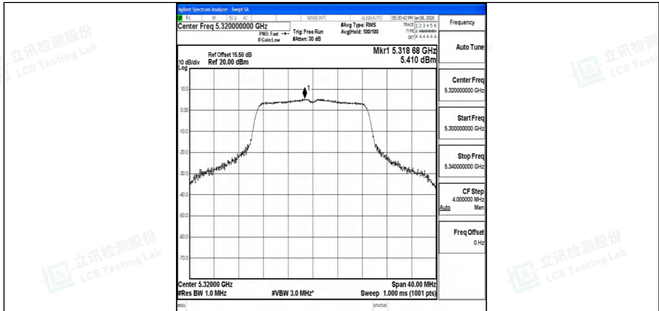
11AC20SISO-Ant1-5320-PASS
