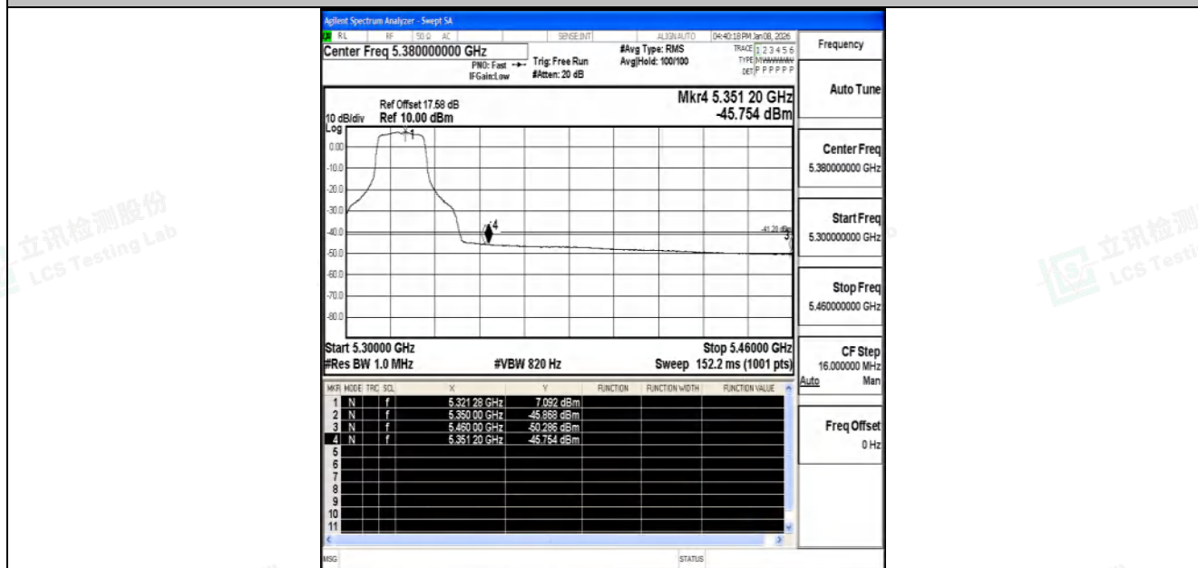
11A-Ant1-5320-PASS
