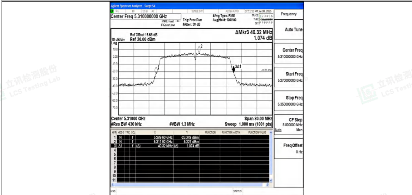
11N40SISO-Ant2-5310
