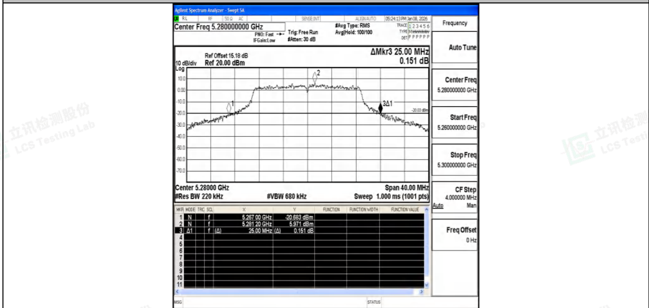
11AC20SISO-Ant1-5280
