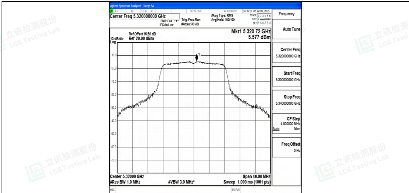
11A-Ant1-5320-PASS
