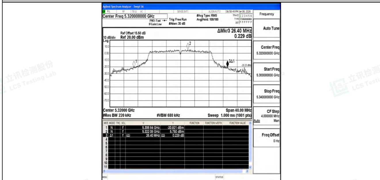
11N20SISO-Ant2-5320
