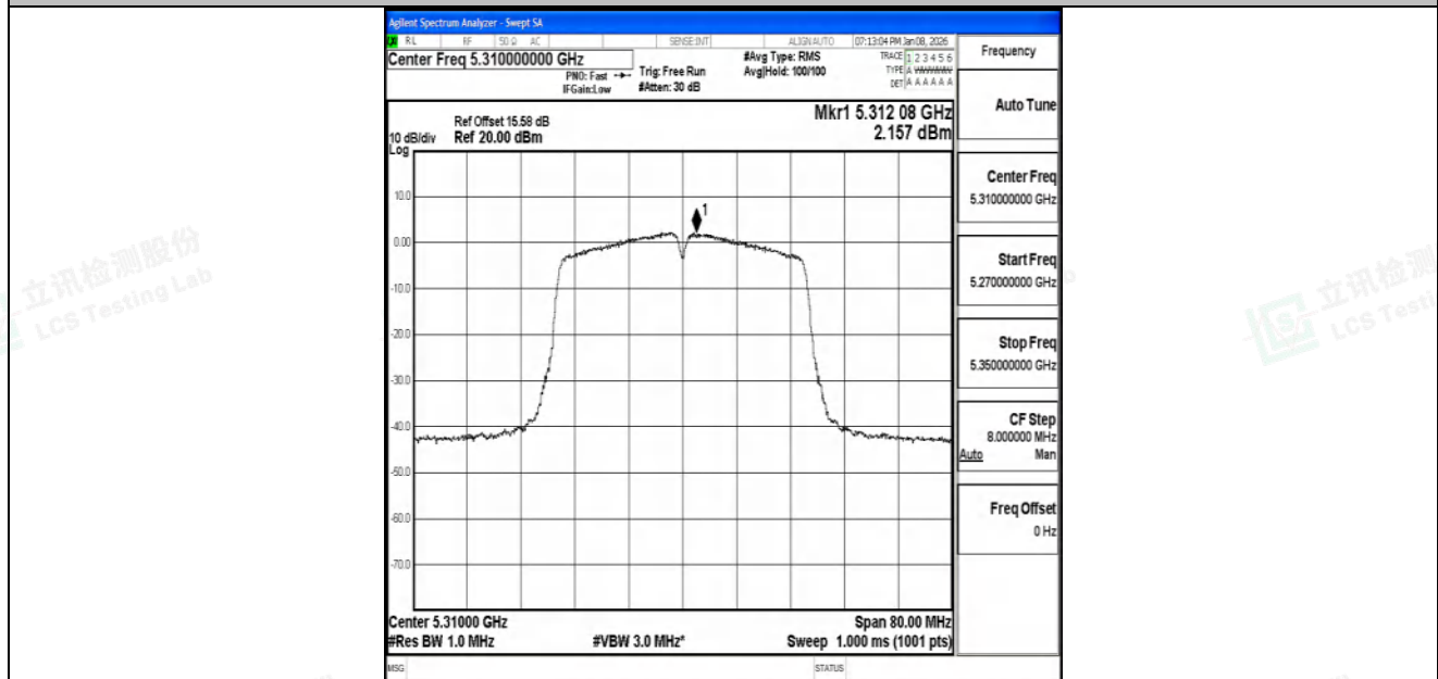
11N40SISO-Ant2-5310-PASS
