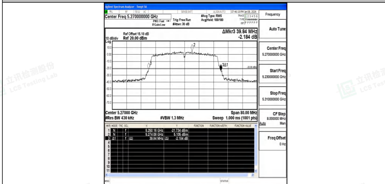
11AC40SISO-Ant2-5270
