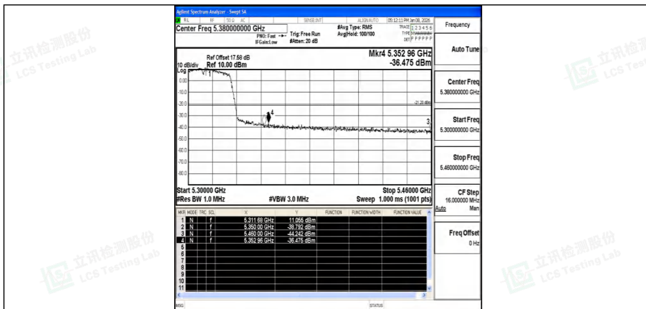
11N40SISO-Ant1-5310-PASS
