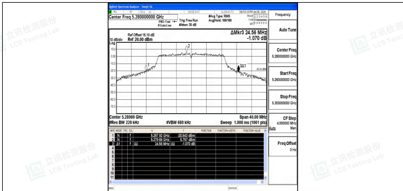
11N20SISO-Ant2-5280
