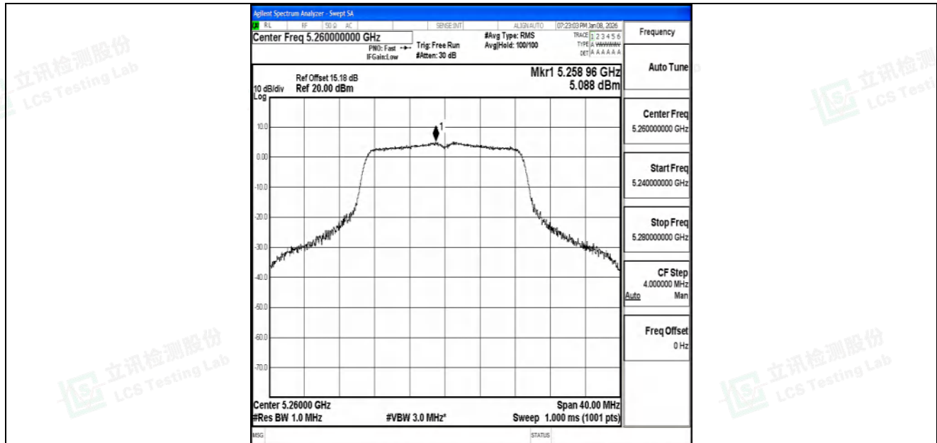
11AC20SISO-Ant2-5260-PASS
