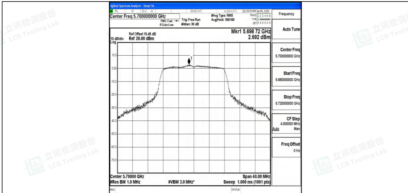
11A-Ant2-5700-PASS
