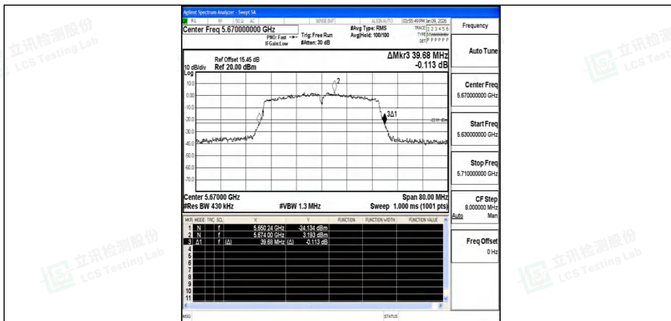
11AC40SISO-Ant2-5670
