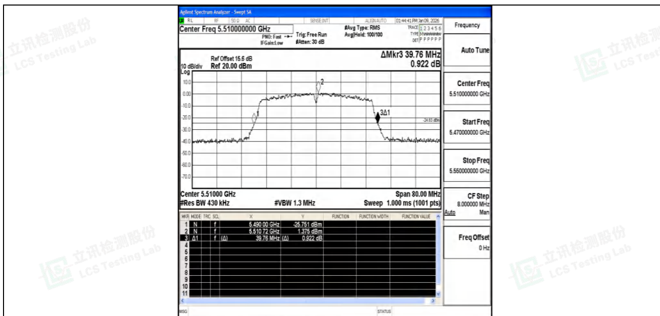
11AC40SISO-Ant1-5510
