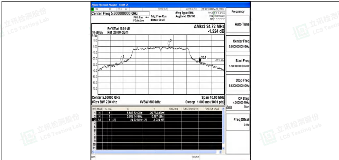
11AC20SISO-Ant1-5600
