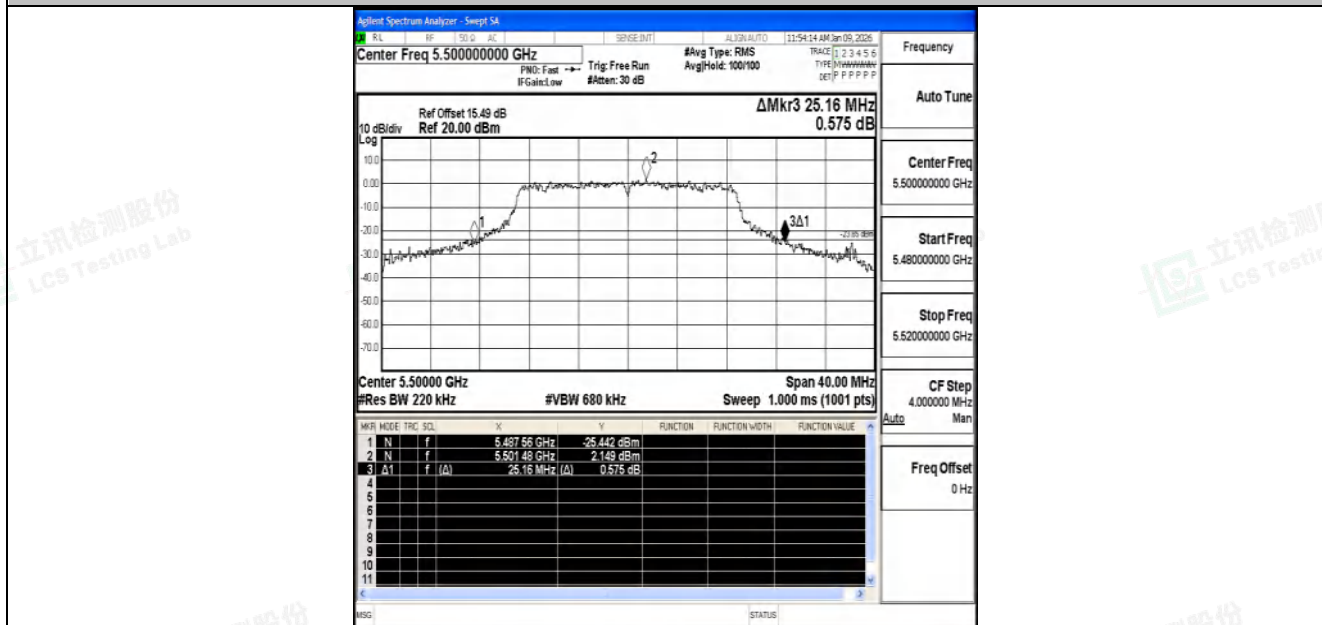
11AC20SISO-Ant1-5500
