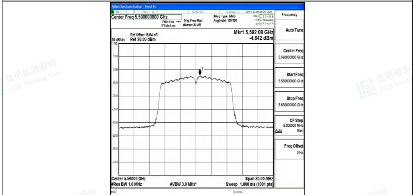
11N40SISO-Ant1-5590-PASS
