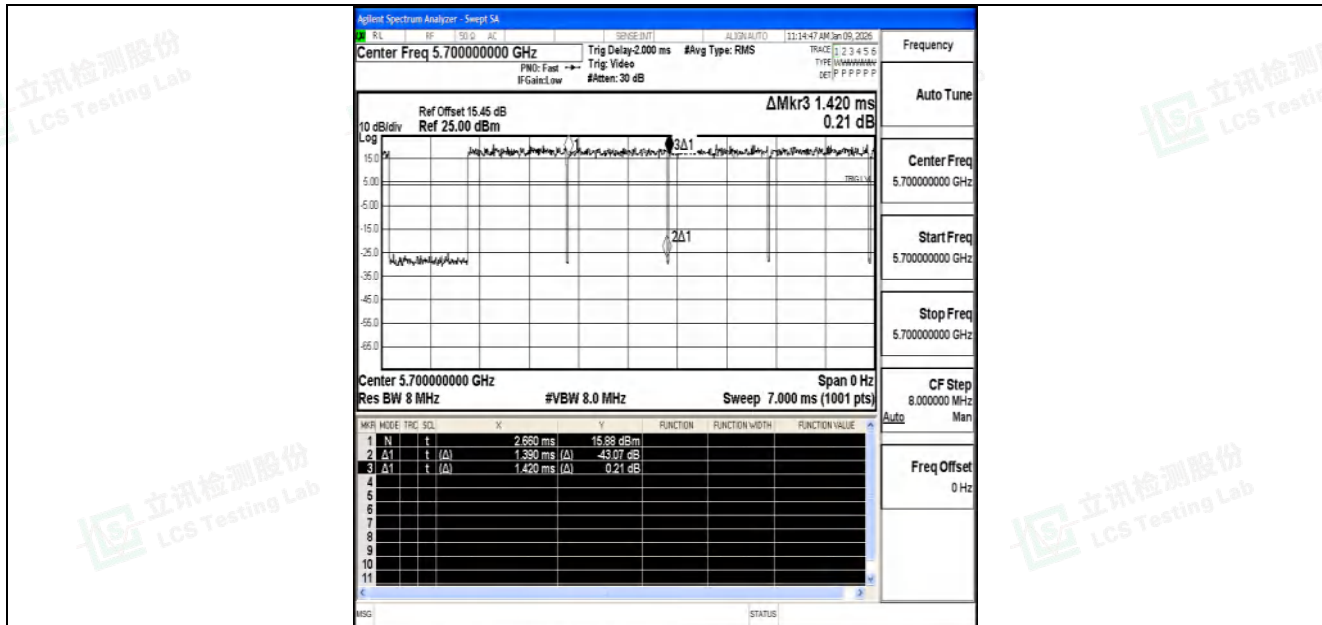
NTNV-11A-Ant1-5700
