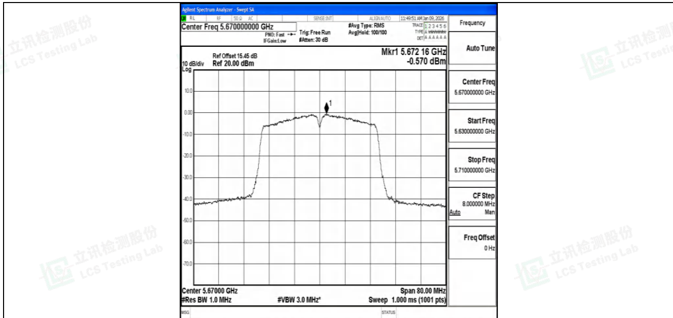
11N40SISO-Ant1-5670-PASS
