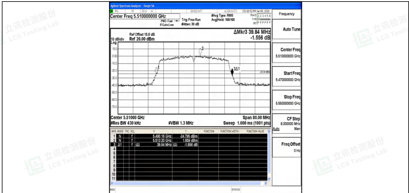
11AC40SISO-Ant2-5510
