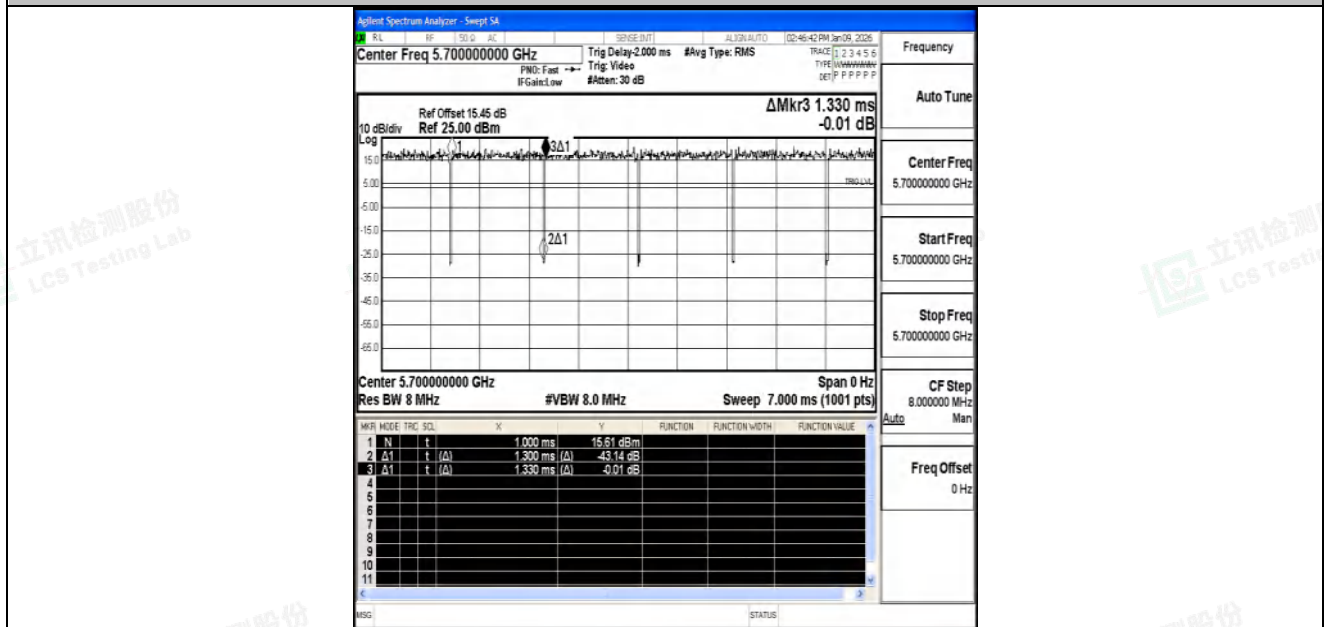
NTNV-11N20SISO-Ant2-5700
