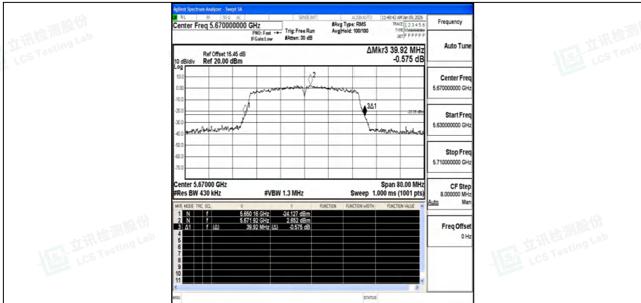
11N40SISO-Ant1-5670
