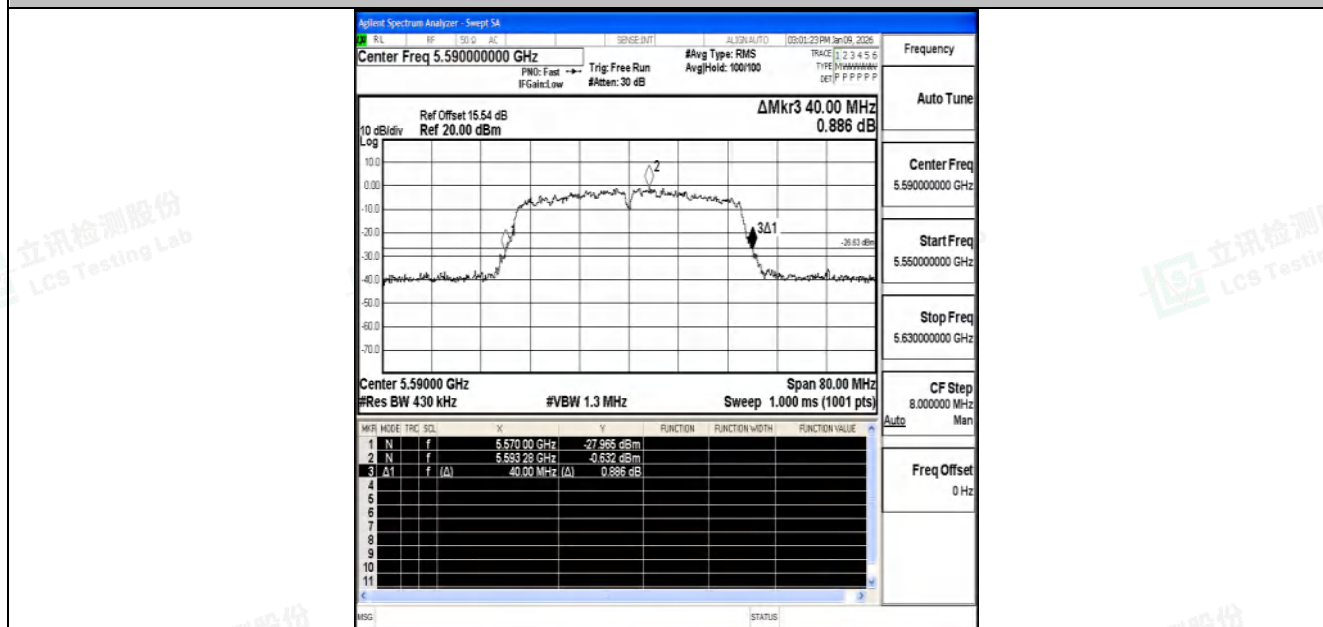
11N40SISO-Ant2-5590
