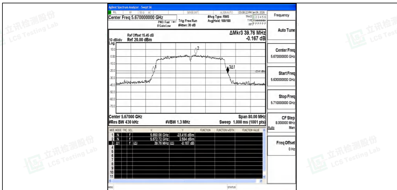
11N40SISO-Ant2-5670
