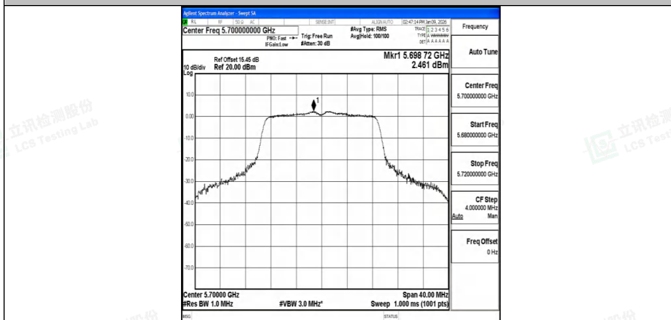
11N20SISO-Ant2-5700-PASS
