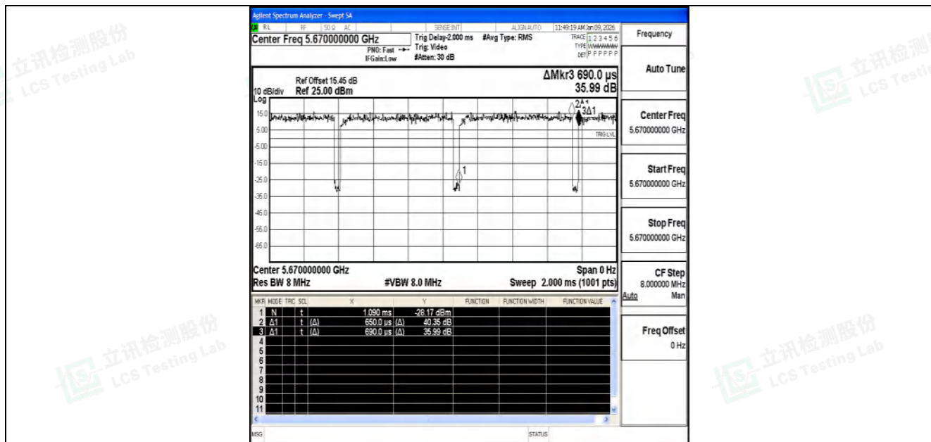
NTNV-11N40SISO-Ant1-5670
