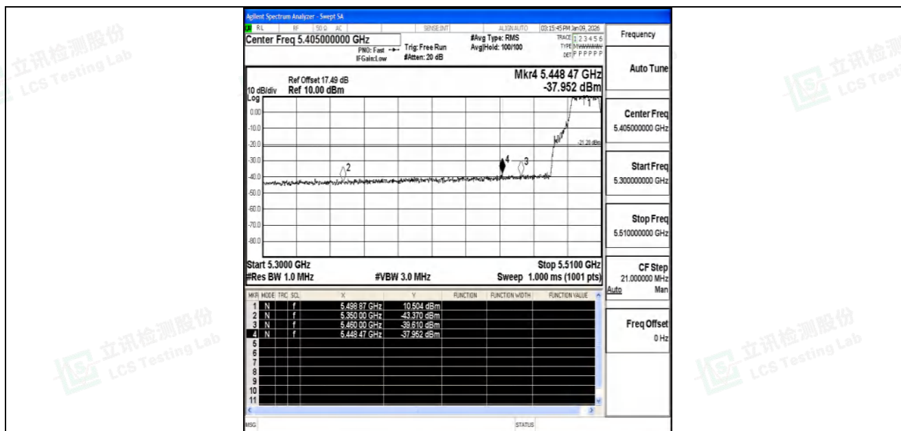
11AC20SISO-Ant2-5500-PASS
