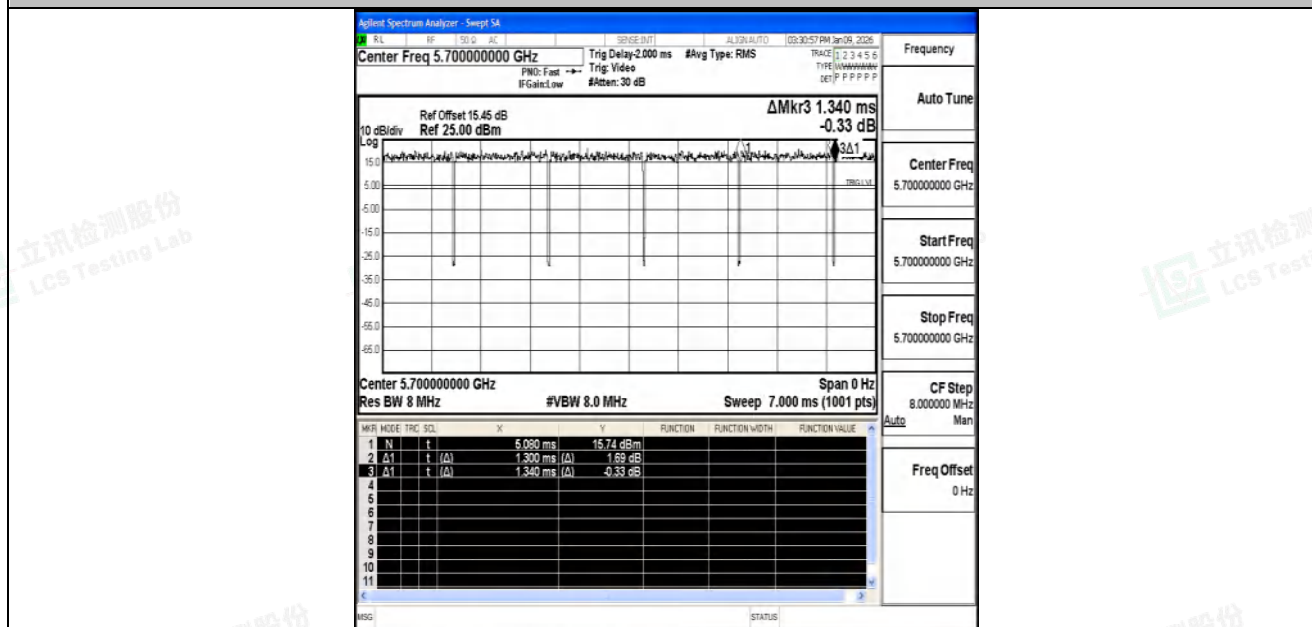
NTNV-11AC20SISO-Ant2-5700
