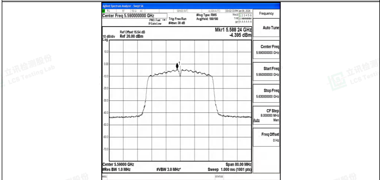
11N40SISO-Ant2-5590-PASS
