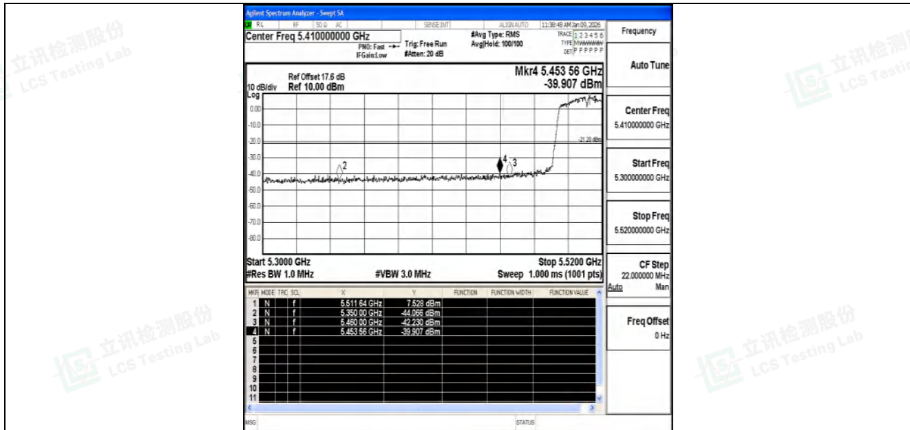
11N40SISO-Ant1-5510-PASS
