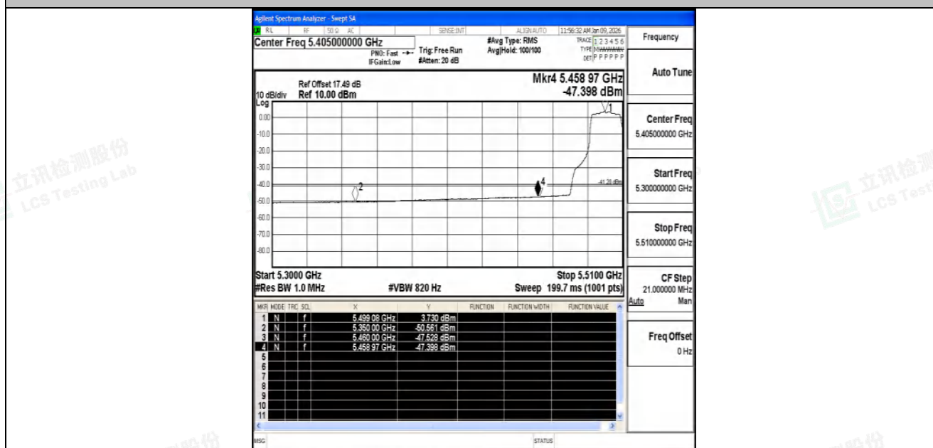
11AC20SISO-Ant1-5500-PASS
