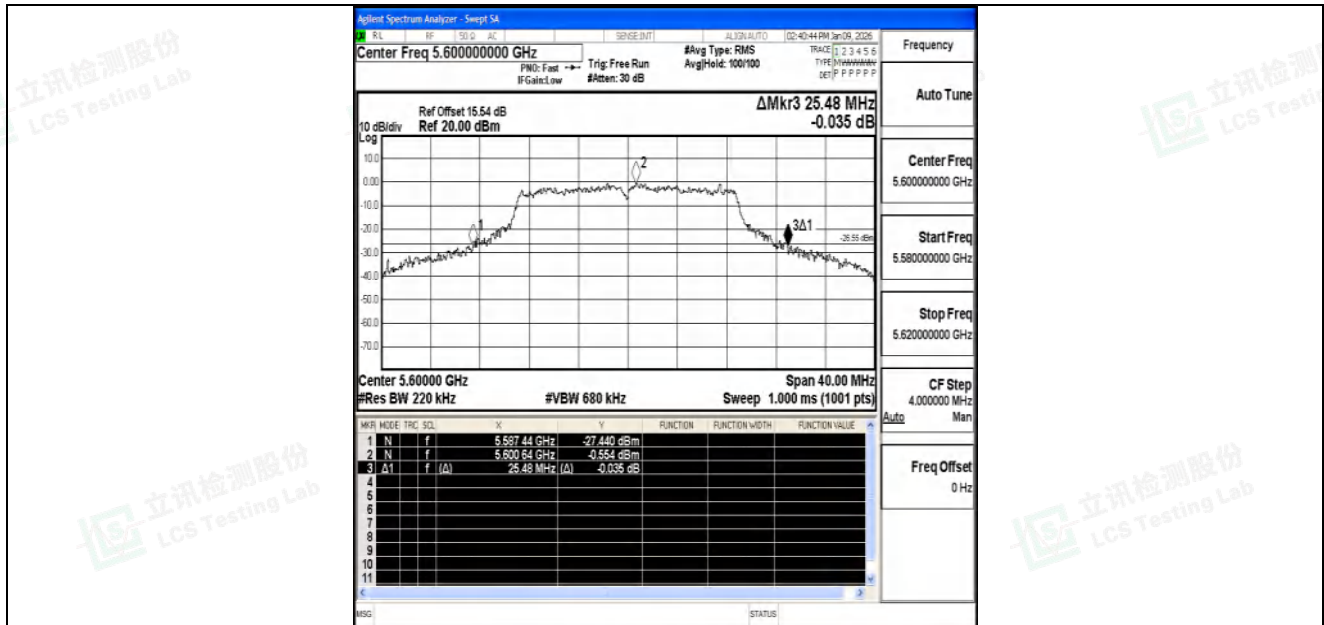
11N20SISO-Ant2-5600
