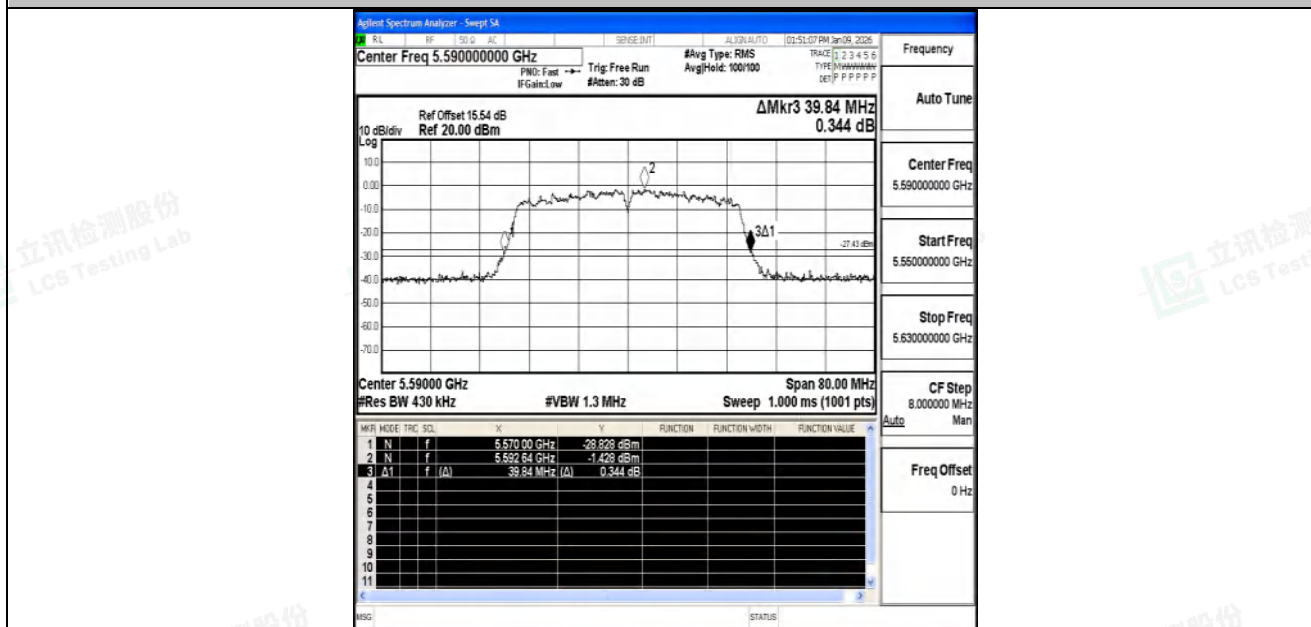
11AC40SISO-Ant1-5590
