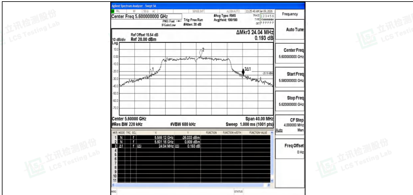
11N20SISO-Ant1-5600
