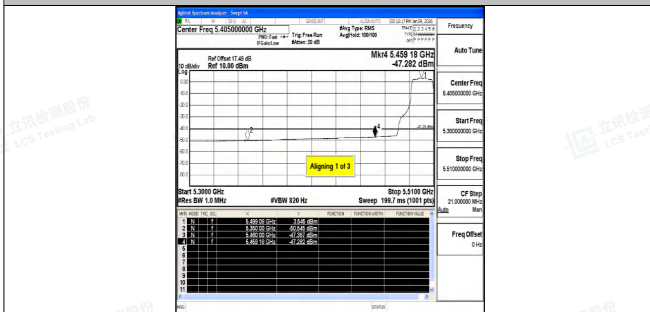
11AC20SISO-Ant2-5500-PASS
