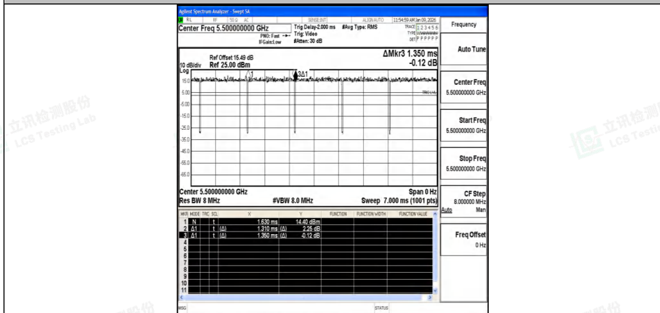
NTNV-11AC20SISO-Ant1-5500
