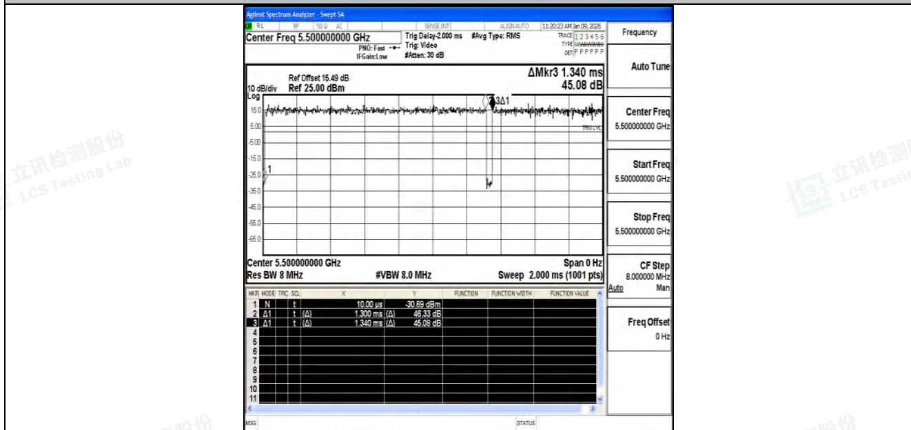
NTNV-11N20SISO-Ant1-5500
