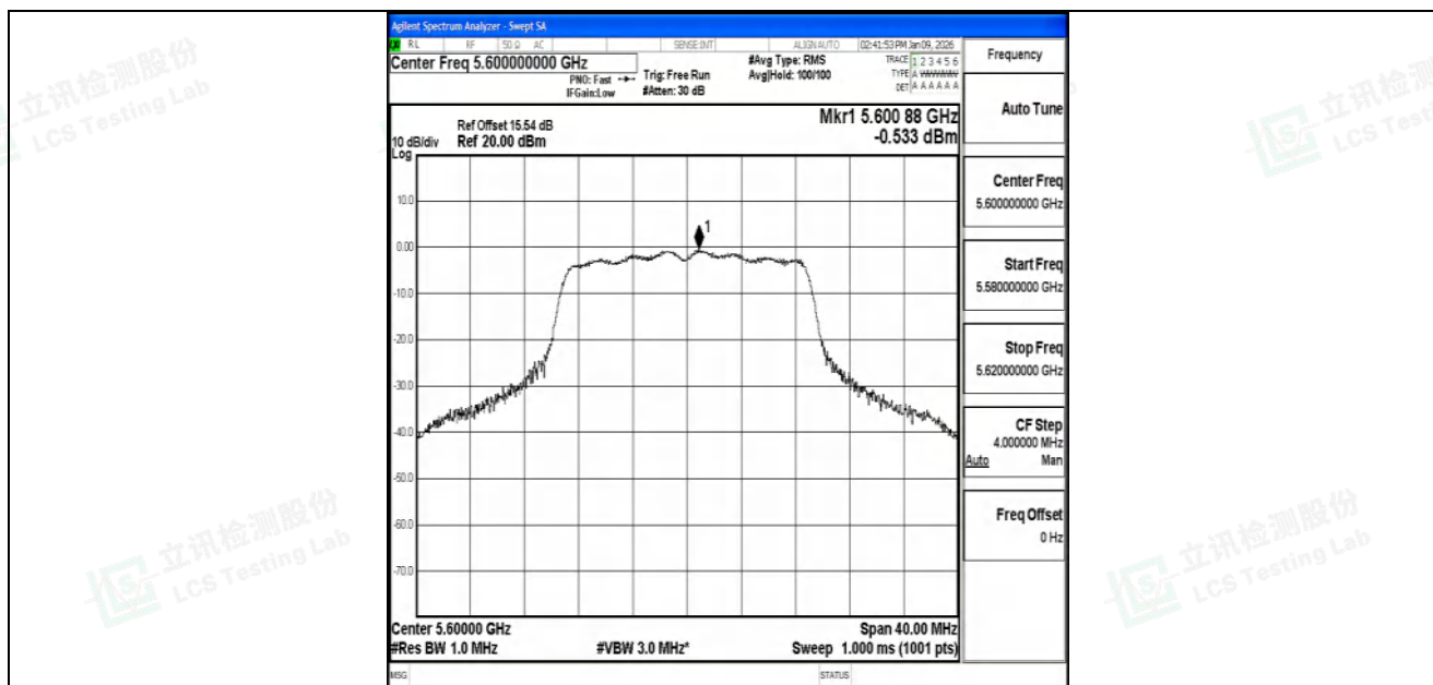
11N20SISO-Ant2-5600-PASS
