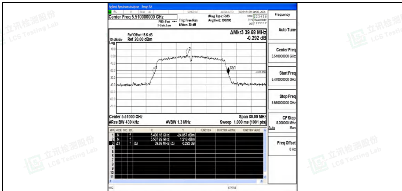
11N40SISO-Ant2-5510
