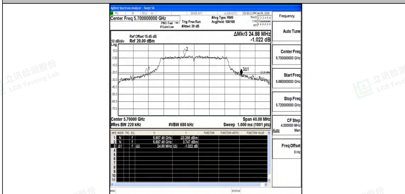
11AC20SISO-Ant2-5700
