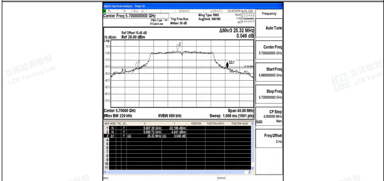
11N20SISO-Ant2-5700
