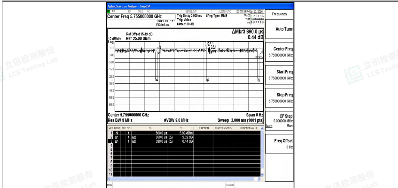
NTNV-11AC40SISO-Ant1-5755
