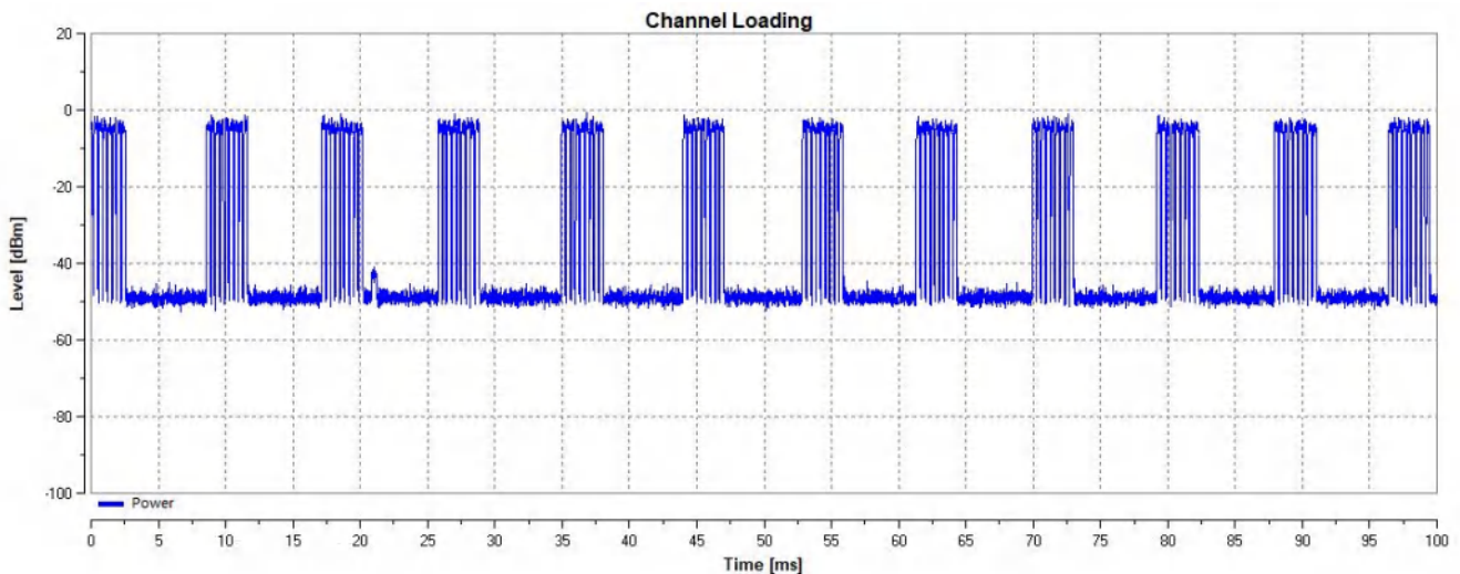
802.11ac-VHT40
