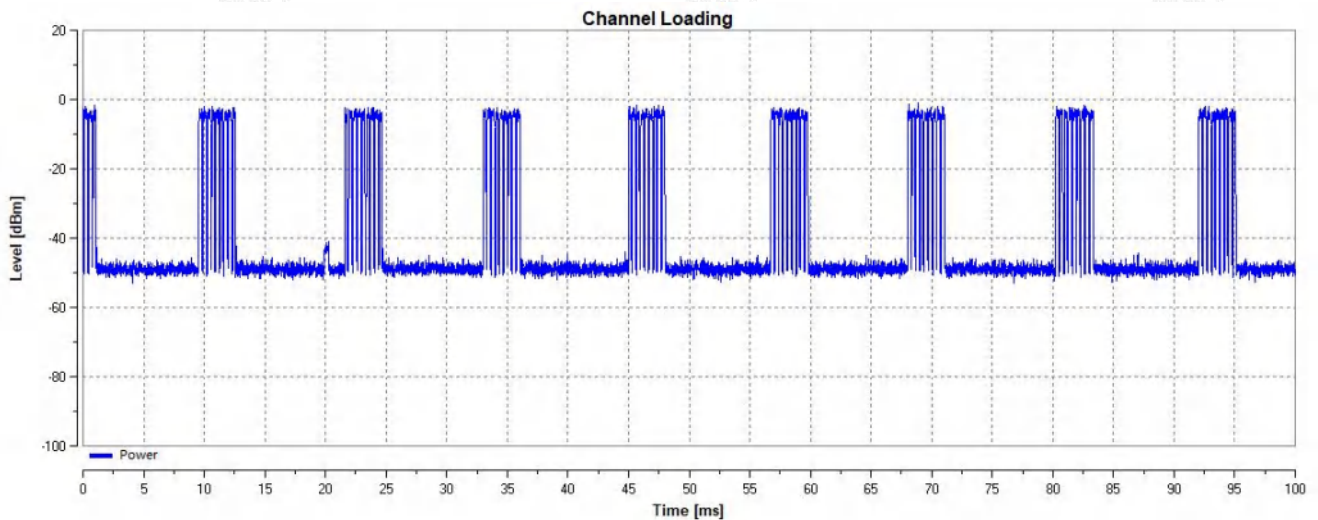
802.11ac-VHT20
