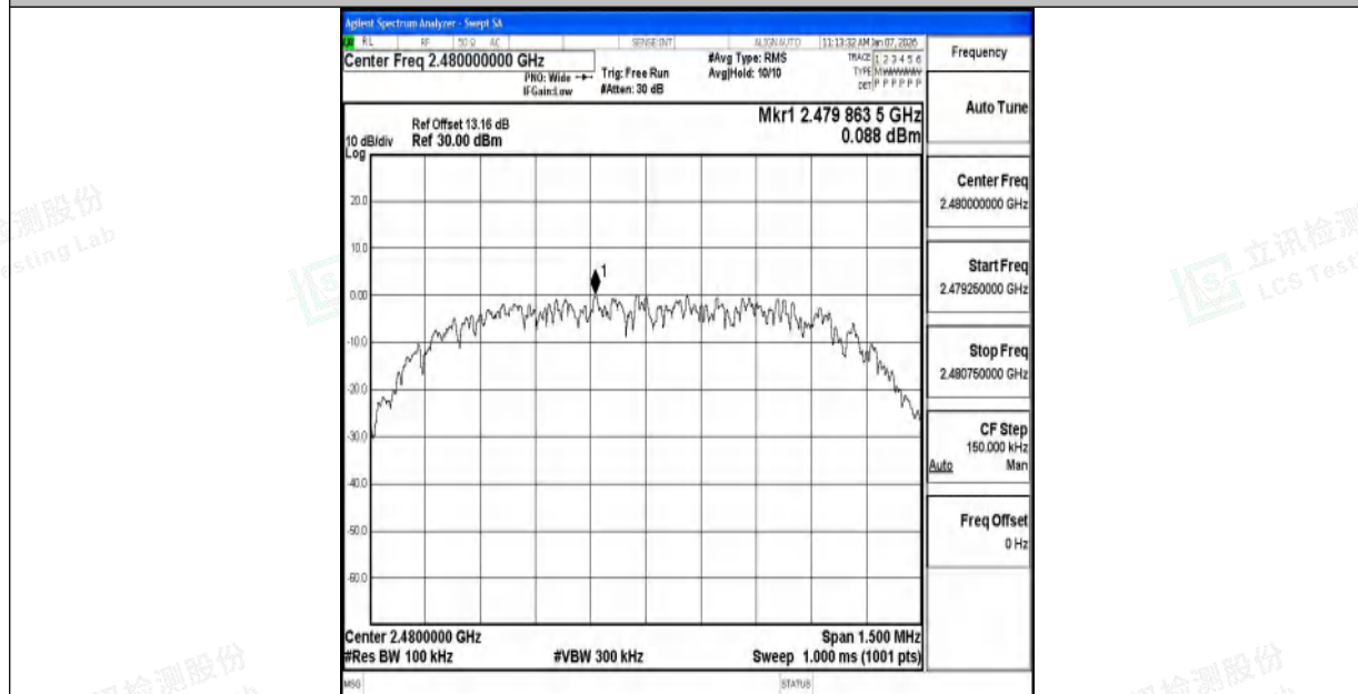
2DH5-Ant1-2480-0~Reference-PASS
