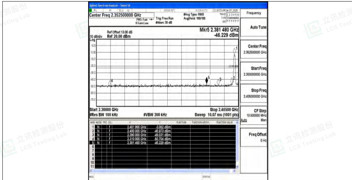
3DH5-Ant1-2402-PASS
