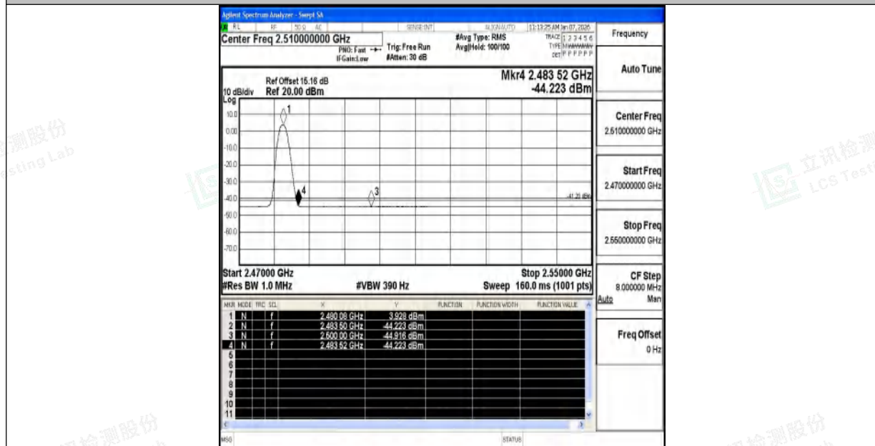
2DH5-Ant1-2480-PASS
