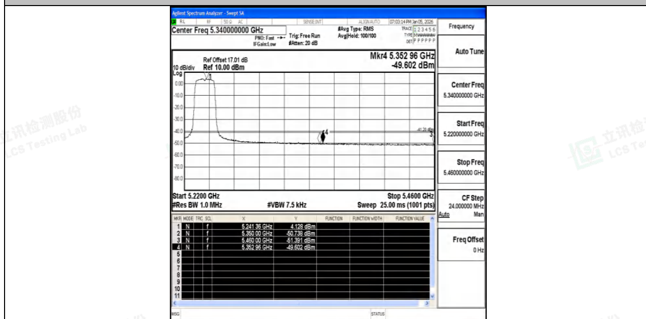
11AC20SISO-Ant1-5240-PASS
