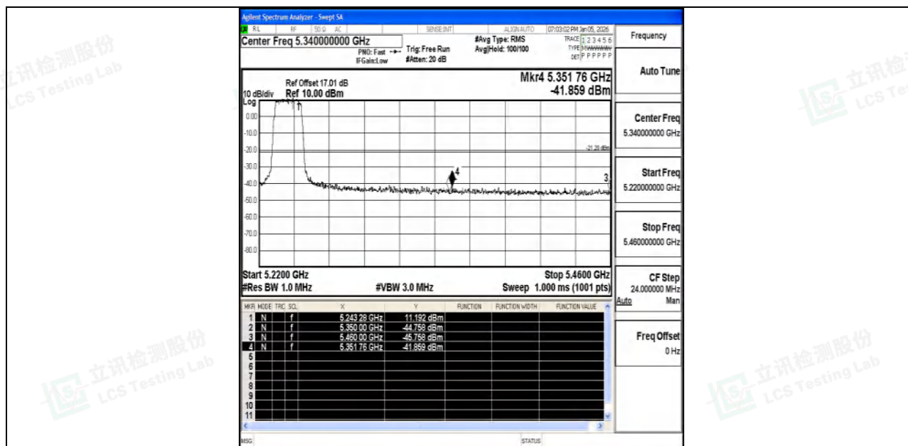
11AC20SISO-Ant1-5240-PASS
