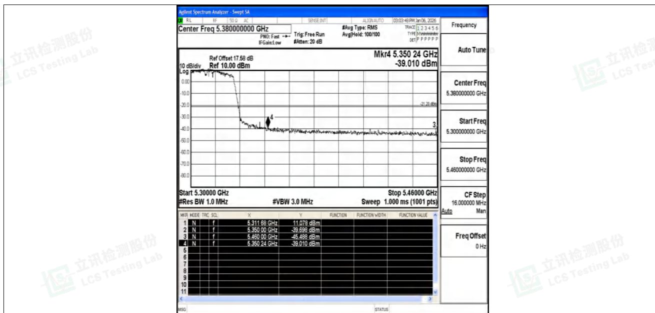
11AC40SISO-Ant2-5310-PASS
