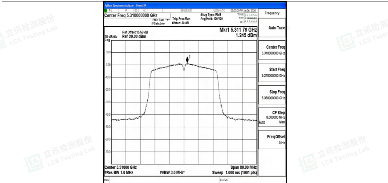
11AC40SISO-Ant2-5310-PASS
