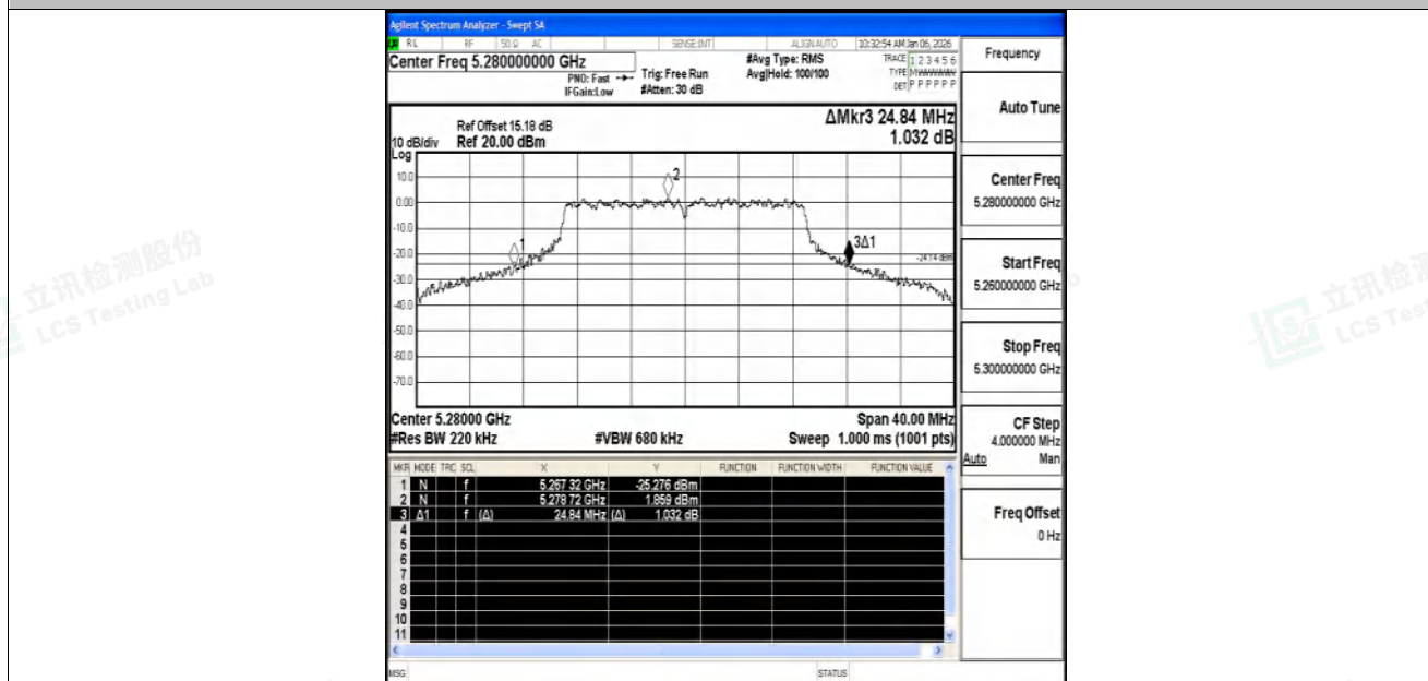
11AC20SISO-Ant1-5280
