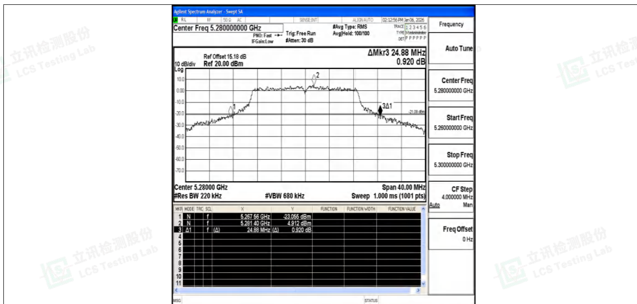
11N20SISO-Ant2-5280
