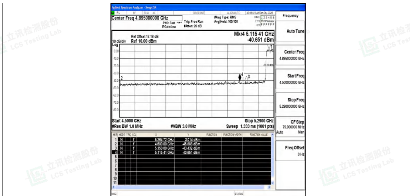
11AC40SISO-Ant1-5270-PASS
