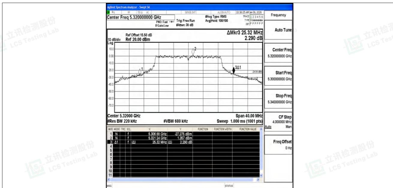
11AC20SISO-Ant1-5320
