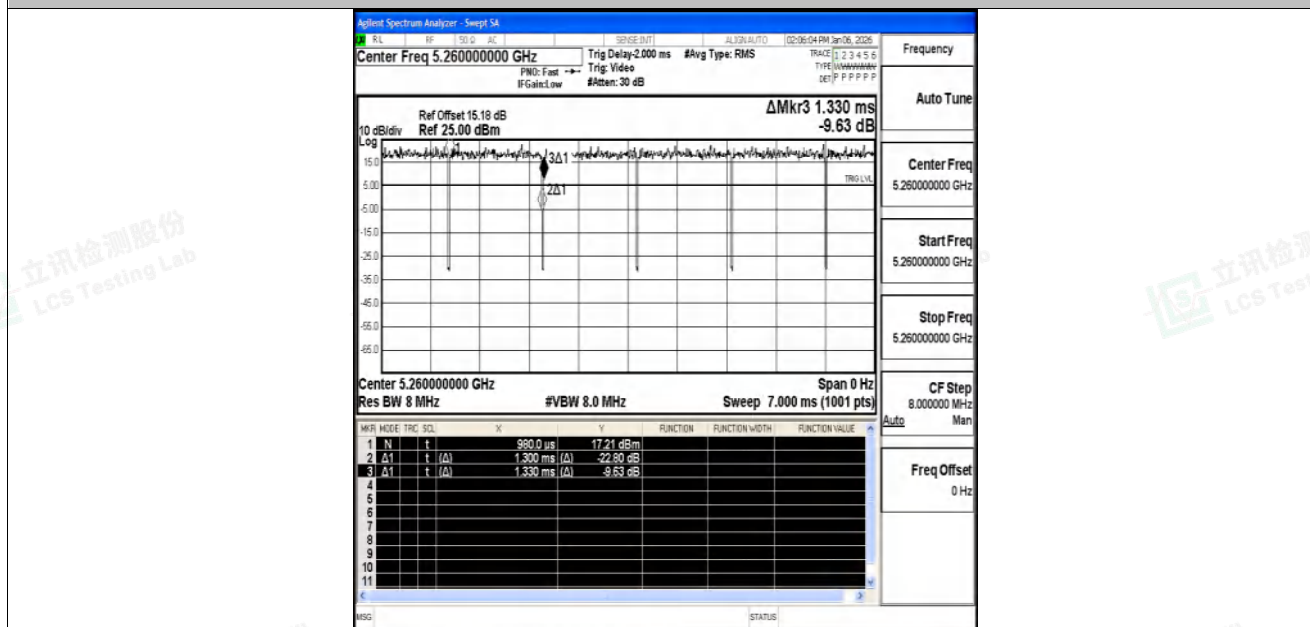
NTNV-11N20SISO-Ant2-5260
