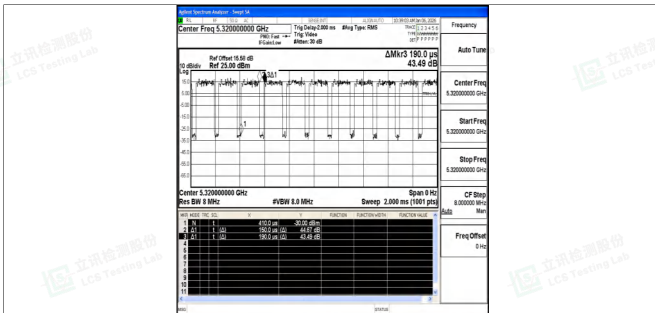
NTNV-11AC20SISO-Ant1-5320
