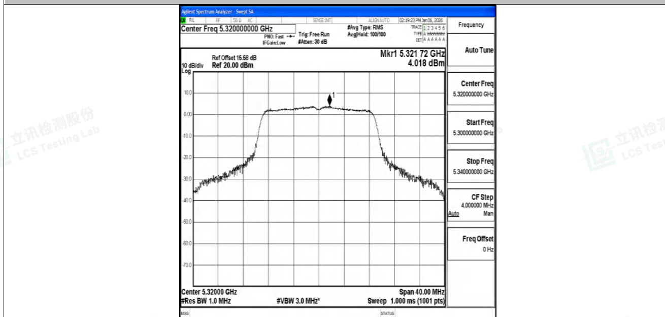
11N20SISO-Ant2-5320-PASS
