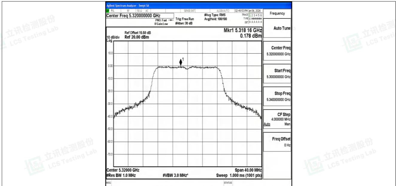
11AC20SISO-Ant2-5320-PASS
