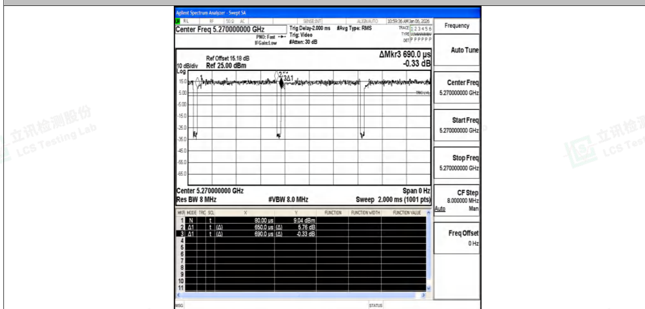
NTNV-11AC40SISO-Ant1-5270
