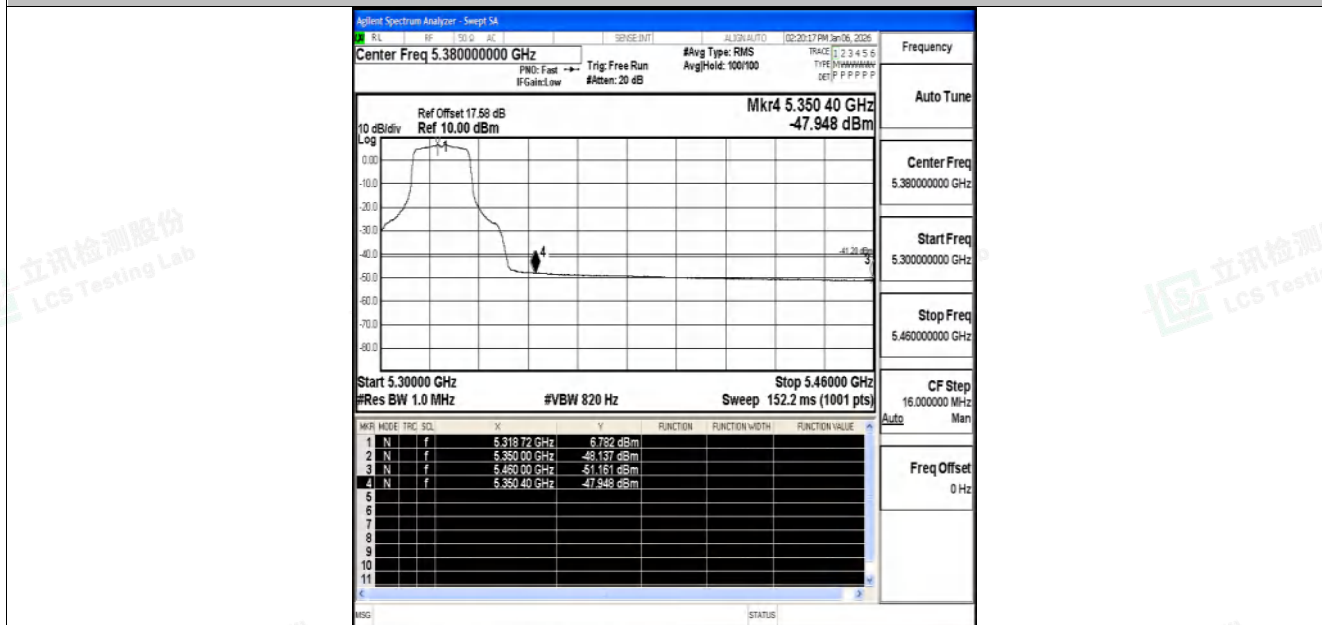
11N20SISO-Ant2-5320-PASS
