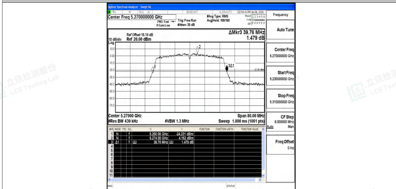
11AC40SISO-Ant2-5270
