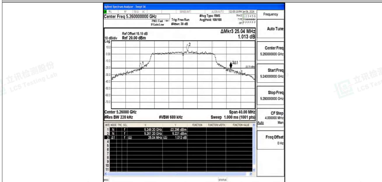
11N20SISO-Ant2-5260
