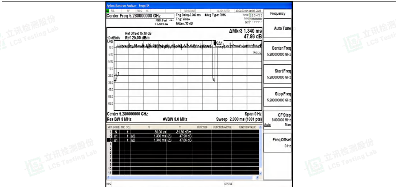
NTNV-11N20SISO-Ant1-5280
