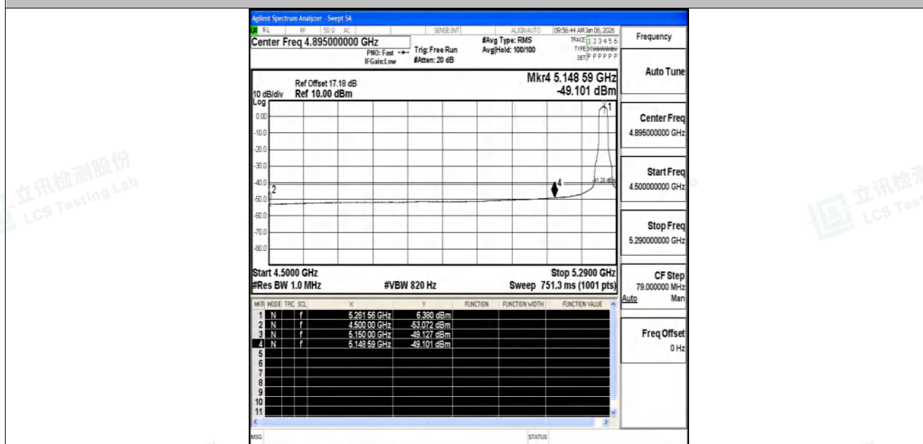
11N20SISO-Ant1-5260-PASS
