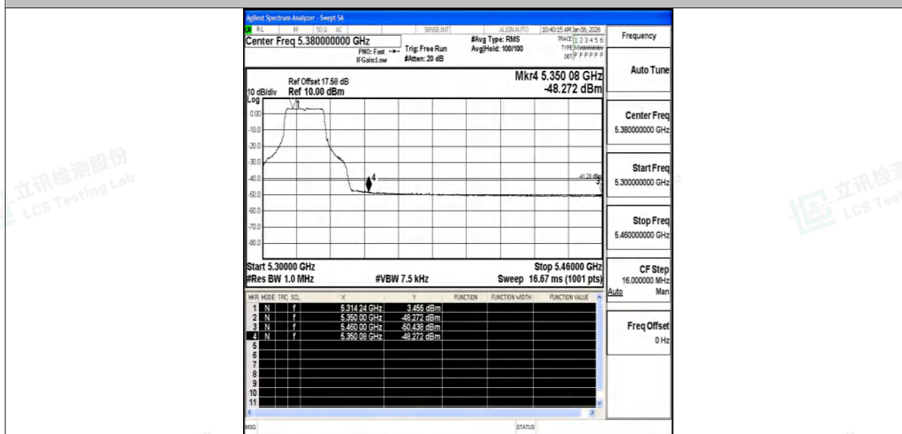
11AC20SISO-Ant1-5320-PASS
