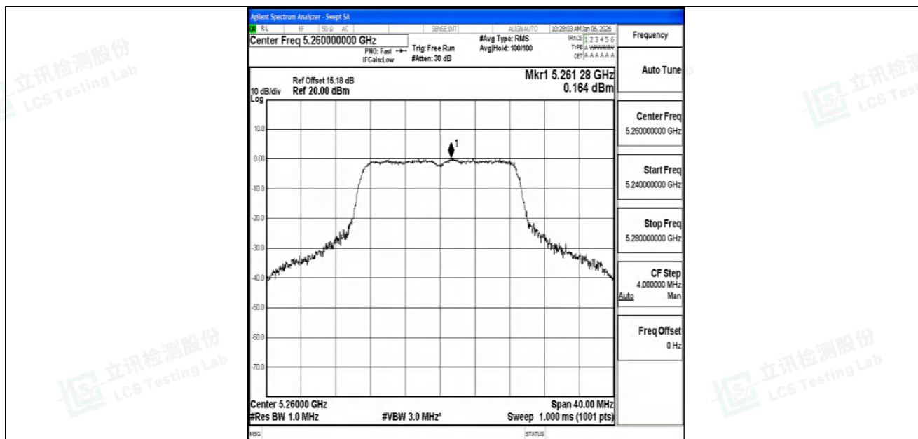
11AC20SISO-Ant1-5260-PASS
