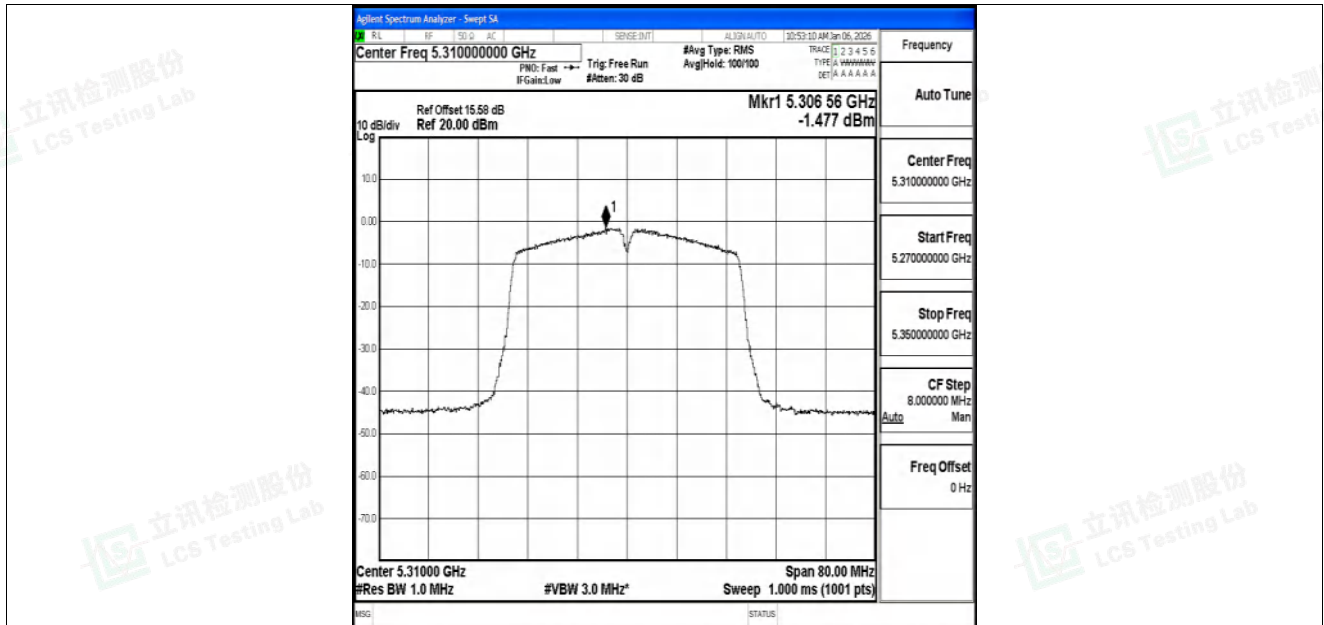
11AC40SISO-Ant1-5310-PASS
