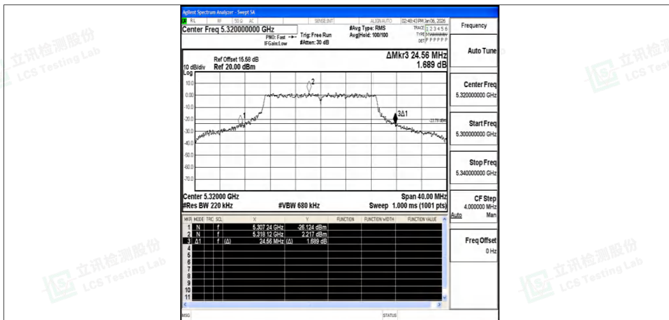
11AC20SISO-Ant2-5320
