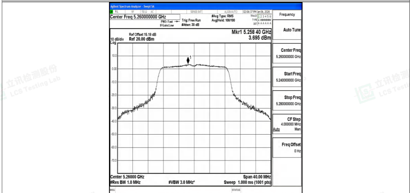
11N20SISO-Ant2-5260-PASS
