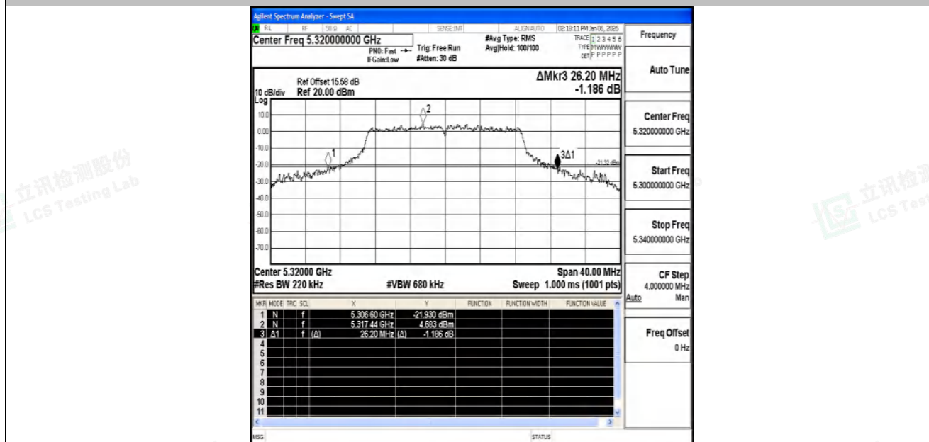
11N20SISO-Ant2-5320
