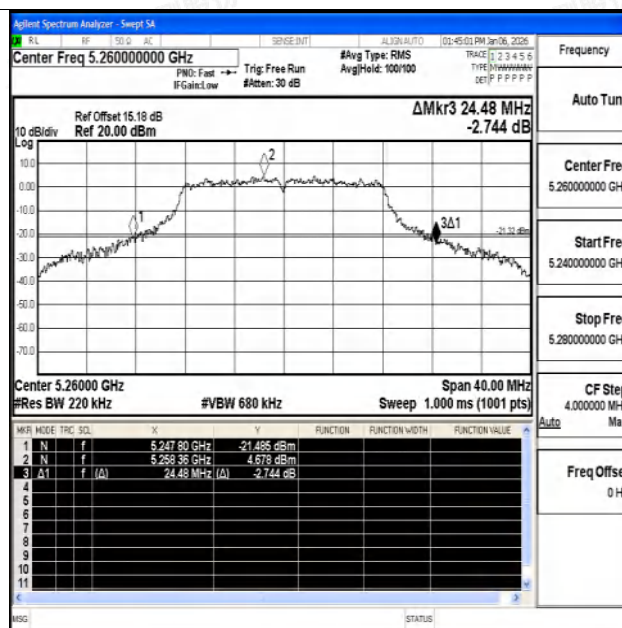
11A-Ant2-5260
