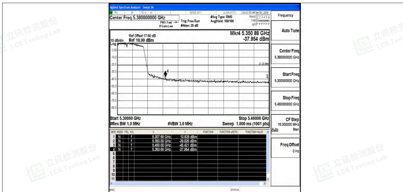
11N40SISO-Ant1-5310-PASS
