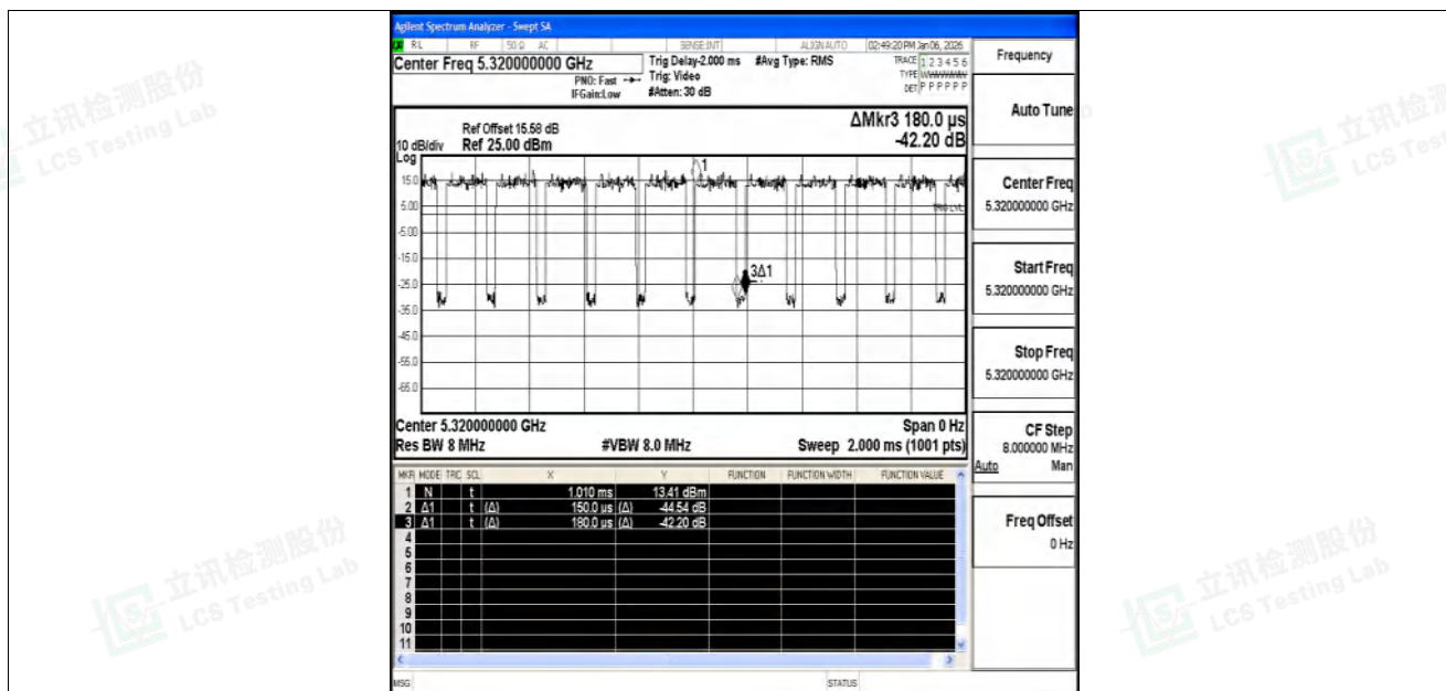
NTNV-11AC20SISO-Ant2-5320
