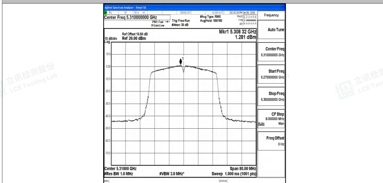
11N40SISO-Ant2-5310-PASS
