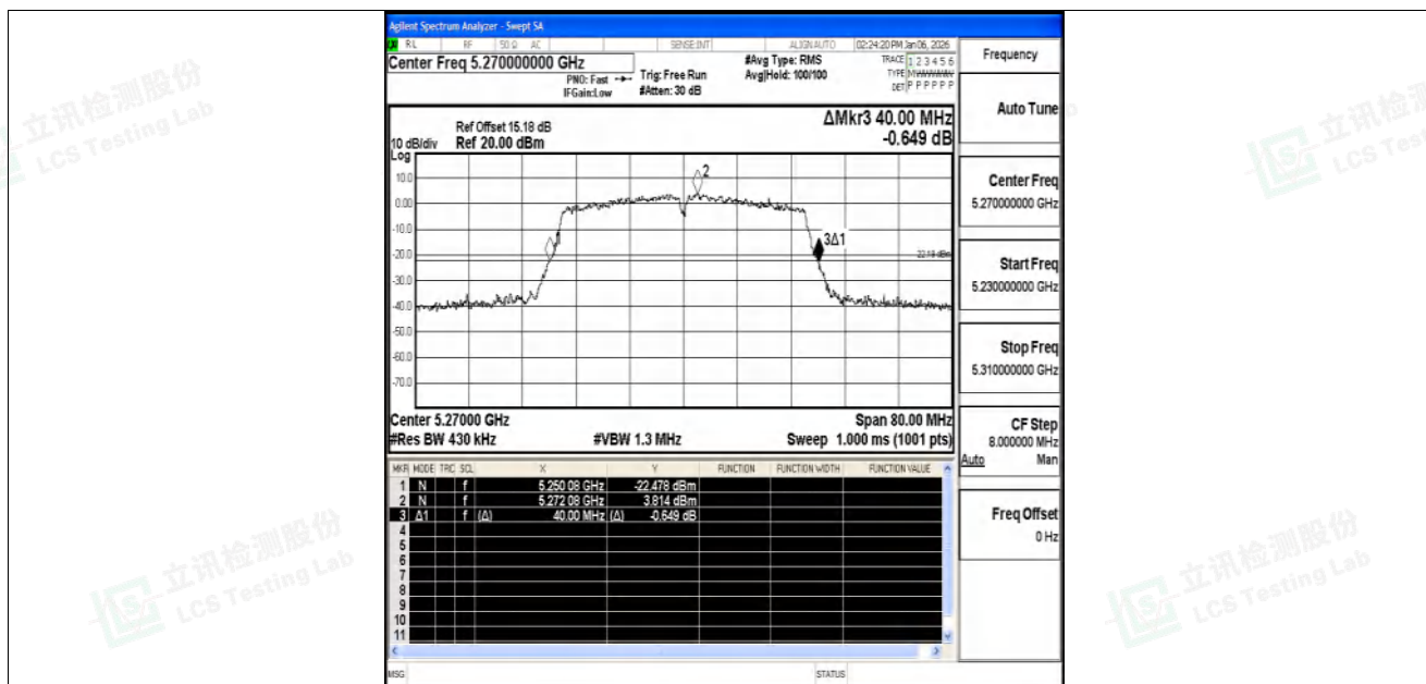
11N40SISO-Ant2-5270
