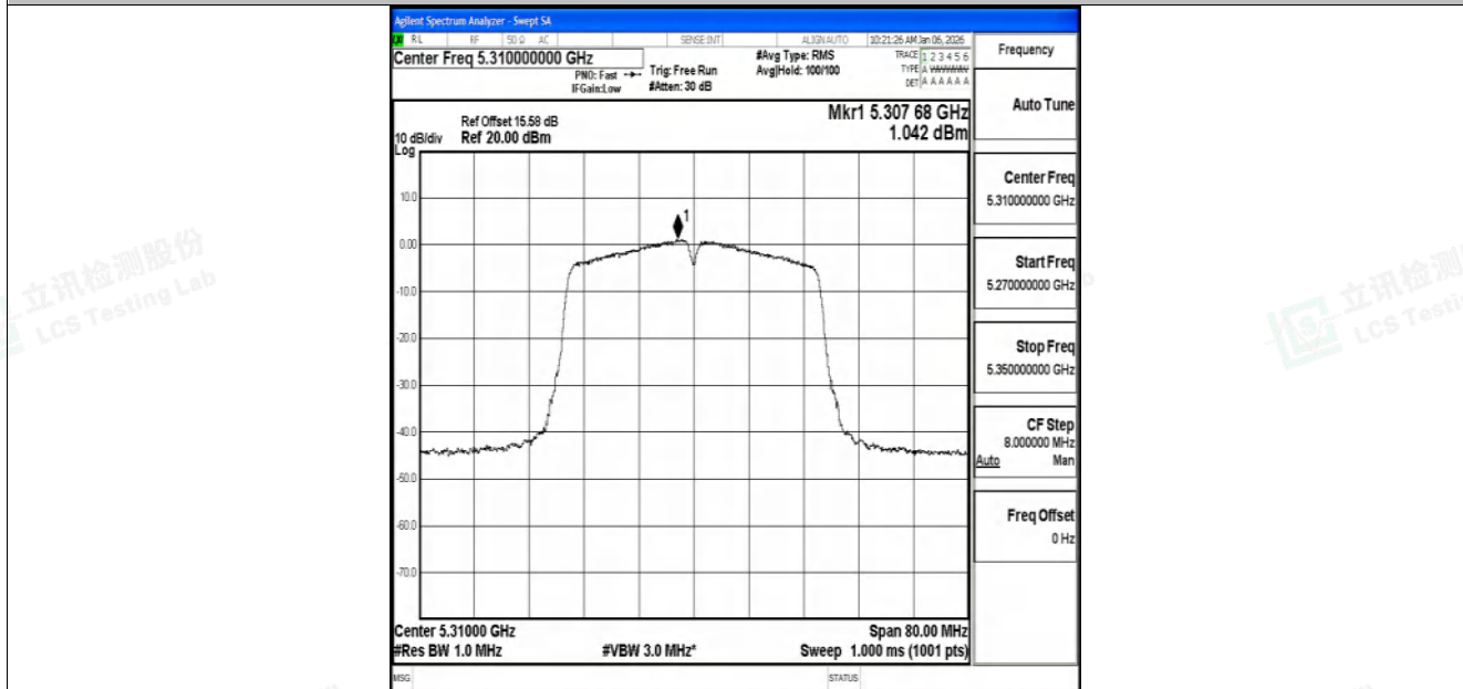
11N40SISO-Ant1-5310-PASS
