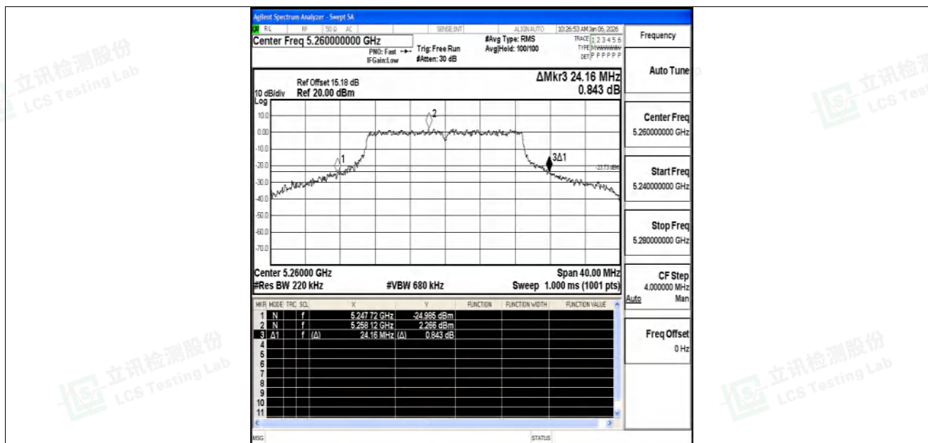
11AC20SISO-Ant1-5260
