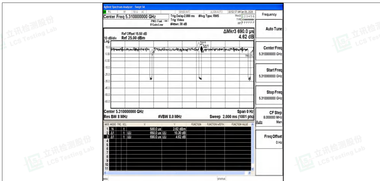
NTNV-11AC40SISO-Ant1-5310
