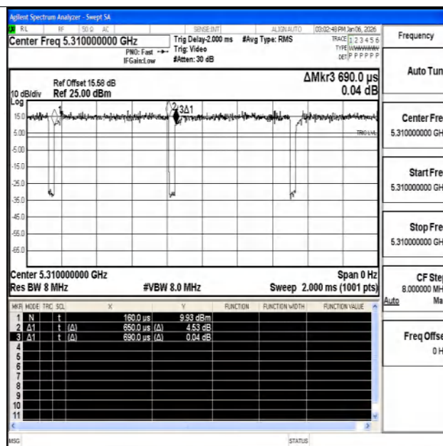
NTNV-11AC40SISO-Ant2-5310
