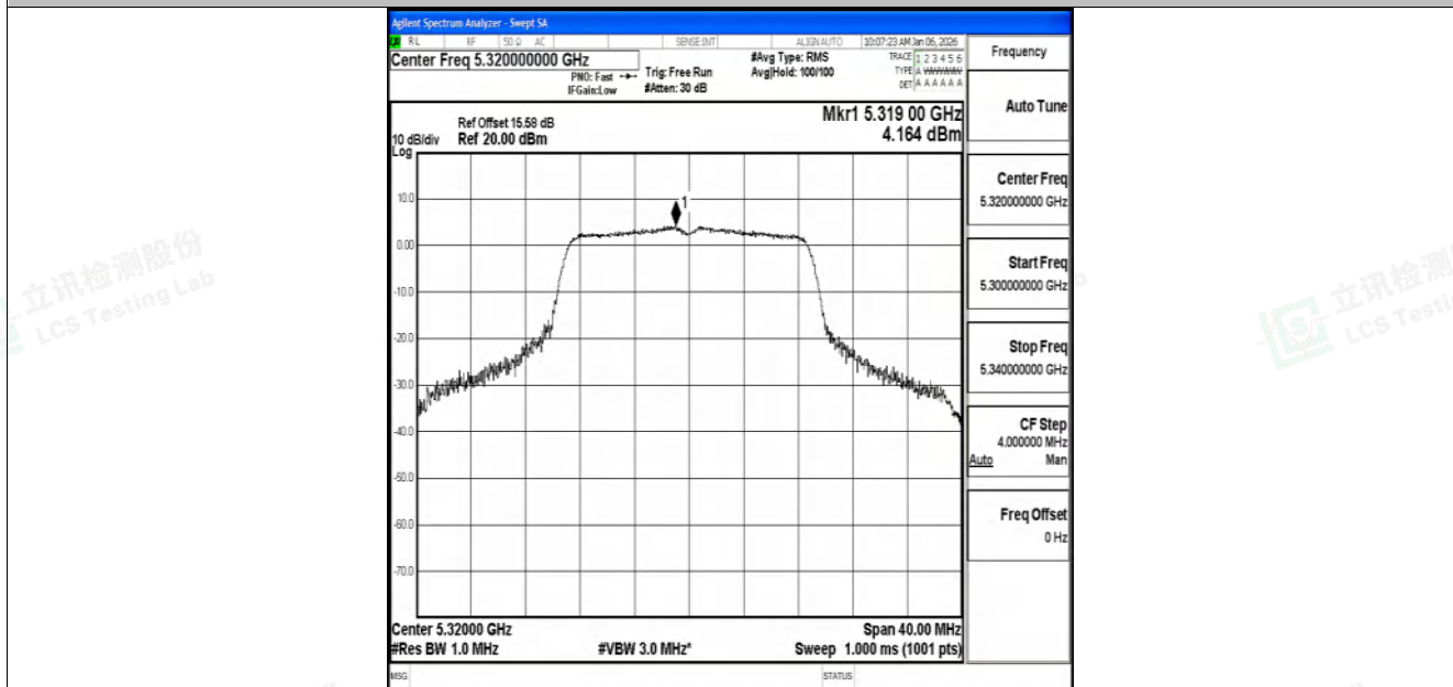
11N20SISO-Ant1-5320-PASS
