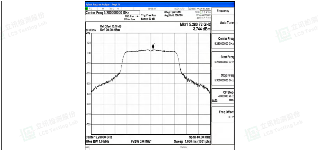
11N20SISO-Ant1-5280-PASS
