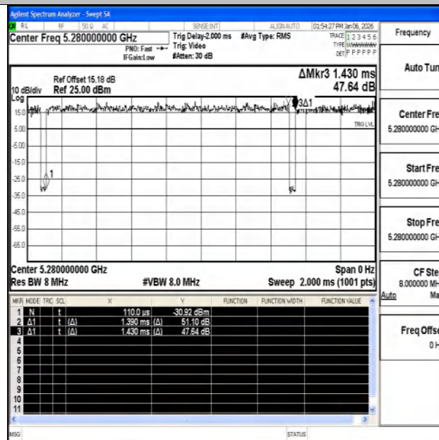
NTNV-11A-Ant2-5280
