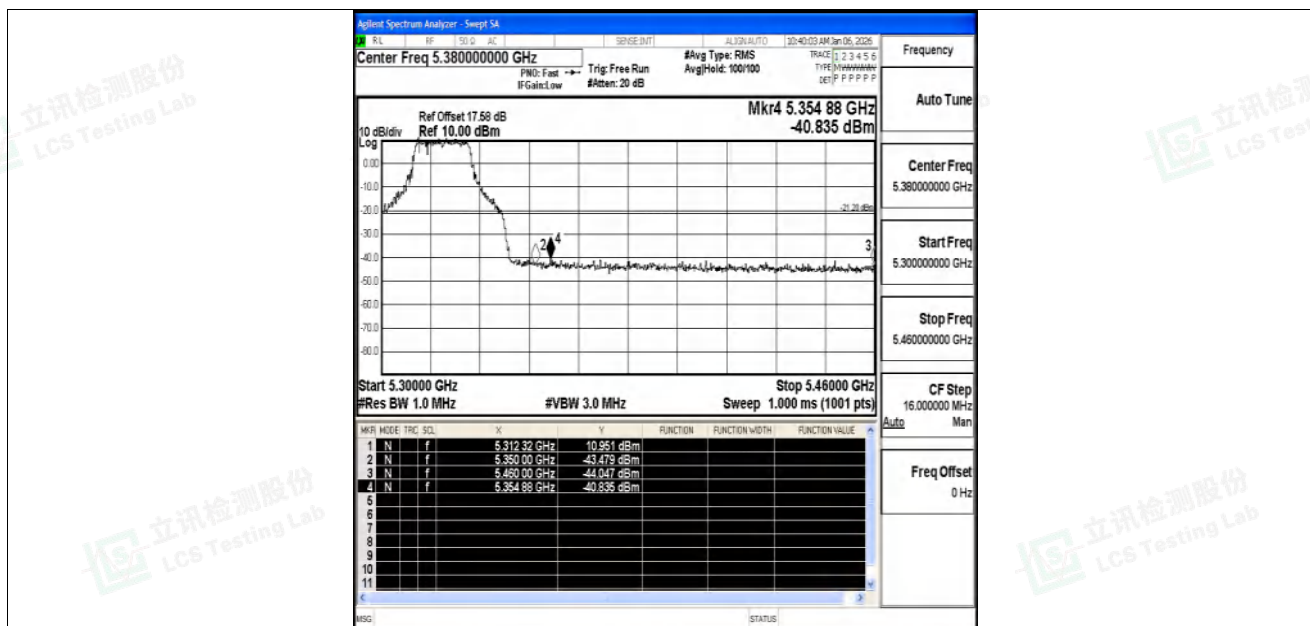
11AC20SISO-Ant1-5320-PASS
