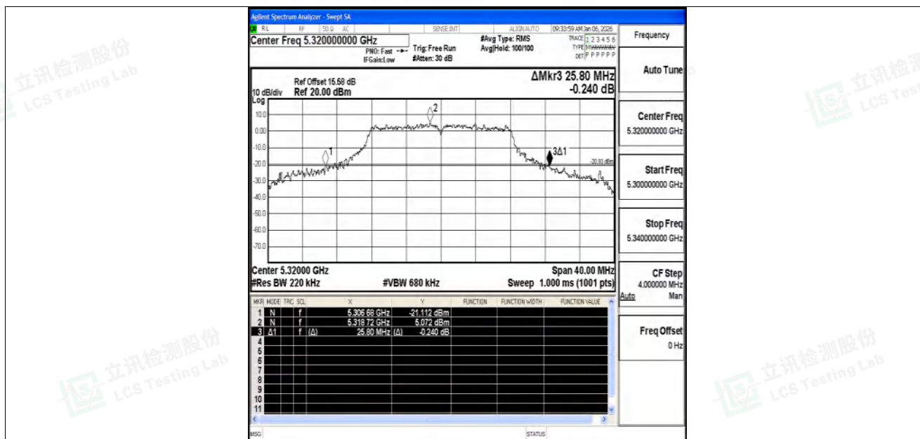
11A-Ant1-5320
