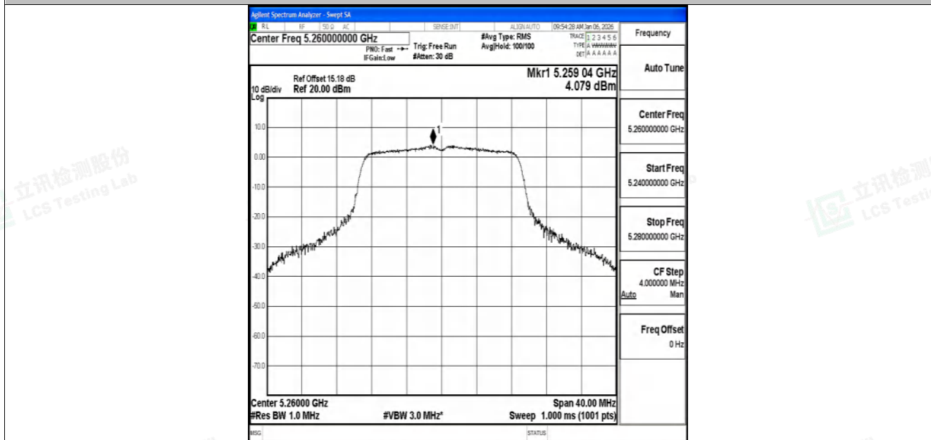
11N20SISO-Ant1-5260-PASS
