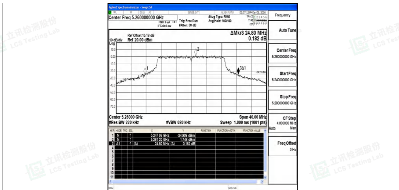
11AC20SISO-Ant2-5260
