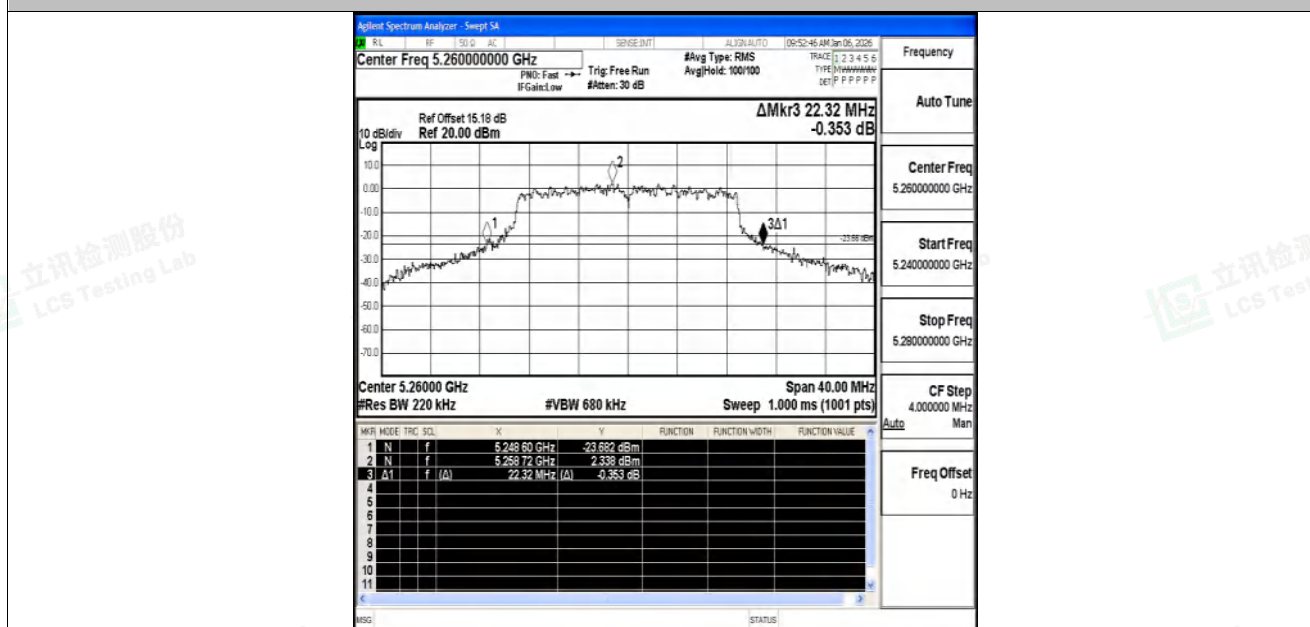
11N20SISO-Ant1-5260
