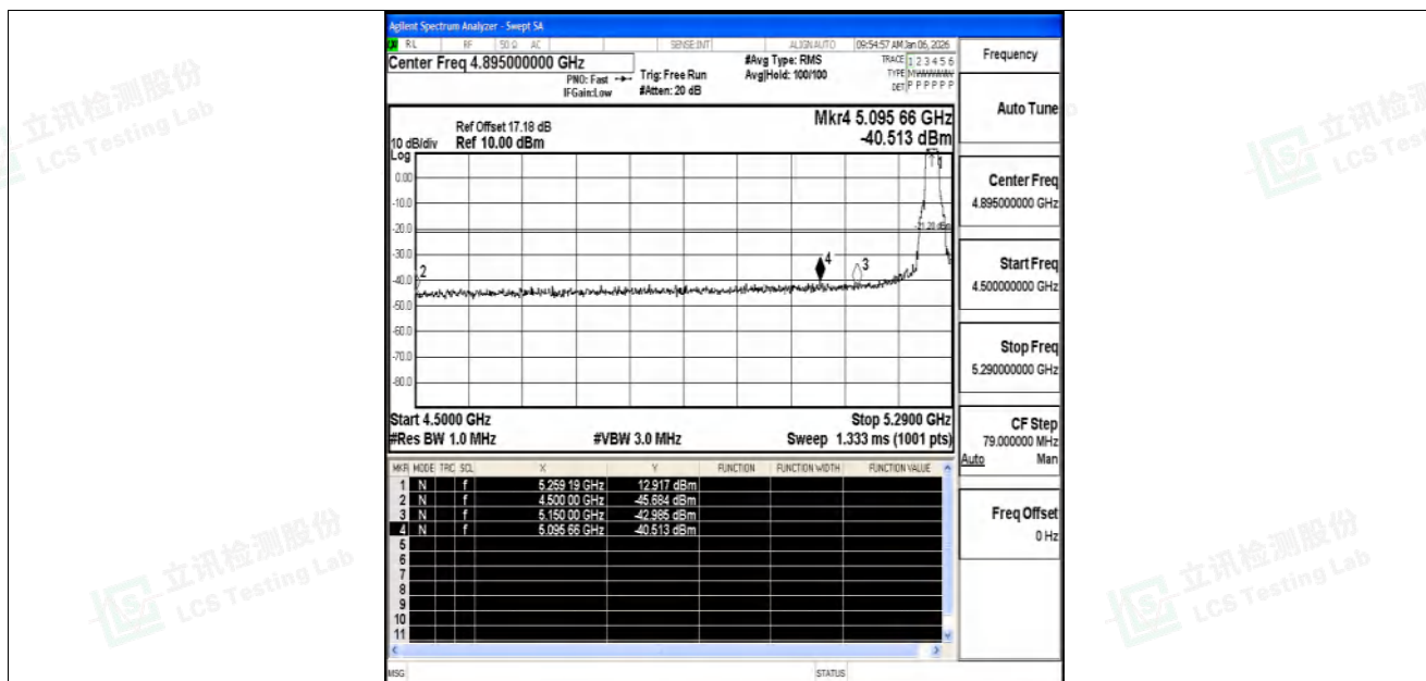
11N20SISO-Ant1-5260-PASS
