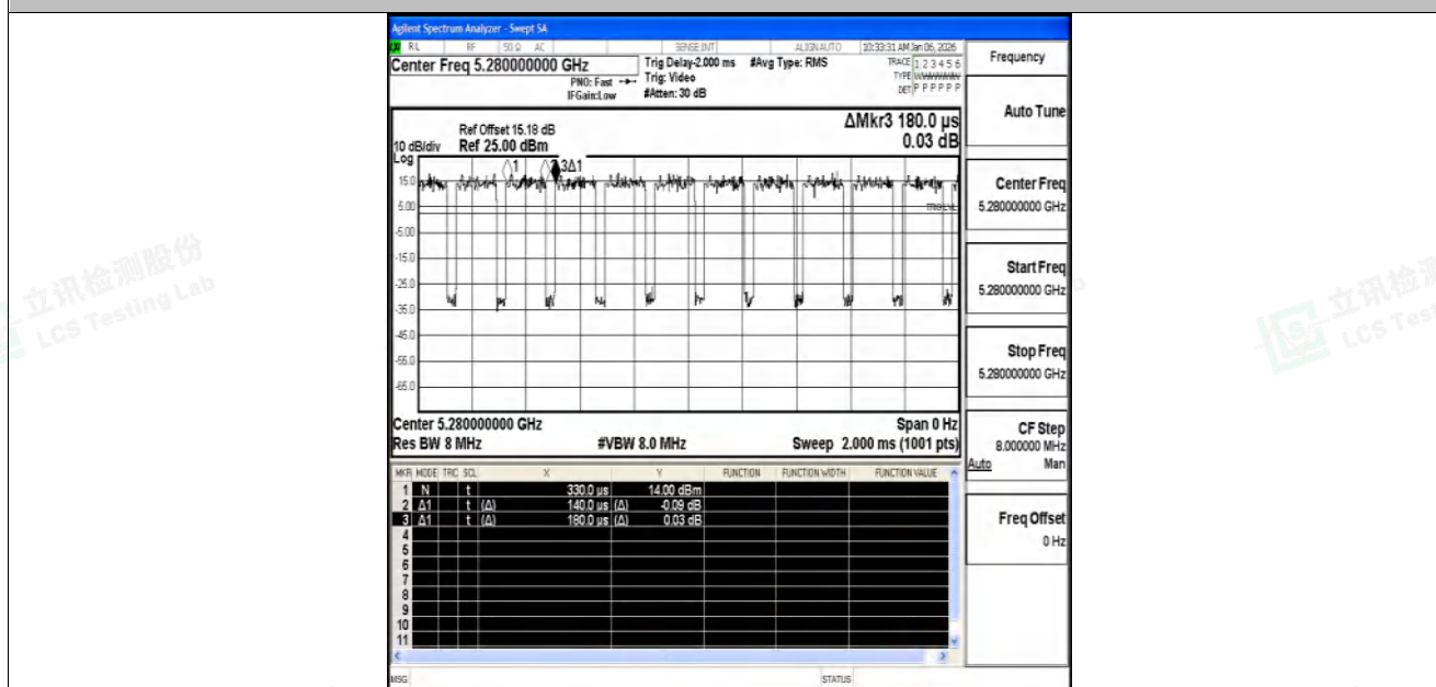
NTNV-11AC20SISO-Ant1-5280
