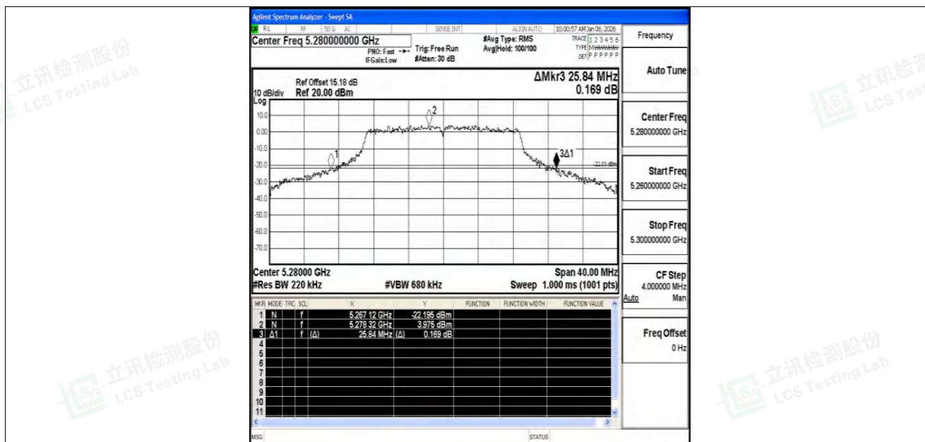
11N20SISO-Ant1-5280
