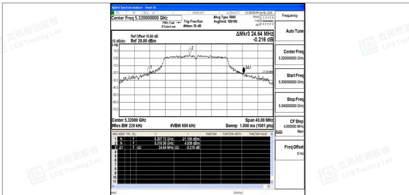
11A-Ant2-5320
