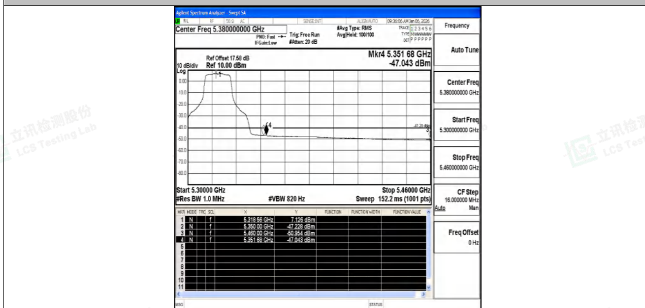
11A-Ant1-5320-PASS
