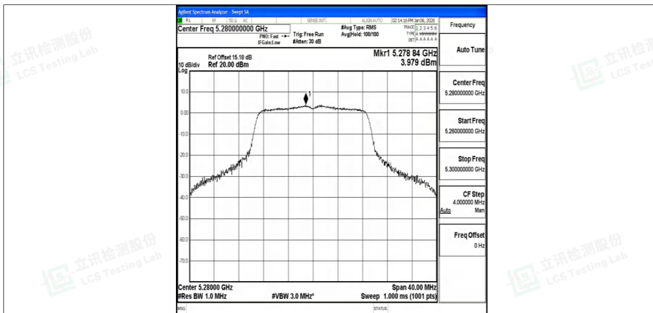
11N20SISO-Ant2-5280-PASS
