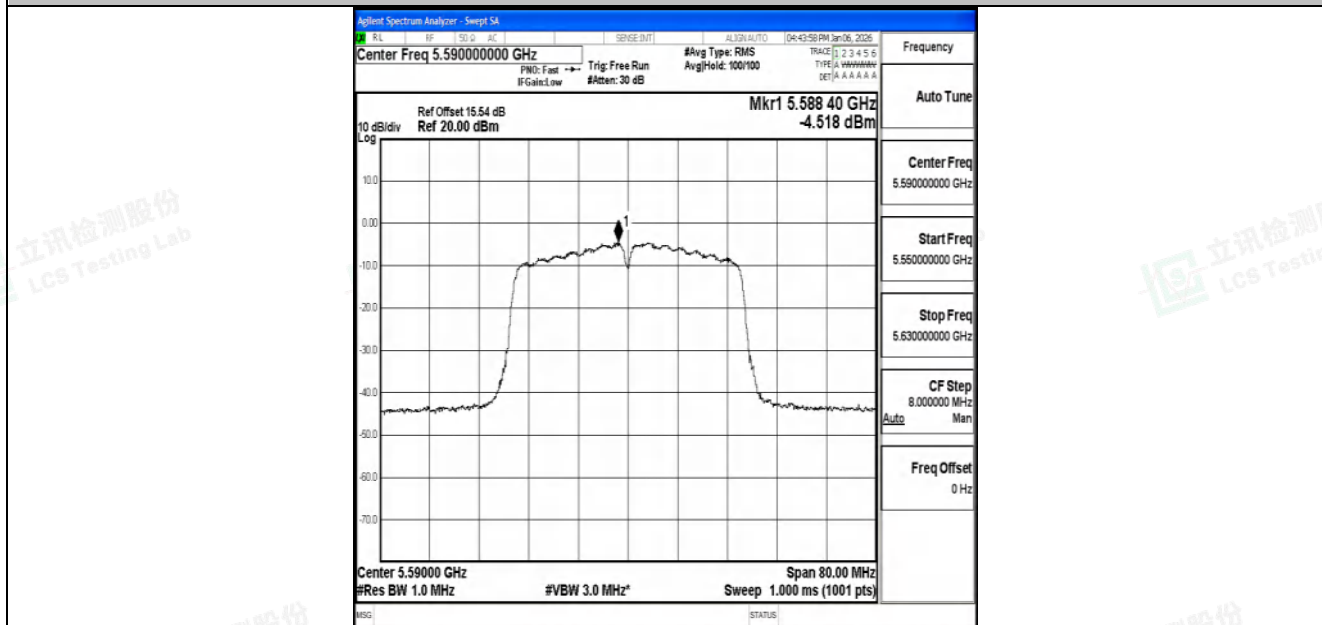
11AC40SISO-Ant1-5590-PASS
