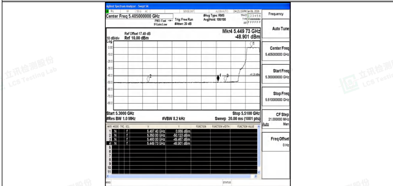
11AC20SISO-Ant1-5500-PASS
