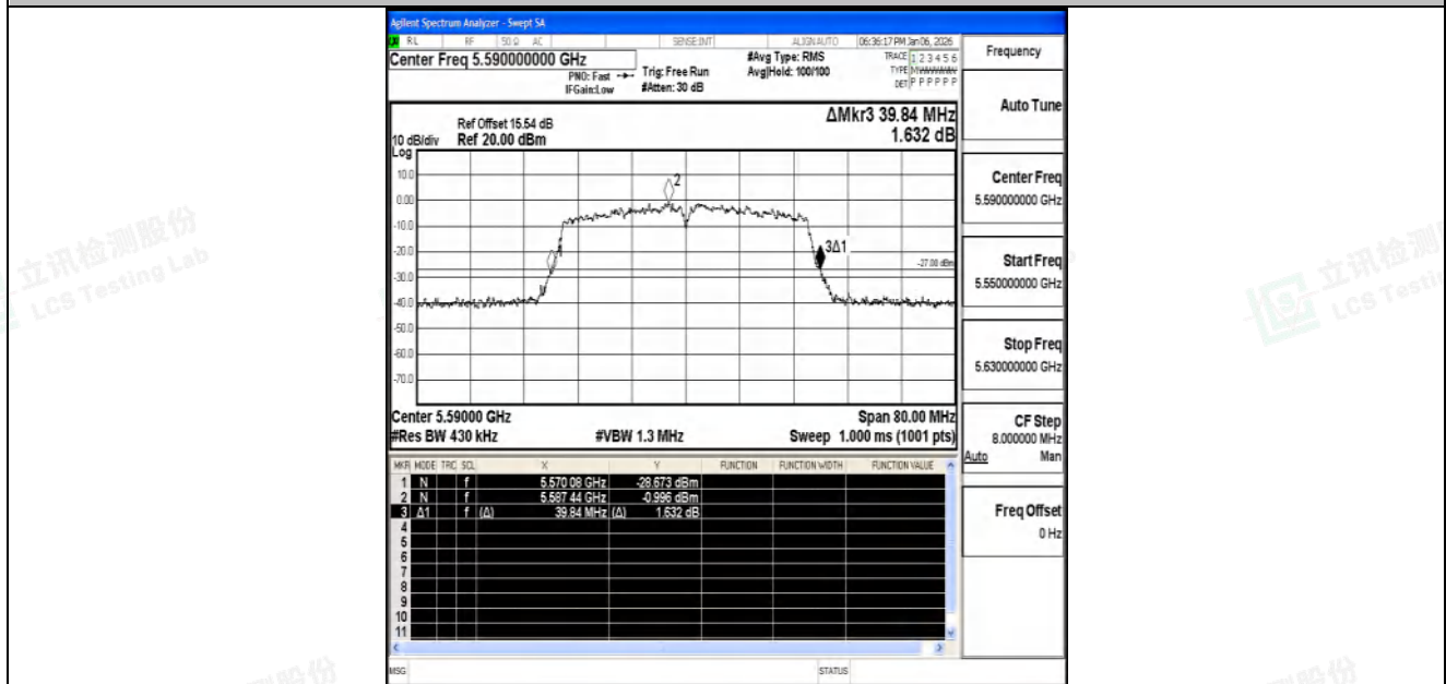
11AC40SISO-Ant2-5590
