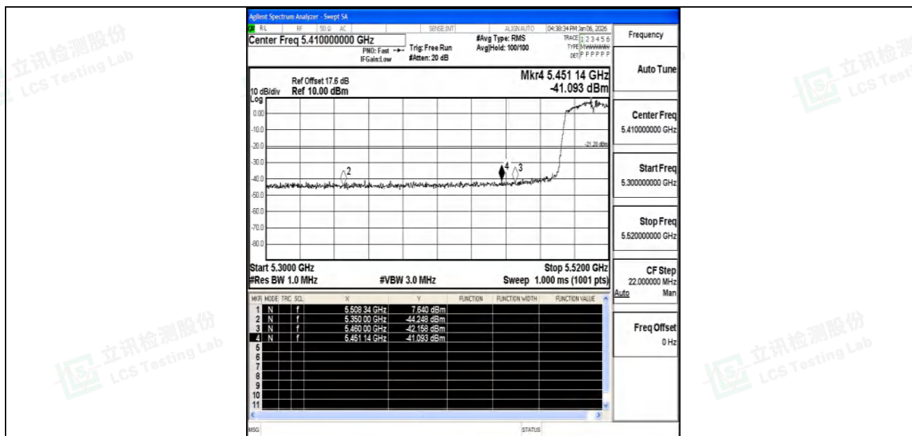
11AC40SISO-Ant1-5510-PASS
