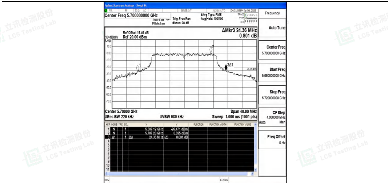
11AC20SISO-Ant1-5700
