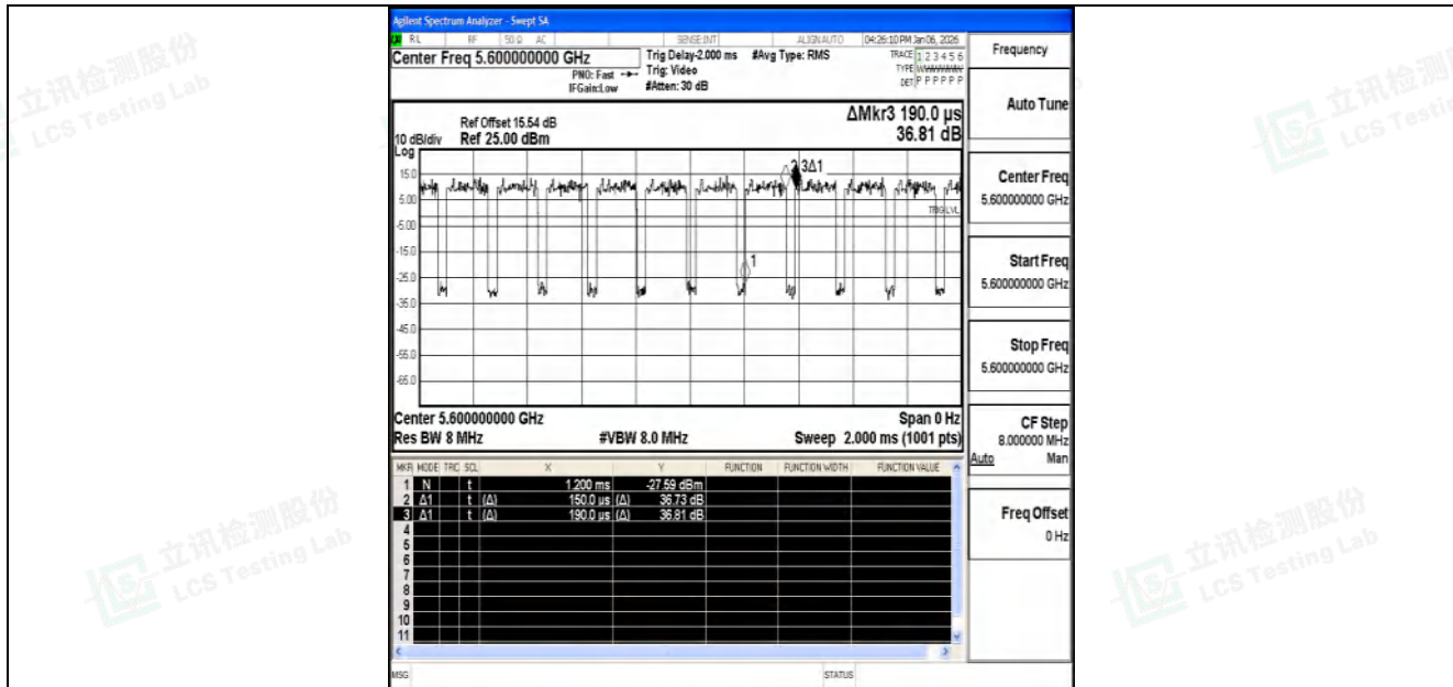
NTNV-11AC20SISO-Ant1-5600
