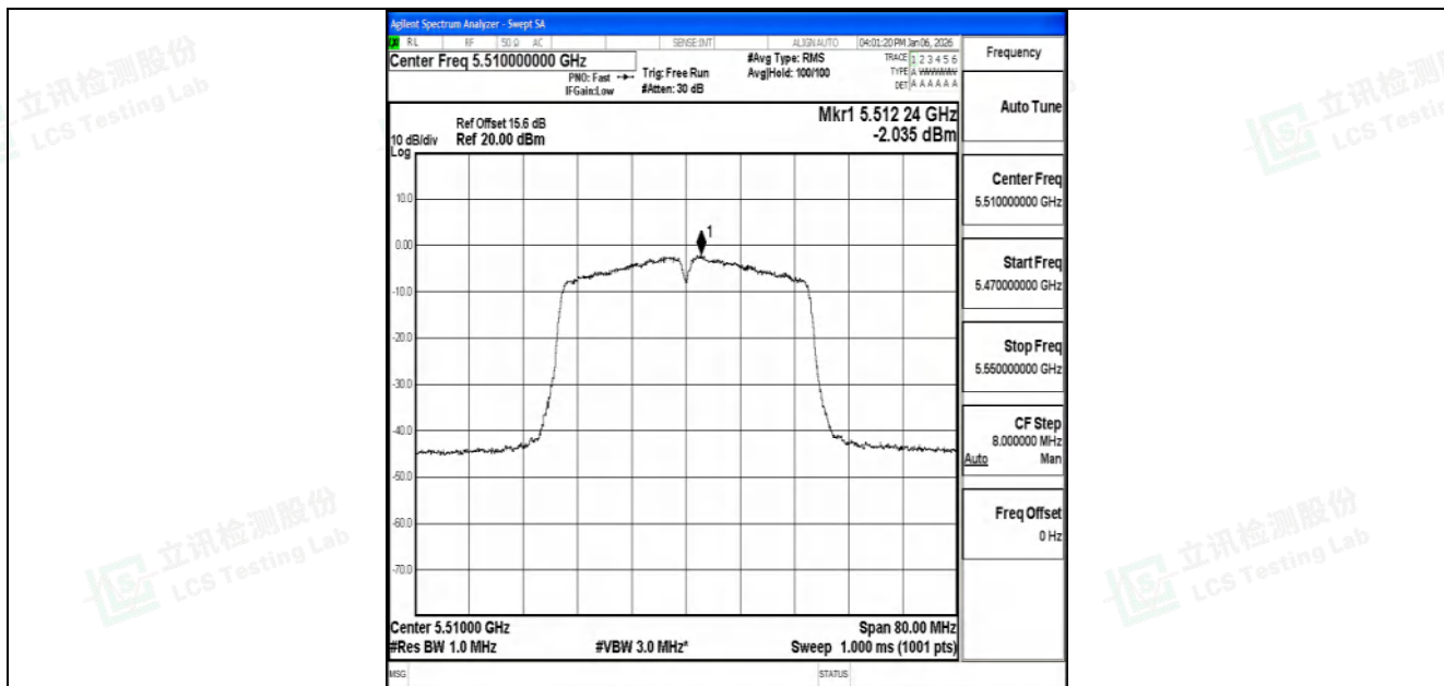
11N40SISO-Ant1-5510-PASS
