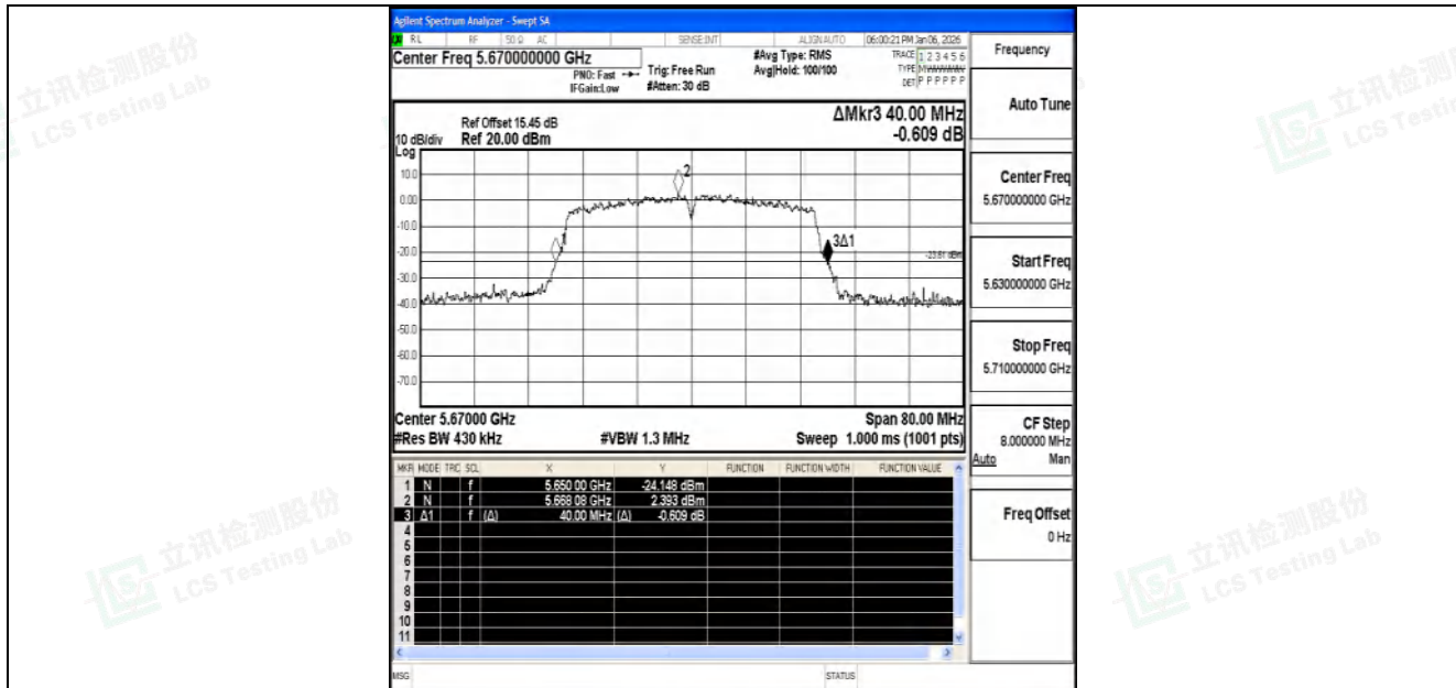
11N40SISO-Ant2-5670
