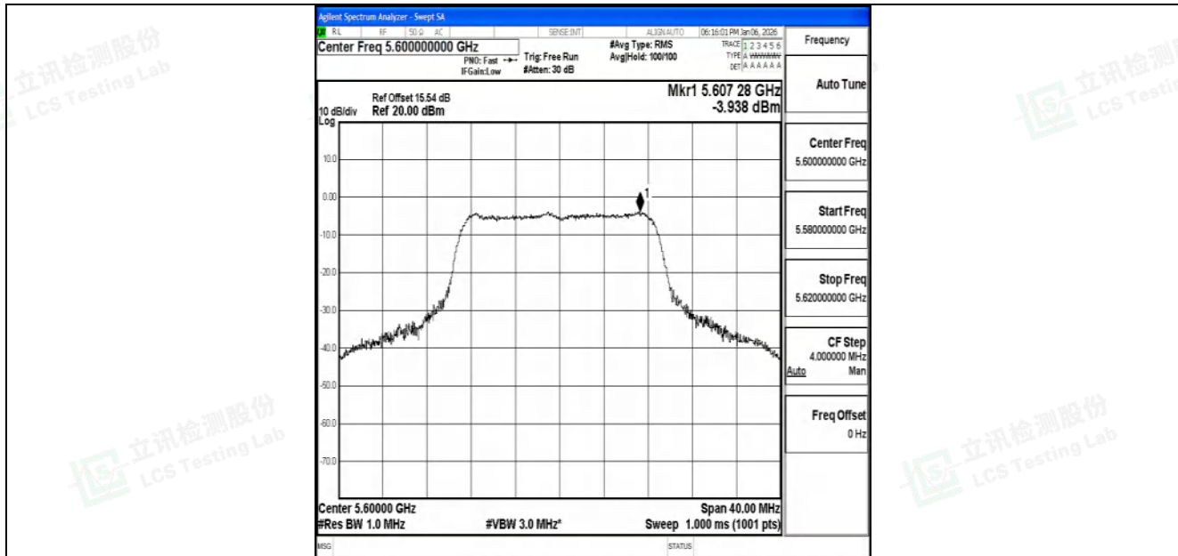
11AC20SISO-Ant2-5600-PASS
