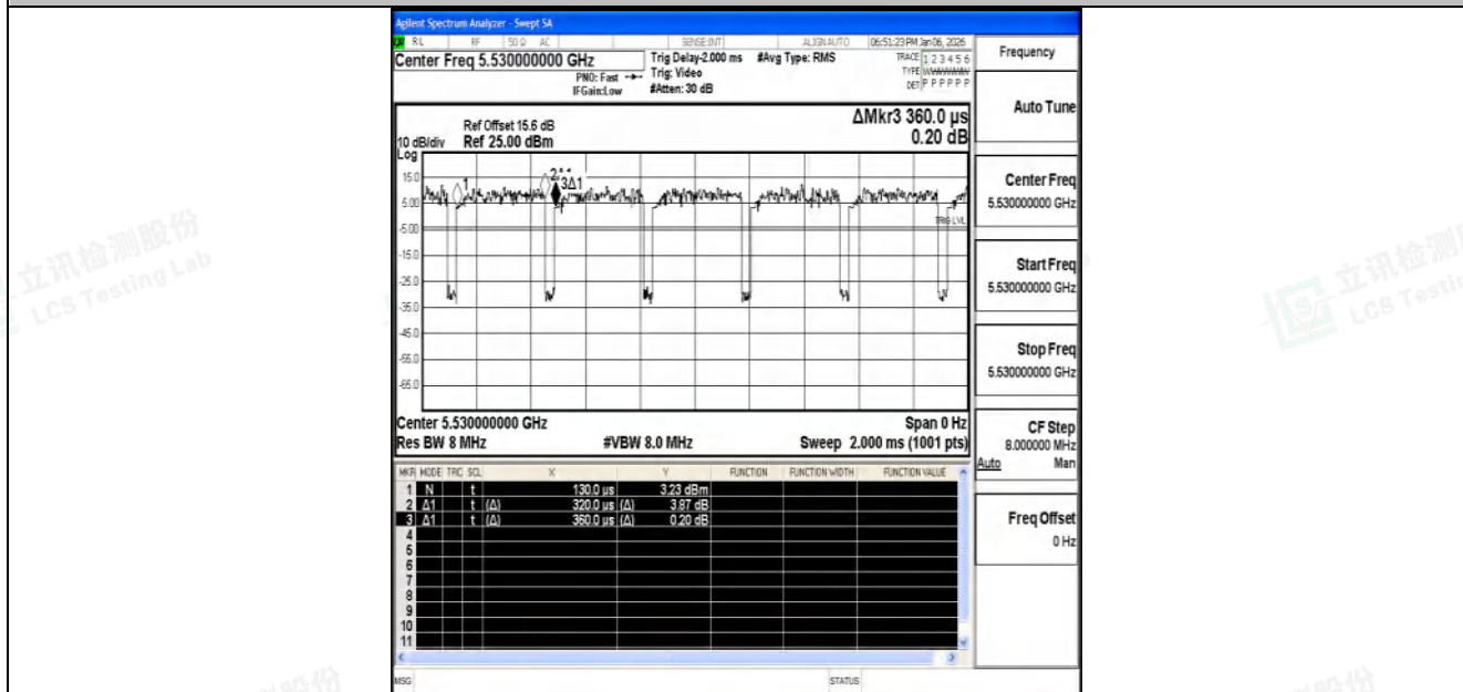
NTNV-11AC80SISO-Ant2-5530
