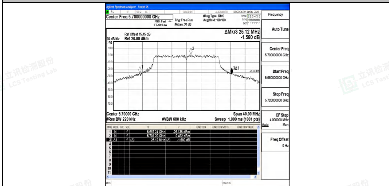
11AC20SISO-Ant2-5700
