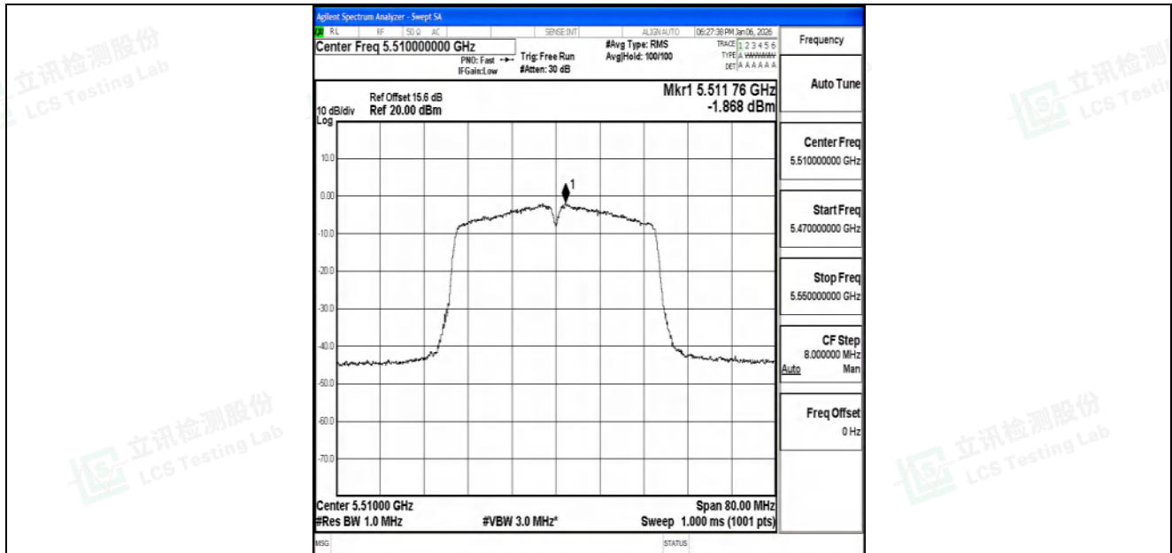
11AC40SISO-Ant2-5510-PASS
