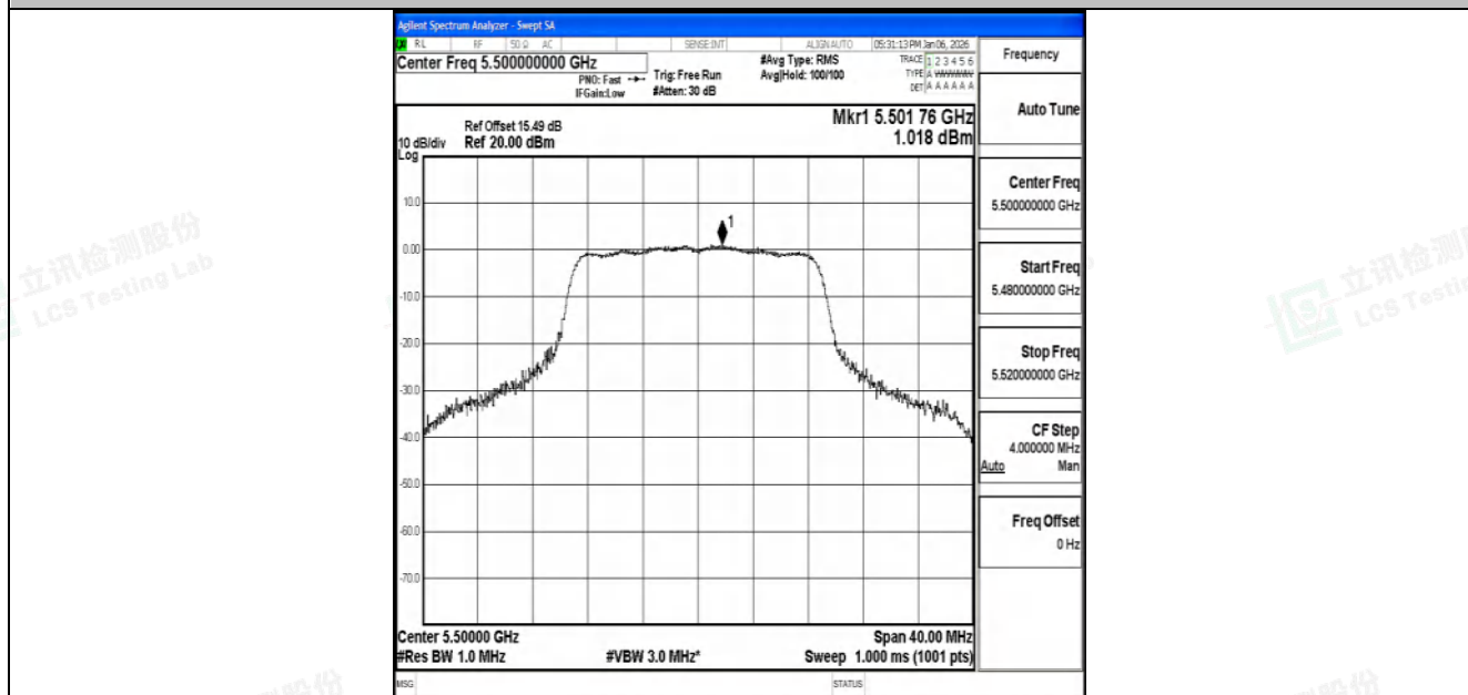
11N20SISO-Ant2-5500-PASS
