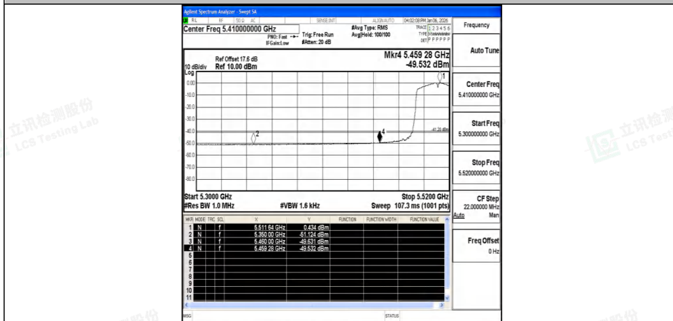
11N40SISO-Ant1-5510-PASS
