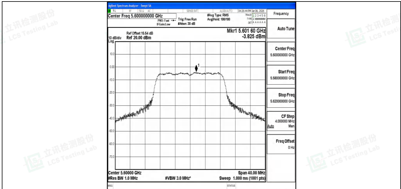
11AC20SISO-Ant1-5600-PASS
