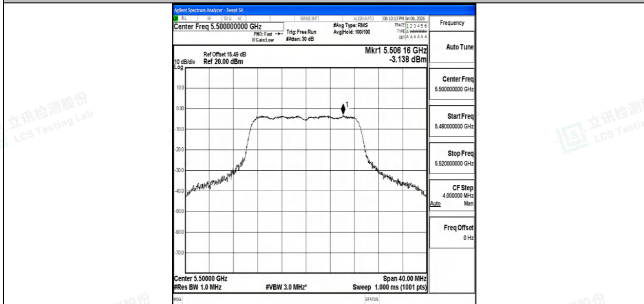
11AC20SISO-Ant2-5500-PASS
