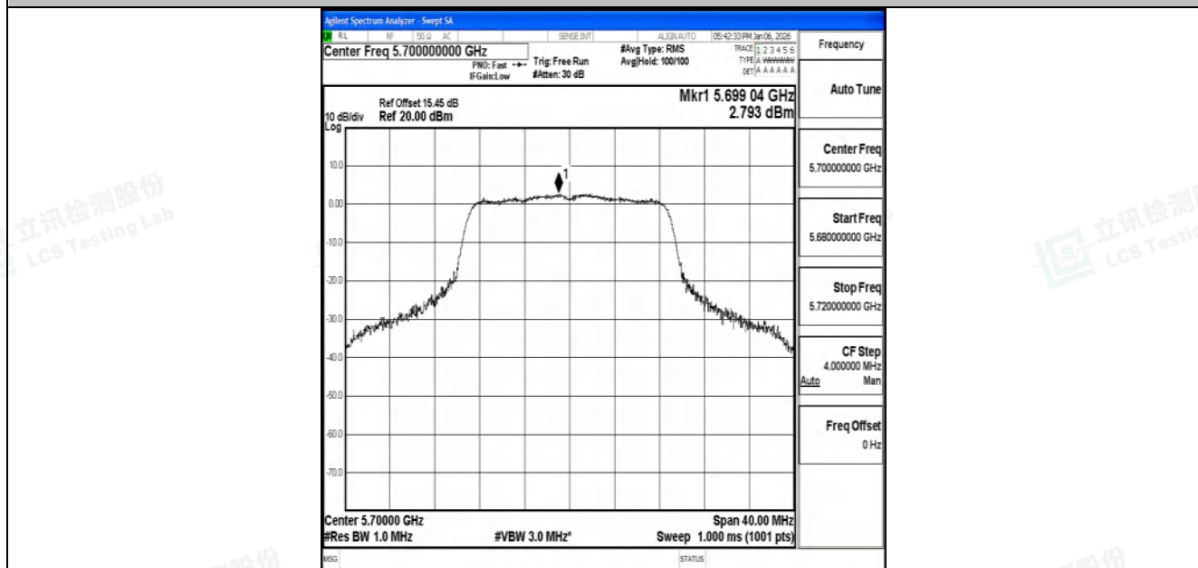
11N20SISO-Ant2-5700-PASS
