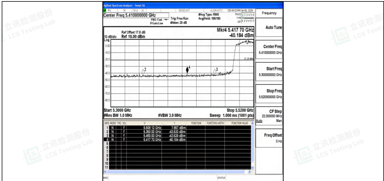
11N40SISO-Ant2-5510-PASS
