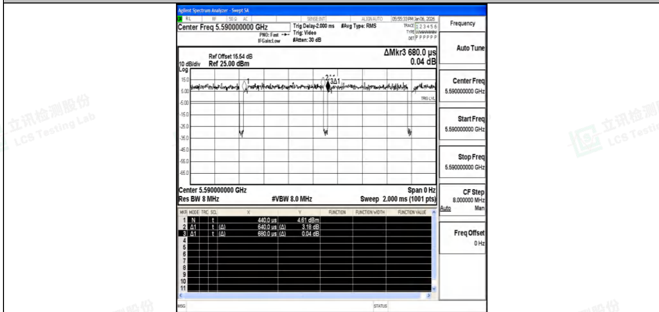
NTNV-11N40SISO-Ant2-5590
