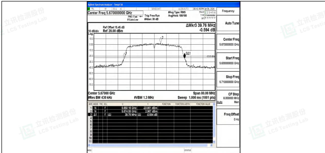
11AC40SISO-Ant2-5670
