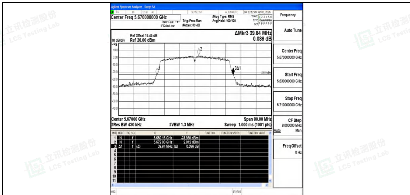
11N40SISO-Ant1-5670
