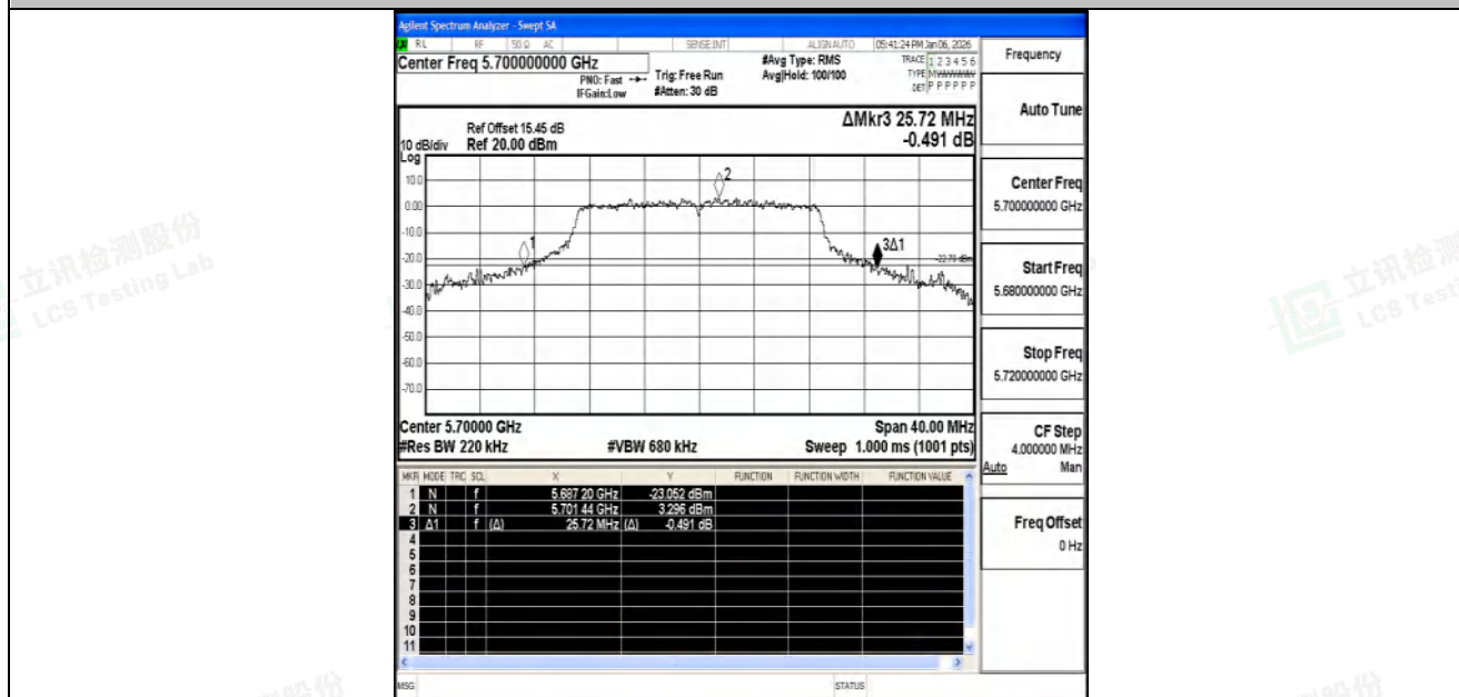
11N20SISO-Ant2-5700
