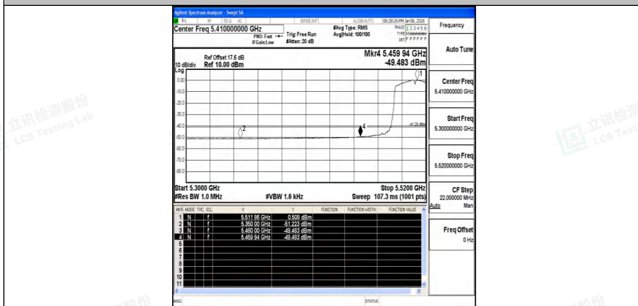
11AC40SISO-Ant2-5510-PASS
