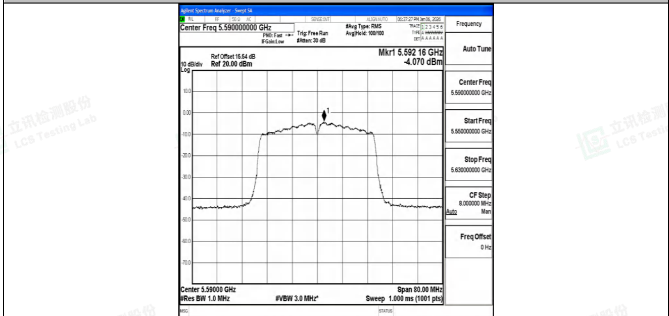
11AC40SISO-Ant2-5590-PASS
