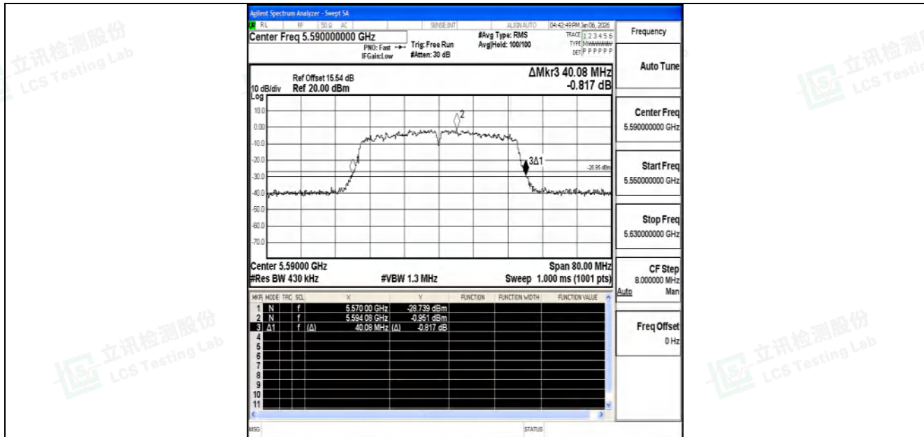
11AC40SISO-Ant1-5590
