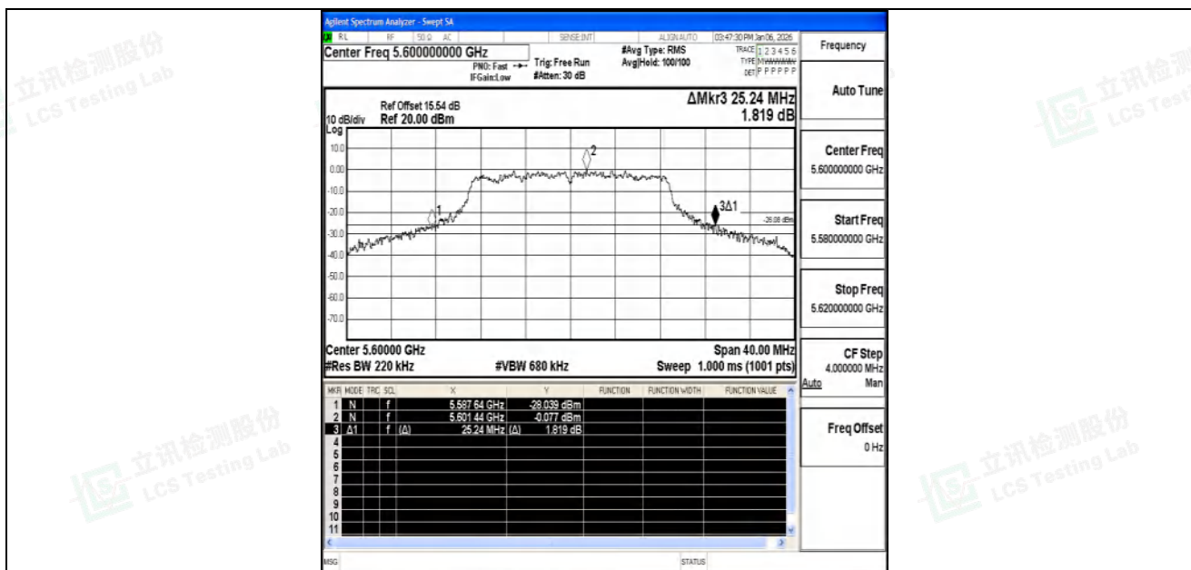
11N20SISO-Ant1-5600
