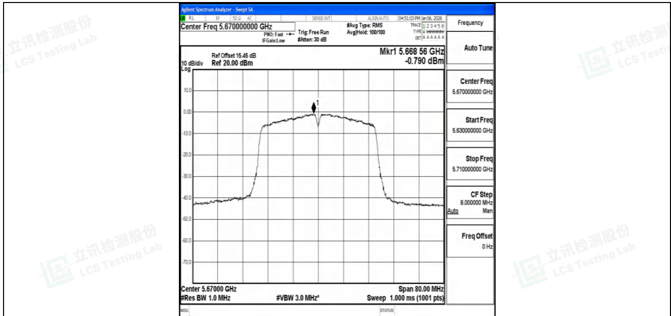
11AC40SISO-Ant1-5670-PASS
