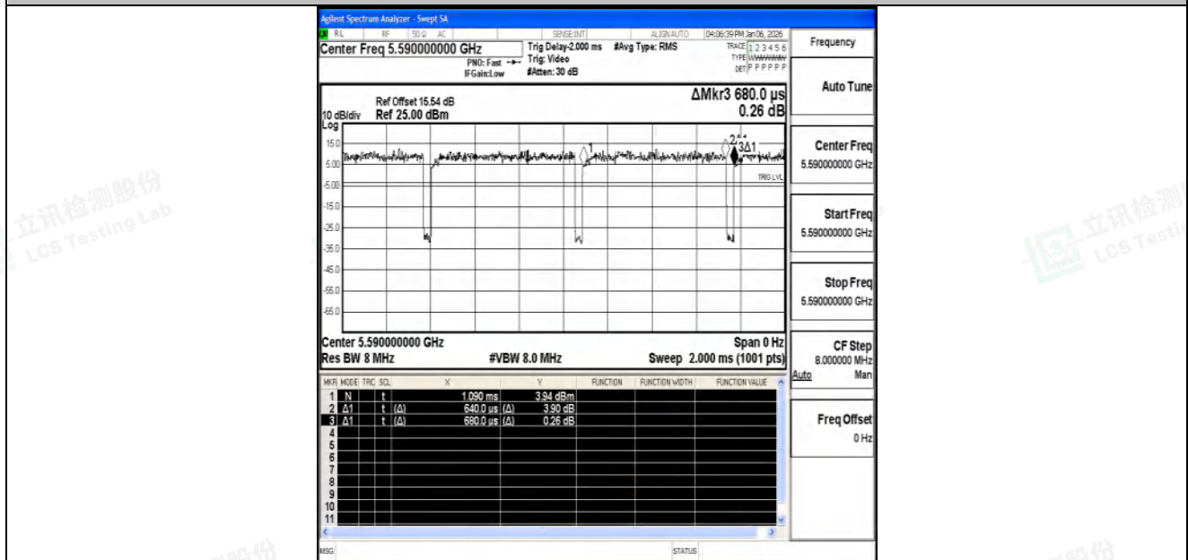
NTNV-11N40SISO-Ant1-5590
