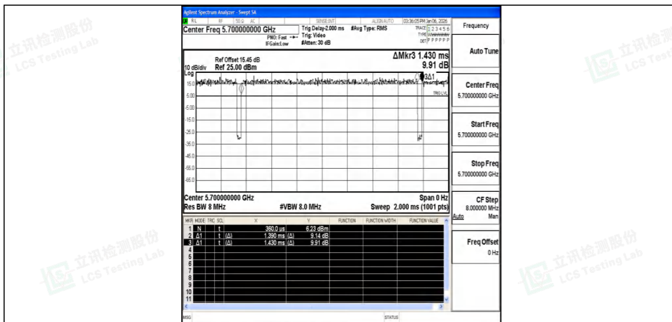
NTNV-11A-Ant1-5700
