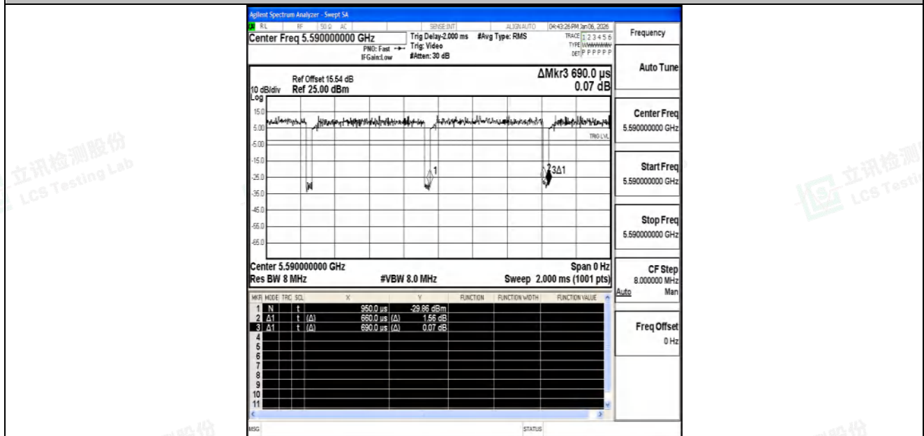
NTNV-11AC40SISO-Ant1-5590
