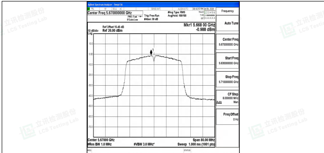
11AC40SISO-Ant2-5670-PASS
