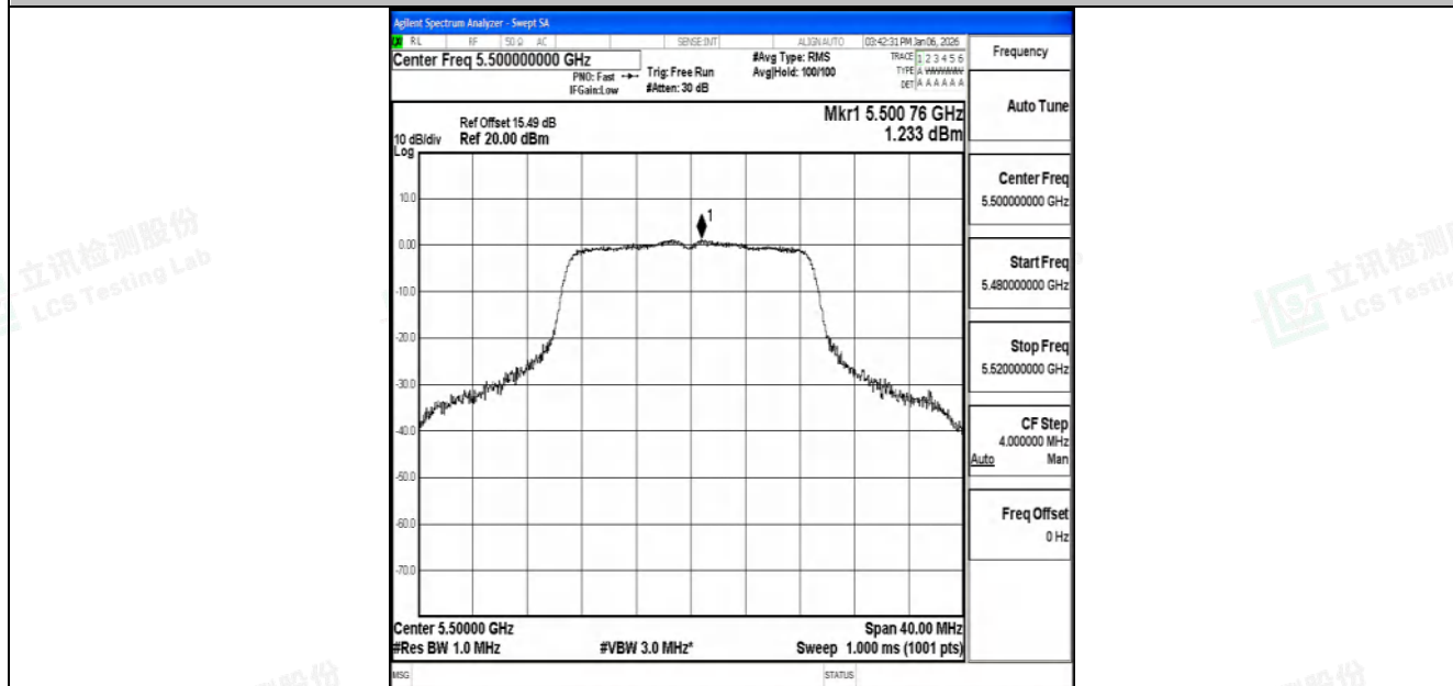
11N20SISO-Ant1-5500-PASS
