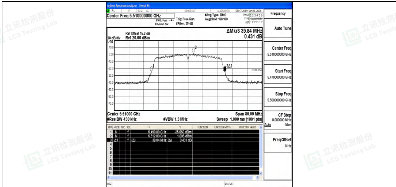
11N40SISO-Ant2-5510
