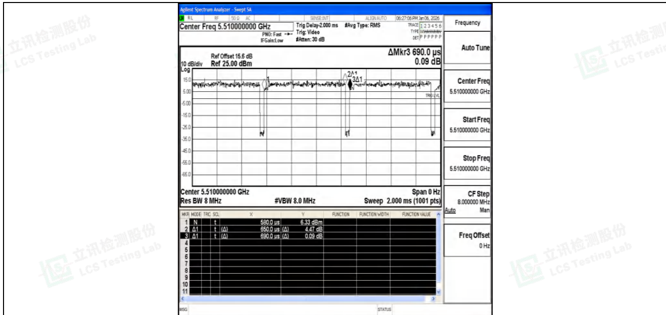
NTNV-11AC40SISO-Ant2-5510
