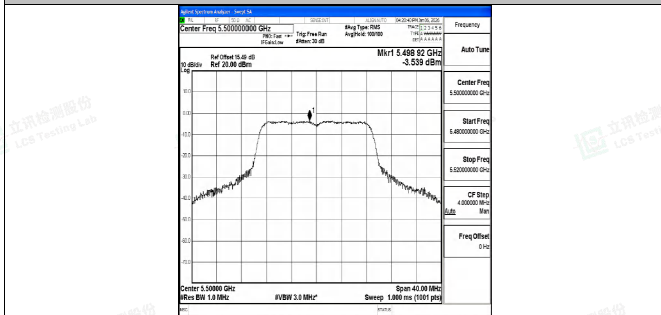
11AC20SISO-Ant1-5500-PASS
