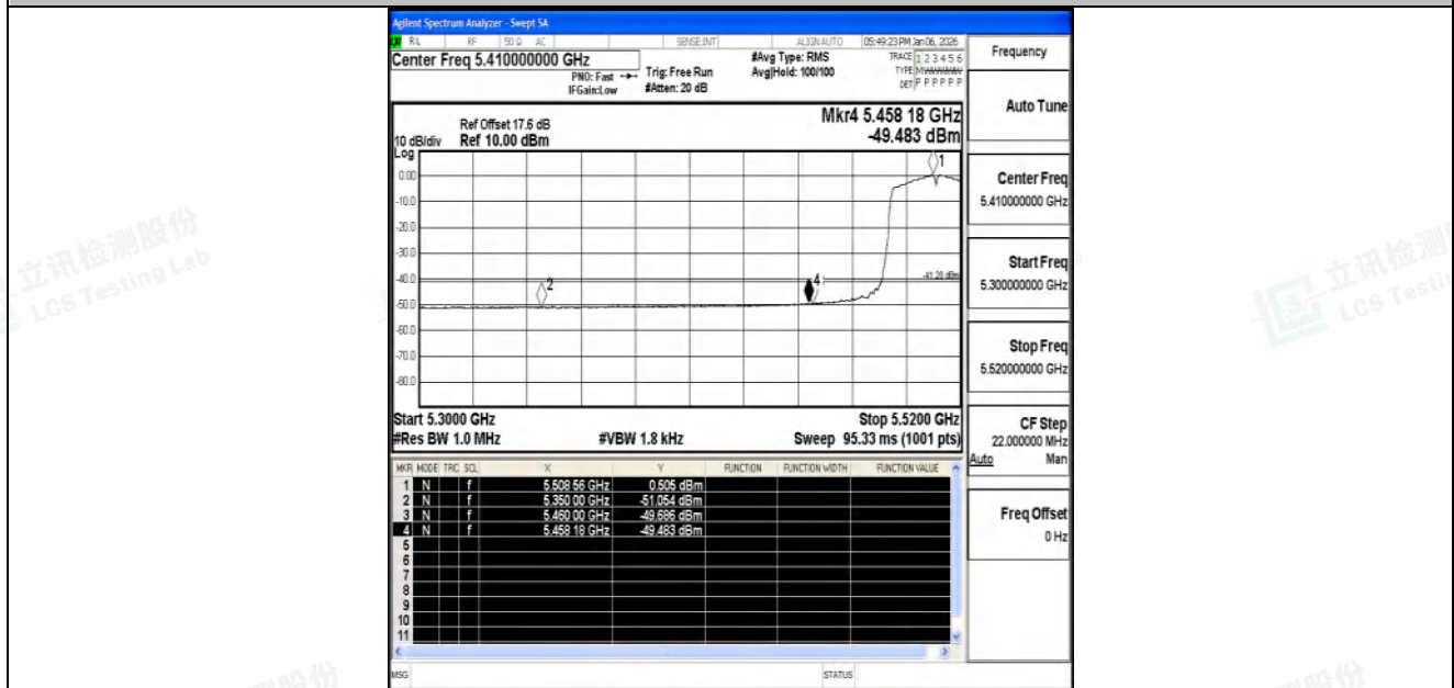
11N40SISO-Ant2-5510-PASS
