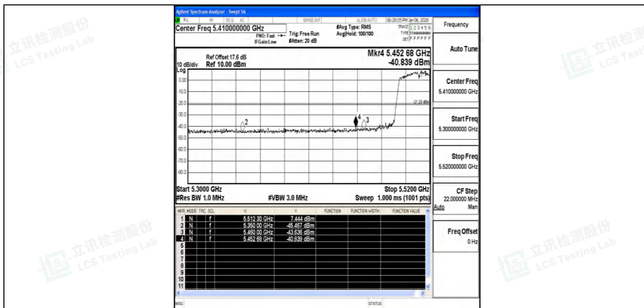
11AC40SISO-Ant2-5510-PASS
