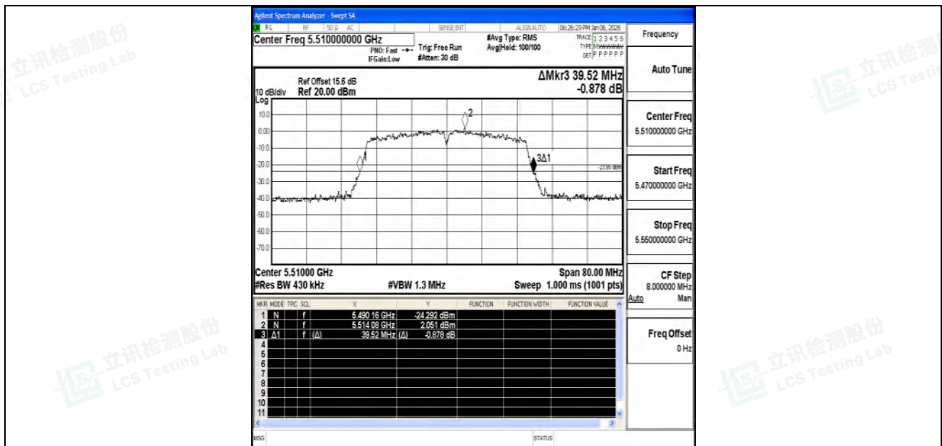
11AC40SISO-Ant2-5510
