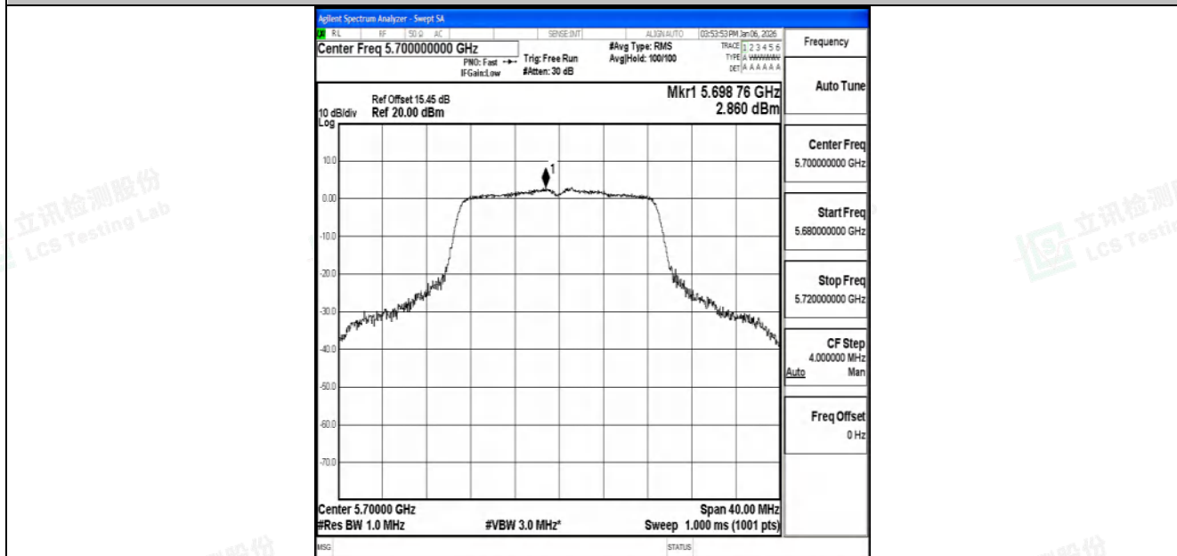
11N20SISO-Ant1-5700-PASS
