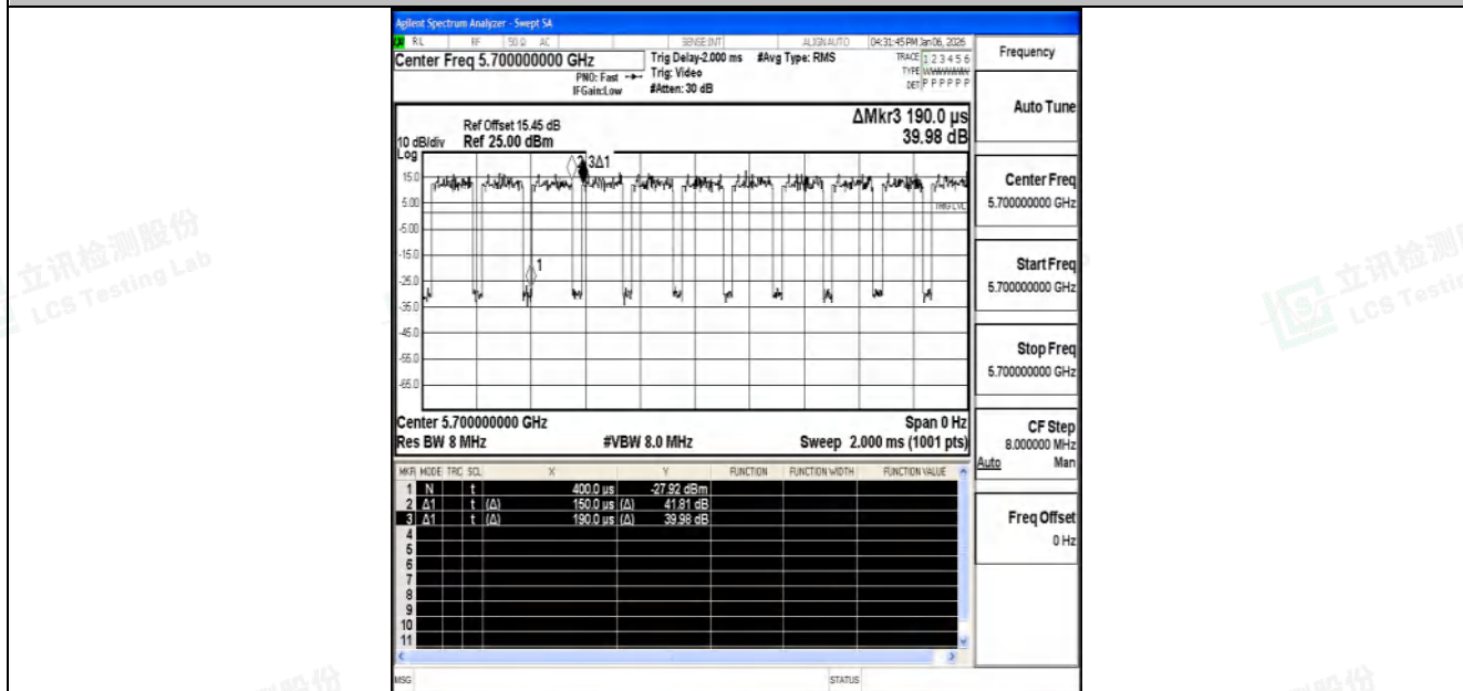
NTNV-11AC20SISO-Ant1-5700
