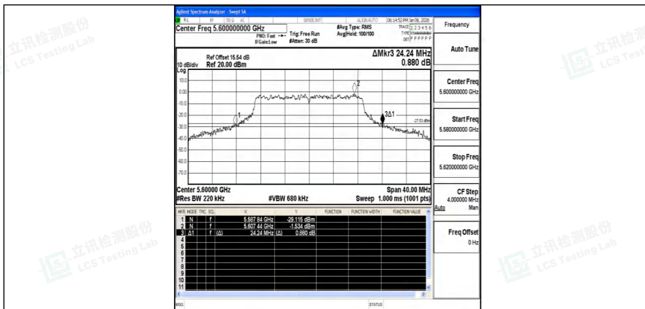
11AC20SISO-Ant2-5600
