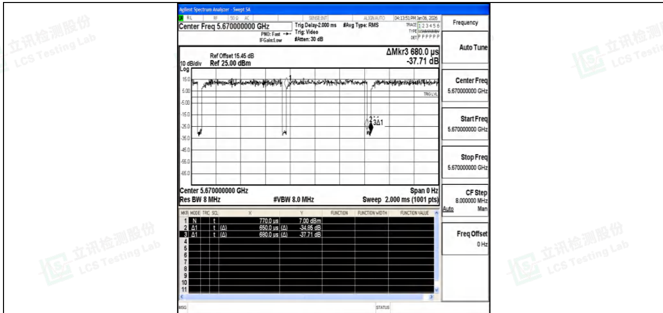
NTNV-11N40SISO-Ant1-5670
