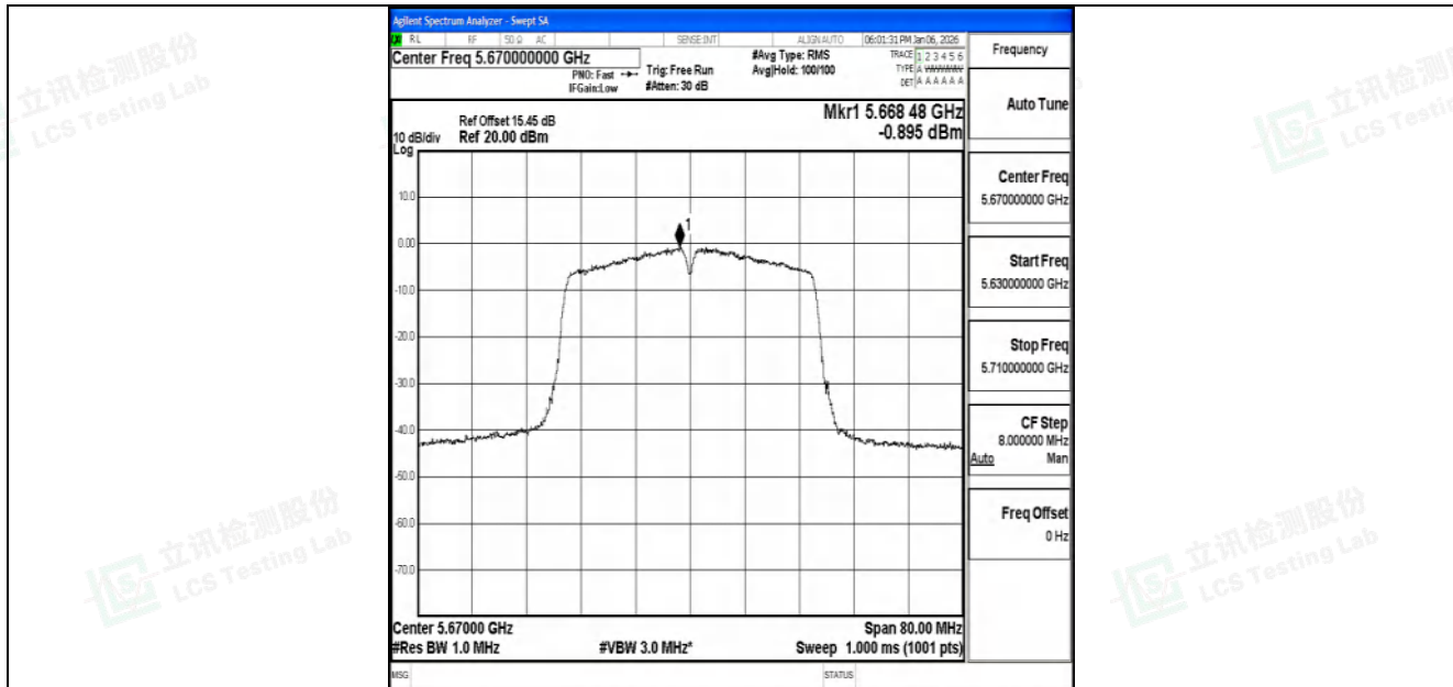
11N40SISO-Ant2-5670-PASS
