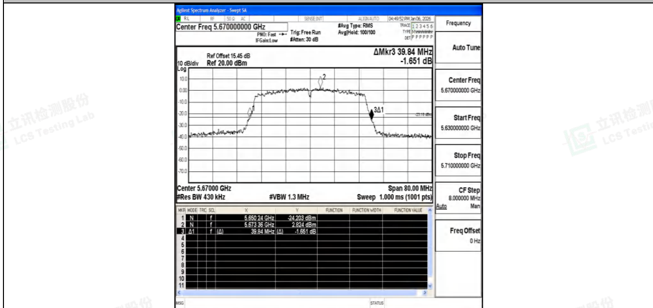
11AC40SISO-Ant1-5670
