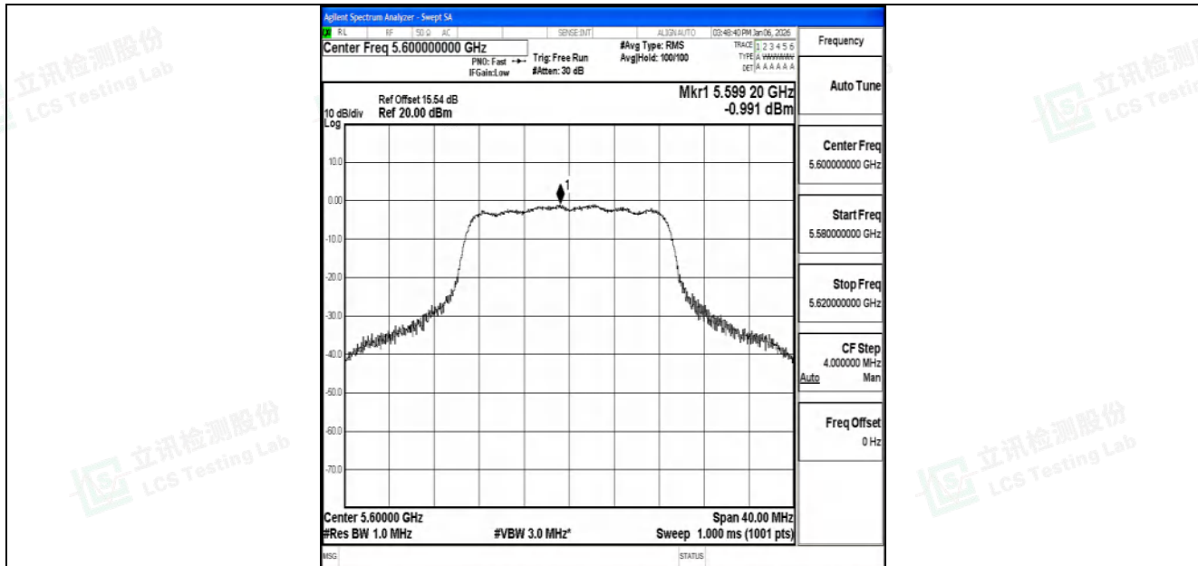
11N20SISO-Ant1-5600-PASS
