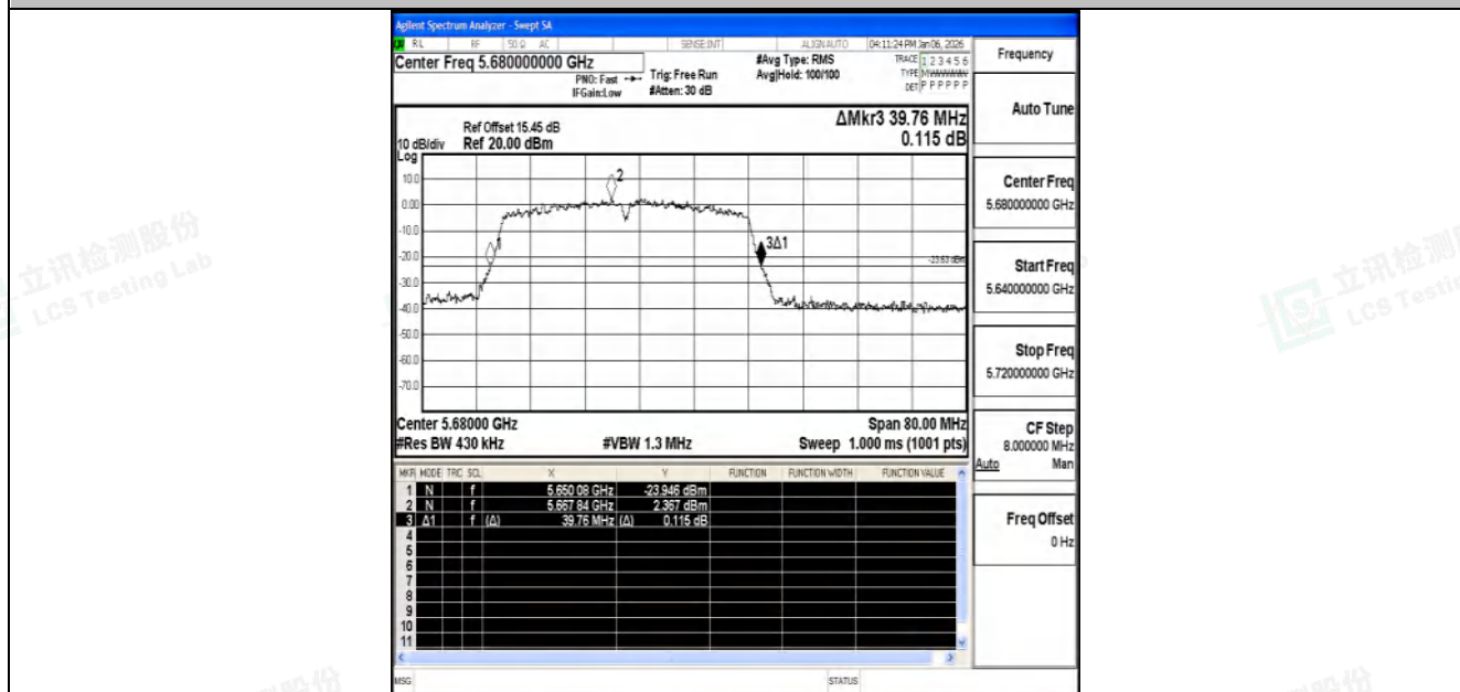
11N40SISO-Ant1-5680
