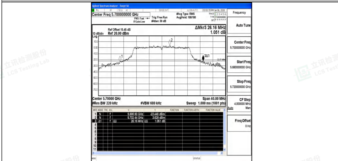
11N20SISO-Ant1-5700
