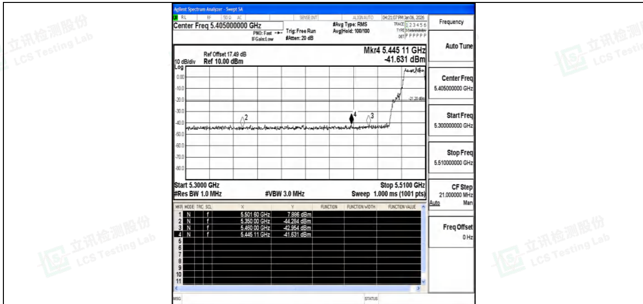
11AC20SISO-Ant1-5500-PASS
