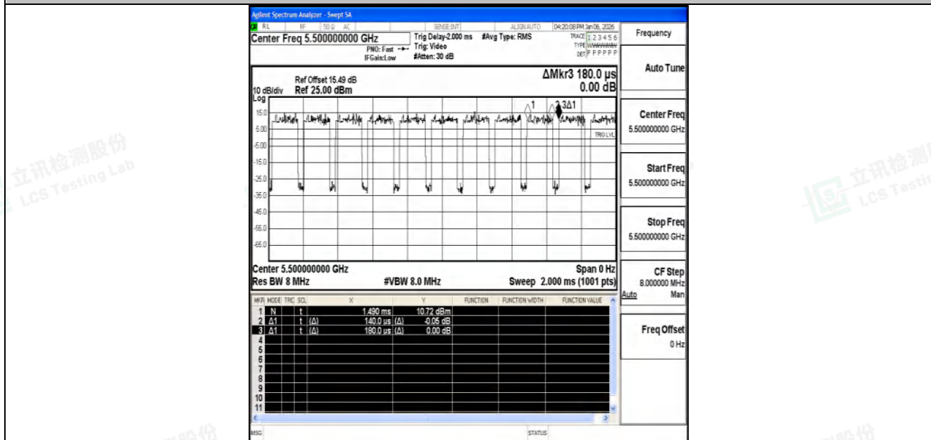
NTNV-11AC20SISO-Ant1-5500
