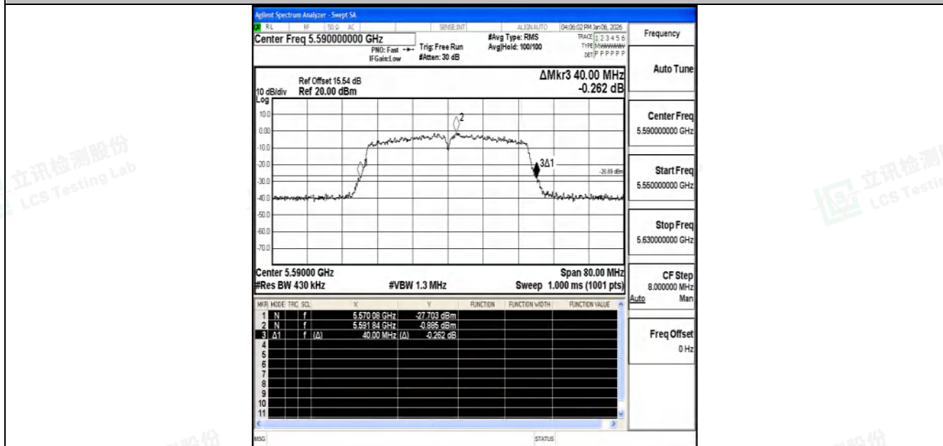
11N40SISO-Ant1-5590
