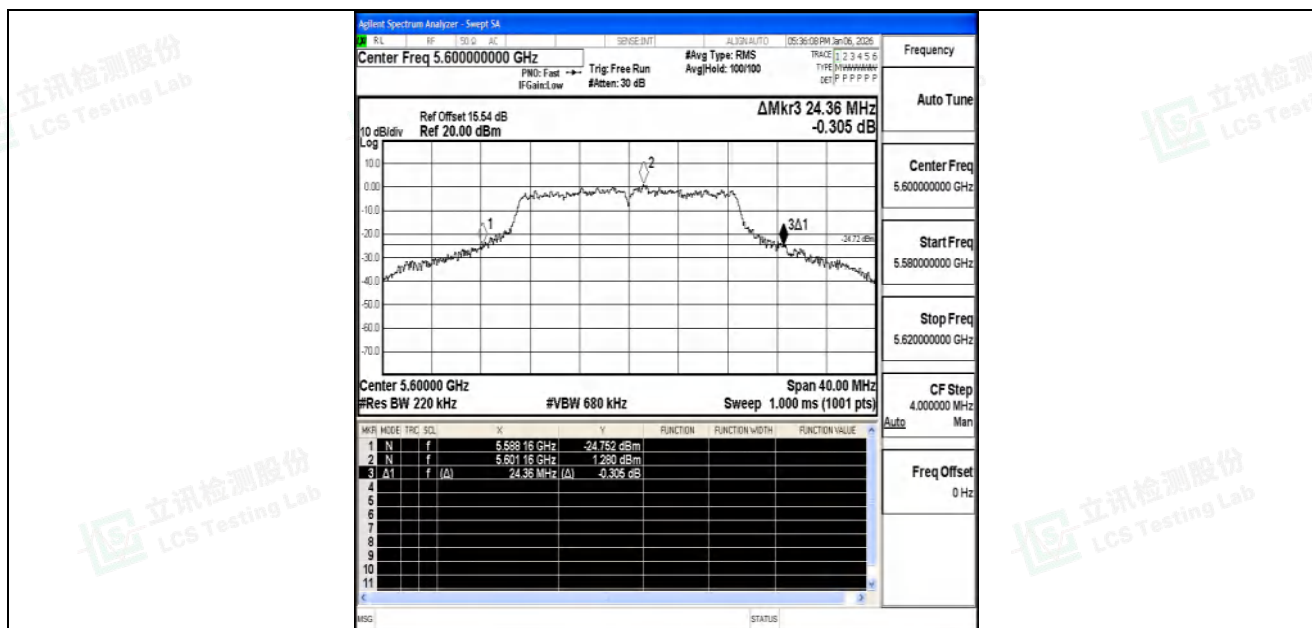
11N20SISO-Ant2-5600
