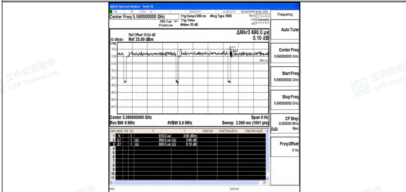
NTNV-11AC40SISO-Ant2-5590
