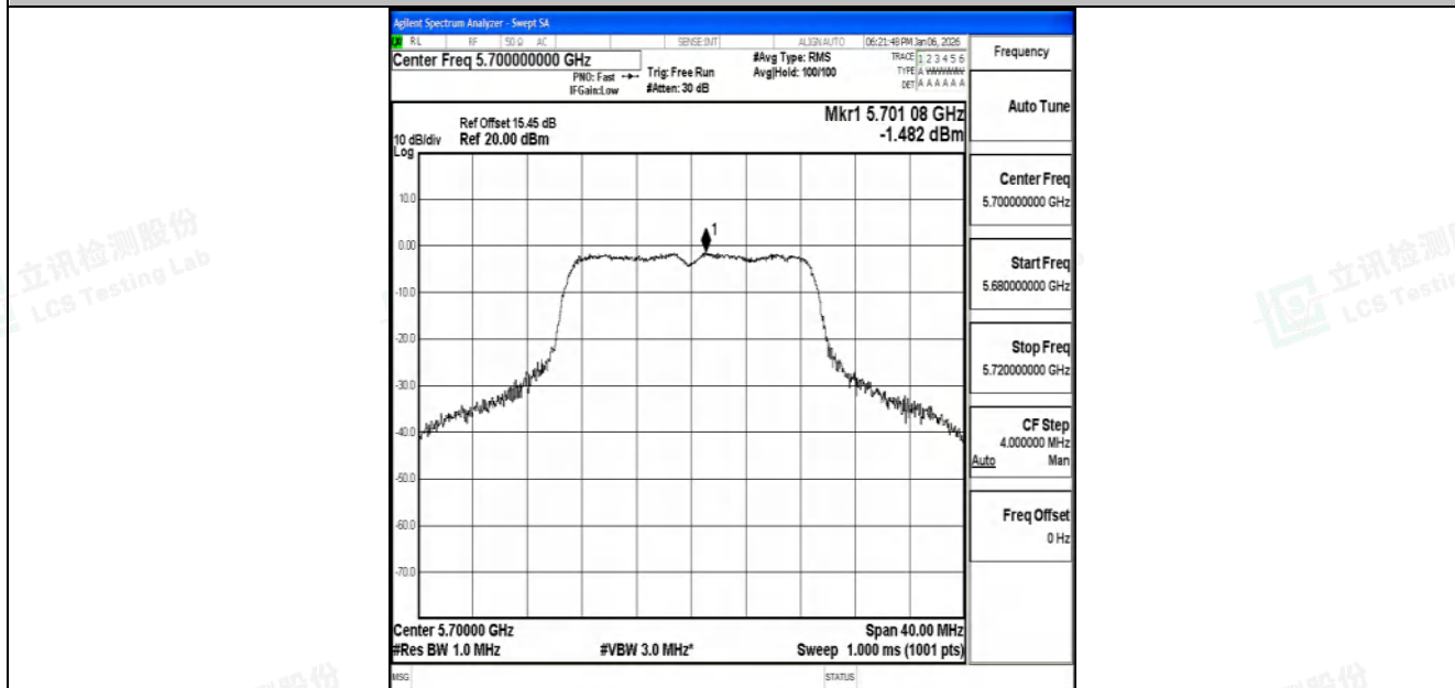
11AC20SISO-Ant2-5700-PASS
