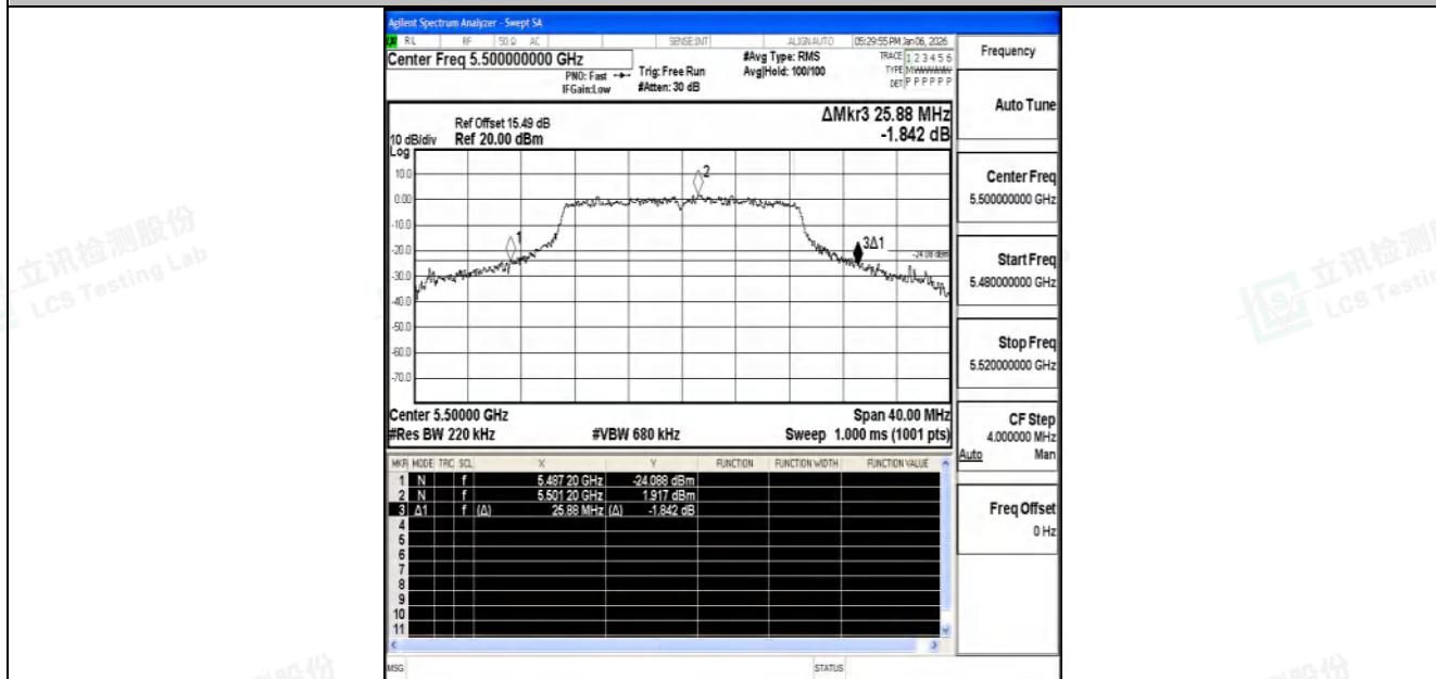
11N20ISO-Ant2-5500
