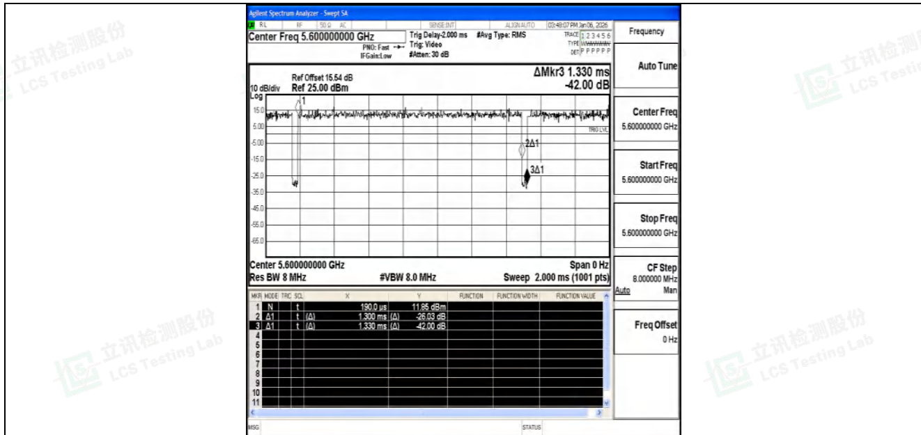
NTNV-11N20SISO-Ant1-5600
