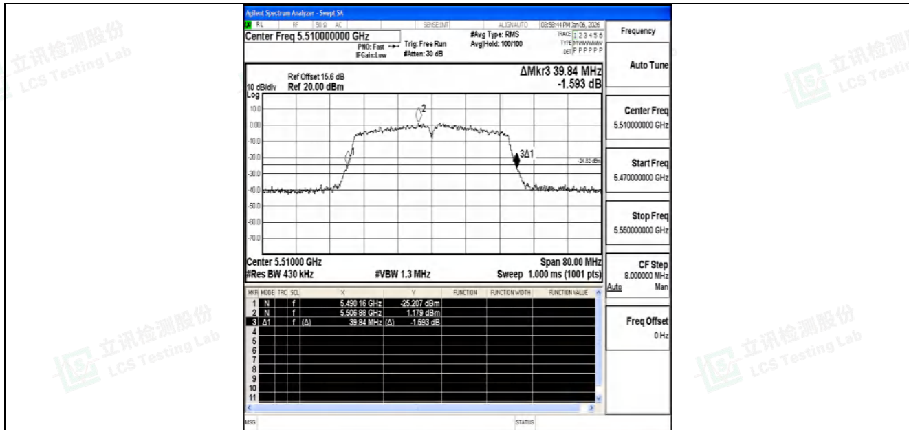
11N40SISO-Ant1-5510
