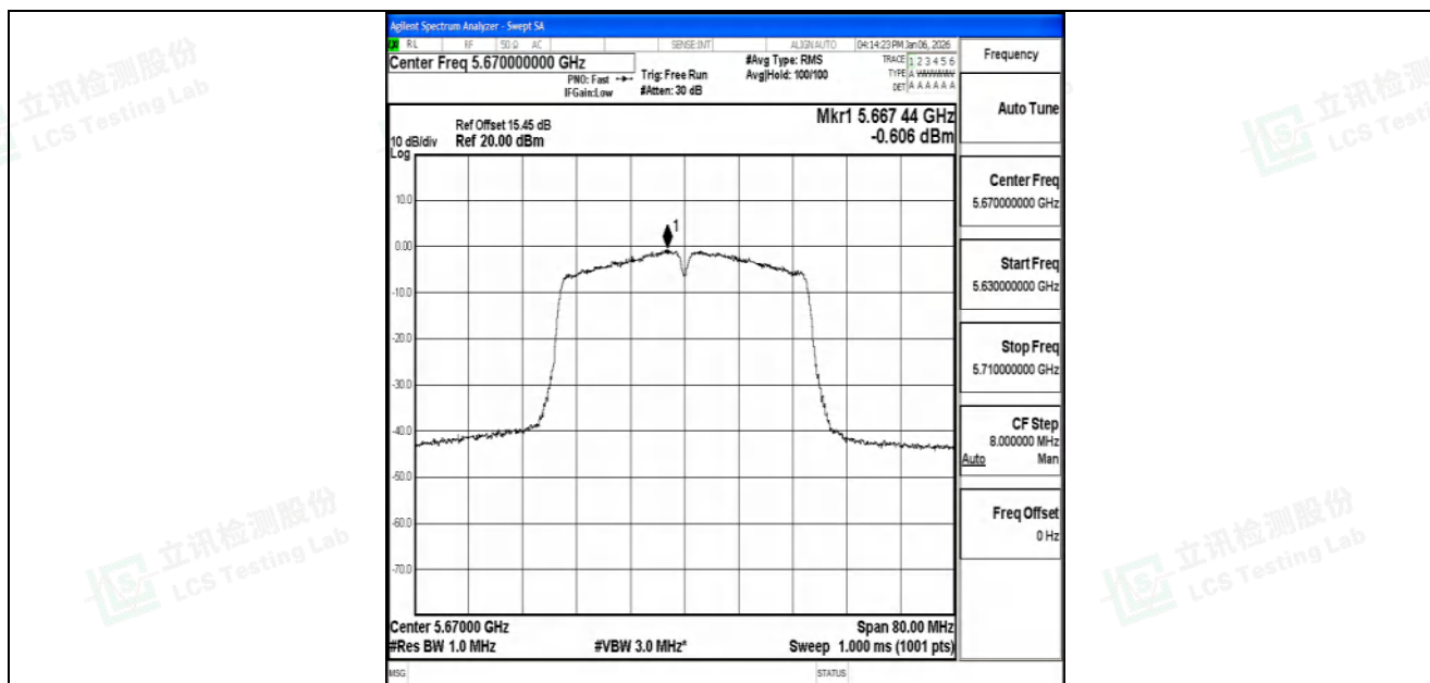
11N40SISO-Ant1-5670-PASS
