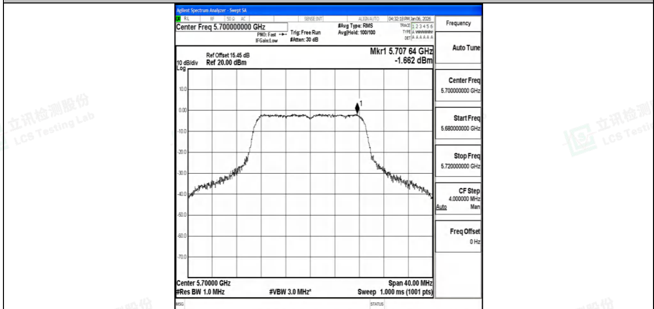
11AC20SISO-Ant1-5700-PASS
