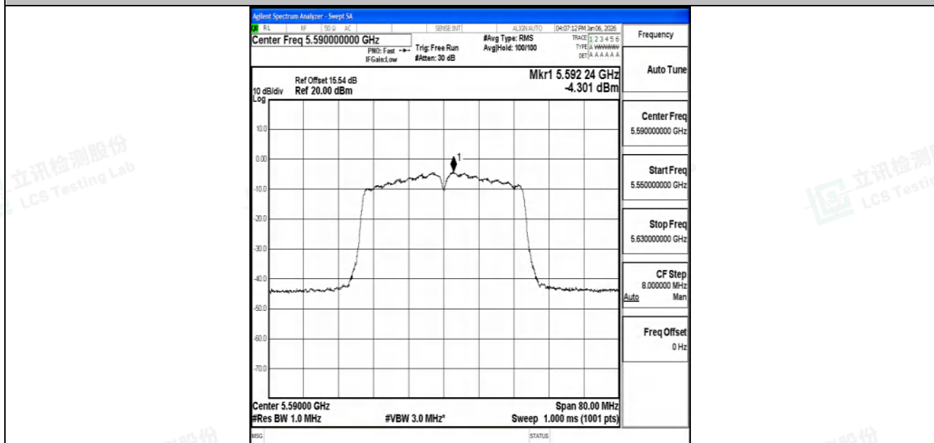
11N40SISO-Ant1-5590-PASS
