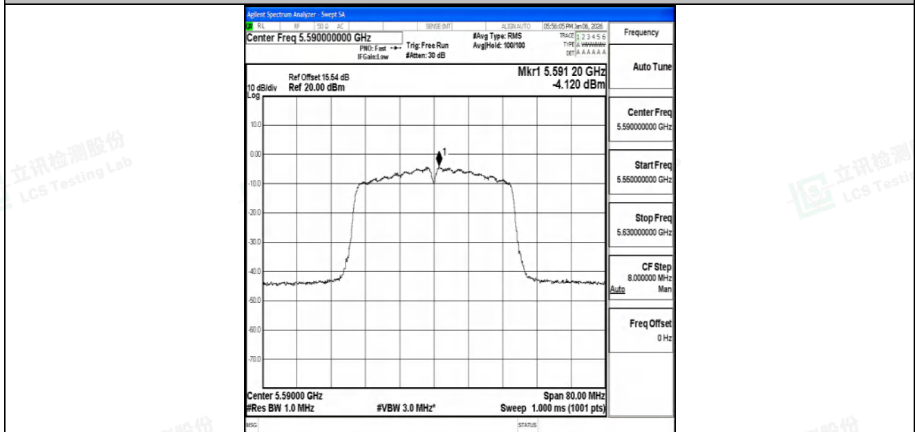
11N40SISO-Ant2-5590-PASS
