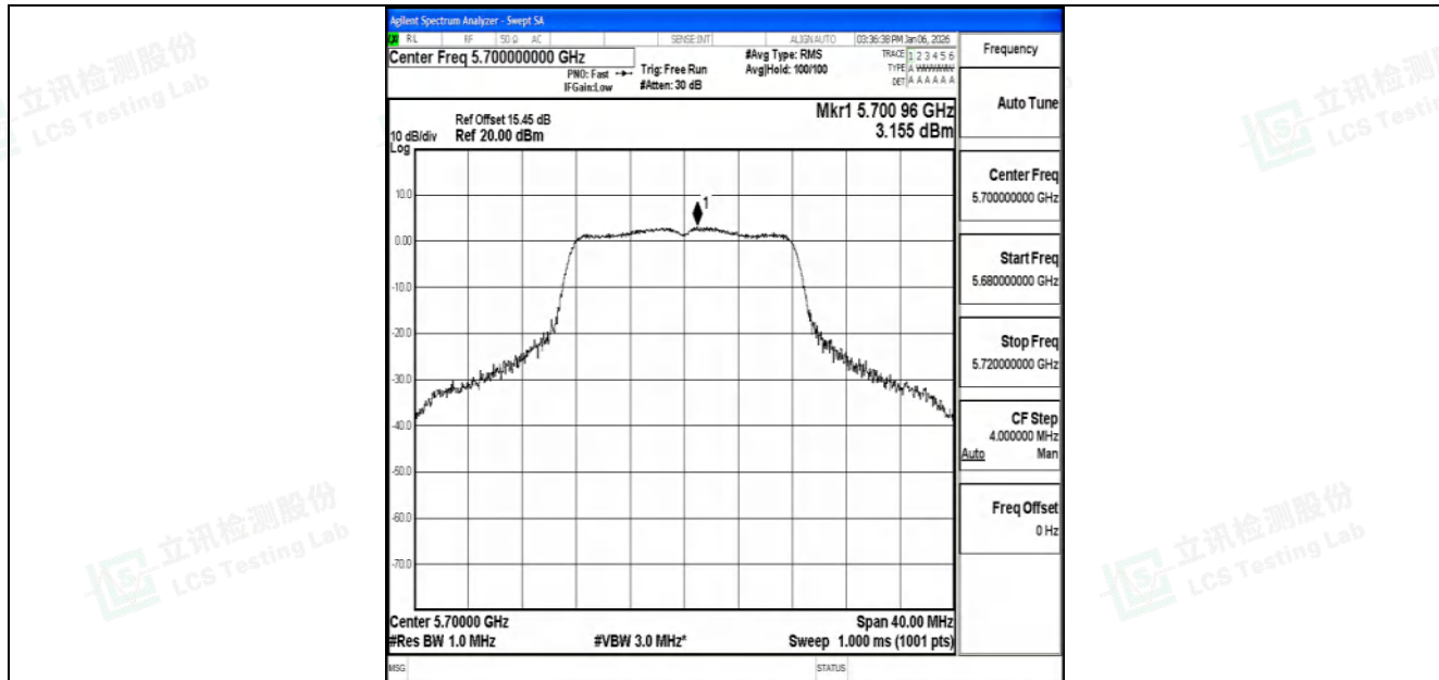
11A-Ant1-5700-PASS
