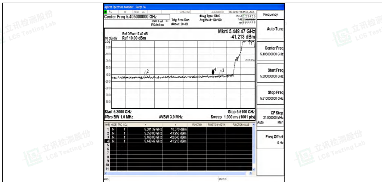
11N20SISO-Ant2-5500-PASS
