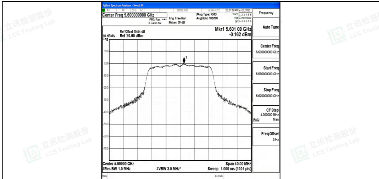
11N20SISO-Ant2-5600-PASS
