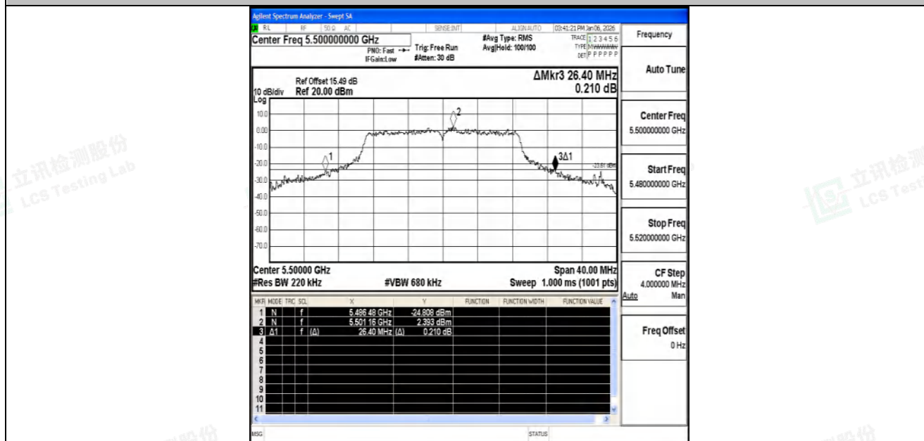
11N20SISO-Ant1-5500
