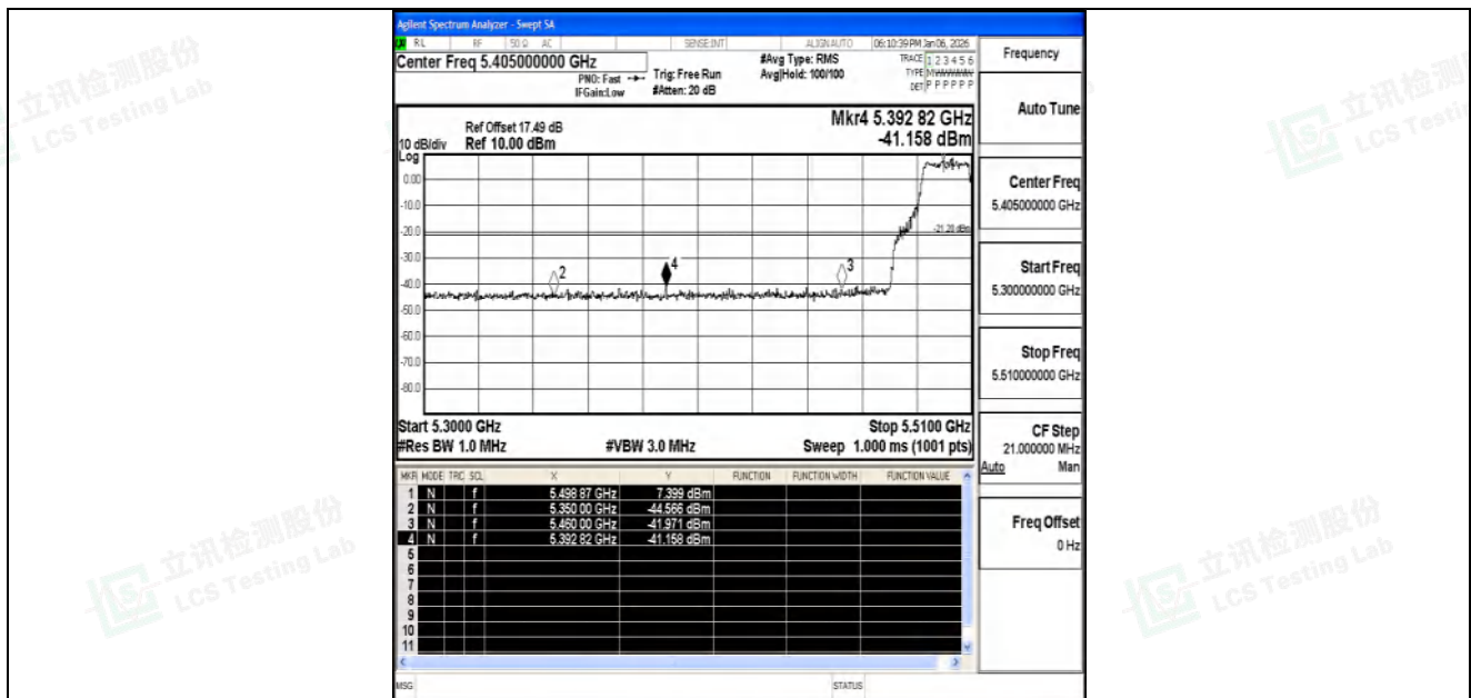
11AC20SISO-Ant2-5500-PASS
