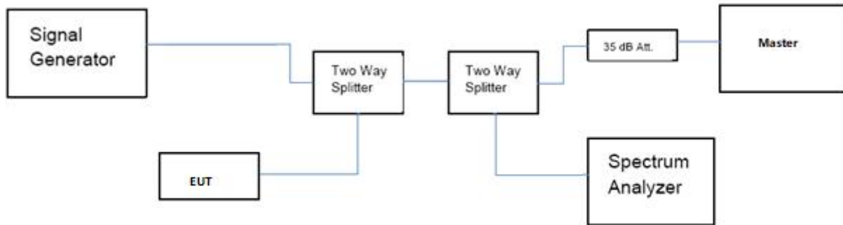
Figure 3-1 Test Setup for Conducted Measurement
