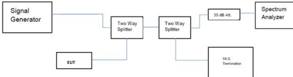
Figure 3-2 Test Setup for Conducted Measurement Radar Verification
