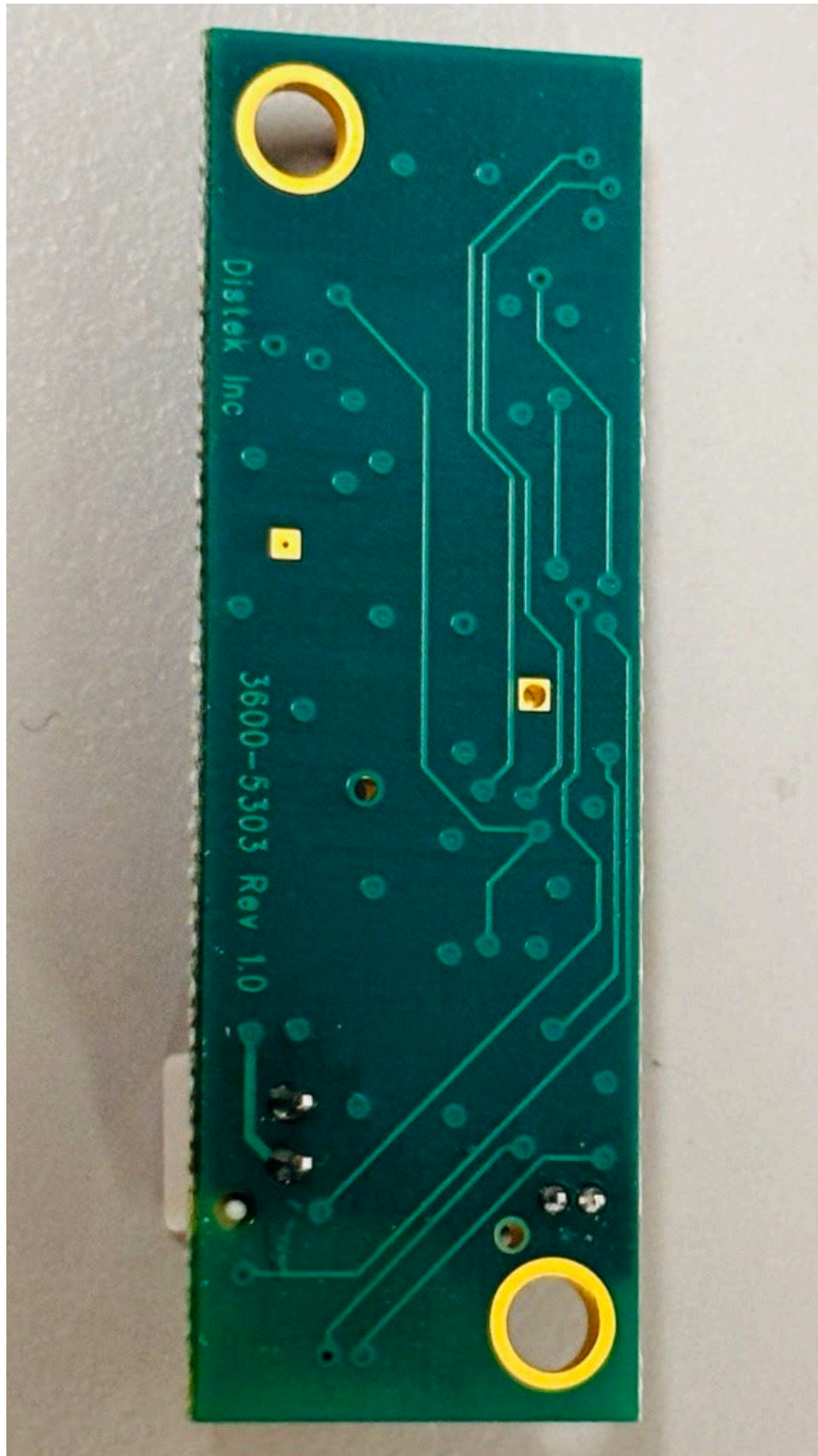
Shaft Board Back Side Detail
