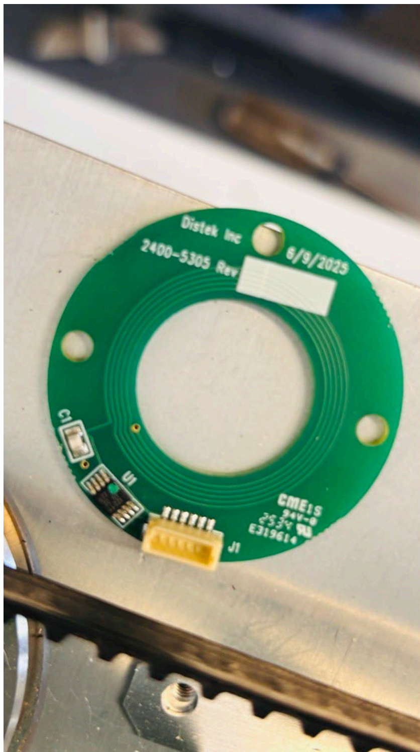
Shaft Antenna Board Component Side Detail
